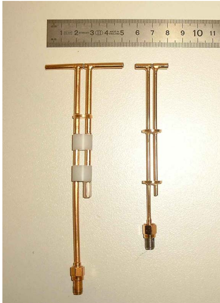
Photo 1: validation dipoles
