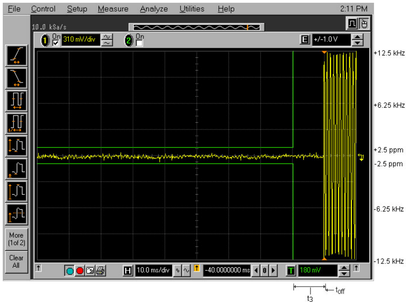
Plot 5.13.4.6. Transient Frequency Behavior Carrier Frequency: 406.3 MHz; Channel Spacing: 12.5 kHz; Power: 10 W Description: Switch off condition t_3 , t_{off}
