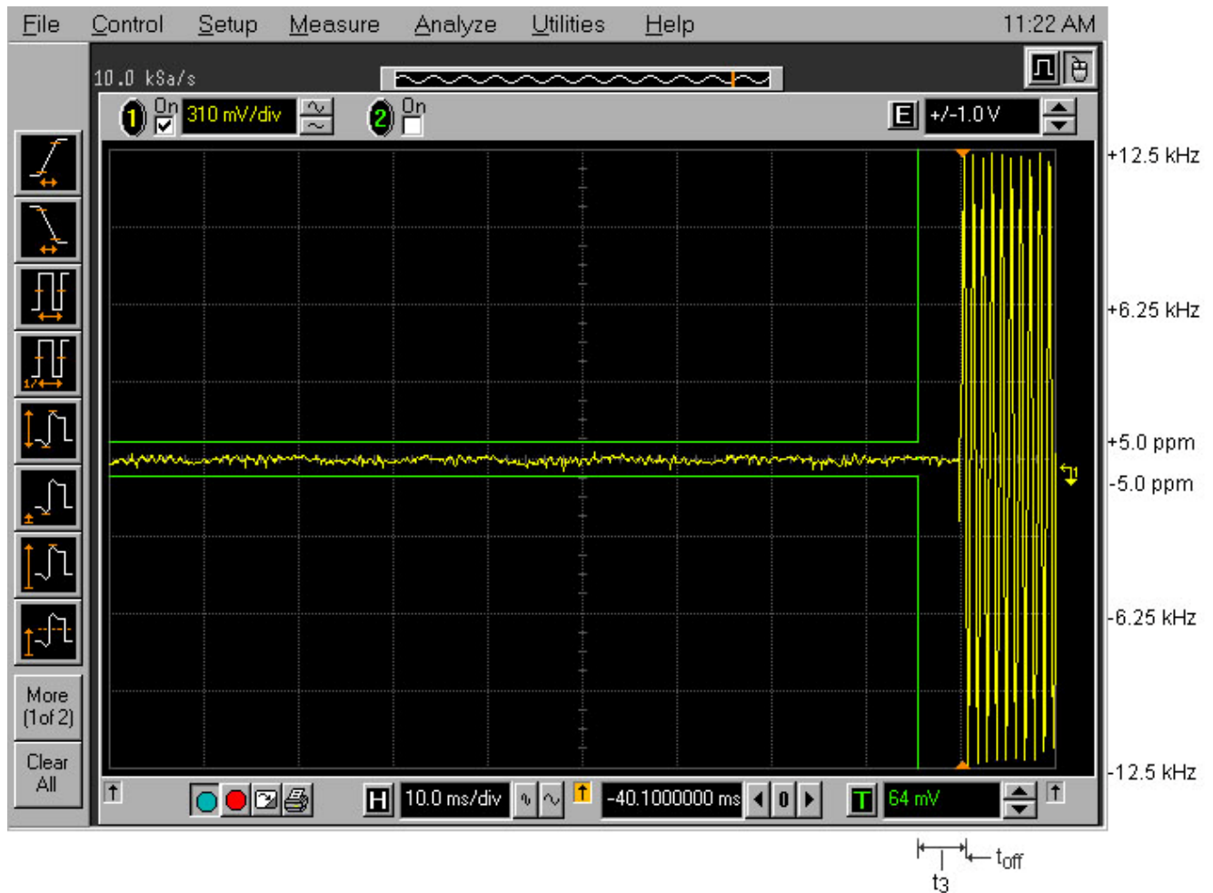
Plot 5.13.4.2. Transient Frequency Behavior Carrier Frequency: 138.1 MHz; Channel Spacing: 12.5 kHz; Power: 10 W Description: Switch off condition t_3 , t_{off}
