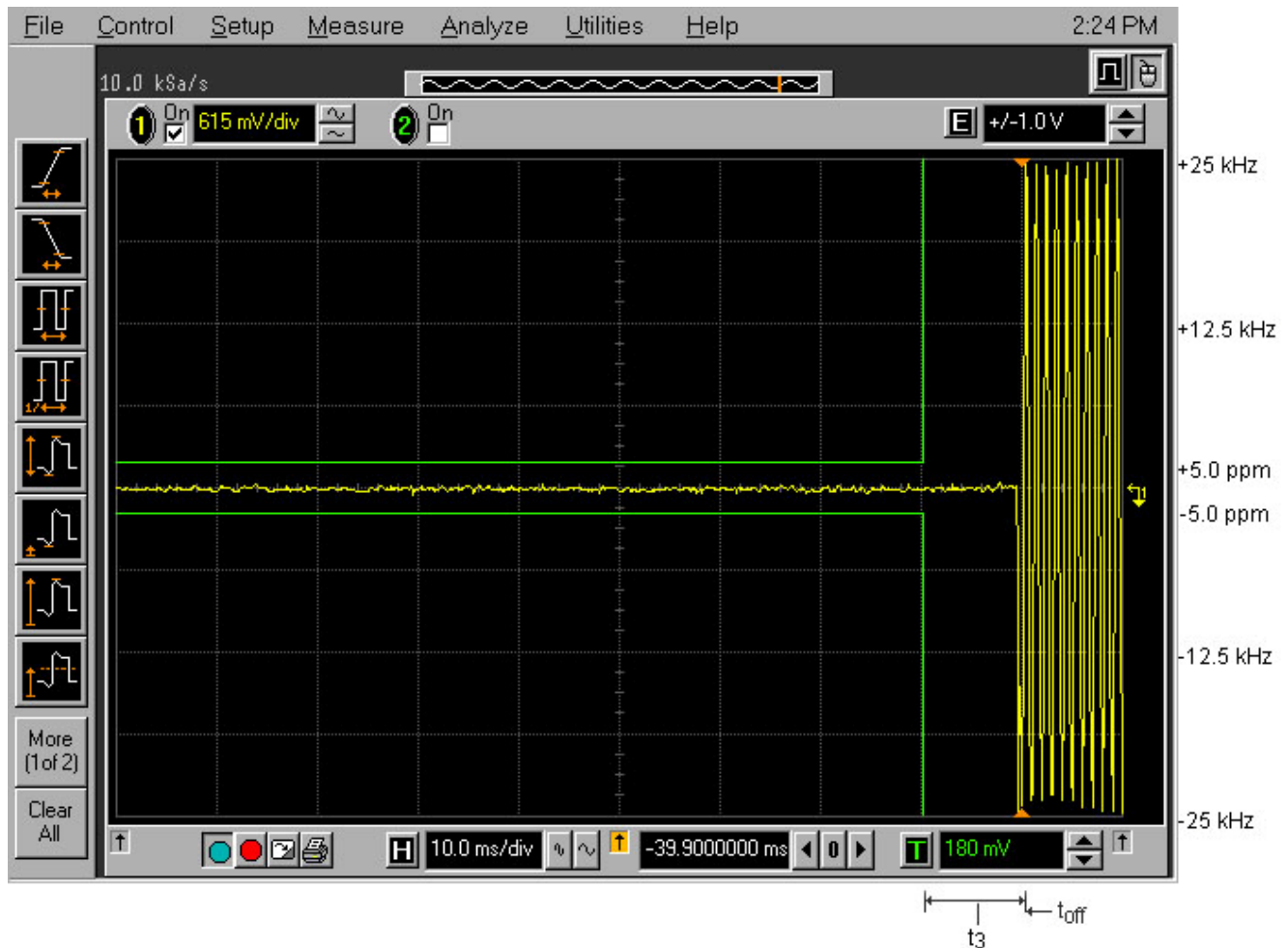
Plot 5.13.4.8. Transient Frequency Behavior Carrier Frequency: 406.3 MHz; Channel Spacing: 25 kHz; Power: 10 W Description: Switch off condition t_3 , t_{off}
