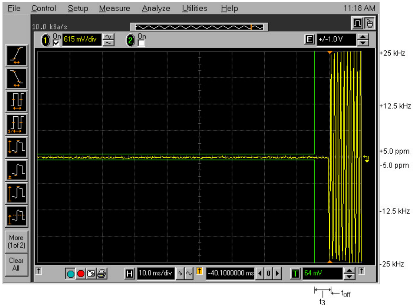
Plot 5.13.4.4. Transient Frequency Behavior Carrier Frequency: 138.1 MHz; Channel Spacing: 25 kHz; Power: 10 W Description: Switch off condition t_3 , t_{off}
