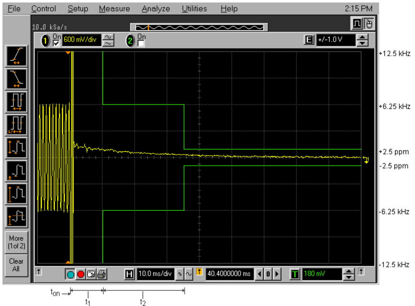
Plot 5.13.4.5. Transient Frequency Behavior Carrier Frequency: 406.3 MHz; Channel Spacing: 12.5 kHz; Power: 10 W Description: Switch on condition t_{on} , t_1 , and t_2
