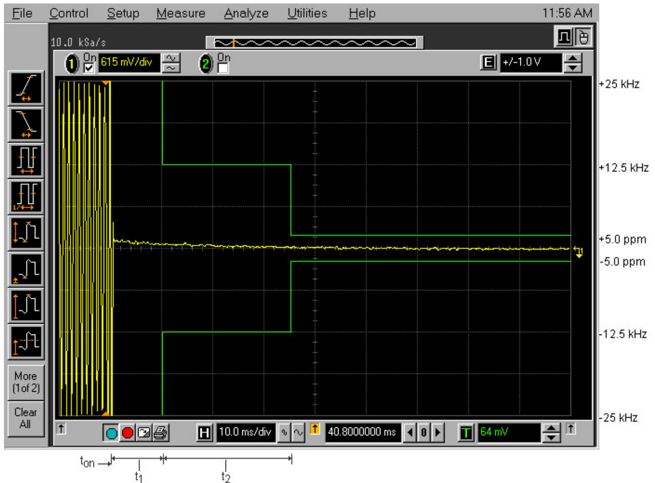
Plot 5.13.4.7. Transient Frequency Behavior Carrier Frequency: 406.3 MHz; Channel Spacing: 25 kHz; Power: 10 W Description: Switch on condition t_{on} , t_1 , and t_2
