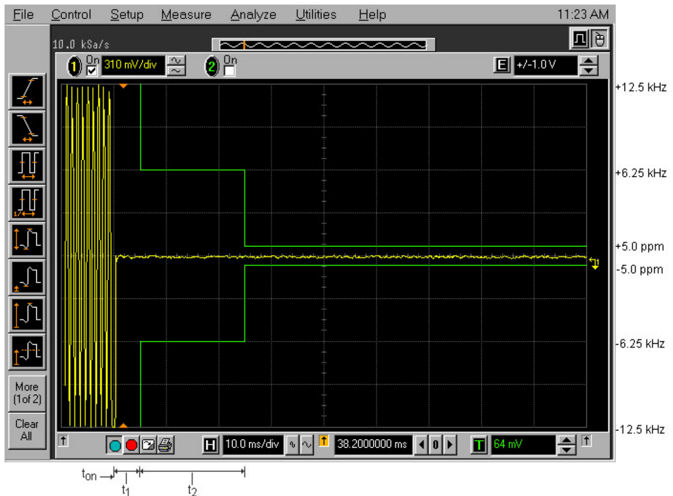
Plot 5.13.4.1. Transient Frequency Behavior Carrier Frequency: 138.1 MHz; Channel Spacing: 12.5 kHz; Power: 10 W Description: Switch on condition t_{on} , t_1 , and t_2
