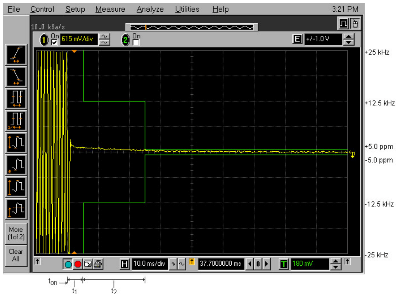
Description: Switch on condition t_{on} , t_1 , and t_2
