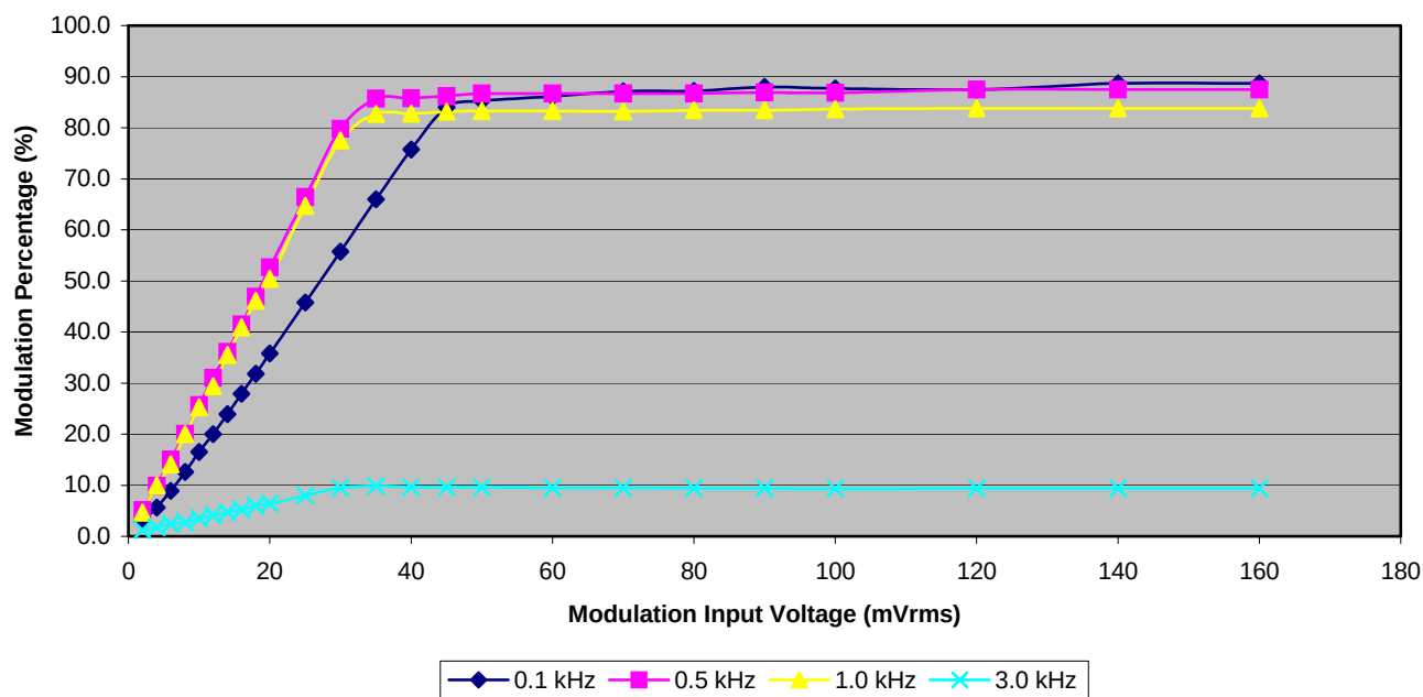
Modulation Limiting Characteristics Test Frequency: 118 MHz, Power Level: 25.0 Watts
