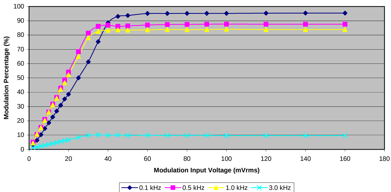
Modulation Limiting Characteristics Test Frequency: 118 MHz, Power Level: 7.0 Watts
