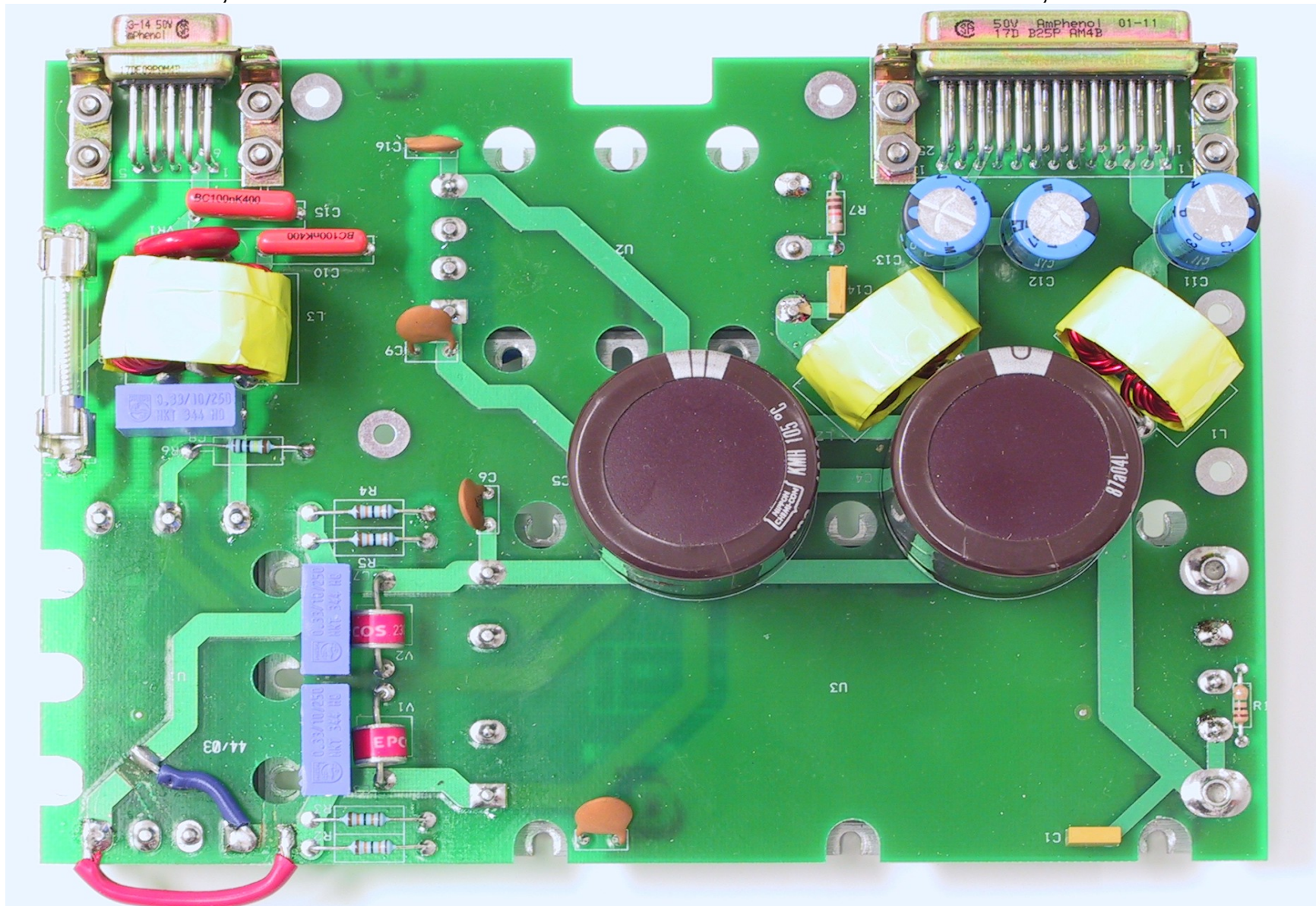
Power Supply
