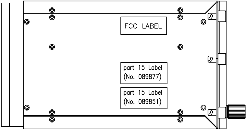
TDFM-7300 LEFT SIDE VIEW
