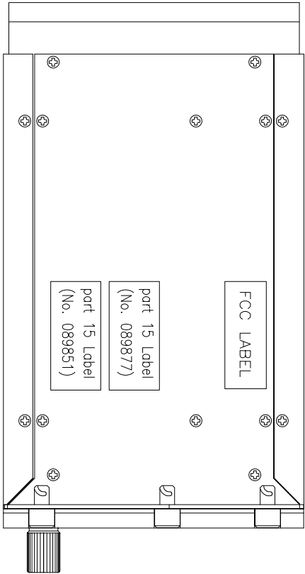
TDFM-7300-3 LEFT SIDE VIEW
