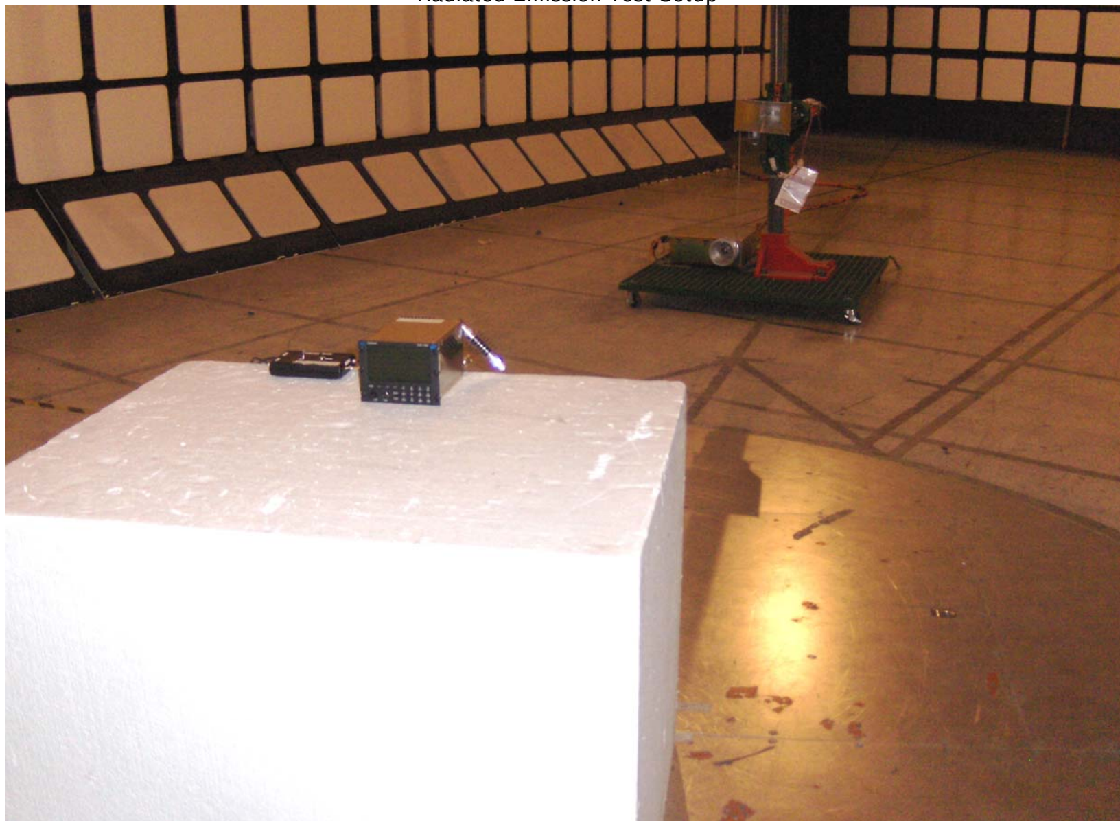
Radiated Emission Test Setup
