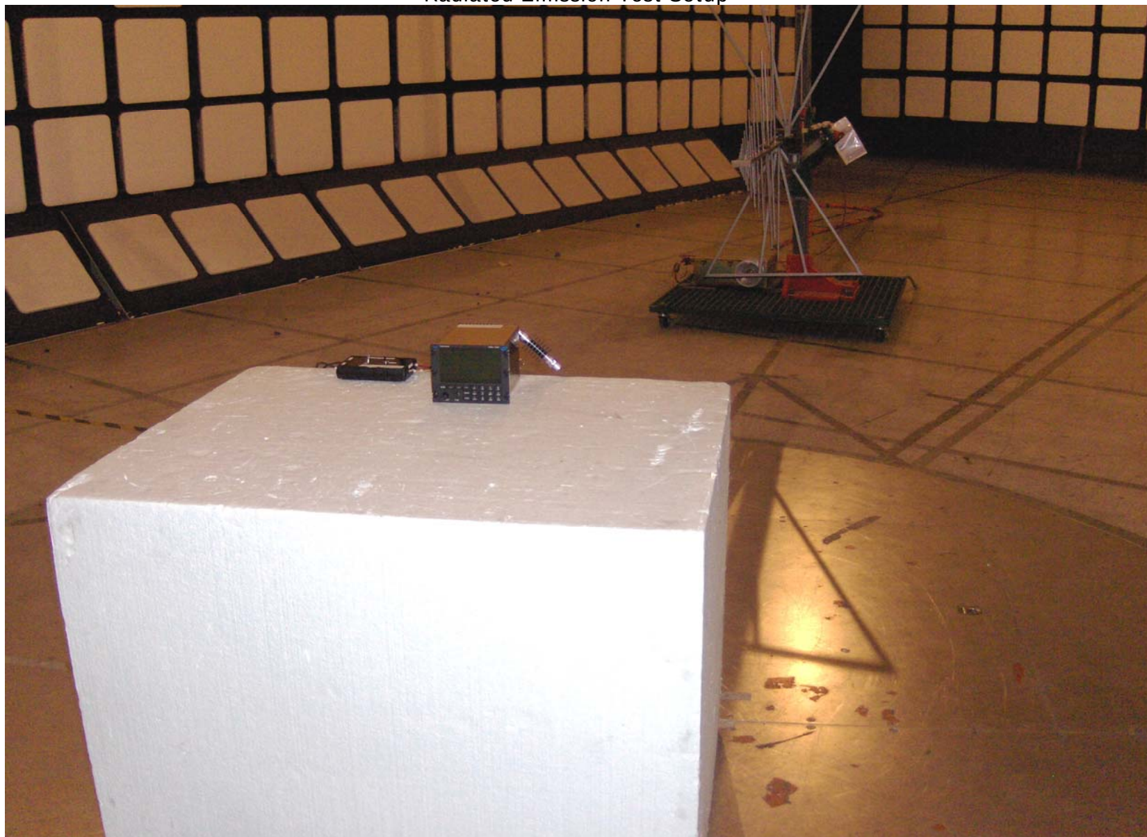
Radiated Emission Test Setup
