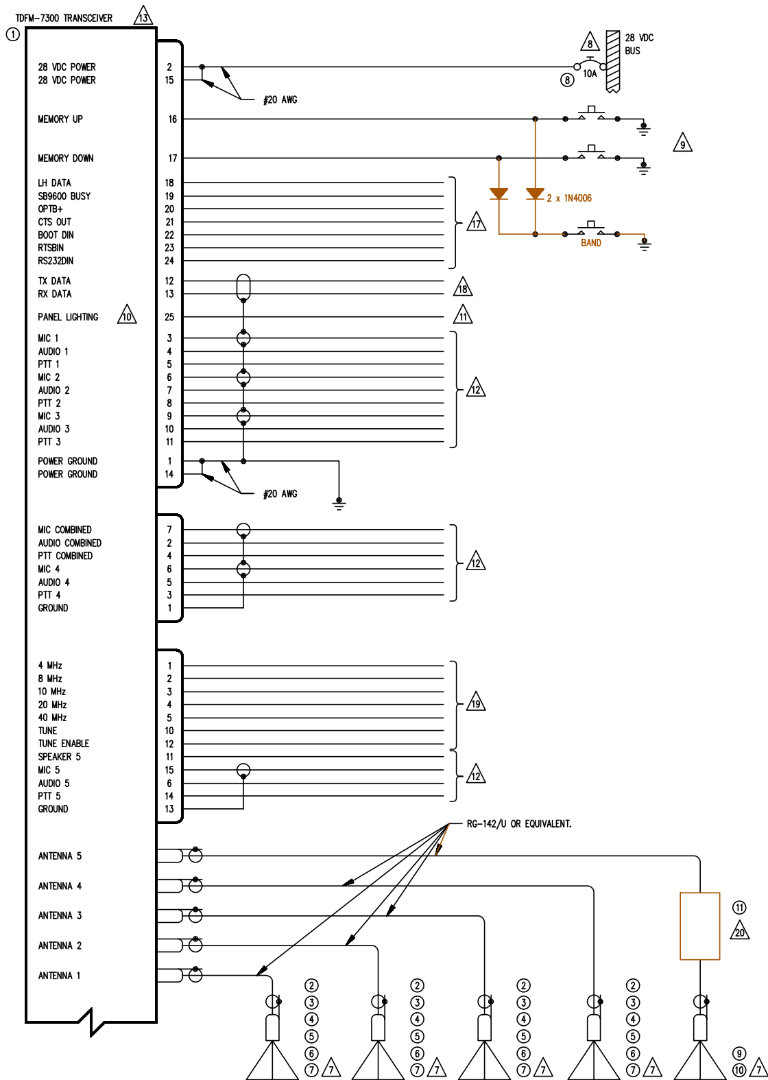
FIGURE 3-2a Wiring connections for the TDFM-7300-2 Transceiver
