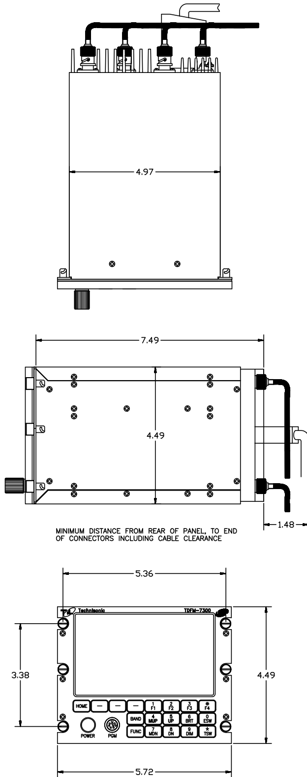
FIGURE 3-1 Outline Drawing for Model TDFM-7300-2
