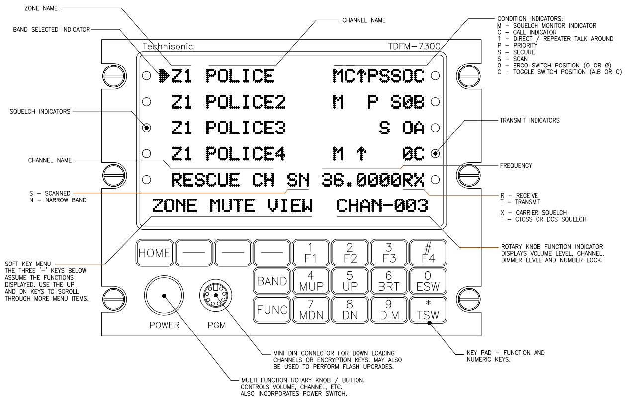
FIGURE 2-1 Front Panel Controls – TDFM-7300-2 Transceiver
