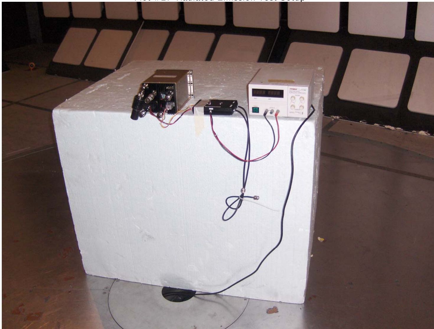
Plot #2: Radiated Emission Test Setup
