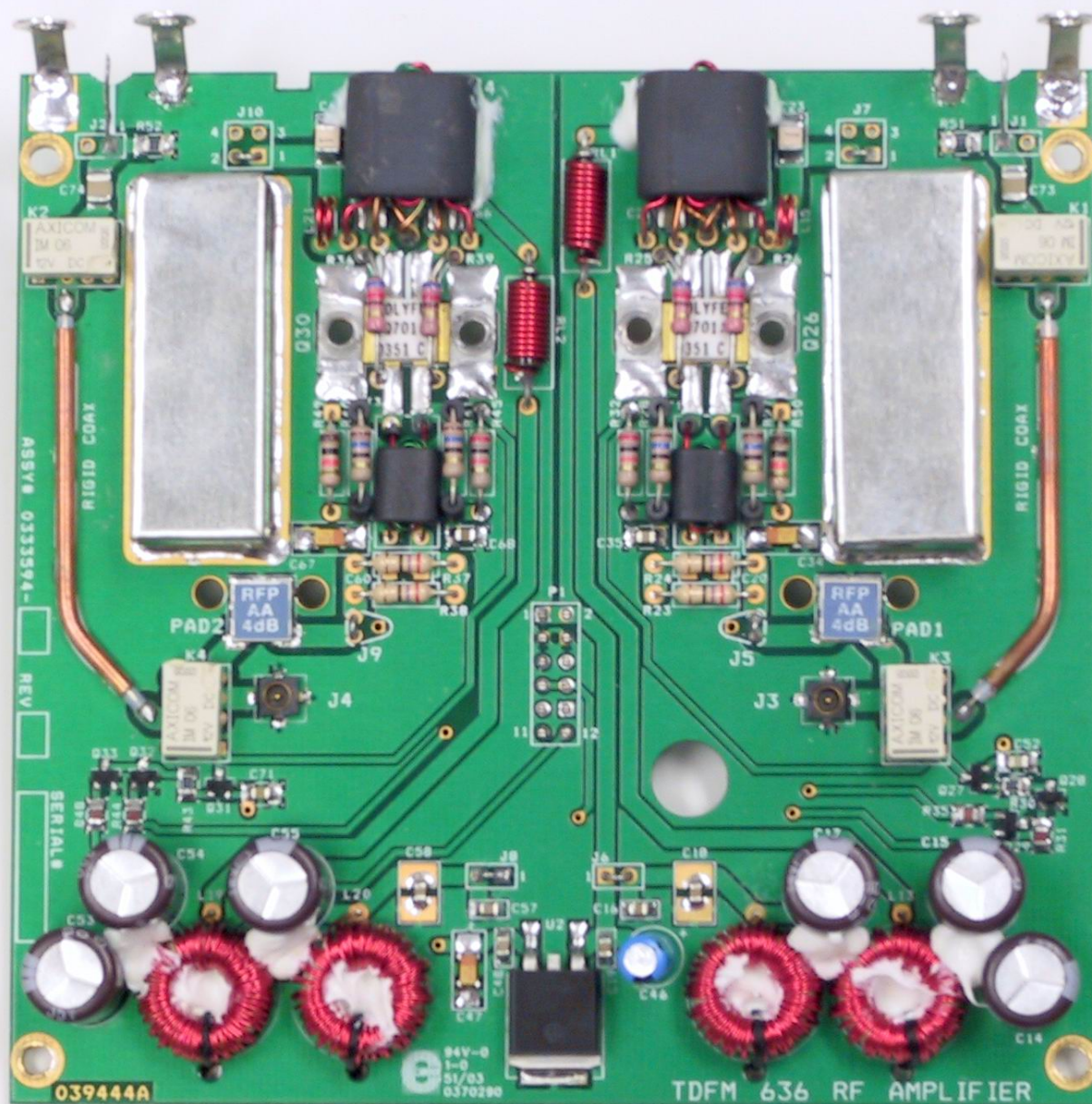
Annex 3 – Internal Photographs of EUT VHF P25 Airborne Transceiver, Model No.: TDFM-636
