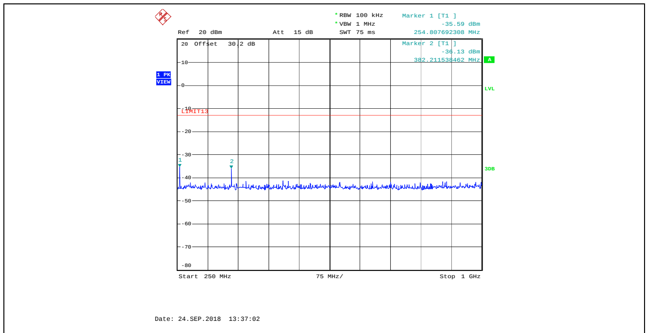
Plot 5.5.4.5. Transmitter Spurious Emissions at Antenna Terminal, 25 kHz Channel Spacing, High Power (10 W) 127.500 MHz, 250 MHz – 1 GHz
