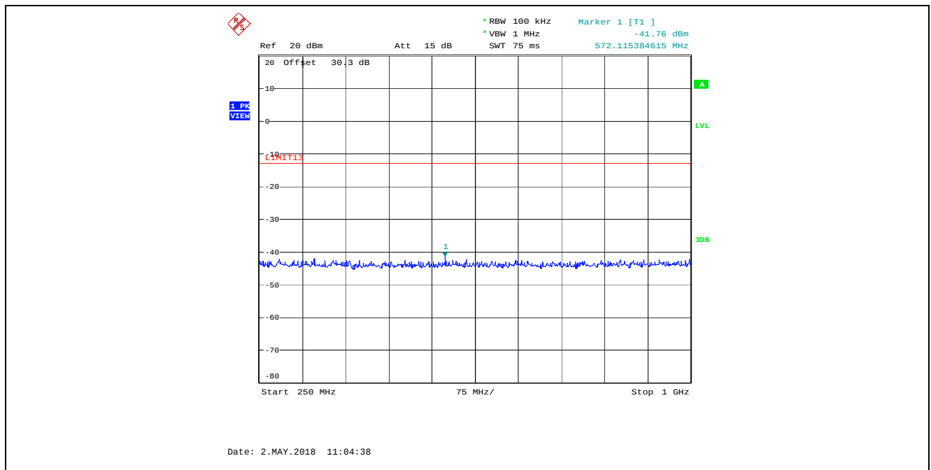
Plot 5.5.4.14. Transmitter Spurious Emissions at Antenna Terminal, 25 kHz Channel Spacing, Low Power (1 W) 127.500 MHz, 250 MHz – 1 GHz
