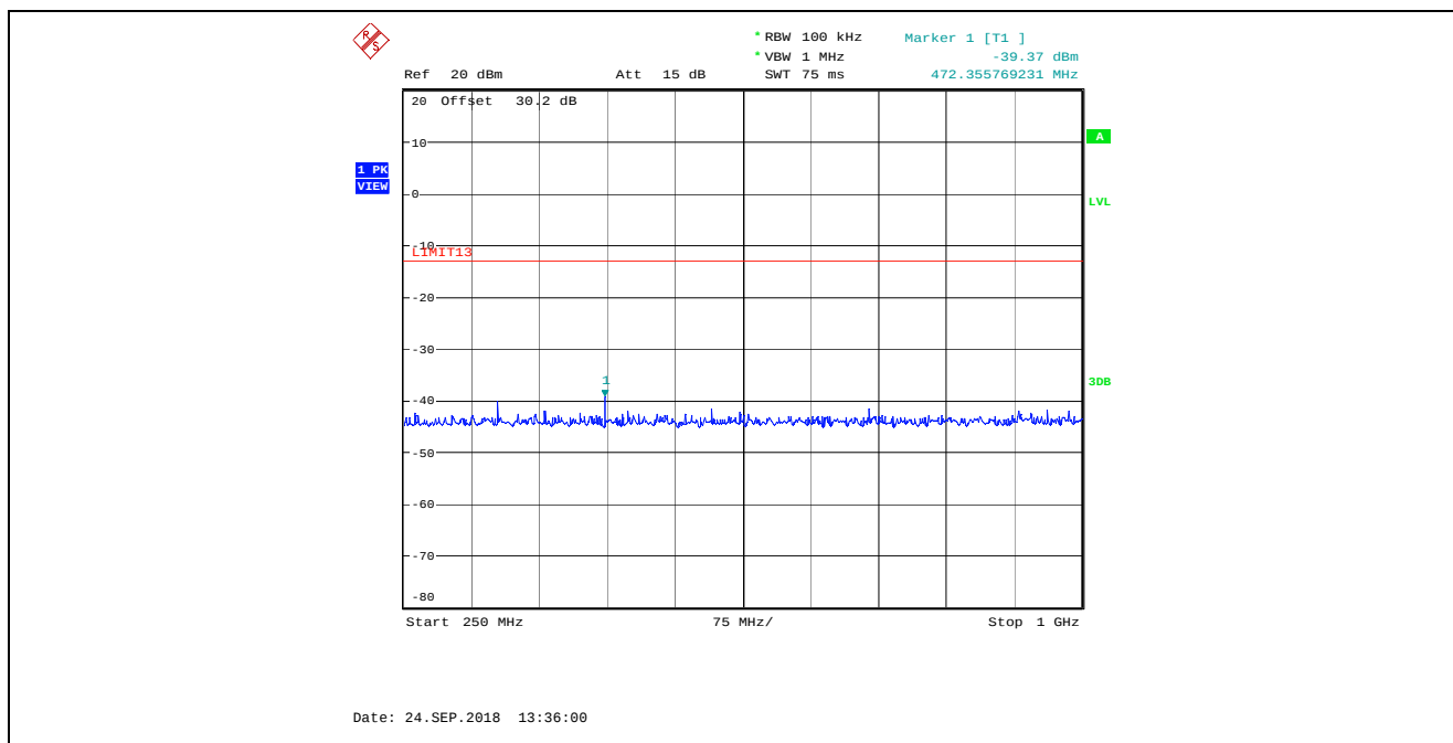
Plot 5.5.4.2. Transmitter Spurious Emissions at Antenna Terminal, 25 kHz Channel Spacing, High Power (10 W) 118.000 MHz, 250 MHz – 1 GHz
