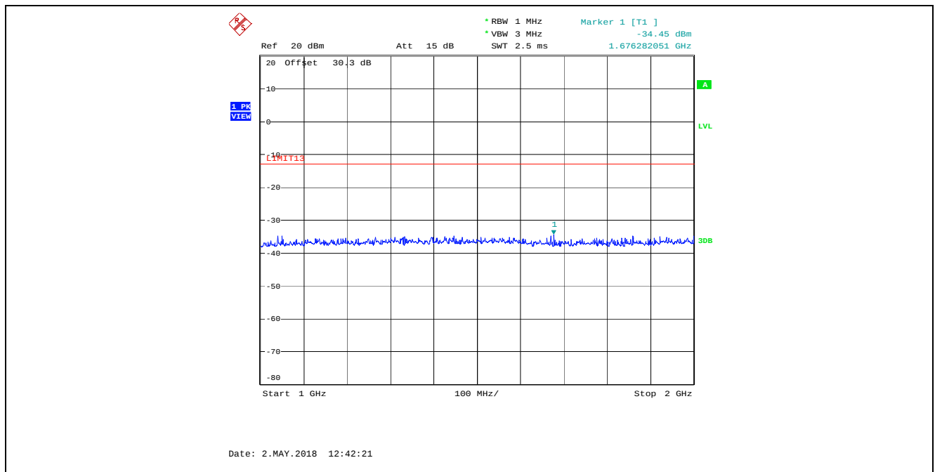
Plot 5.5.4.18. Transmitter Spurious Emissions at Antenna Terminal, 25 kHz Channel Spacing, Low Power (1 W) 136.975 MHz, 1 GHz - 2 GHz
