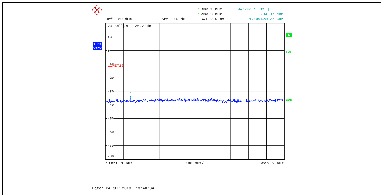
Plot 5.5.4.6. Transmitter Spurious Emissions at Antenna Terminal, 25 kHz Channel Spacing, High Power (10 W) 127.500 MHz, 1 GHz - 2 GHz
