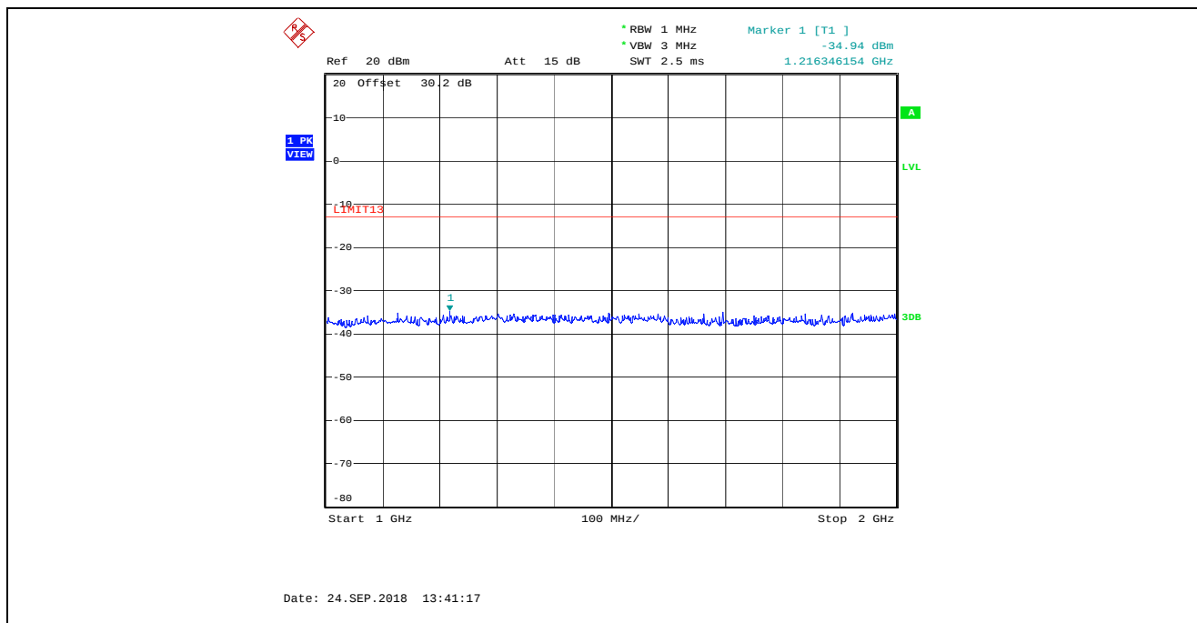
Plot 5.5.4.9. Transmitter Spurious Emissions at Antenna Terminal, 25 kHz Channel Spacing, High Power (10 W) 136.975 MHz, 1 GHz - 2 GHz
