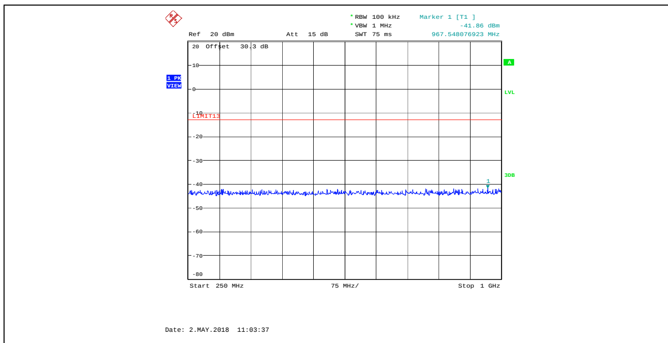
Plot 5.5.4.11. Transmitter Spurious Emissions at Antenna Terminal, 25 kHz Channel Spacing, Low Power (1 W) 118.000 MHz, 250 MHz – 1 GHz
