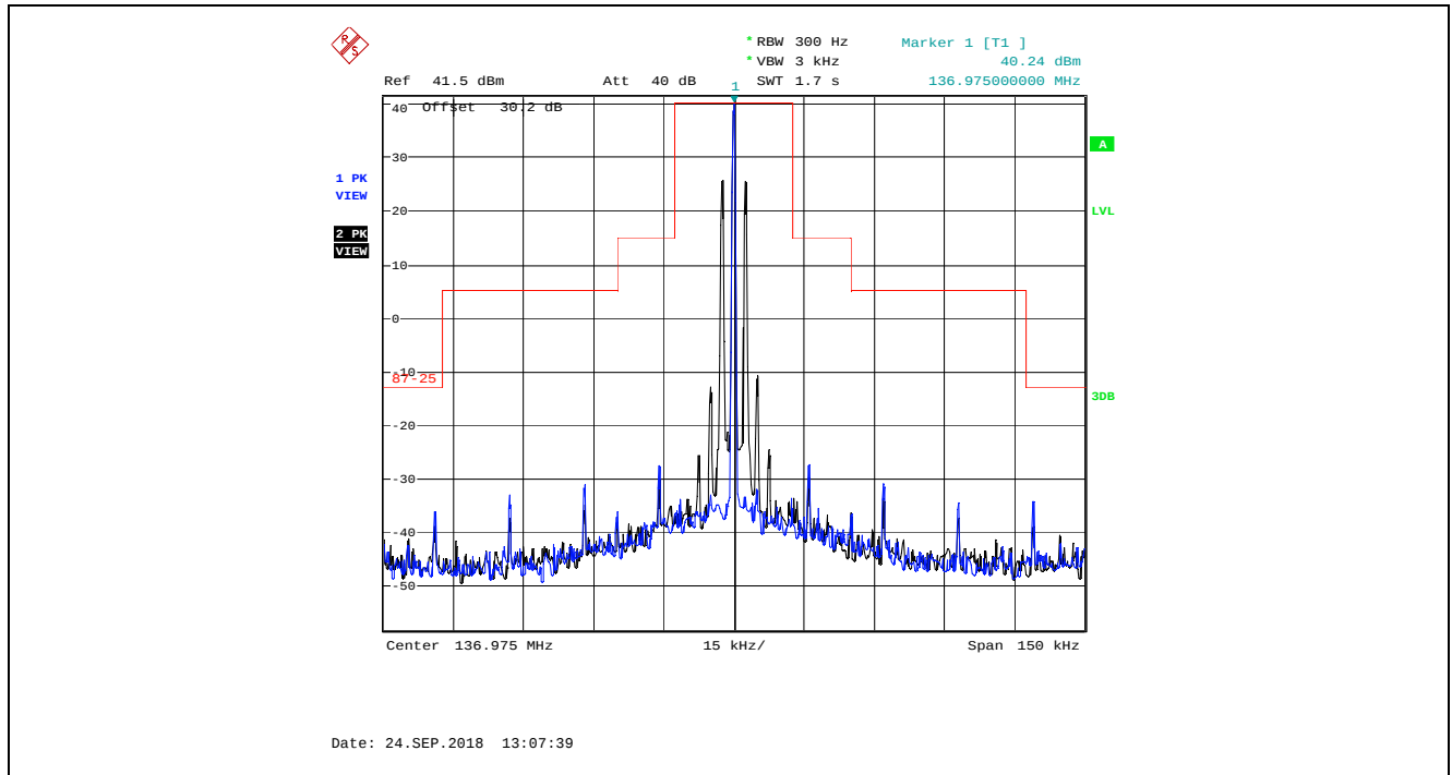
Plot 5.4.4.2.11. Emissions Limitation, 25 kHz Channel Spacing, 136.975 MHz, High Power (10 W)
