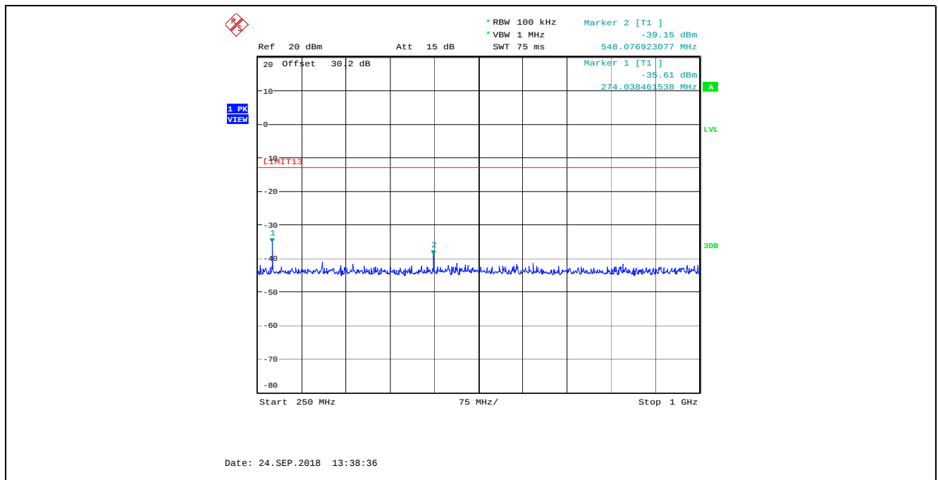
Plot 5.5.4.8. Transmitter Spurious Emissions at Antenna Terminal, 25 kHz Channel Spacing, High Power (10 W) 136.975 MHz, 250 MHz – 1 GHz
