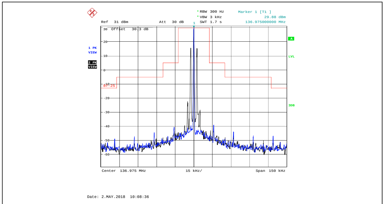
Plot 5.4.4.2.12. Emissions Limitation, 25 kHz Channel Spacing, 136.975MHz, Low Power (1 W)
