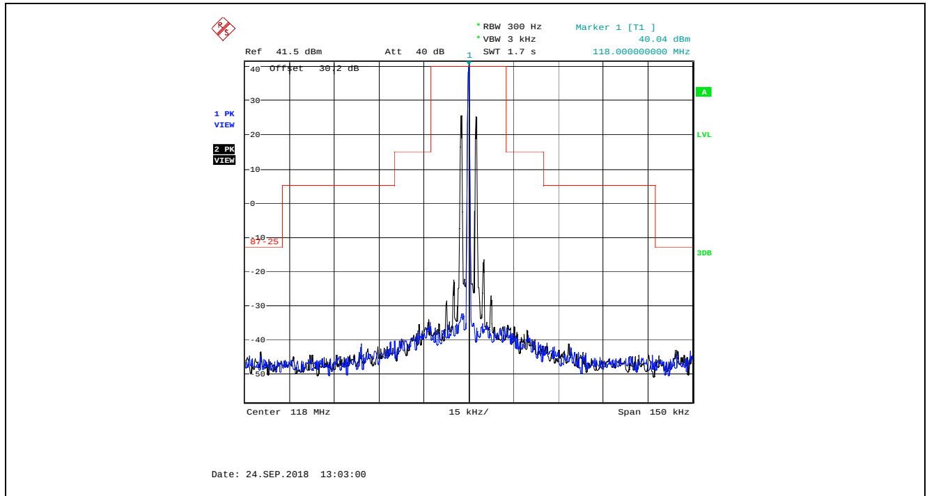
Plot 5.4.4.2.7. Emissions Limitation, 25 kHz Channel Spacing, 118.000 MHz, High Power (10 W)
