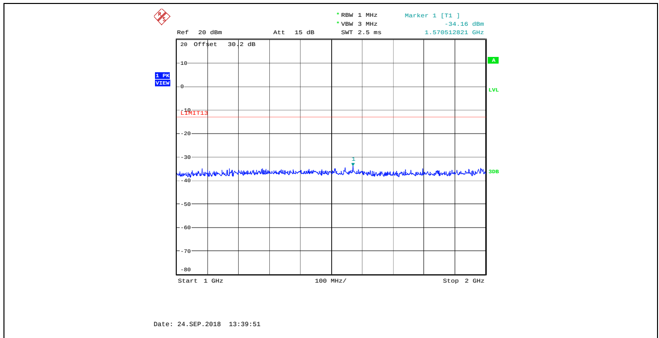
Plot 5.5.4.3. Transmitter Spurious Emissions at Antenna Terminal, 25 kHz Channel Spacing, High Power (10 W) 118.000 MHz, 1 GHz - 2 GHz
