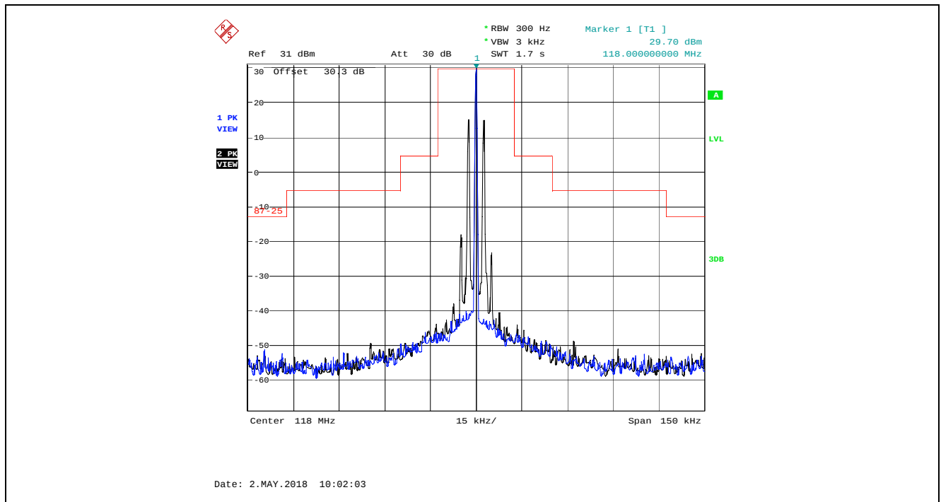
Plot 5.4.4.2.8. Emissions Limitation, 25 kHz Channel Spacing, 118.000 MHz, Low Power (1 W)
