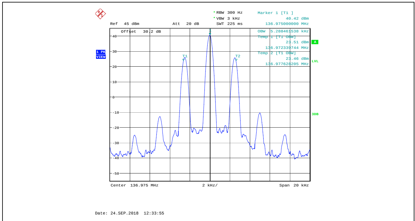
Plot 5.4.4.1.6. 99% Occupied Bandwidth, 25 kHz Channel Spacing, 136.975 MHz
