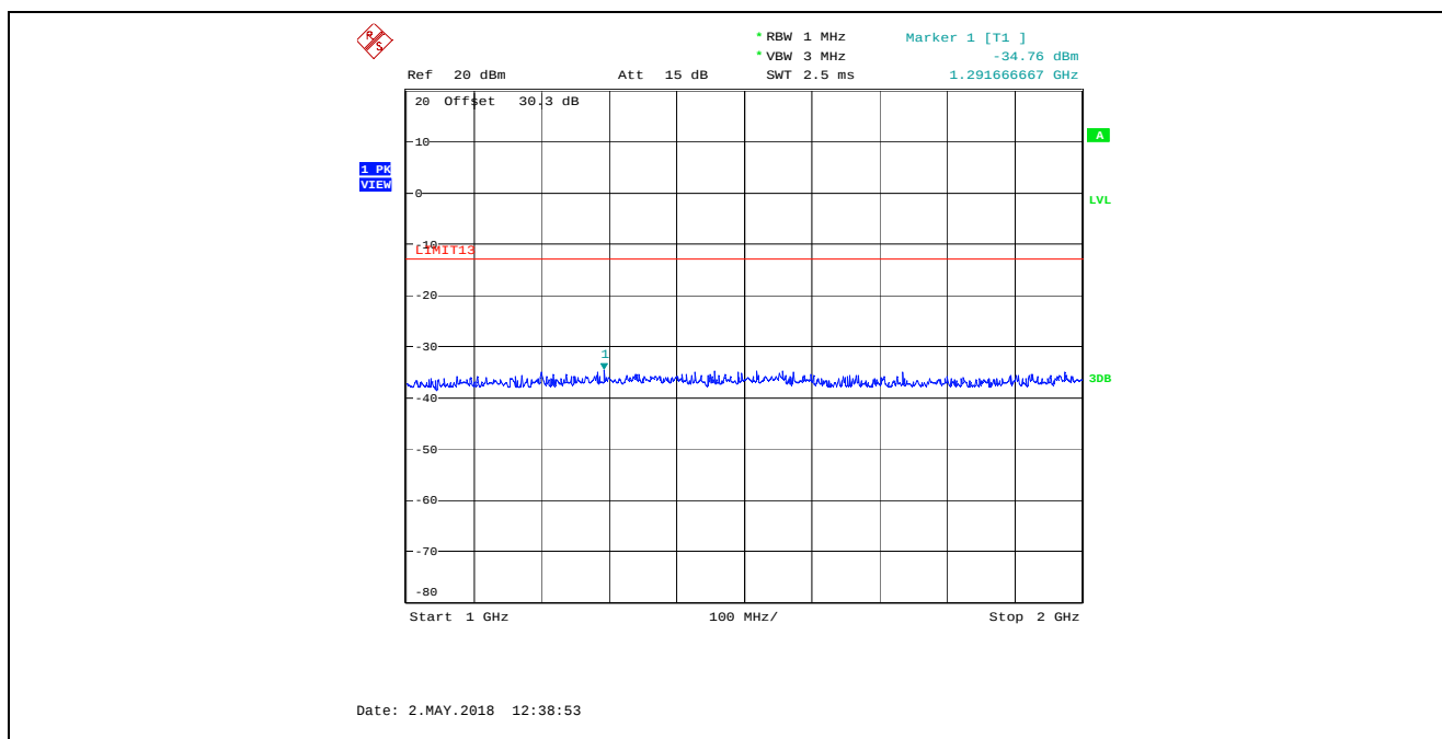
Plot 5.5.4.12. Transmitter Spurious Emissions at Antenna Terminal, 25 kHz Channel Spacing, Low Power (1 W) 118.000 MHz, 1 GHz - 2 GHz
