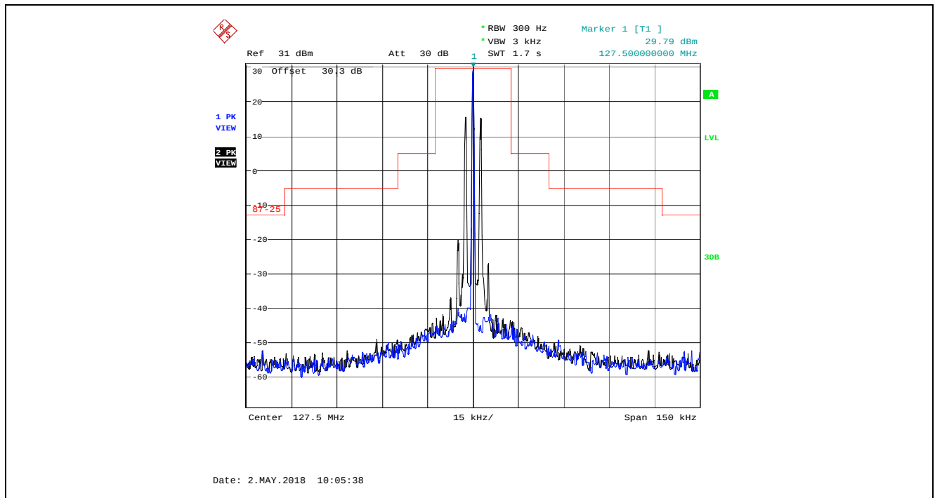
Plot 5.4.4.2.10. Emissions Limitation, 25 kHz Channel Spacing, 127.500 MHz, Low Power (1 W)
