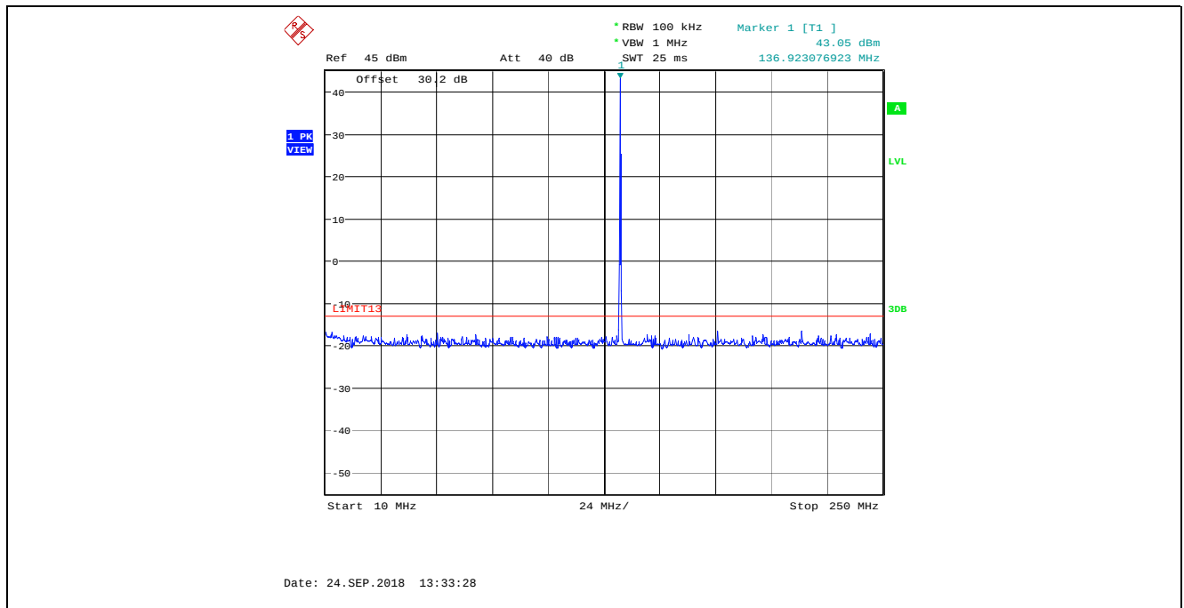
Plot 5.5.4.7. Transmitter Spurious Emissions at Antenna Terminal, 25 kHz Channel Spacing, High Power (10 W) 136.975 MHz, 10 MHz – 250 MHz
