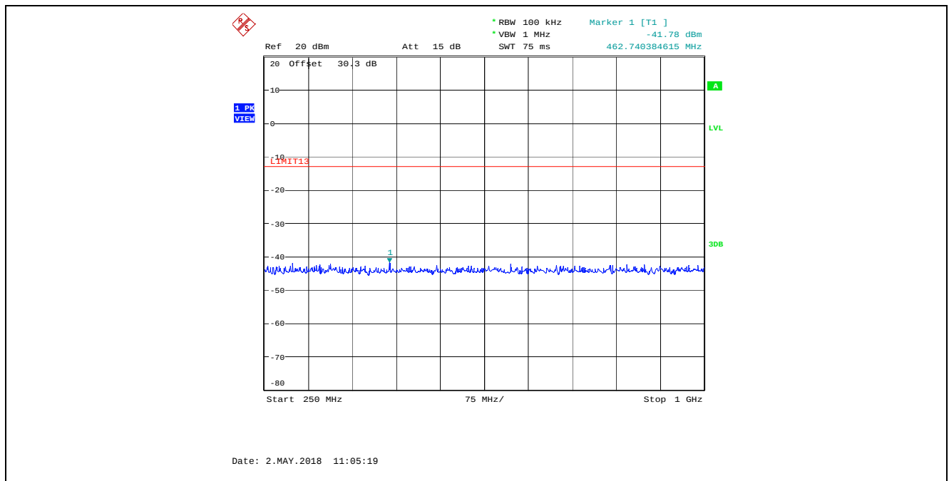
Plot 5.5.4.17. Transmitter Spurious Emissions at Antenna Terminal, 25 kHz Channel Spacing, Low Power (1 W) 136.975 MHz, 250 MHz – 1 GHz
