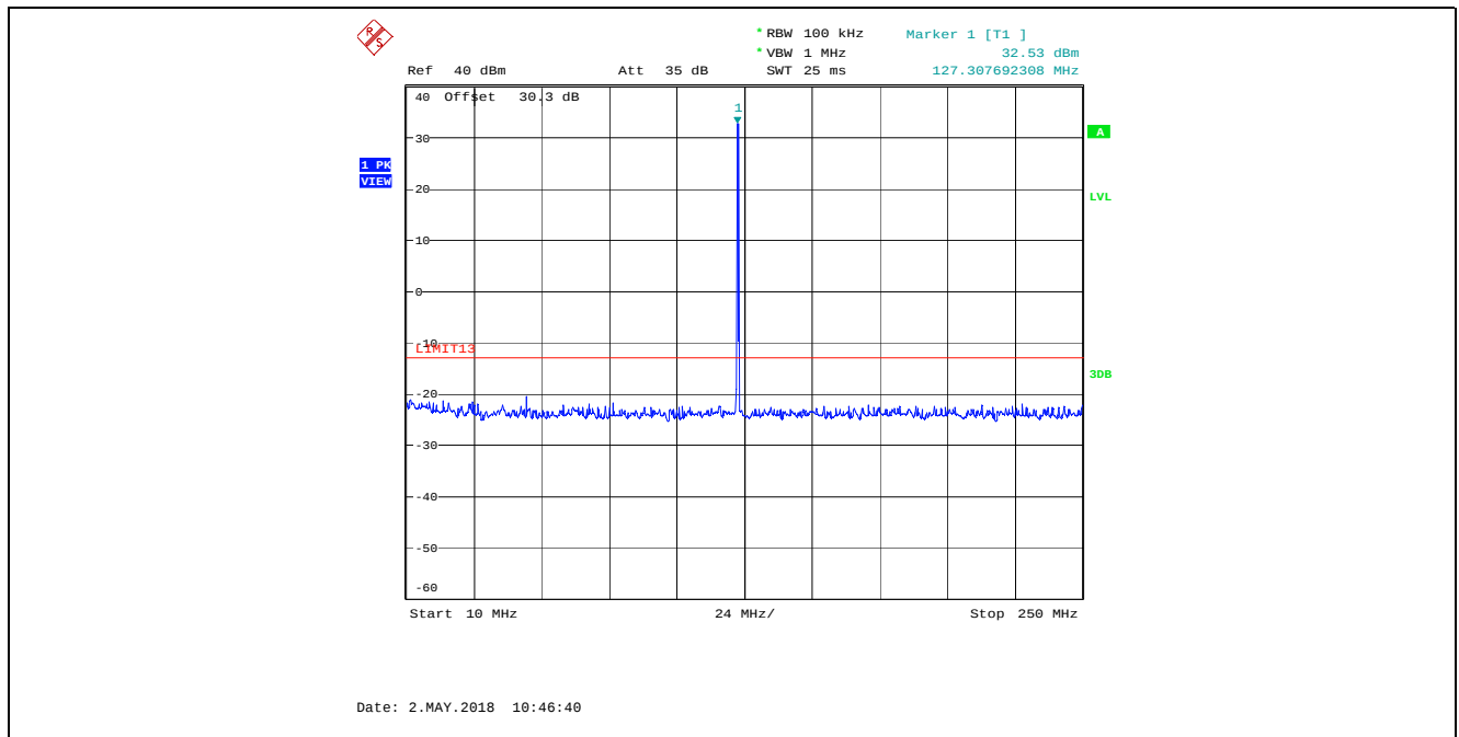
Plot 5.5.4.13. Transmitter Spurious Emissions at Antenna Terminal, 25 kHz Channel Spacing, Low Power (1 W) 127.500 MHz, 10 MHz – 250 MHz
