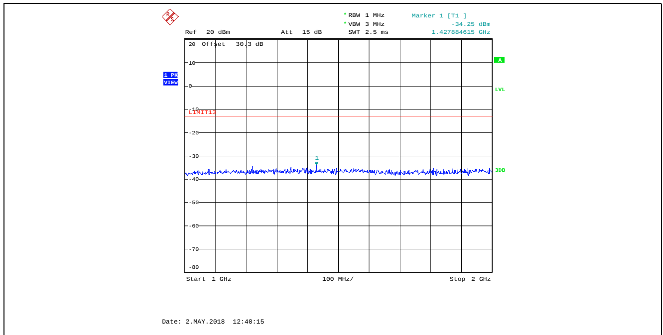
Plot 5.5.4.15. Transmitter Spurious Emissions at Antenna Terminal, 25 kHz Channel Spacing, Low Power (1 W) 127.500 MHz, 1 GHz - 2 GHz
