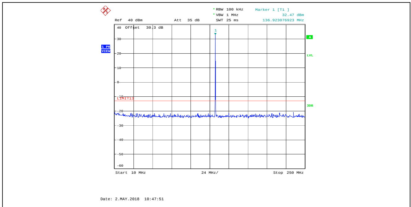
Plot 5.5.4.16. Transmitter Spurious Emissions at Antenna Terminal, 25 kHz Channel Spacing, Low Power (1 W) 136.975 MHz, 10 MHz – 250 MHz
