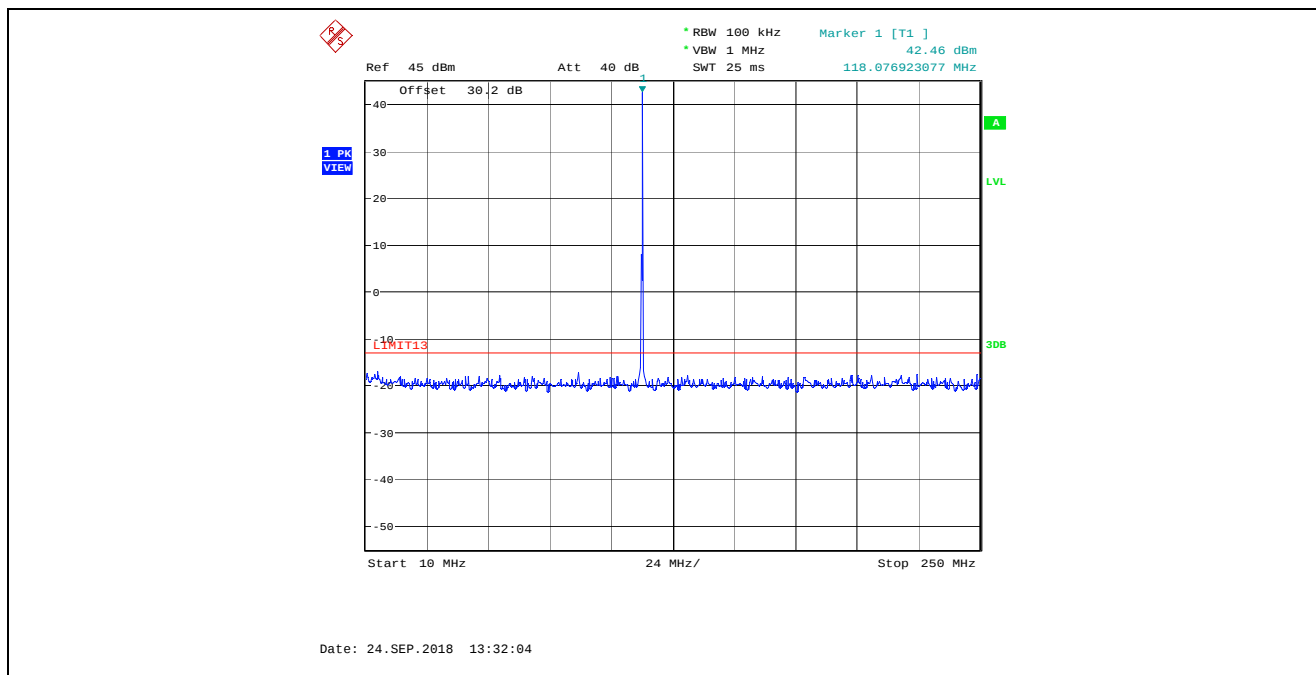
Plot 5.5.4.1. Transmitter Spurious Emissions at Antenna Terminal, 25 kHz Channel Spacing, High Power (10 W) 118.000 MHz, 10 MHz – 250 MHz
