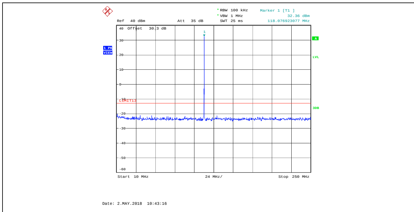
Plot 5.5.4.10. Transmitter Spurious Emissions at Antenna Terminal, 25 kHz Channel Spacing, Low Power (1 W) 118.000 MHz, 10 MHz – 250 MHz
