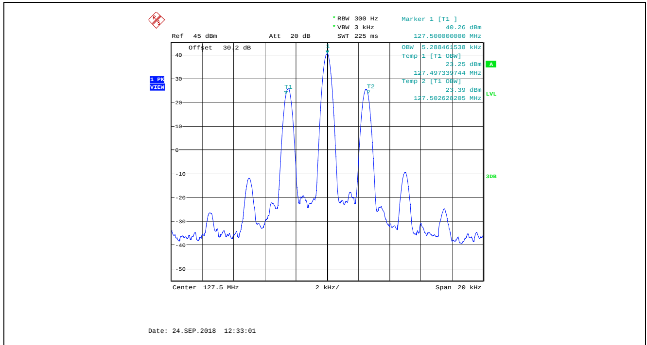
Plot 5.4.4.1.5. 99% Occupied Bandwidth, 25 kHz Channel Spacing, 127.500 MHz
