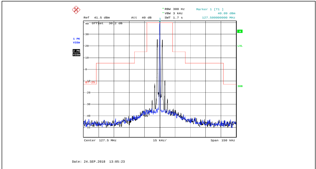
Plot 5.4.4.2.9. Emissions Limitation, 25 kHz Channel Spacing, 127.500 MHz, High Power (10 W)
