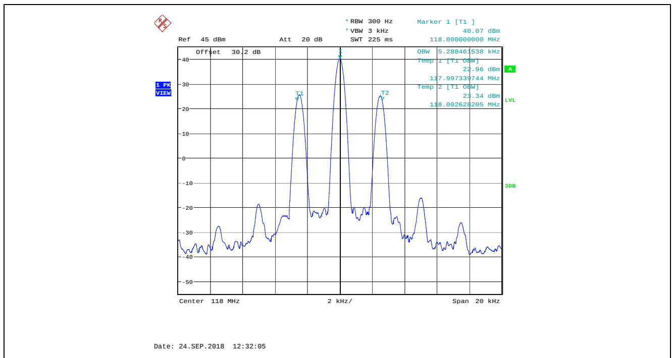
Plot 5.4.4.1.4. 99% Occupied Bandwidth, 25 kHz Channel Spacing, 118.000 MHz
