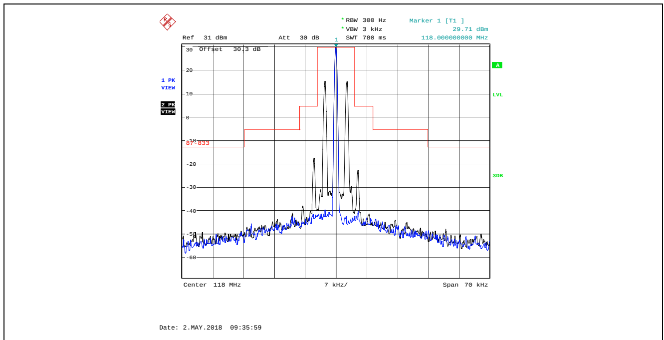
Plot 5.4.4.2.2. Emissions Limitation, 8.33 kHz Channel Spacing, 118.005 MHz, Low Power (1 W)
