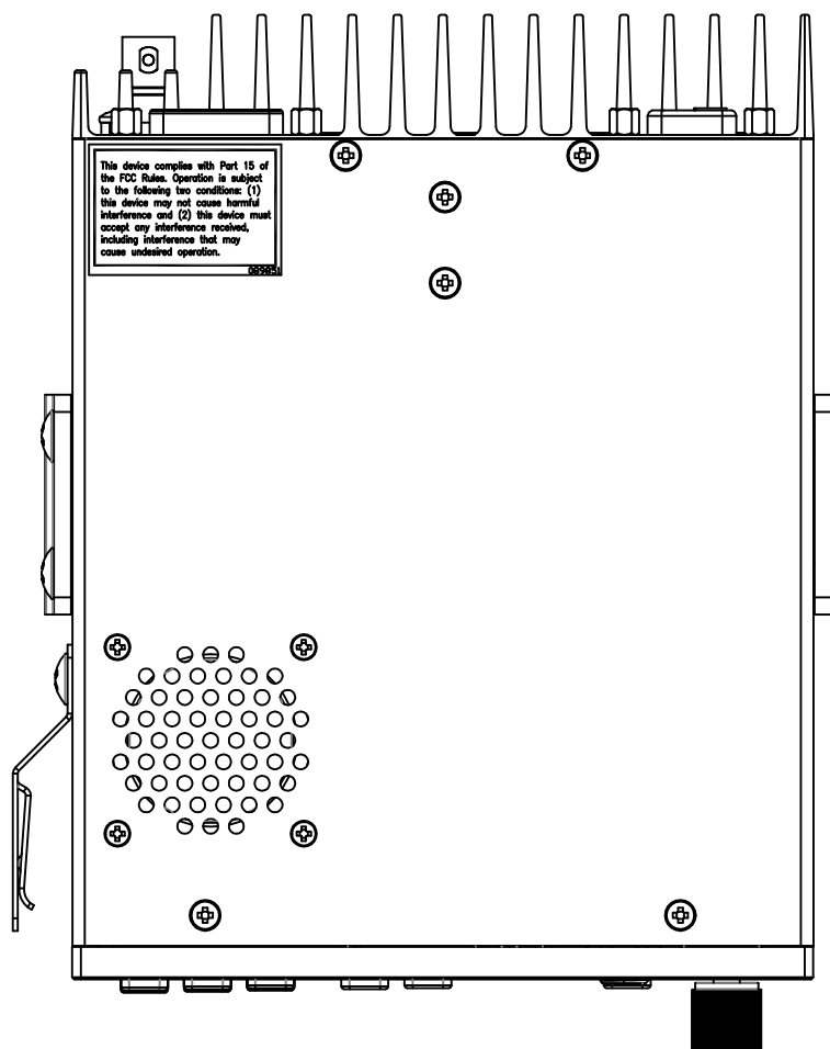
Figure 3. TDAM-1000 FCC Part 15 label placement bottom chassis.
