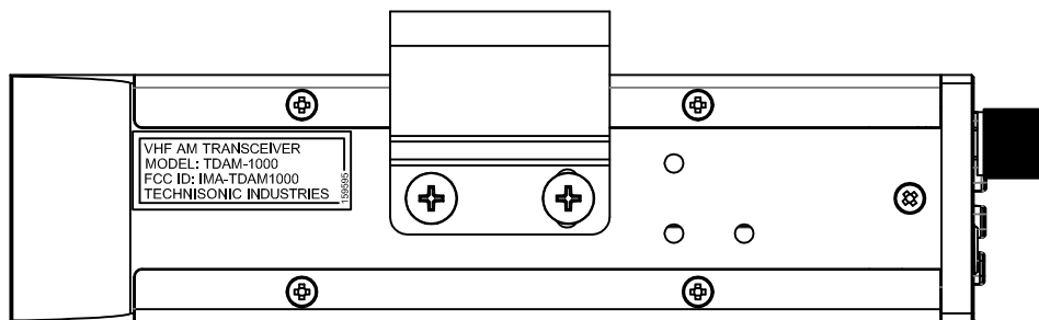
Figure 1. TDAM-1000 FCC label placement left side chassis.
