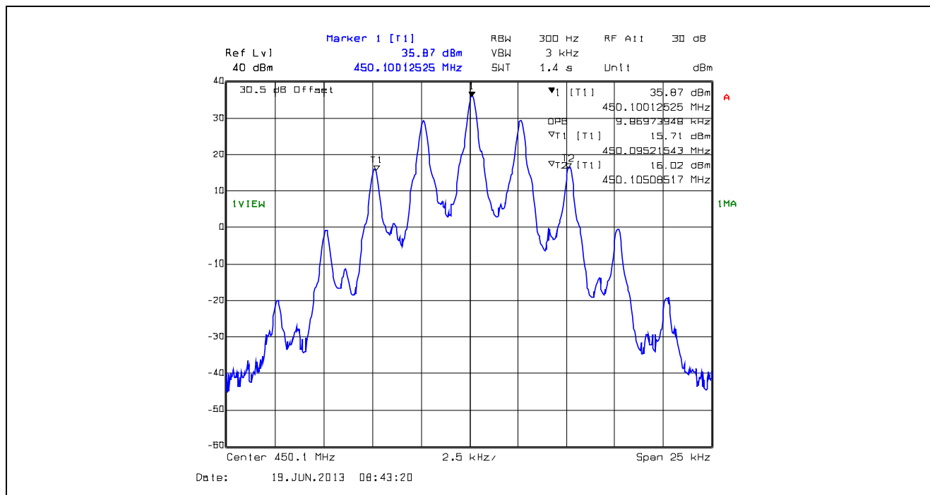
Plot 5.4.4.1.1. 99% Occupied Bandwidth, 12.5 kHz Channel Spacing, F3E, 450.1 MHz
