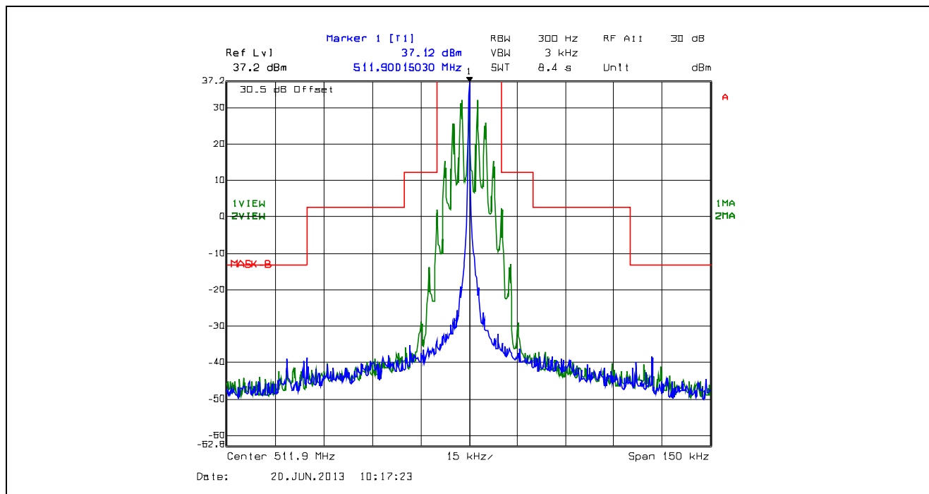
Plot 5.4.4.2.11. Emission Mask B, 25 kHz Channel Spacing, F3E, High Power, 511.9 MHz
