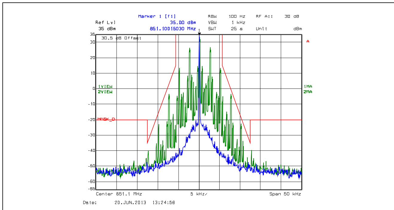
Plot 5.4.4.2.61. Emission Mask D, 12.5 kHz Channel Spacing, F3E, High Power, 851.1 MHz
