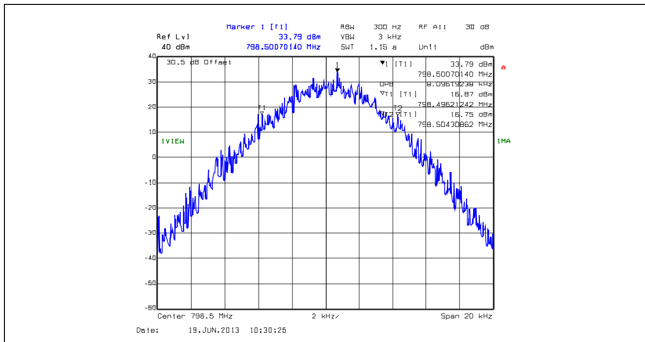
Plot 5.4.4.1.38. 99% Occupied Bandwidth, 12.5 kHz Channel Spacing, F1E, 798.5 MHz
