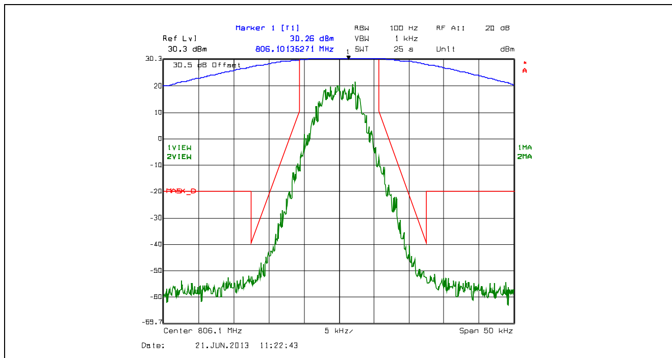
Plot 5.4.4.2.56. Emission Mask D, 12.5 kHz Channel Spacing, F1W, Low Power, 806.1 MHz
