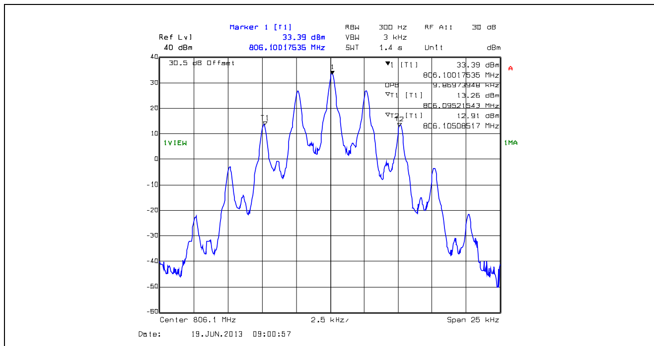
Plot 5.4.4.1.46. 99% Occupied Bandwidth, 12.5 kHz Channel Spacing, F3E, 806.1 MHz
