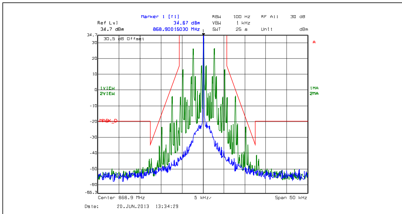
Plot 5.4.4.2.65. Emission Mask D, 12.5 kHz Channel Spacing, F3E, High Power, 868.9 MHz
