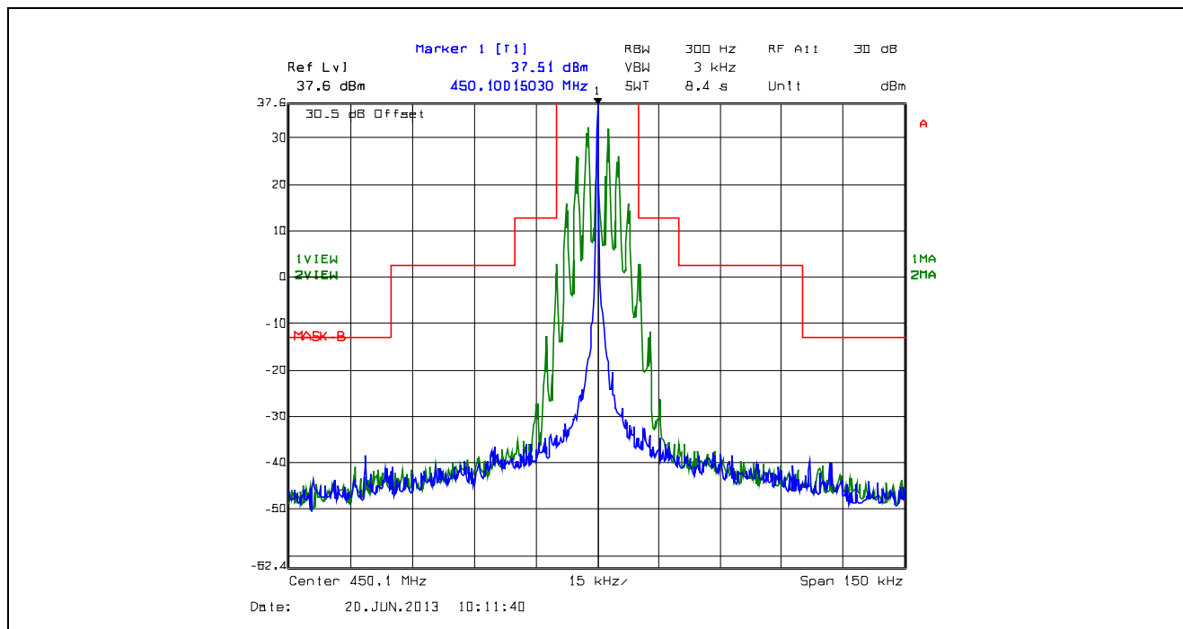
Plot 5.4.4.2.7. Emission Mask B, 25 kHz Channel Spacing, F3E, High Power, 450.1 MHz
