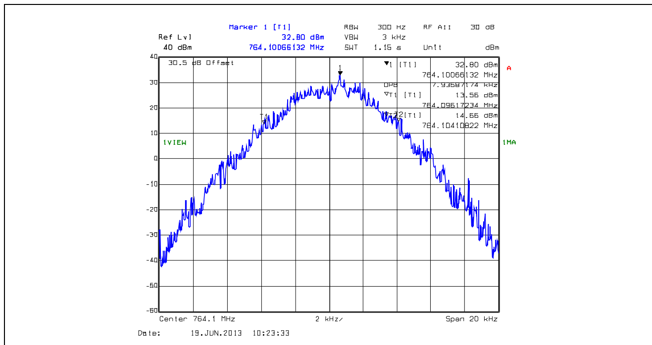
Plot 5.4.4.1.22. 99% Occupied Bandwidth, 12.5 kHz Channel Spacing, F1E, 764.1 MHz
