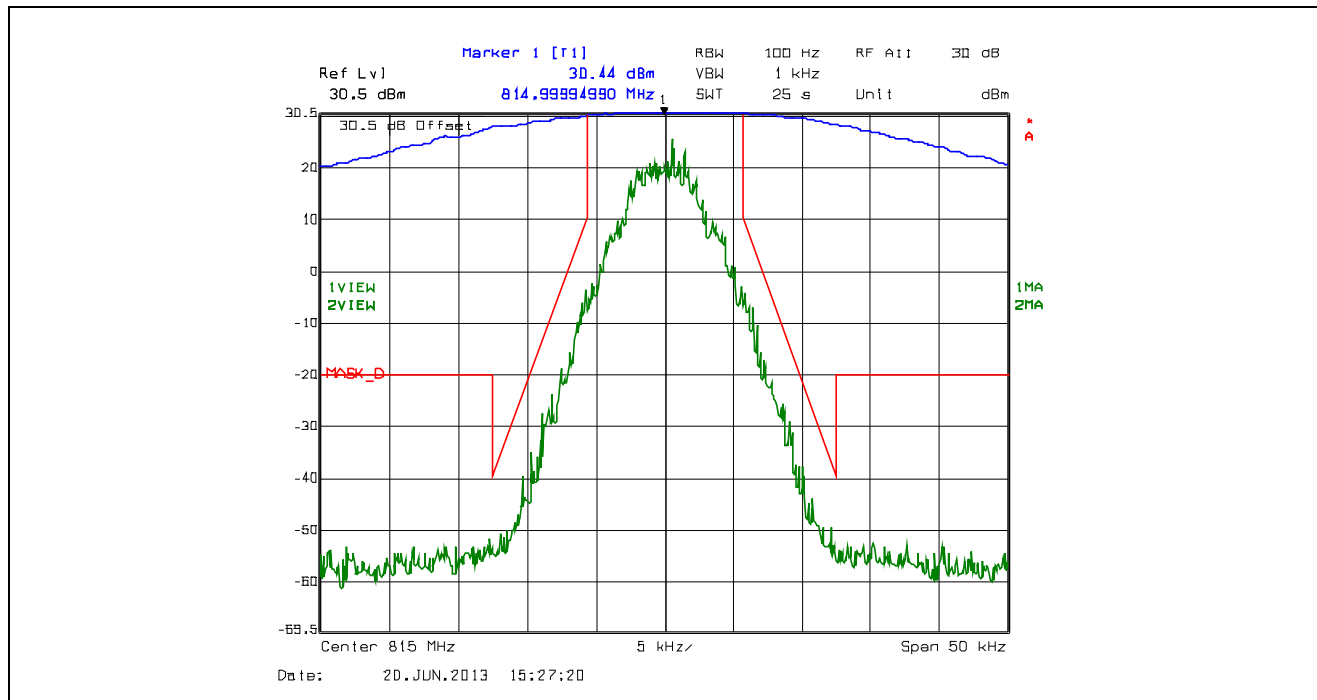
Plot 5.4.4.2.46. Emission Mask D, 12.5 kHz Channel Spacing, F1E, Low Power, 815.0 MHz
