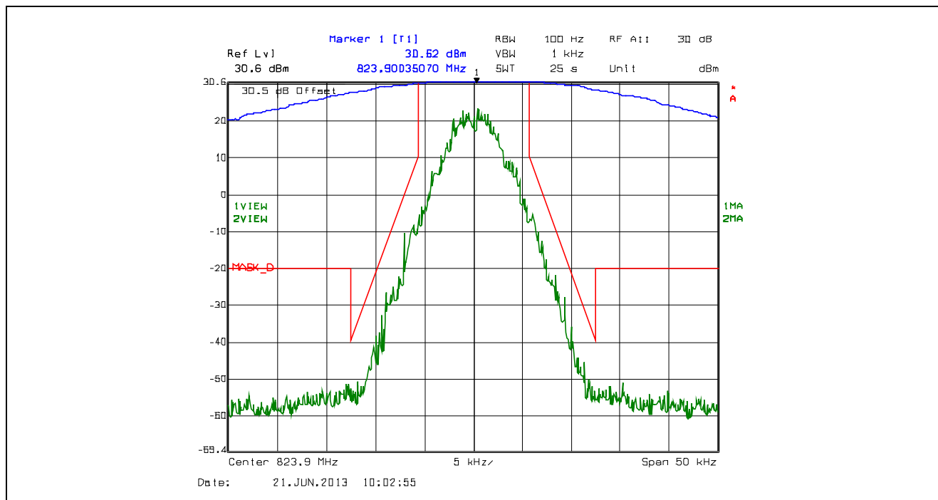
Plot 5.4.4.2.54. Emission Mask D, 12.5 kHz Channel Spacing, F1D, Low Power, 823.9 MHz
