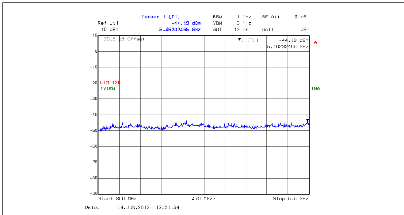
Plot 5.5.4.4. Conducted Transmitter Spurious Emissions, Low Power, 450.1 MHz, 800 MHz – 5.5 GHz
