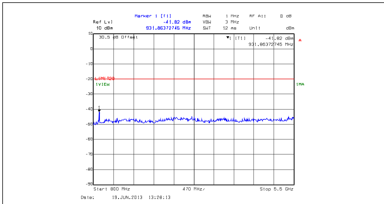
Plot 5.5.4.6. Conducted Transmitter Spurious Emissions, High Power, 469.9 MHz, 800 MHz – 5.5 GHz
