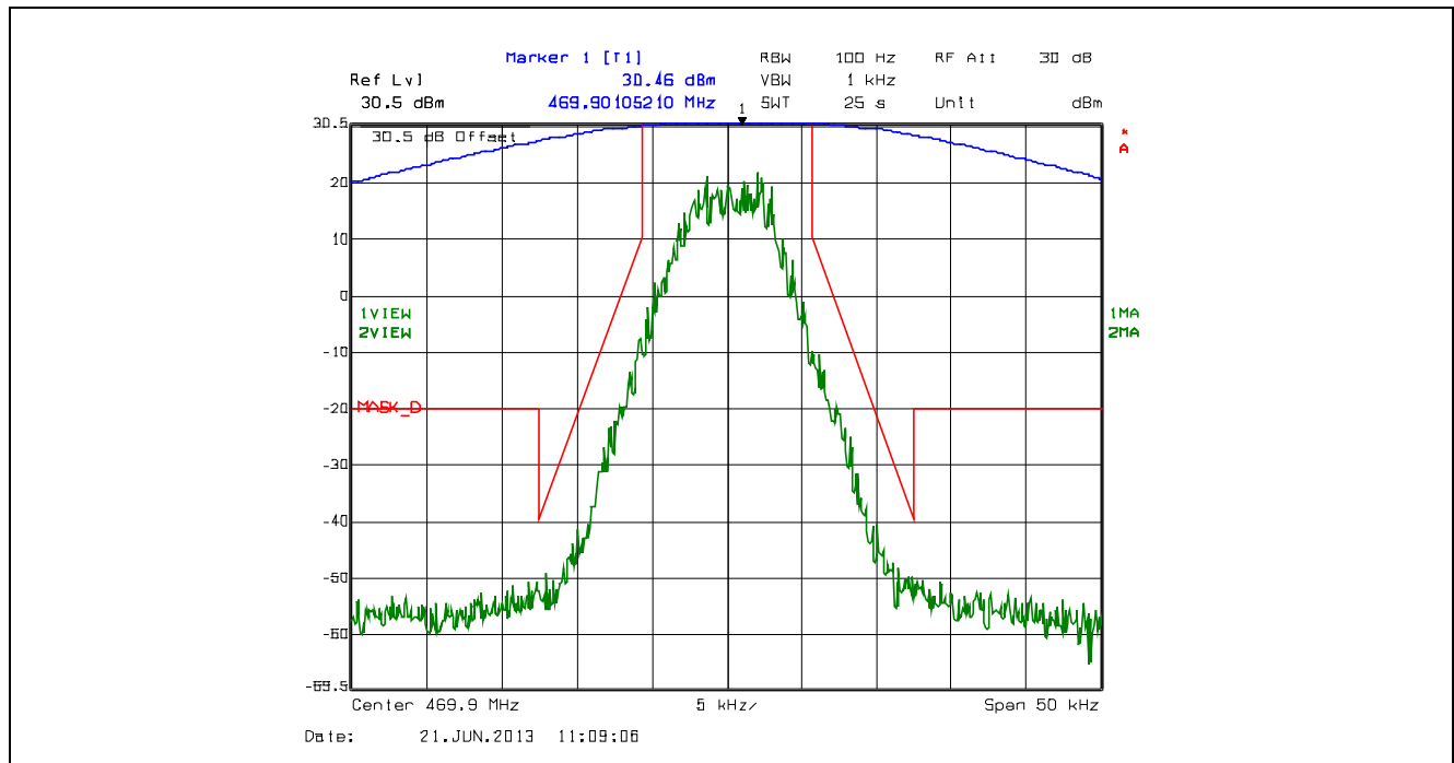
Plot 5.4.4.2.28. Emission Mask D, 12.5 kHz Channel Spacing, F1W, Low Power, 469.9 MHz
