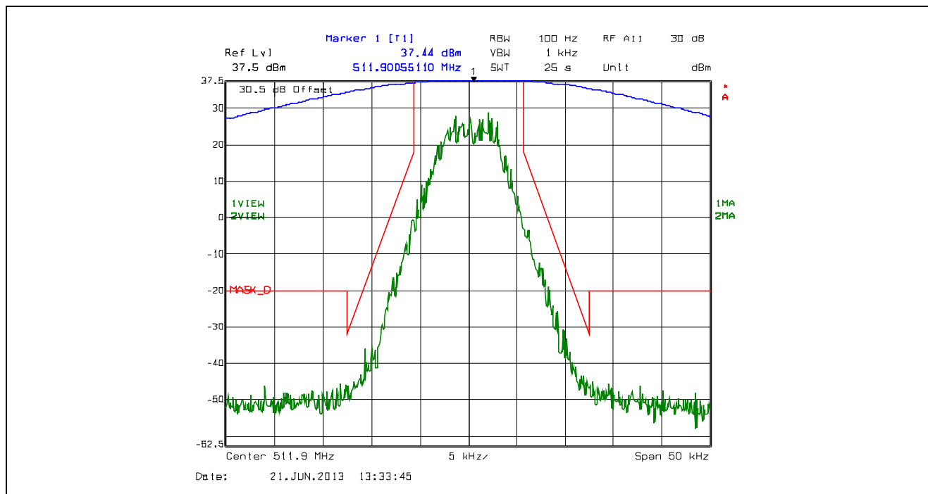
Plot 5.4.4.2.29. Emission Mask D, 12.5 kHz Channel Spacing, F1W, High Power, 511.9 MHz
