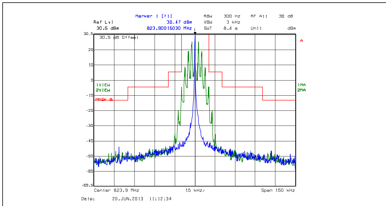
Plot 5.4.4.2.42. Emission Mask B, 25 kHz Channel Spacing, F3E, Low Power, 823.9 MHz
