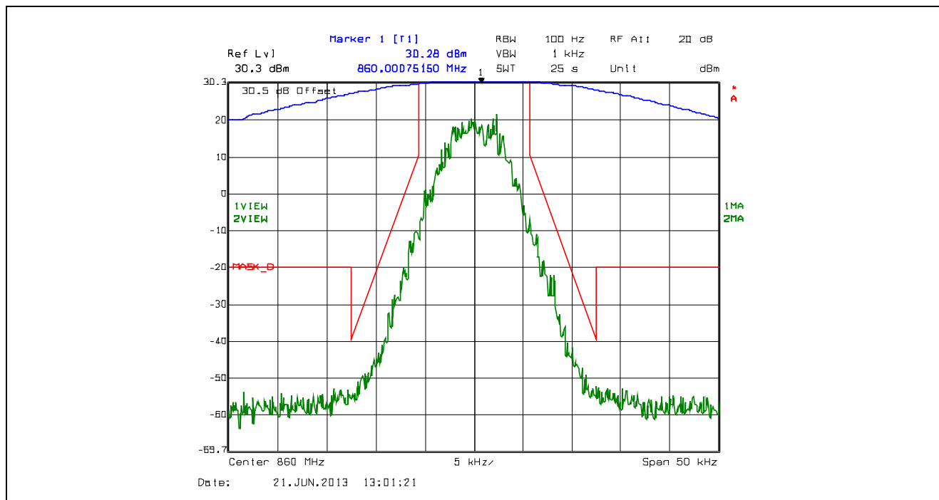
Plot 5.4.4.2.88. Emission Mask D, 12.5 kHz Channel Spacing, F1W, Low Power, 860.0 MHz
