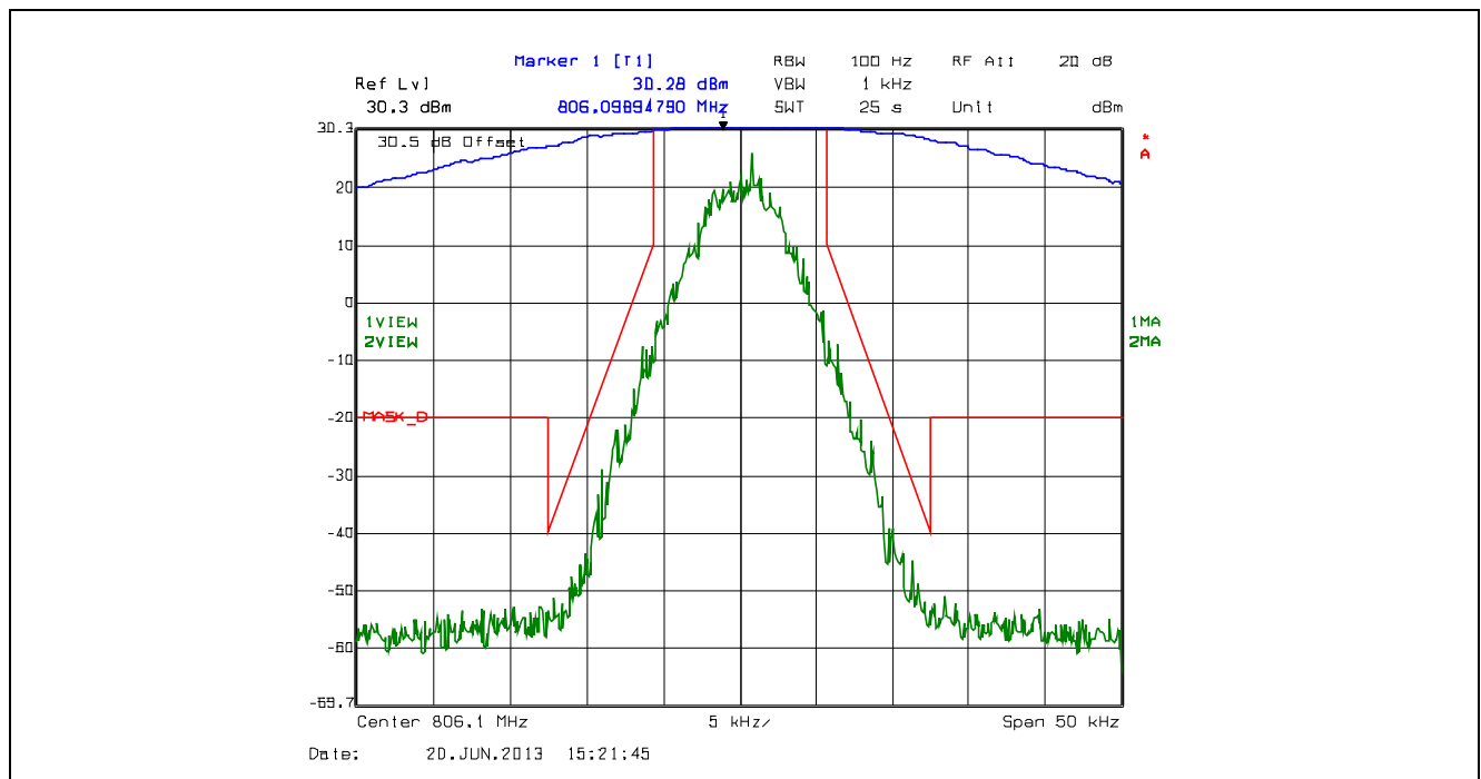
Plot 5.4.4.2.44. Emission Mask D, 12.5 kHz Channel Spacing, F1E, Low Power, 806.1 MHz
