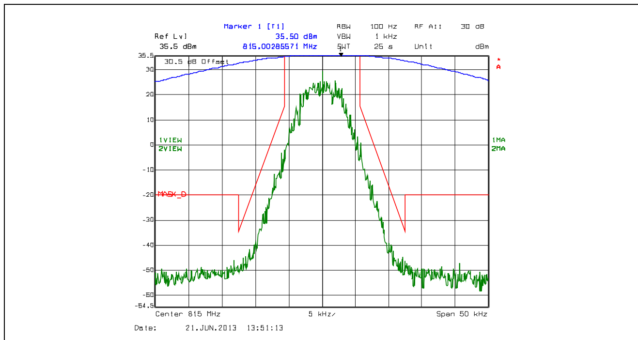
Plot 5.4.4.2.57. Emission Mask D, 12.5 kHz Channel Spacing, F1W, High Power, 815.0 MHz
