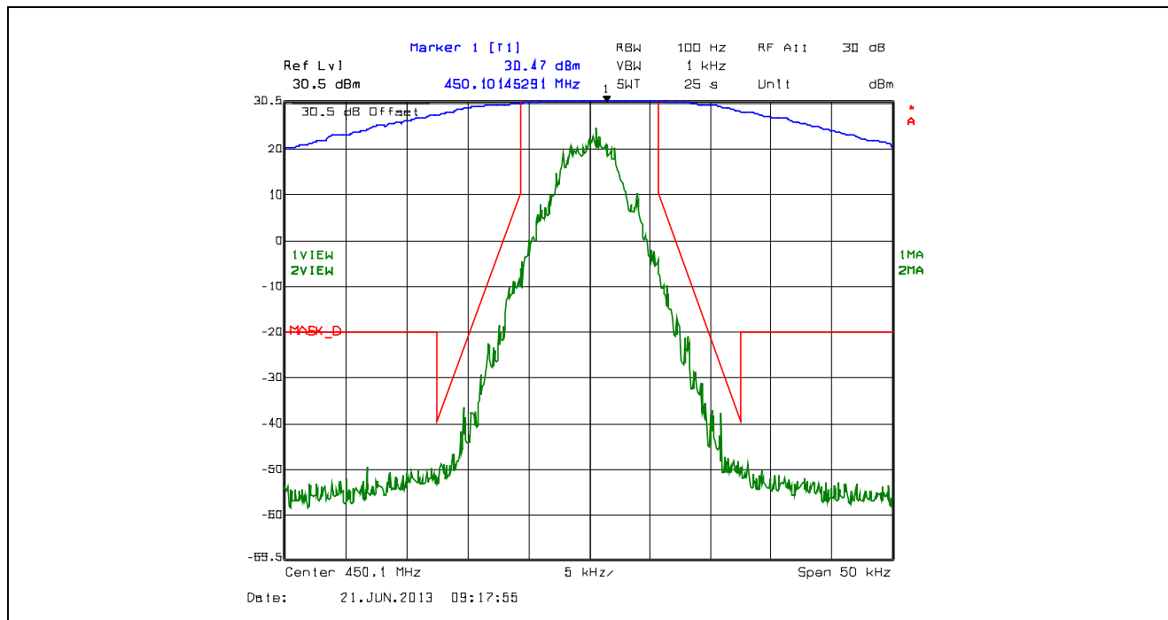
Plot 5.4.4.2.20. Emission Mask D, 12.5 kHz Channel Spacing, F1D, Low Power, 450.1 MHz
