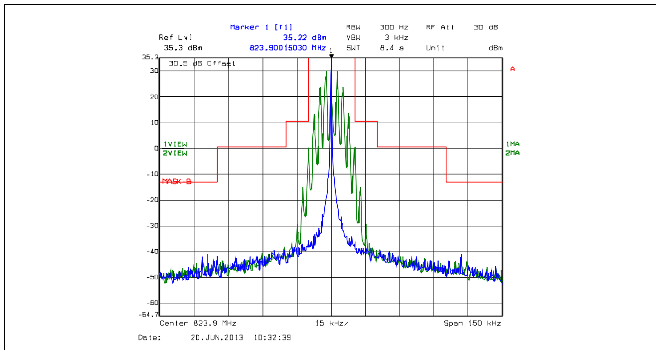
Plot 5.4.4.2.41. Emission Mask B, 25 kHz Channel Spacing, F3E, High Power, 823.9 MHz
