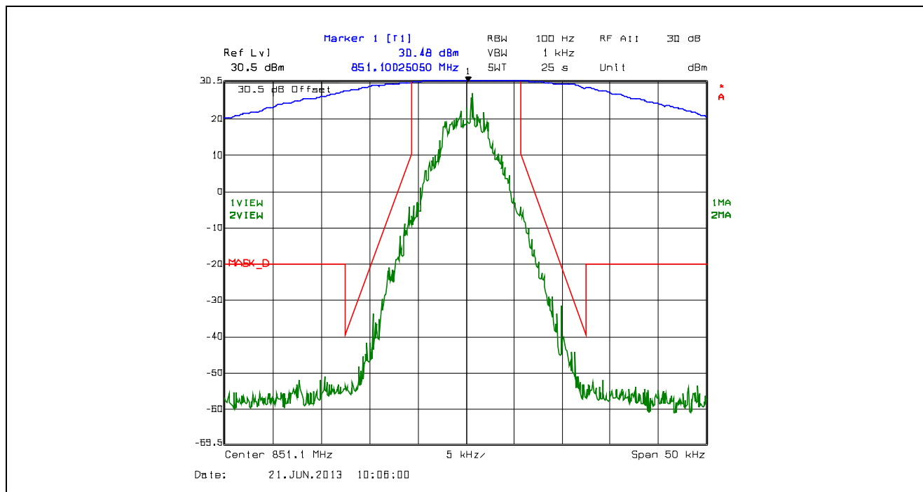
Plot 5.4.4.2.80. Emission Mask D, 12.5 kHz Channel Spacing, F1D, Low Power, 851.1 MHz
