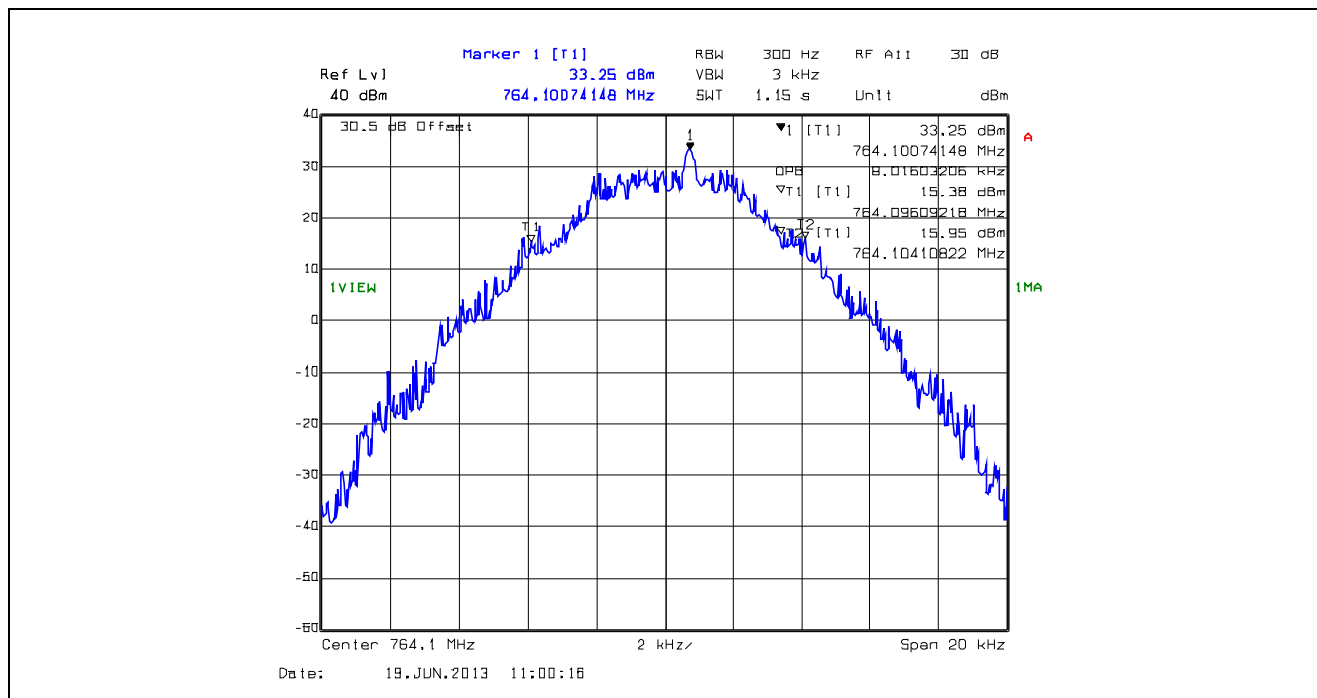
Plot 5.4.4.1.25. 99% Occupied Bandwidth, 12.5 kHz Channel Spacing, F1D, 764.1 MHz
