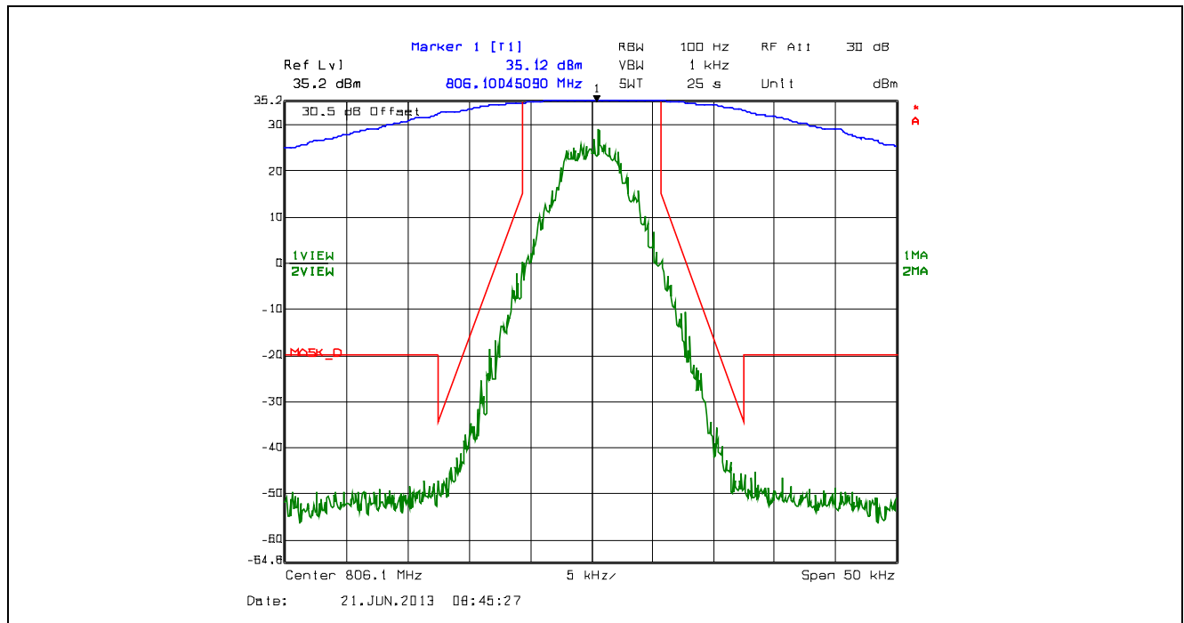
Plot 5.4.4.2.49. Emission Mask D, 12.5 kHz Channel Spacing, F1D, High Power, 806.1 MHz
