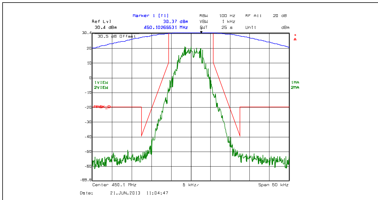
Plot 5.4.4.2.26. Emission Mask D, 12.5 kHz Channel Spacing, F1W, Low Power, 450.1 MHz
