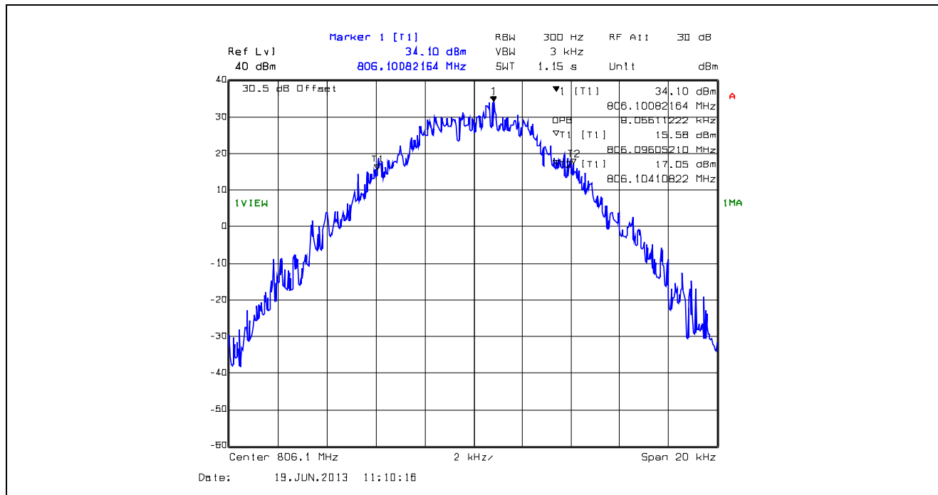
Plot 5.4.4.1.55. 99% Occupied Bandwidth, 12.5 kHz Channel Spacing, F1D, 806.1 MHz
