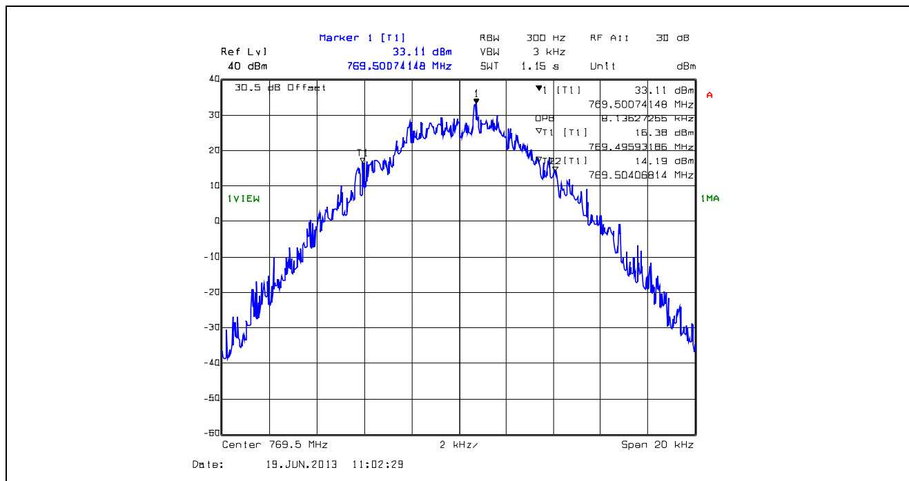
Plot 5.4.4.1.26. 99% Occupied Bandwidth, 12.5 kHz Channel Spacing, F1D, 769.5 MHz
