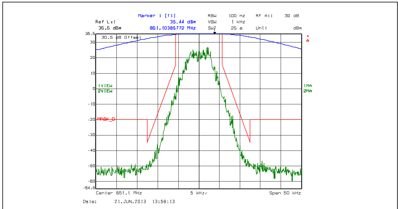
Plot 5.4.4.2.85. Emission Mask D, 12.5 kHz Channel Spacing, F1W, High Power, 851.1 MHz
