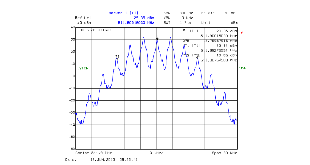
Plot 5.4.4.1.6. 99% Occupied Bandwidth, 25 kHz Channel Spacing, F3E, 511.9 MHz
