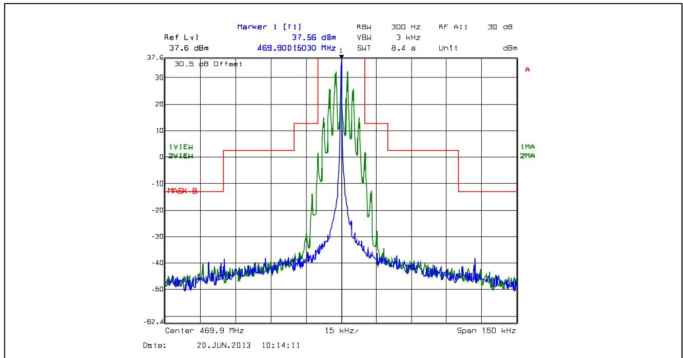
Plot 5.4.4.2.9. Emission Mask B, 25 kHz Channel Spacing, F3E, High Power, 469.9 MHz
