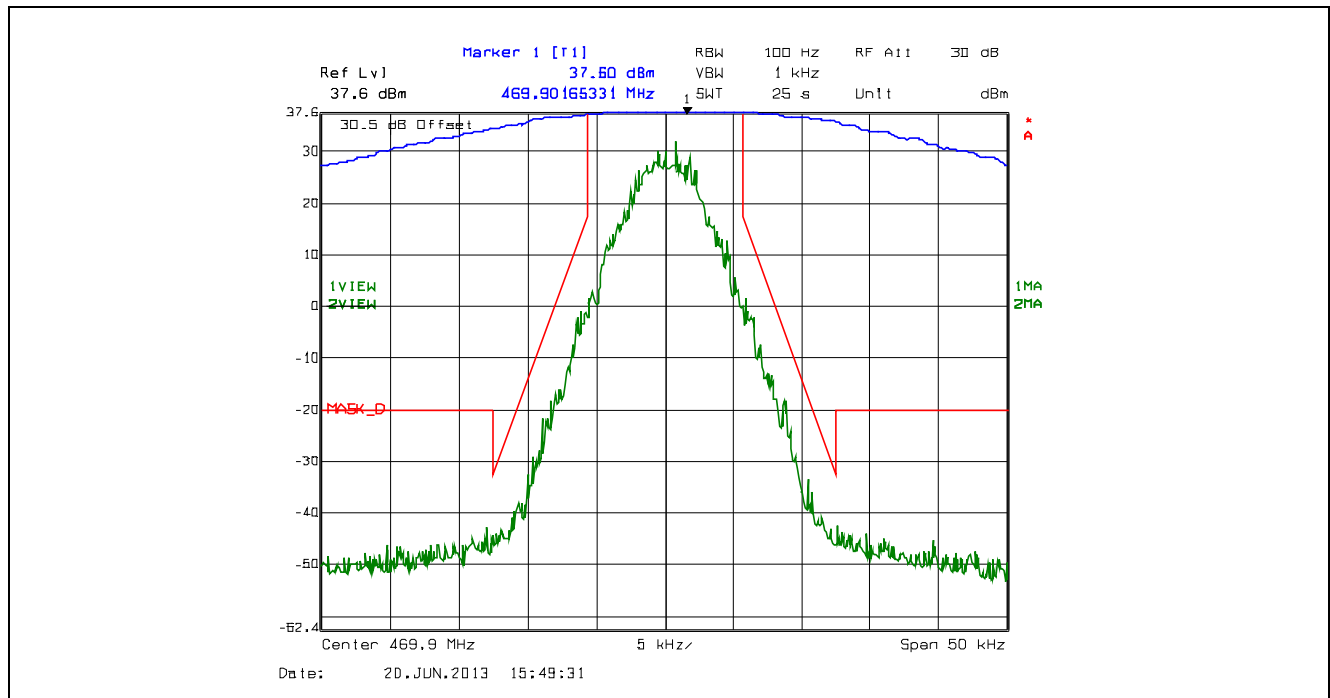
Plot 5.4.4.2.15. Emission Mask D, 12.5 kHz Channel Spacing, F1E, High Power, 469.9 MHz
