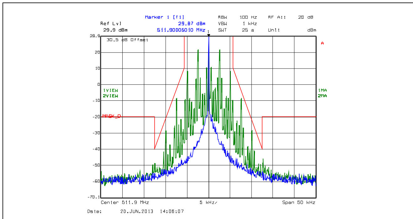
Plot 5.4.4.2.6. Emission Mask D, 12.5 kHz Channel Spacing, F3E, Low Power, 511.9 MHz
