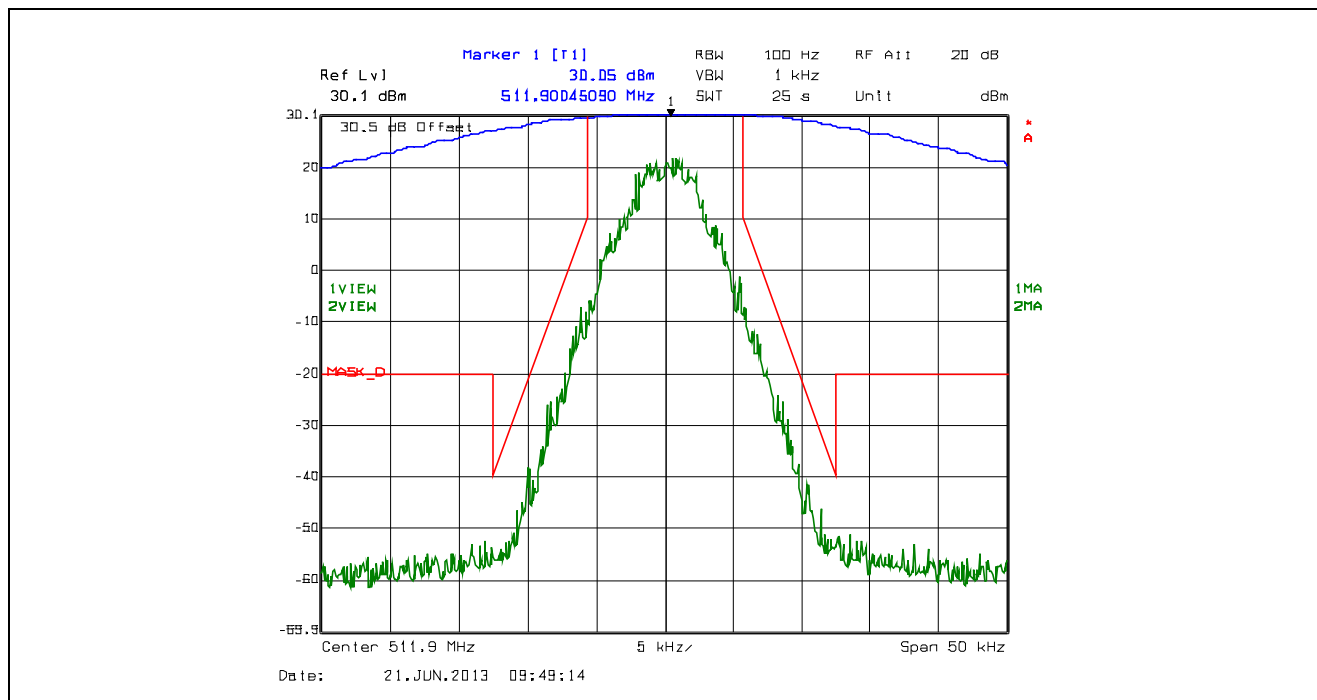
Plot 5.4.4.2.24. Emission Mask D, 12.5 kHz Channel Spacing, F1D, Low Power, 511.9 MHz
