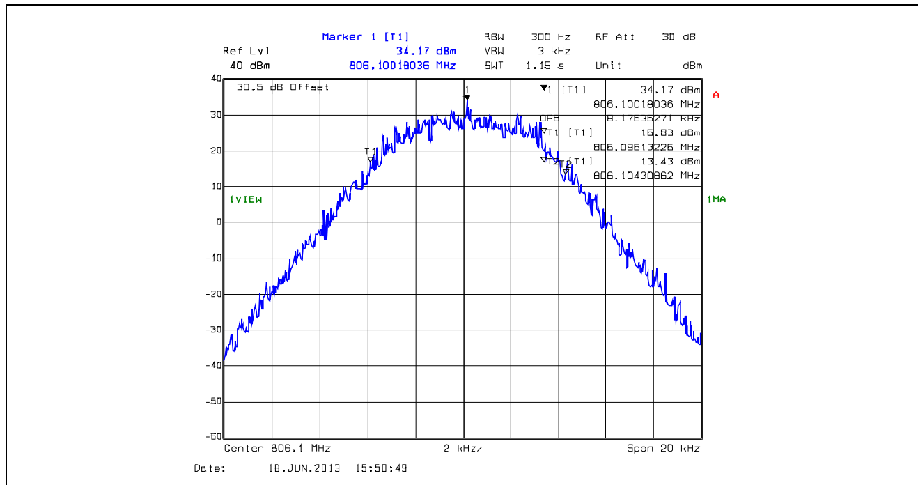
Plot 5.4.4.1.58. 99% Occupied Bandwidth, 12.5 kHz Channel Spacing, F1W, 806.1 MHz
