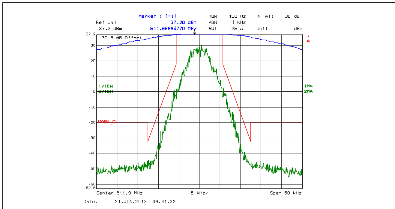
Plot 5.4.4.2.23. Emission Mask D, 12.5 kHz Channel Spacing, F1D, High Power, 511.9 MHz
