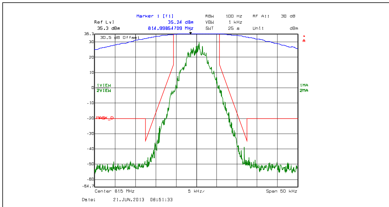
Plot 5.4.4.2.51. Emission Mask D, 12.5 kHz Channel Spacing, F1D, High Power, 815.0 MHz
