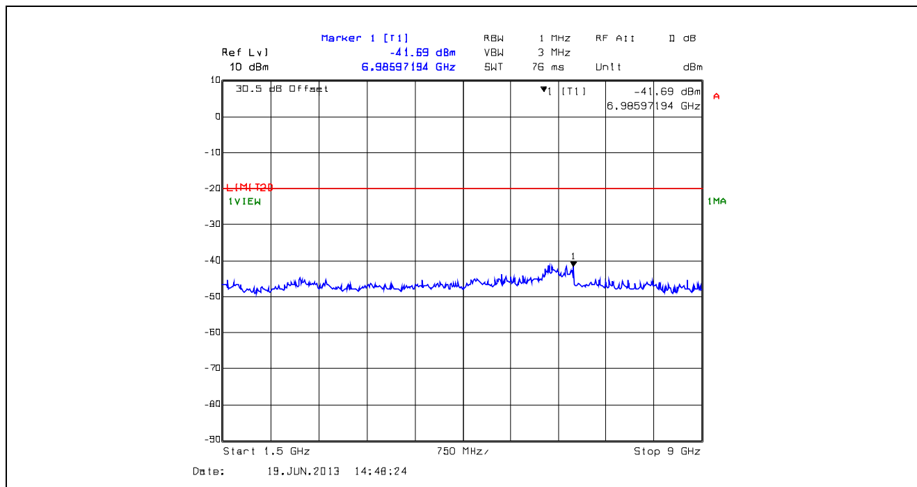
Plot 5.5.4.26. Conducted Transmitter Spurious Emissions, High Power, 794.1 MHz, 1.5 GHz - 9 GHz
