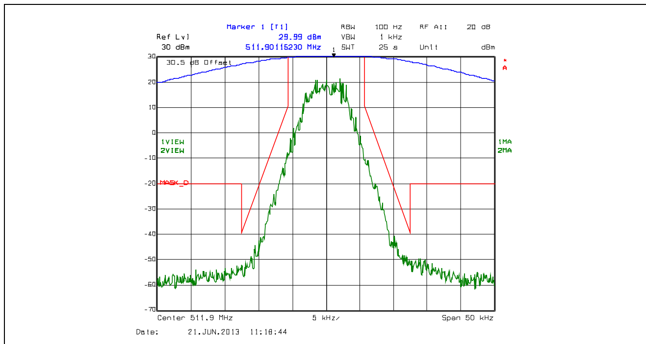
Plot 5.4.4.2.30. Emission Mask D, 12.5 kHz Channel Spacing, F1W, Low Power, 511.9 MHz
