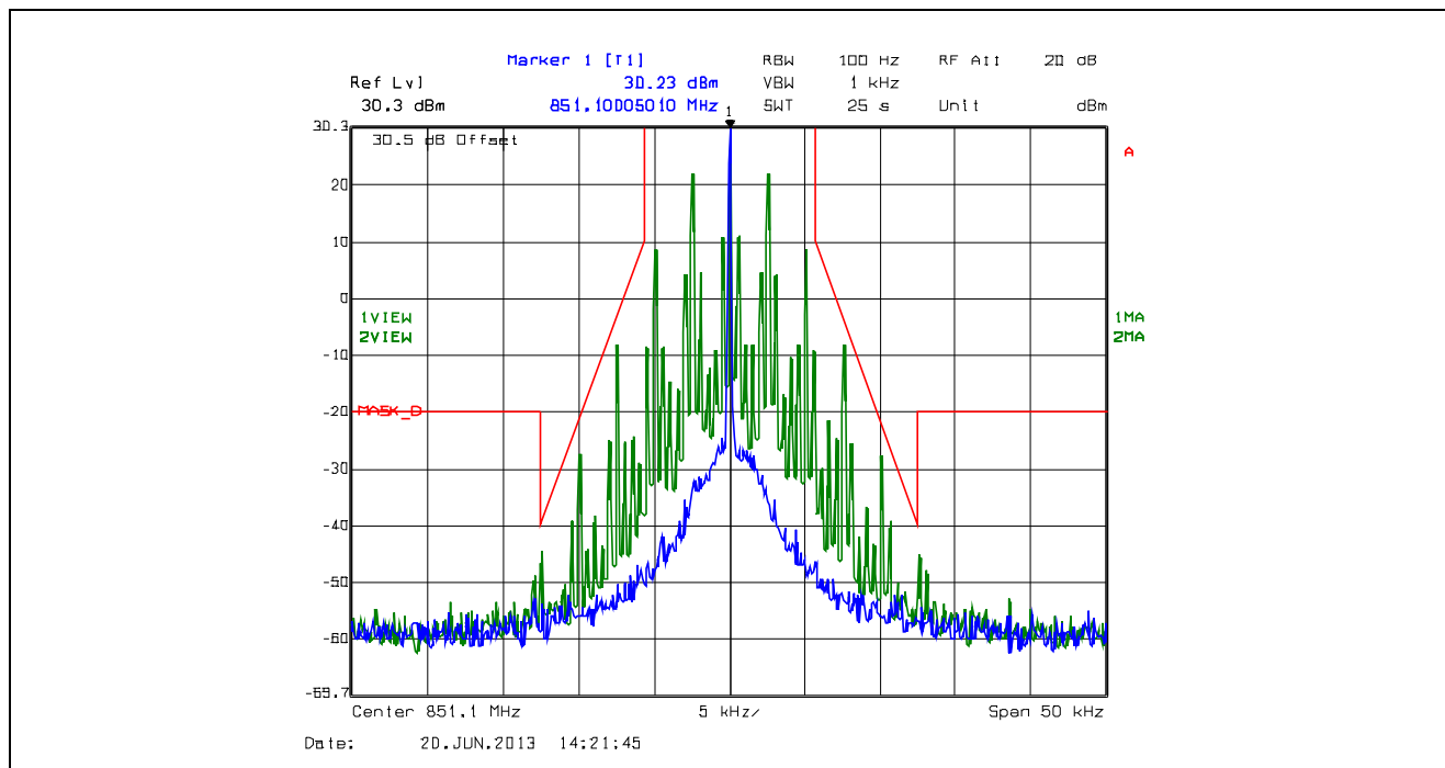
Plot 5.4.4.2.62. Emission Mask D, 12.5 kHz Channel Spacing, F3E, Low Power, 851.1 MHz
