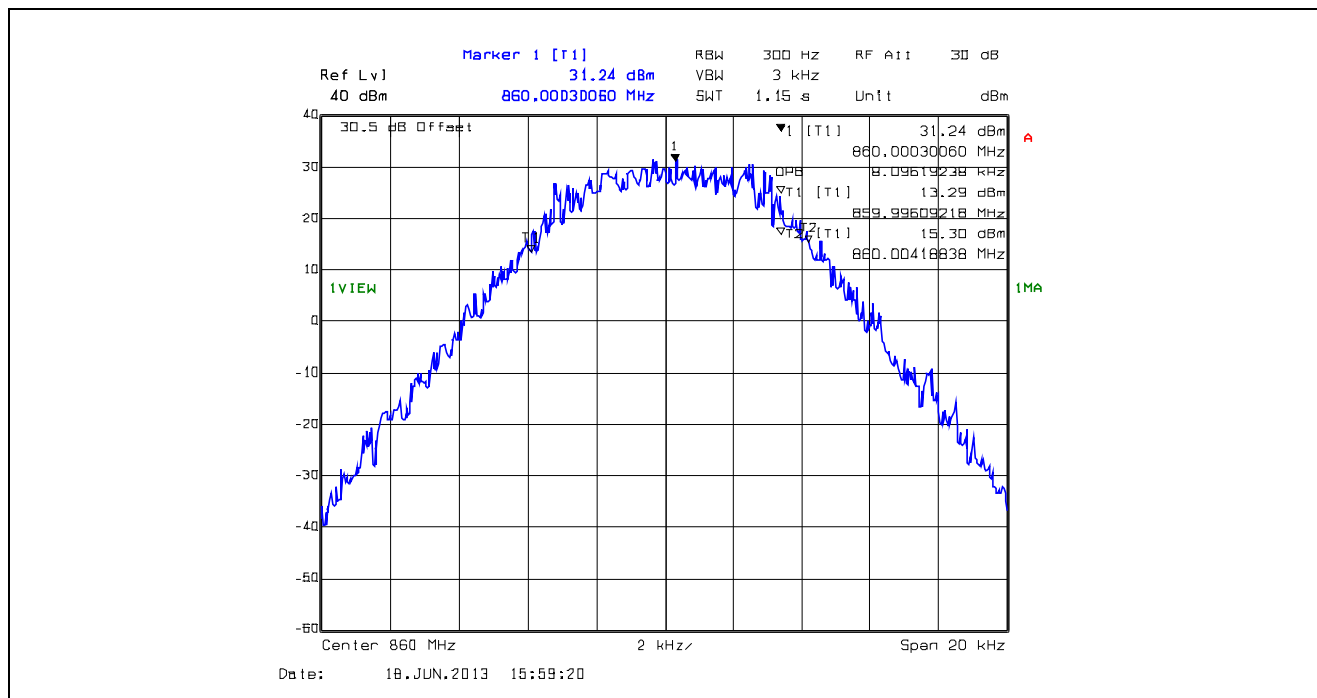
Plot 5.4.4.1.74. 99% Occupied Bandwidth, 12.5 kHz Channel Spacing, F1W, 860.0 MHz
