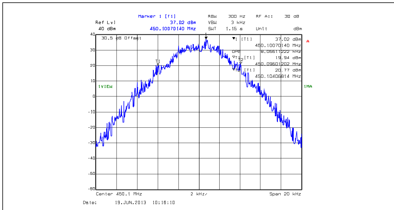
Plot 5.4.4.1.7. 99% Occupied Bandwidth, 12.5 kHz Channel Spacing, F1E, 450.1 MHz
