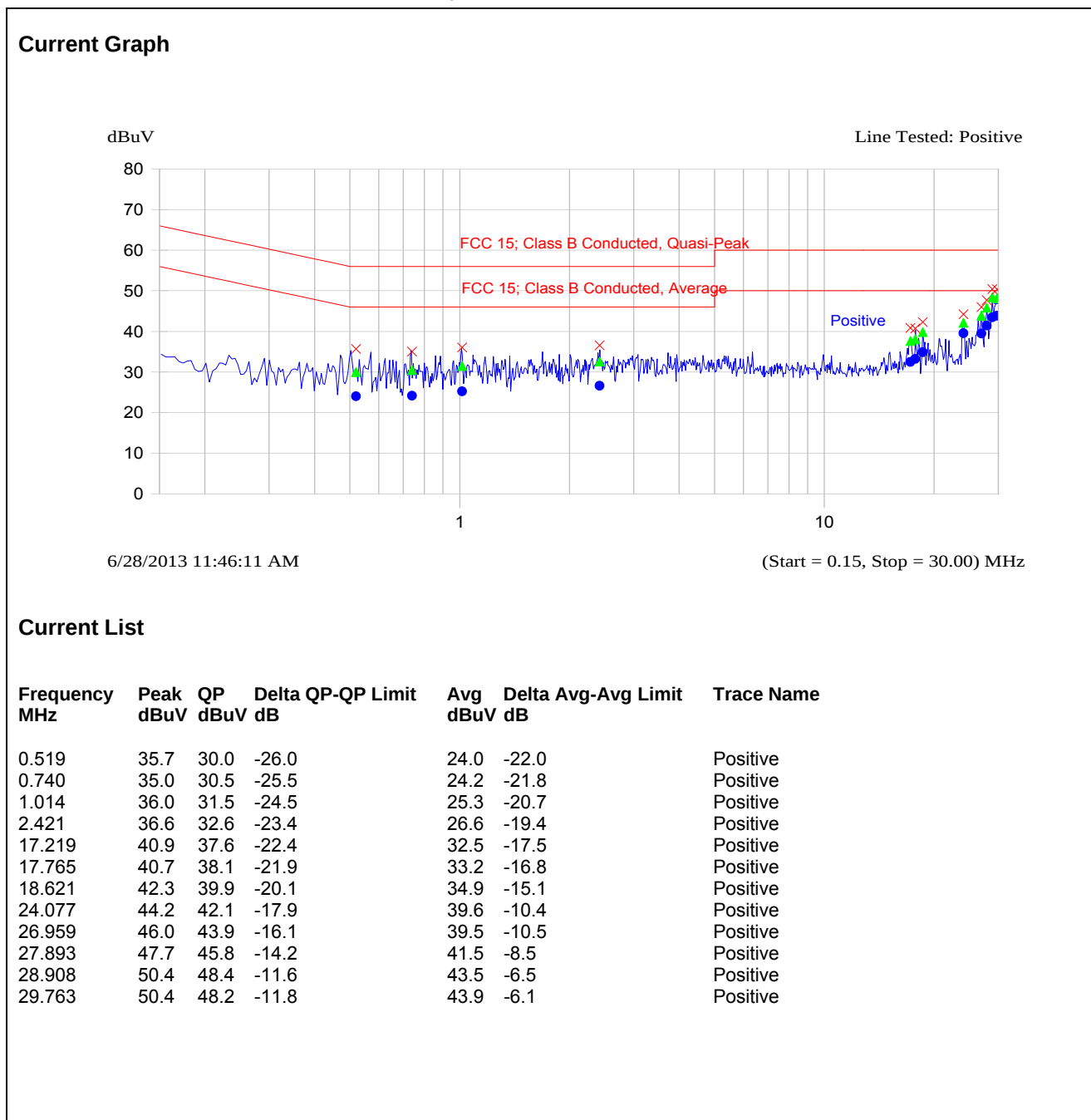
Plot 5.11.3.1. Power Line Conducted Emissions (Tx Mode) Line Voltage: 7.5 VDC; Line Tested: Positive
