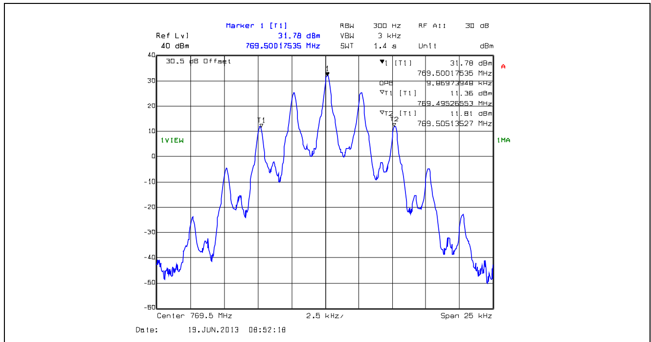
Plot 5.4.4.1.17. 99% Occupied Bandwidth, 12.5 kHz Channel Spacing, F3E, 769.5 MHz
