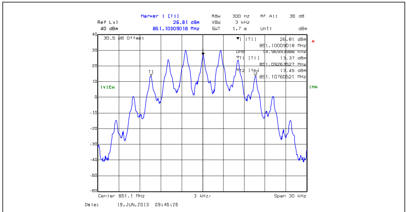
Plot 5.4.4.1.64. 99% Occupied Bandwidth, 25 kHz Channel Spacing, F3E, 851.1 MHz
