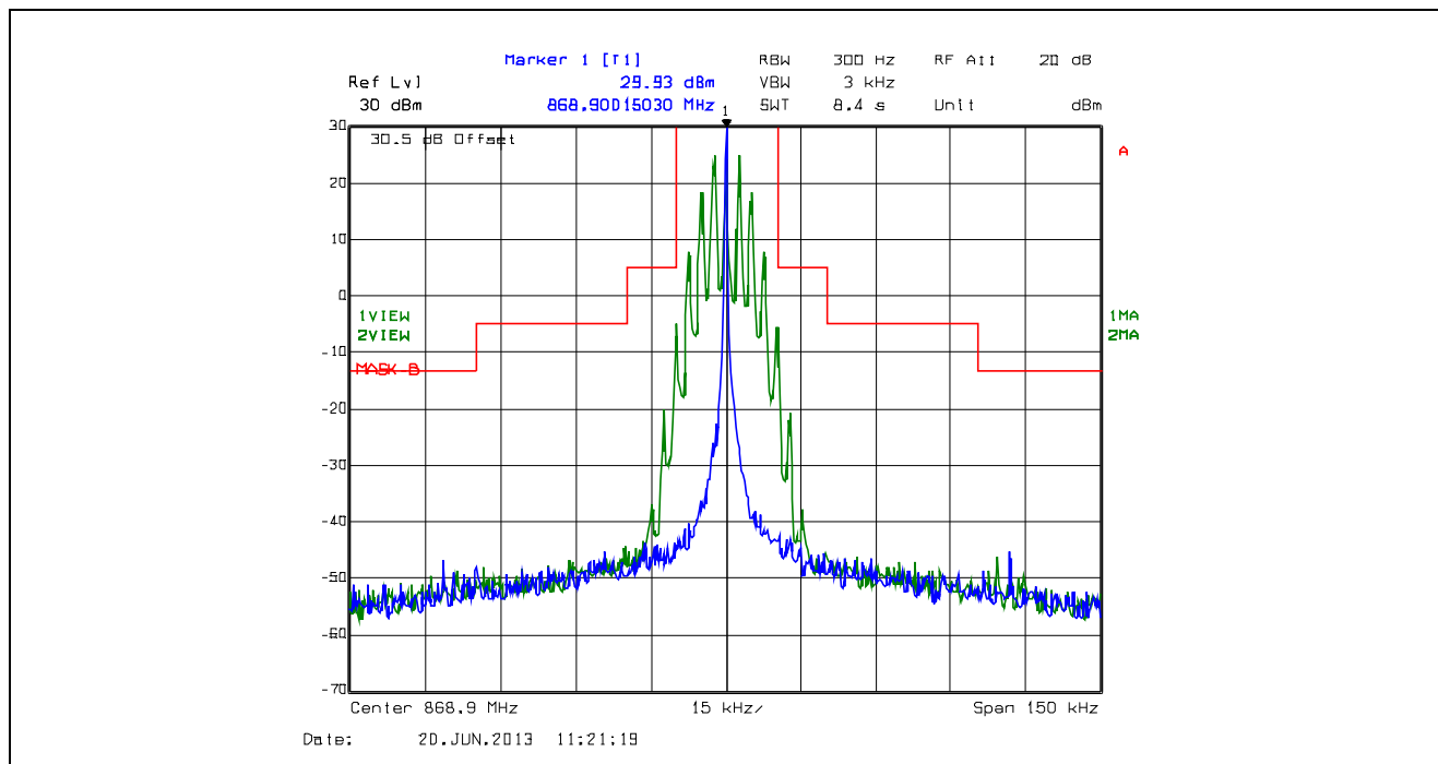
Plot 5.4.4.2.72. Emission Mask B, 25 kHz Channel Spacing, F3E, Low Power, 868.9 MHz
