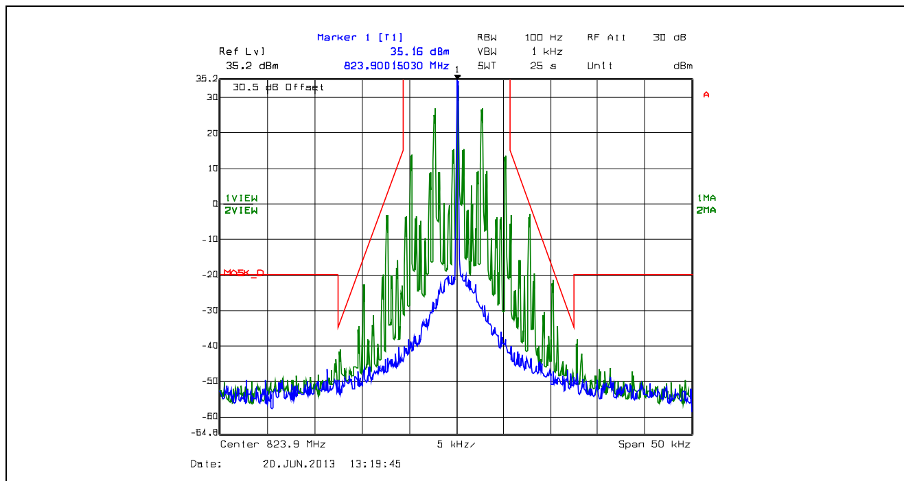
Plot 5.4.4.2.35. Emission Mask D, 12.5 kHz Channel Spacing, F3E, High Power, 823.9 MHz
