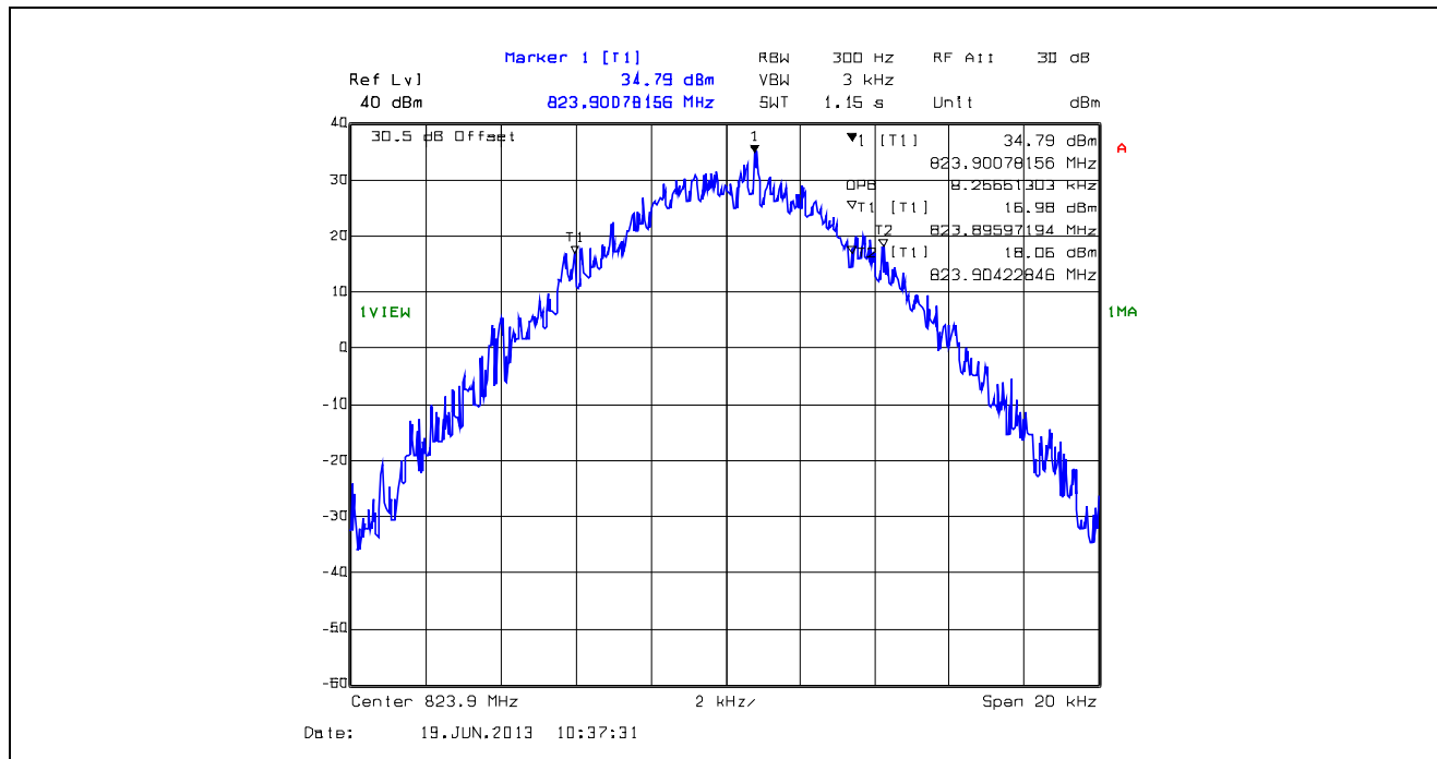
Plot 5.4.4.1.54. 99% Occupied Bandwidth, 12.5 kHz Channel Spacing, F1E, 823.9 MHz
