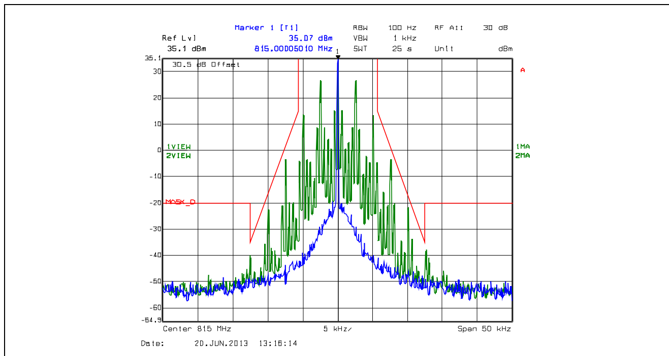
Plot 5.4.4.2.33. Emission Mask D, 12.5 kHz Channel Spacing, F3E, High Power, 815.0 MHz
