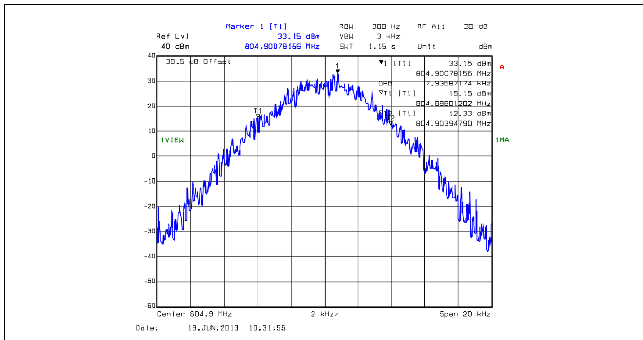
Plot 5.4.4.1.39. 99% Occupied Bandwidth, 12.5 kHz Channel Spacing, F1E, 804.9 MHz
