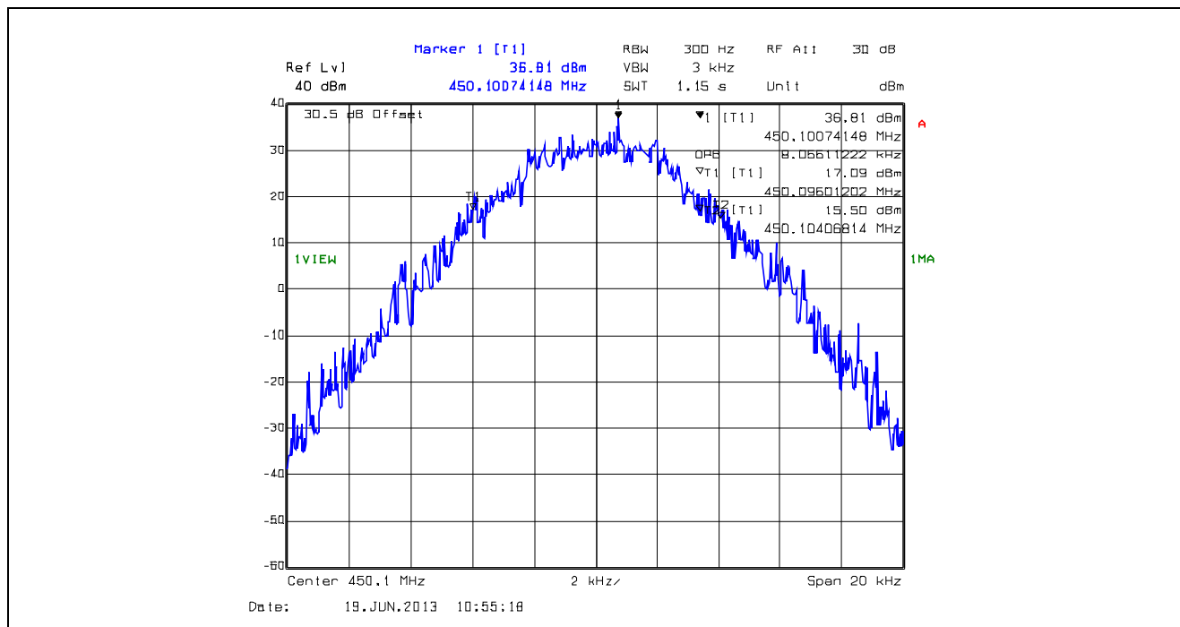
Plot 5.4.4.1.10. 99% Occupied Bandwidth, 12.5 kHz Channel Spacing, F1D, 450.1 MHz
