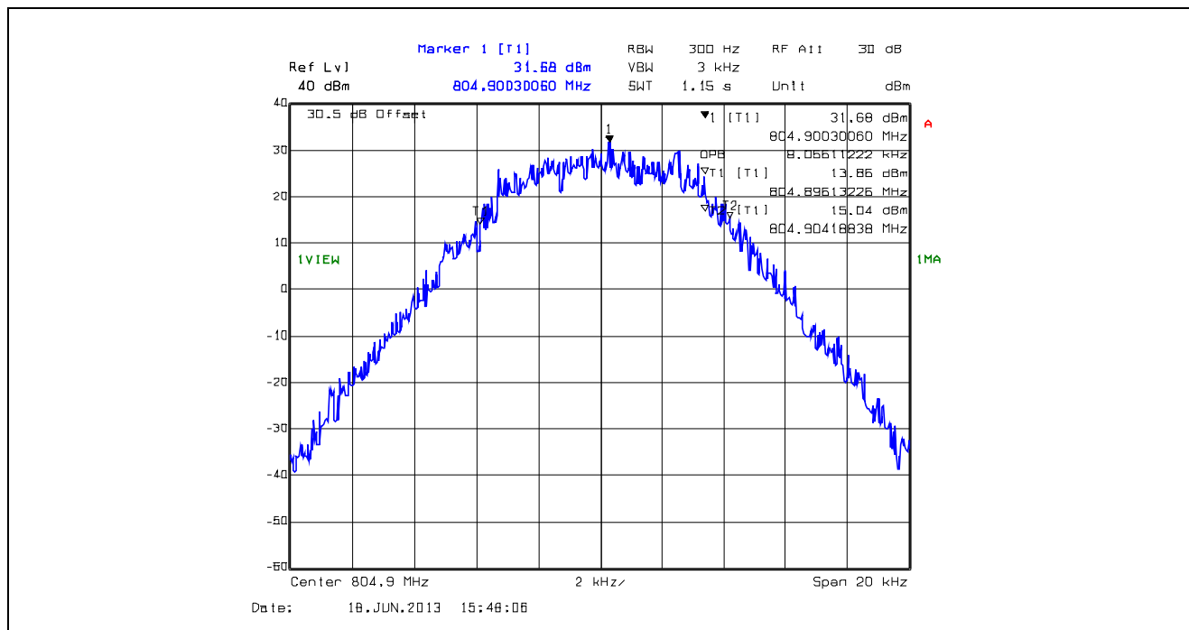
Plot 5.4.4.1.45. 99% Occupied Bandwidth, 12.5 kHz Channel Spacing, F1W, 804.9 MHz
