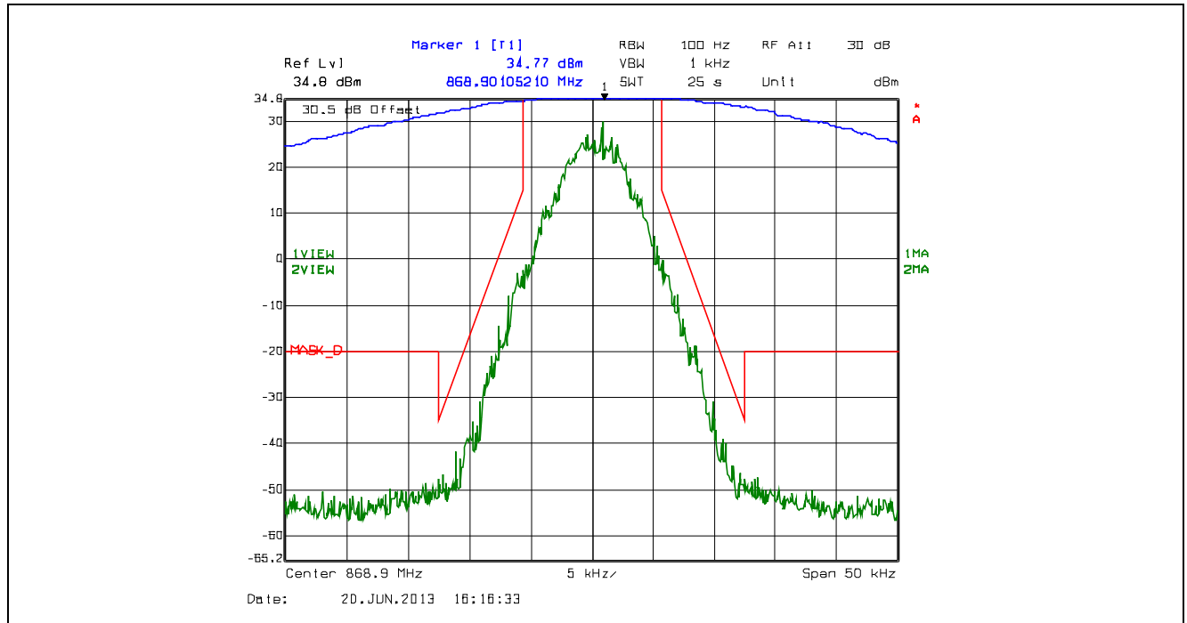
Plot 5.4.4.2.77. Emission Mask D, 12.5 kHz Channel Spacing, F1E, High Power, 868.9 MHz
