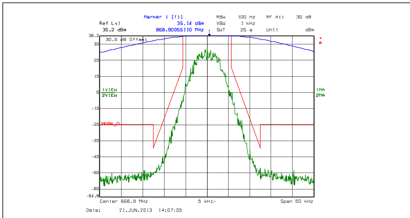
Plot 5.4.4.2.89. Emission Mask D, 12.5 kHz Channel Spacing, F1W, High Power, 868.9 MHz
