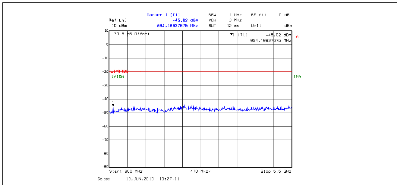
Plot 5.5.4.2. Conducted Transmitter Spurious Emissions, High Power, 450.1 MHz, 800 MHz – 5.5 GHz
