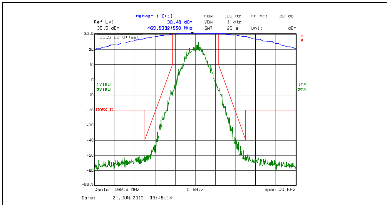
Plot 5.4.4.2.22. Emission Mask D, 12.5 kHz Channel Spacing, F1D, Low Power, 469.9 MHz
