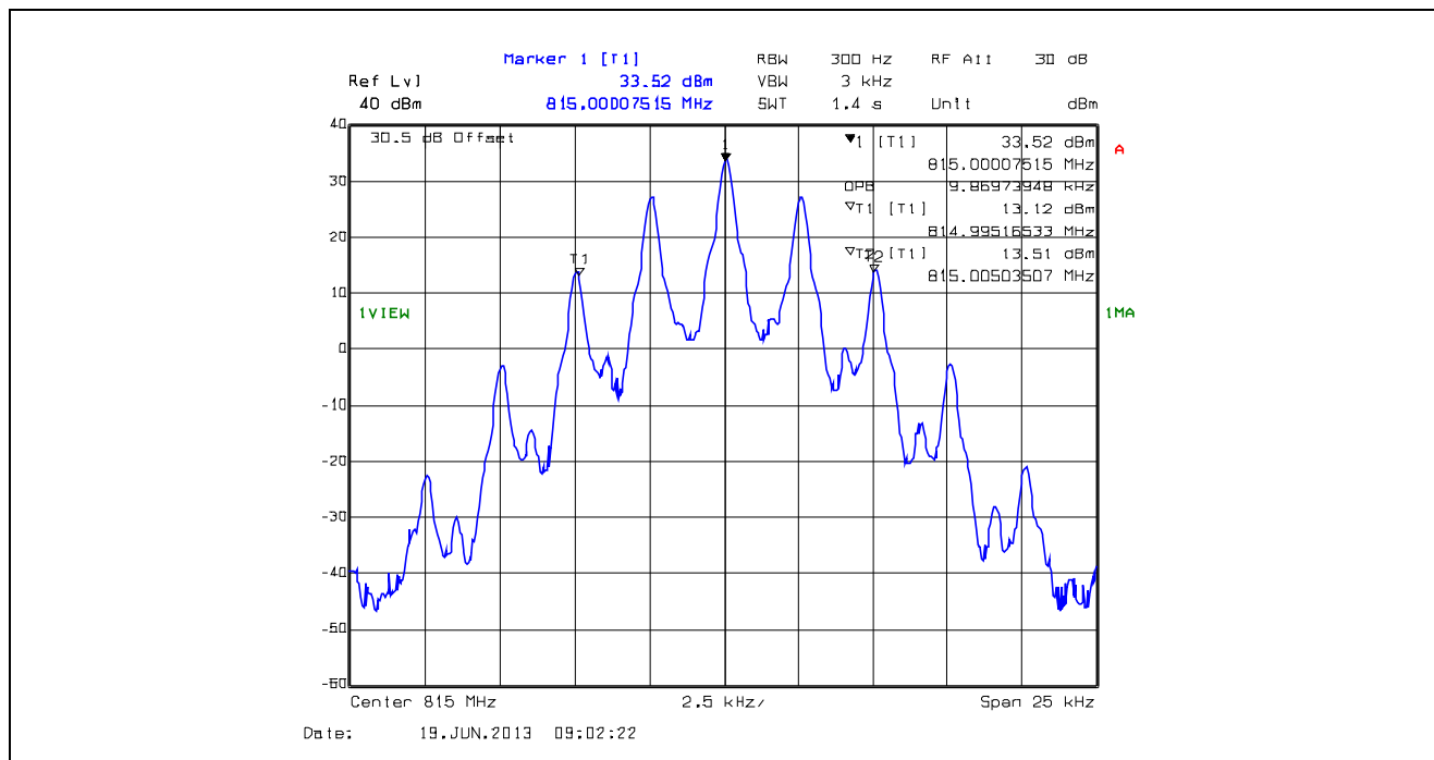
Plot 5.4.4.1.47. 99% Occupied Bandwidth, 12.5 kHz Channel Spacing, F3E, 815.0 MHz
