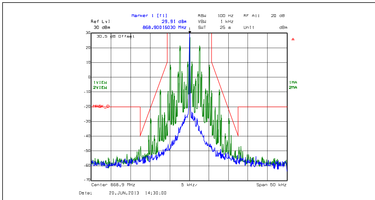
Plot 5.4.4.2.66. Emission Mask D, 12.5 kHz Channel Spacing, F3E, Low Power, 868.9 MHz
