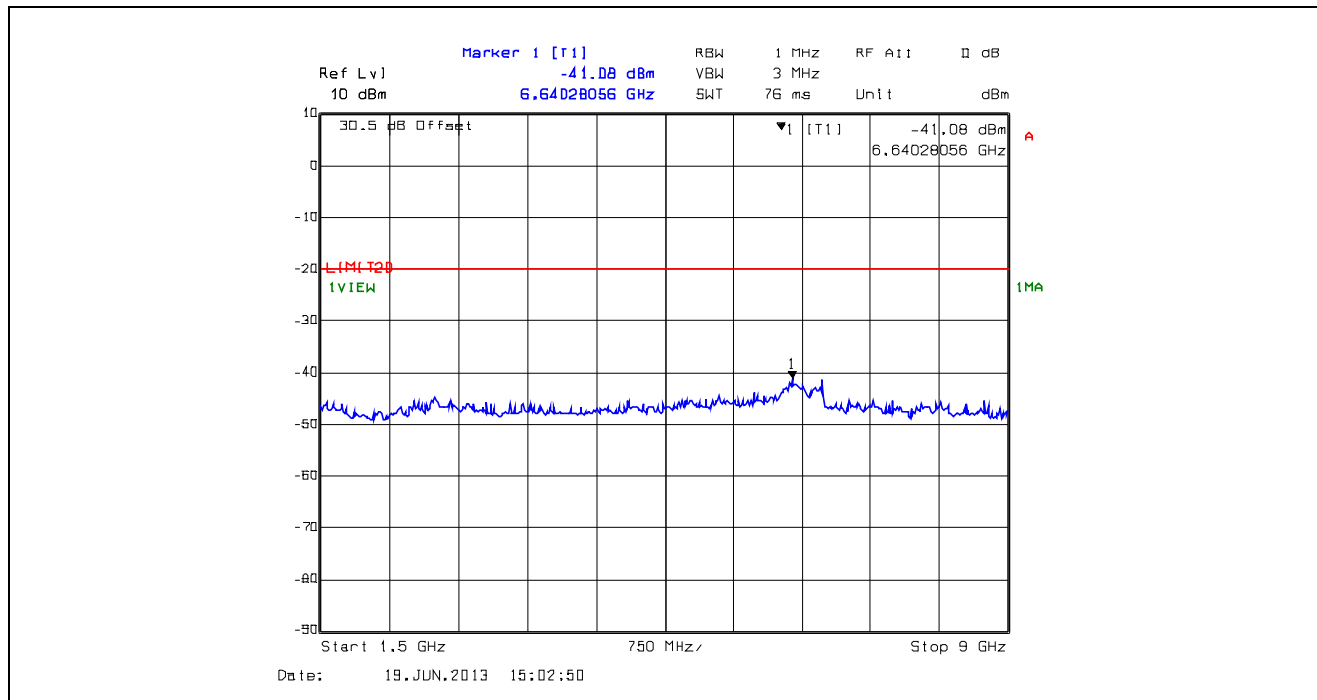
Plot 5.5.4.36. Conducted Transmitter Spurious Emissions, Low Power, 804.9 MHz, 1.5 GHz - 9 GHz
