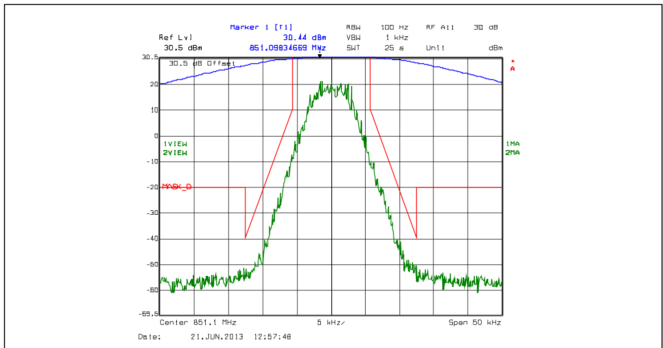
Plot 5.4.4.2.86. Emission Mask D, 12.5 kHz Channel Spacing, F1W, Low Power, 851.1 MHz
