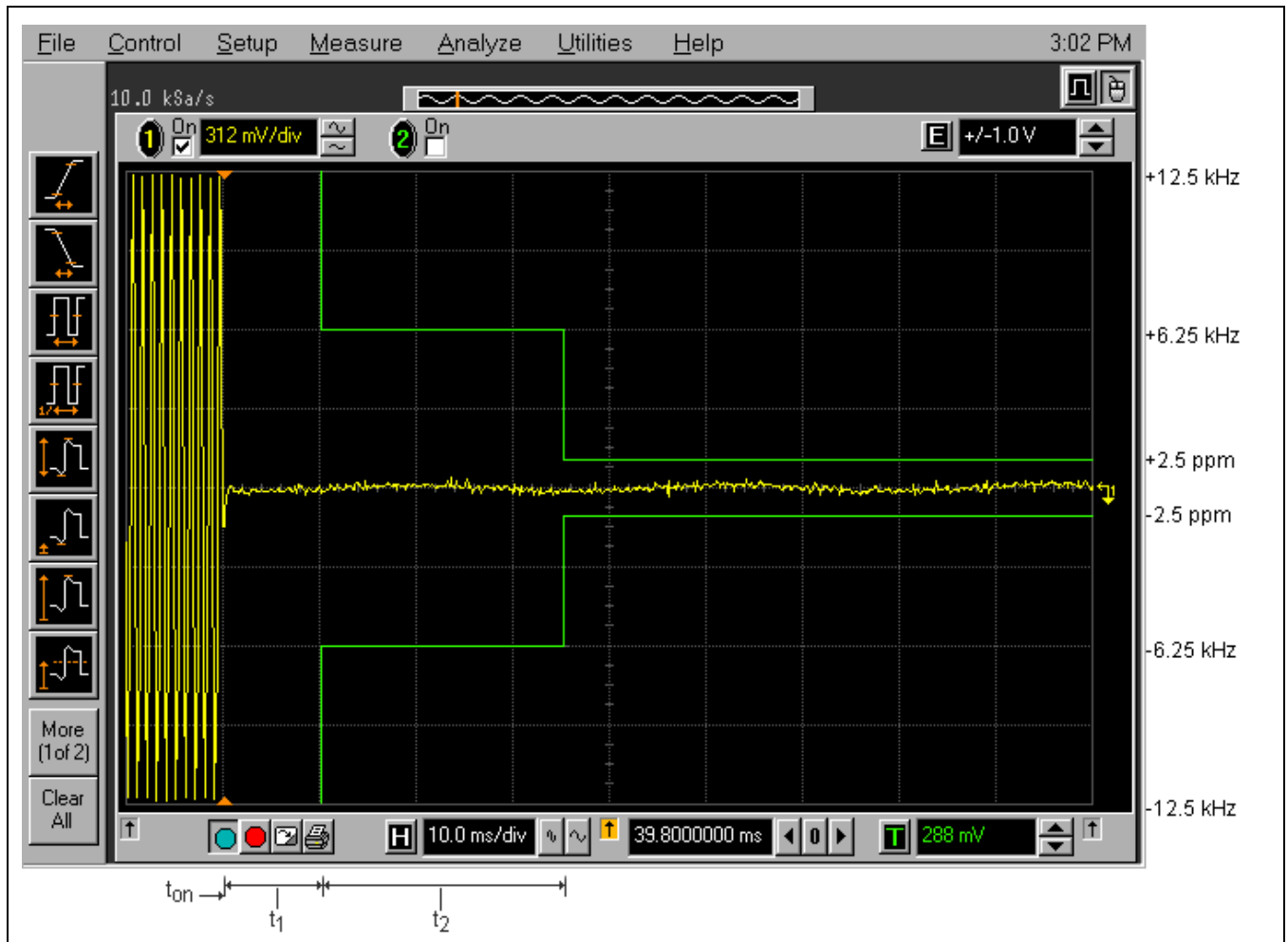
Plot 5.8.4.1. Transient Frequency Behavior on 12.5 kHz Channels Test Frequency: 450.1 MHz; Power: 5 W; Test Conditions: Switch on condition t_{on} , t_1 , and t_2
