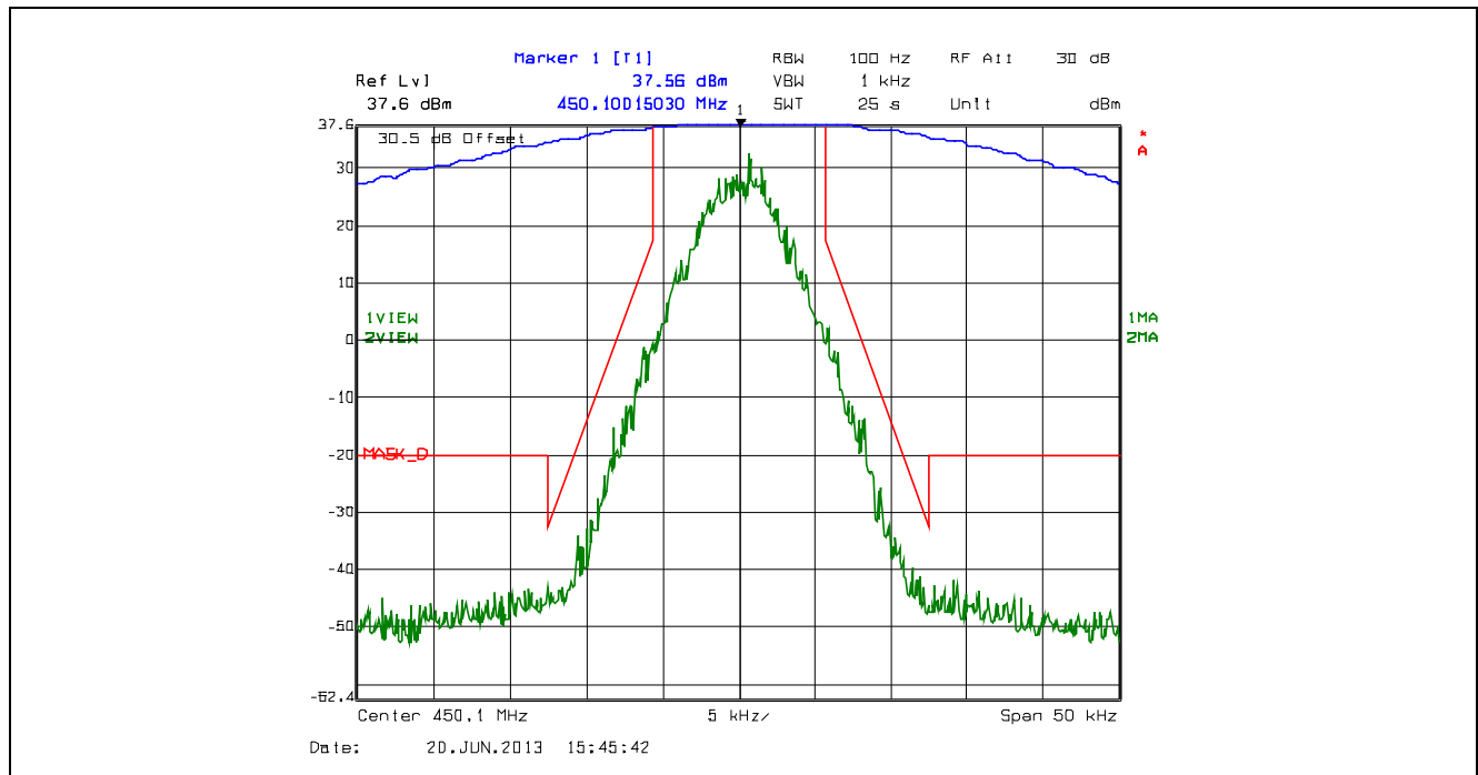
Plot 5.4.4.2.13. Emission Mask D, 12.5 kHz Channel Spacing, F1E, High Power, 450.1 MHz
