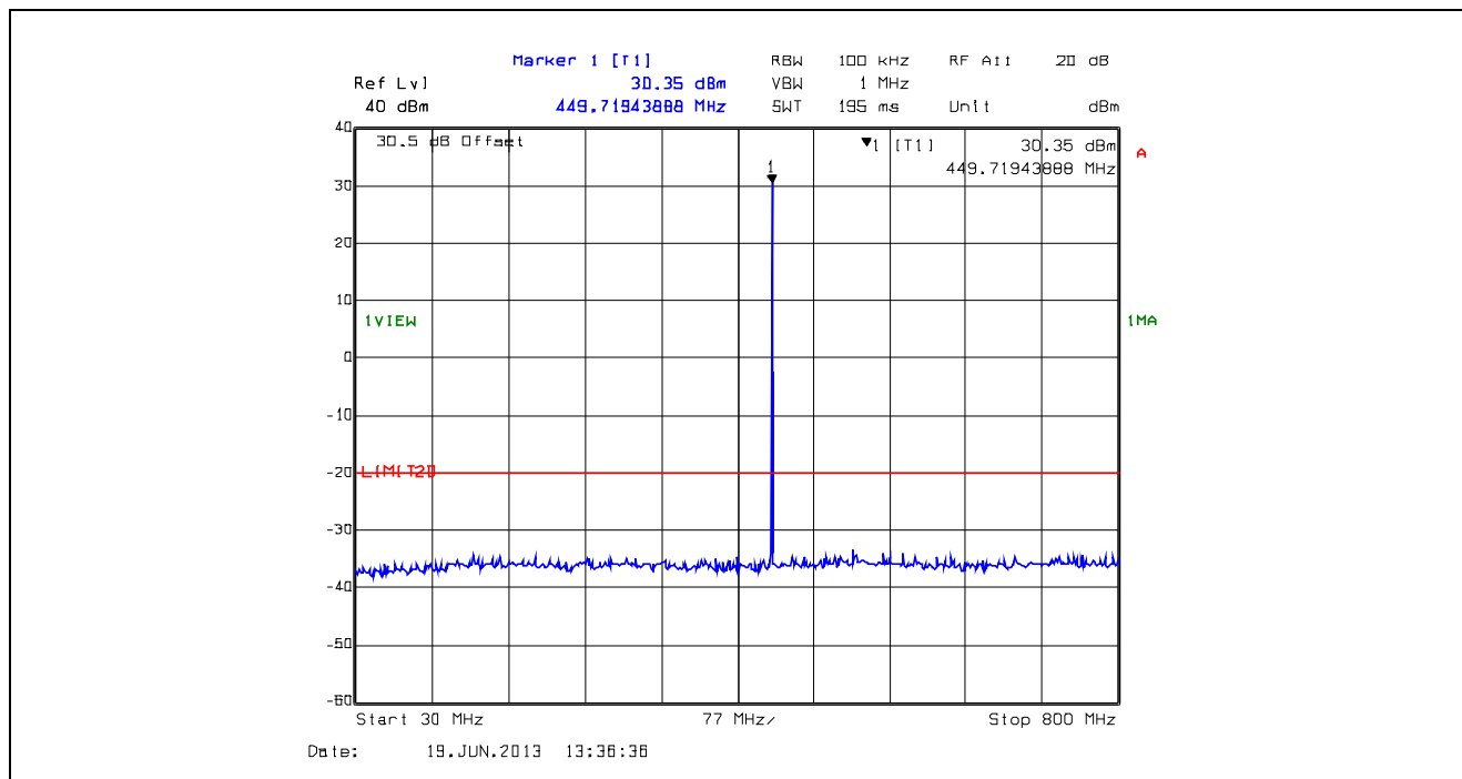
Plot 5.5.4.3. Conducted Transmitter Spurious Emissions, Low Power, 450.1 MHz, 30 MHz - 800 MHz
