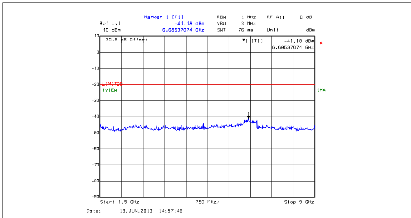
Plot 5.5.4.16. Conducted Transmitter Spurious Emissions, Low Power, 764.1 MHz, 1.5 GHz - 9 GHz
