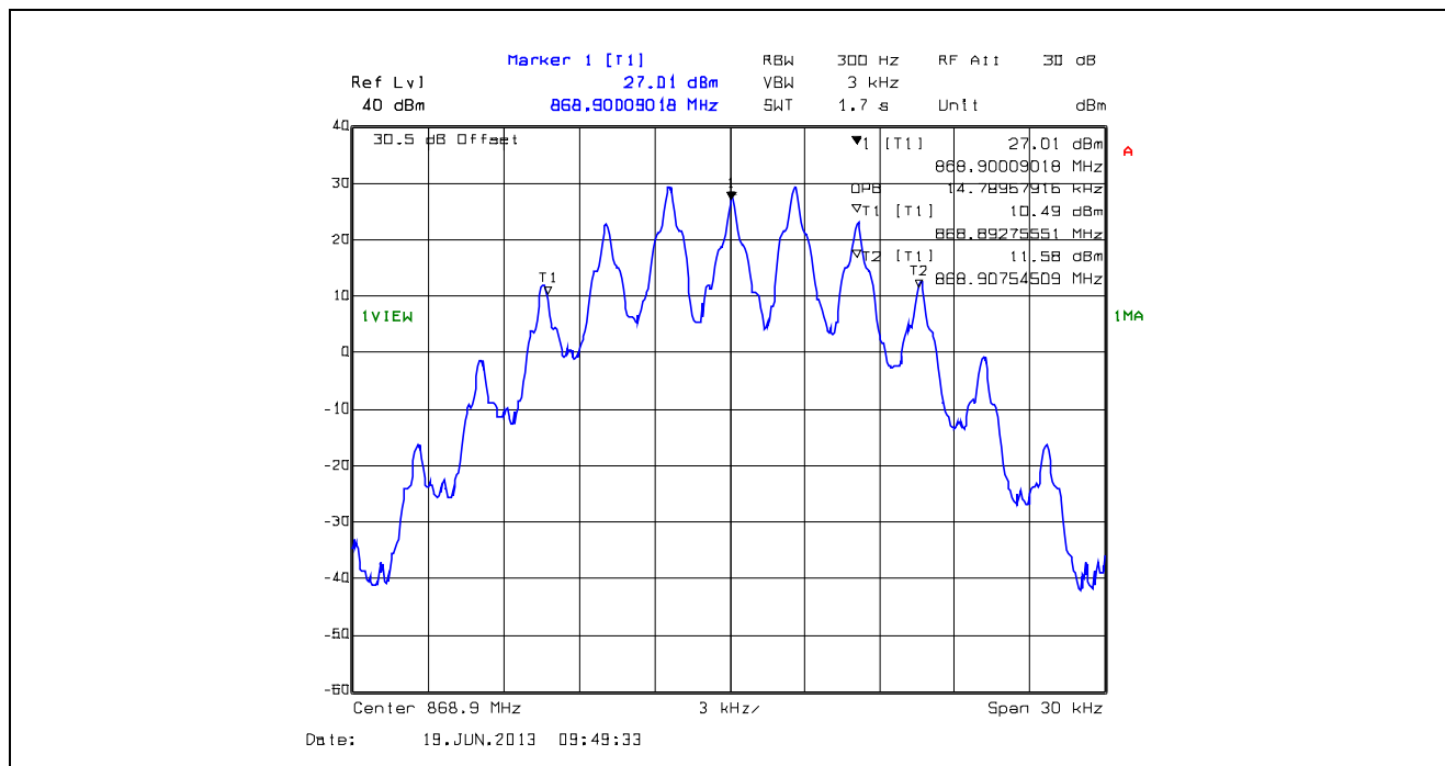
Plot 5.4.4.1.66. 99% Occupied Bandwidth, 25 kHz Channel Spacing, F3E, 868.9 MHz
