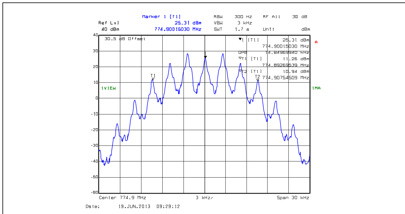
Plot 5.4.4.1.21. 99% Occupied Bandwidth, 25 kHz Channel Spacing, F3E, 774.9MHz
