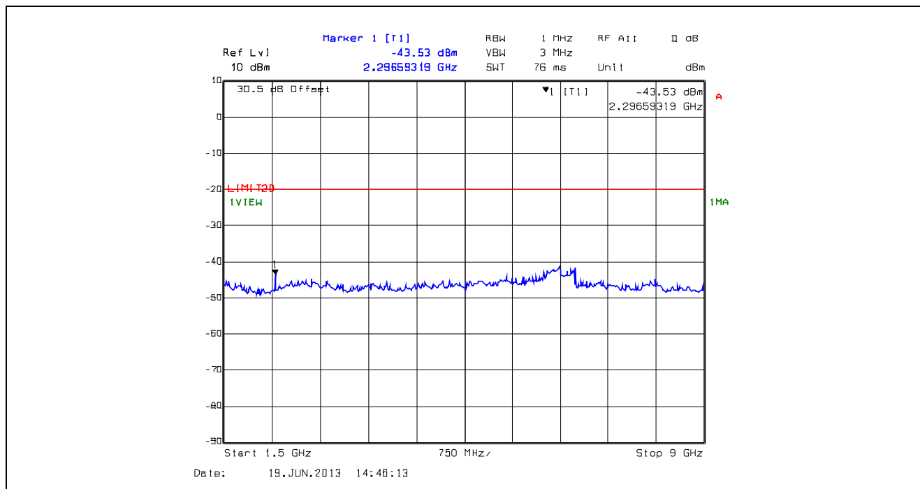
Plot 5.5.4.18. Conducted Transmitter Spurious Emissions, High Power, 769.5 MHz, 1.5 GHz - 9 GHz
