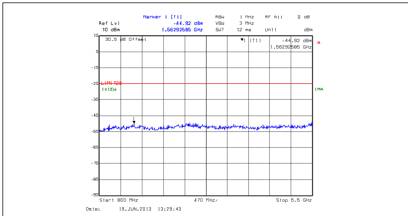
Plot 5.5.4.10. Conducted Transmitter Spurious Emissions, High Power, 511.9 MHz, 800 MHz - 5.5 GHz
