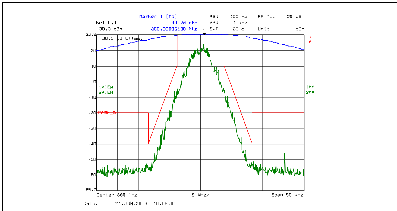
Plot 5.4.4.2.82. Emission Mask D, 12.5 kHz Channel Spacing, F1D, Low Power, 860.0 MHz
