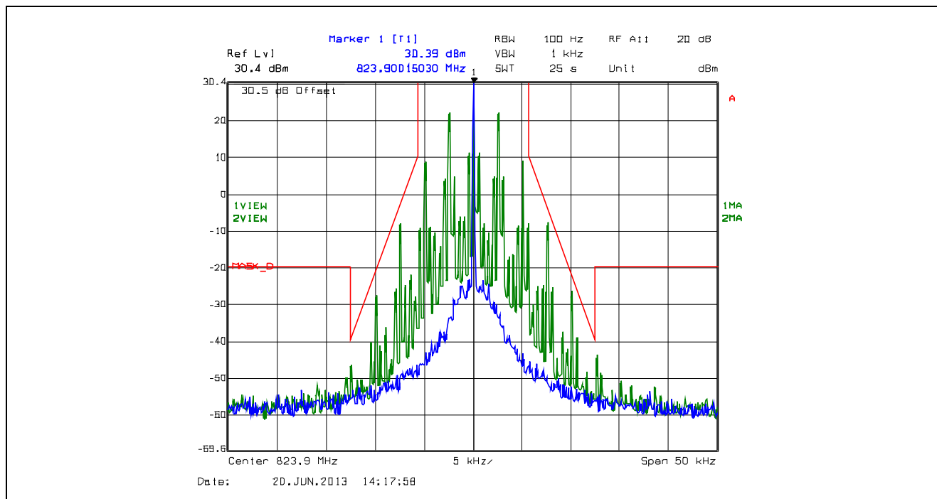
Plot 5.4.4.2.36. Emission Mask D, 12.5 kHz Channel Spacing, F3E, Low Power, 823.9 MHz
