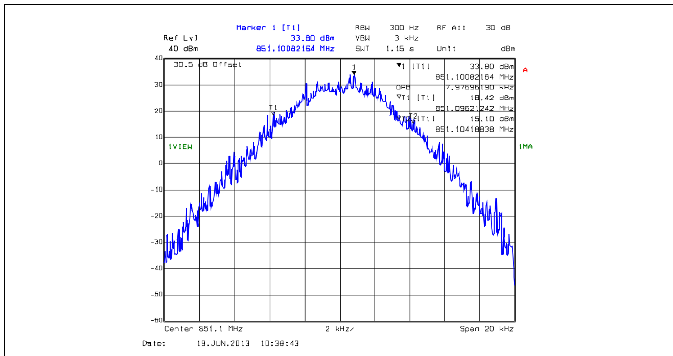
Plot 5.4.4.1.67. 99% Occupied Bandwidth, 12.5 kHz Channel Spacing, F1E, 851.1 MHz
