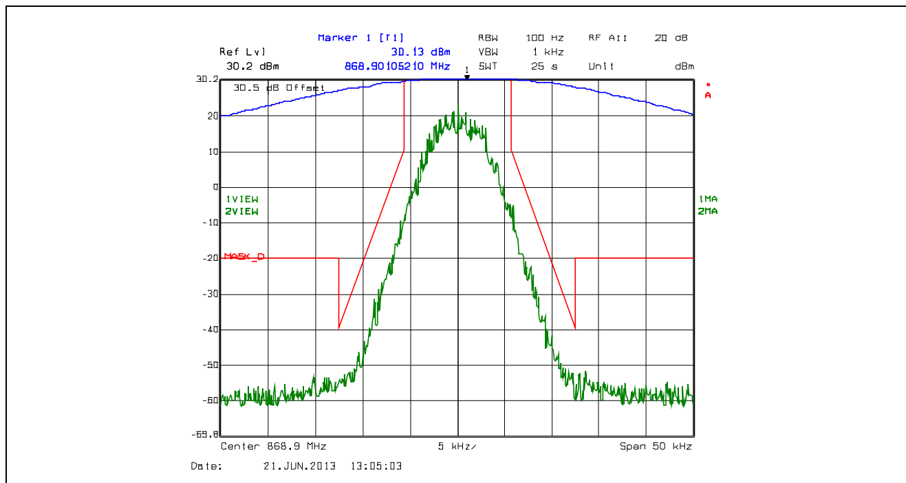
Plot 5.4.4.2.90. Emission Mask D, 12.5 kHz Channel Spacing, F1W, Low Power, 868.9 MHz
