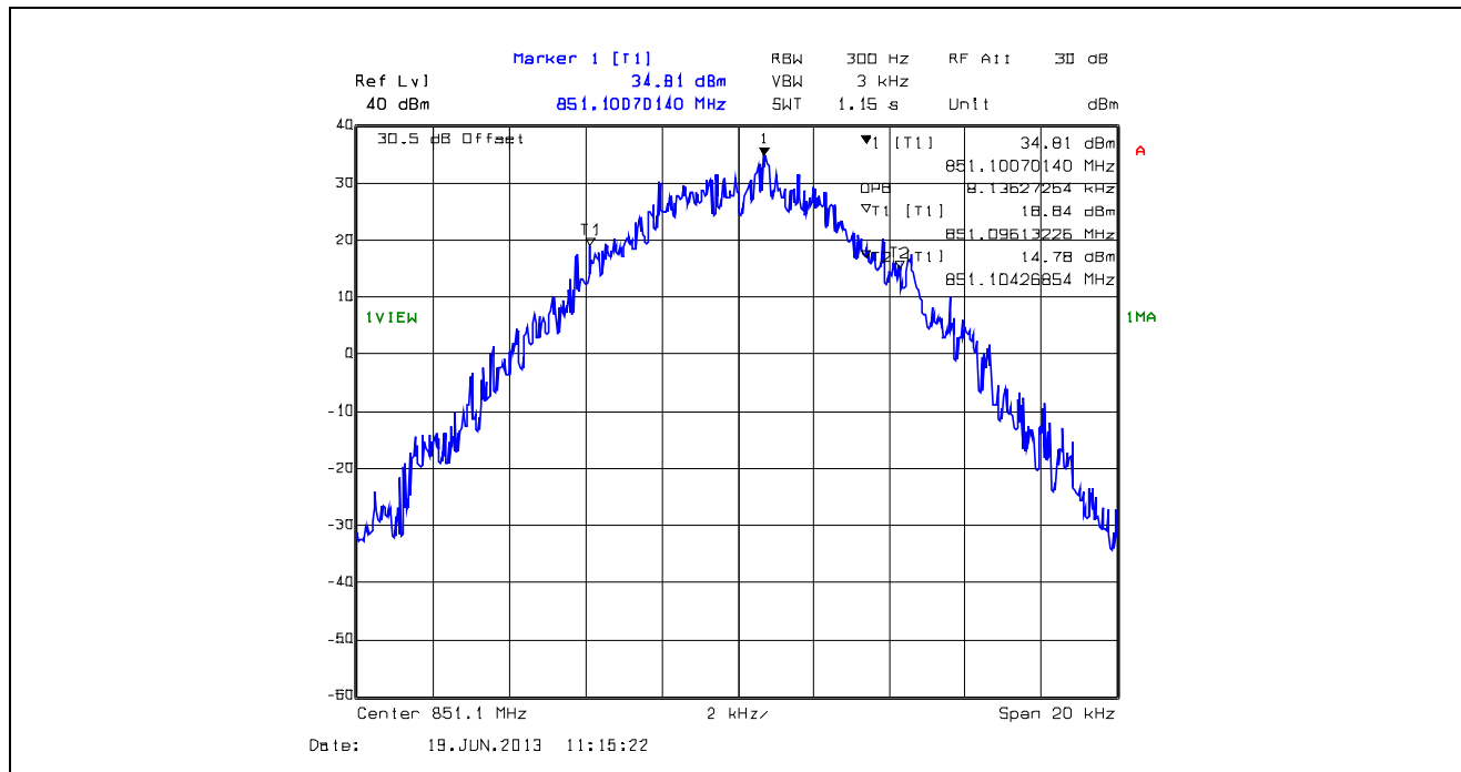
Plot 5.4.4.1.70. 99% Occupied Bandwidth, 12.5 kHz Channel Spacing, F1D, 851.1 MHz
