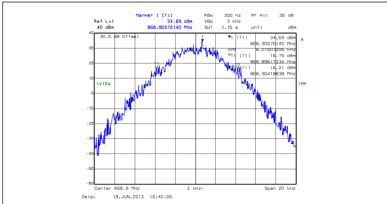
Plot 5.4.4.1.69. 99% Occupied Bandwidth, 12.5 kHz Channel Spacing, F1E, 868.9 MHz
