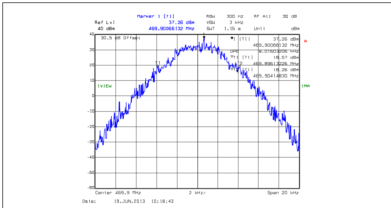
Plot 5.4.4.1.8. 99% Occupied Bandwidth, 12.5 kHz Channel Spacing, F1E, 469.9 MHz
