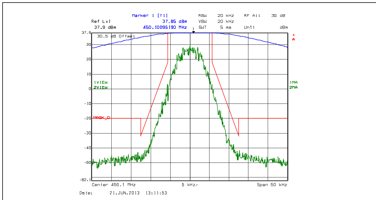
Plot 5.4.4.2.25. Emission Mask D, 12.5 kHz Channel Spacing, F1W, High Power, 450.1 MHz
