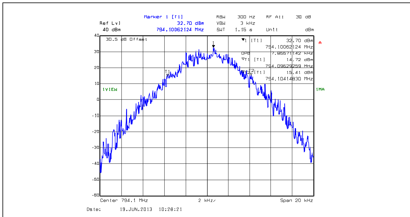
Plot 5.4.4.1.37. 99% Occupied Bandwidth, 12.5 kHz Channel Spacing, F1E, 794.1 MHz
