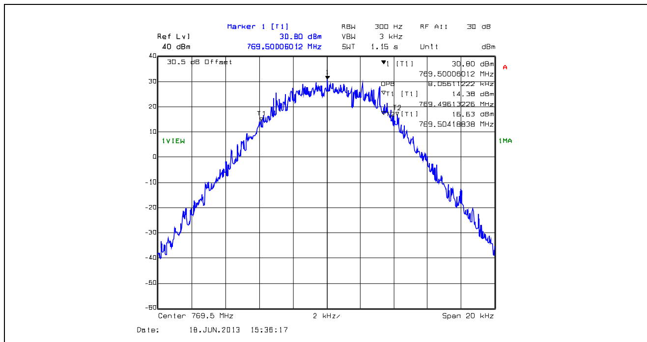
Plot 5.4.4.1.29. 99% Occupied Bandwidth, 12.5 kHz Channel Spacing, F1W, 769.5 MHz
