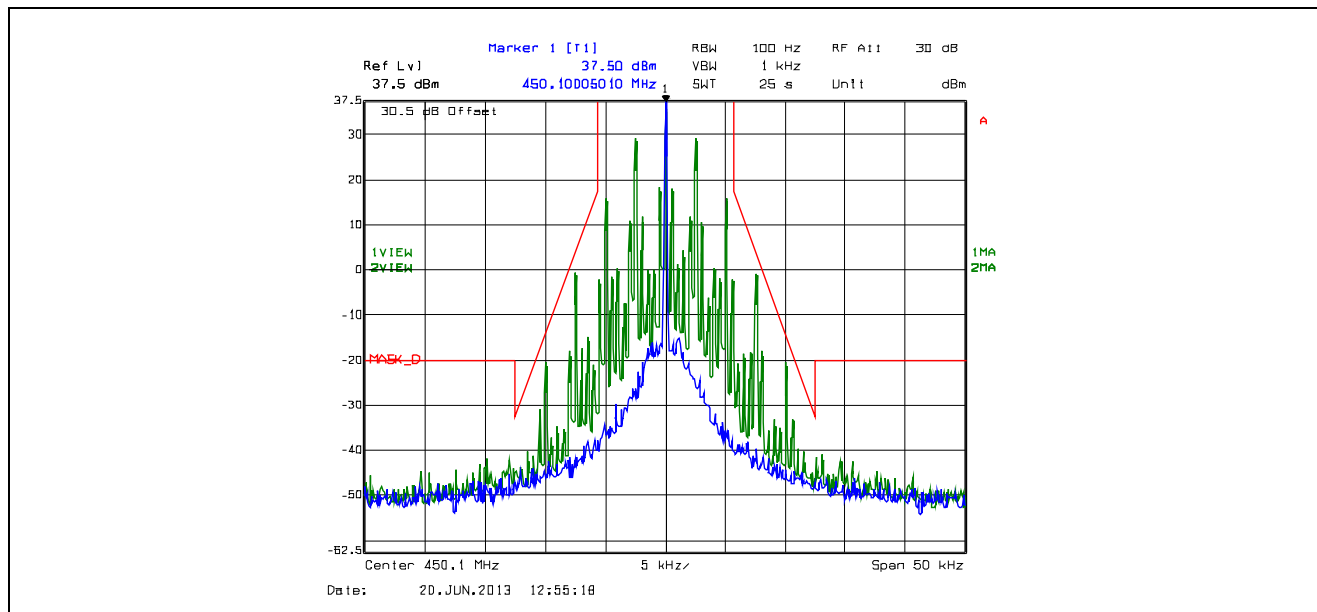
Plot 5.4.4.2.1. Emission Mask D, 12.5 kHz Channel Spacing, F3E, High Power, 450.1 MHz
