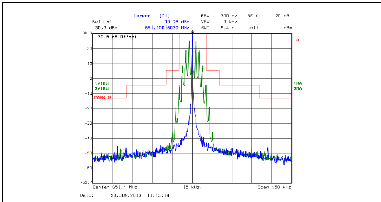
Plot 5.4.4.2.68. Emission Mask B, 25 kHz Channel Spacing, F3E, Low Power, 851.1 MHz
