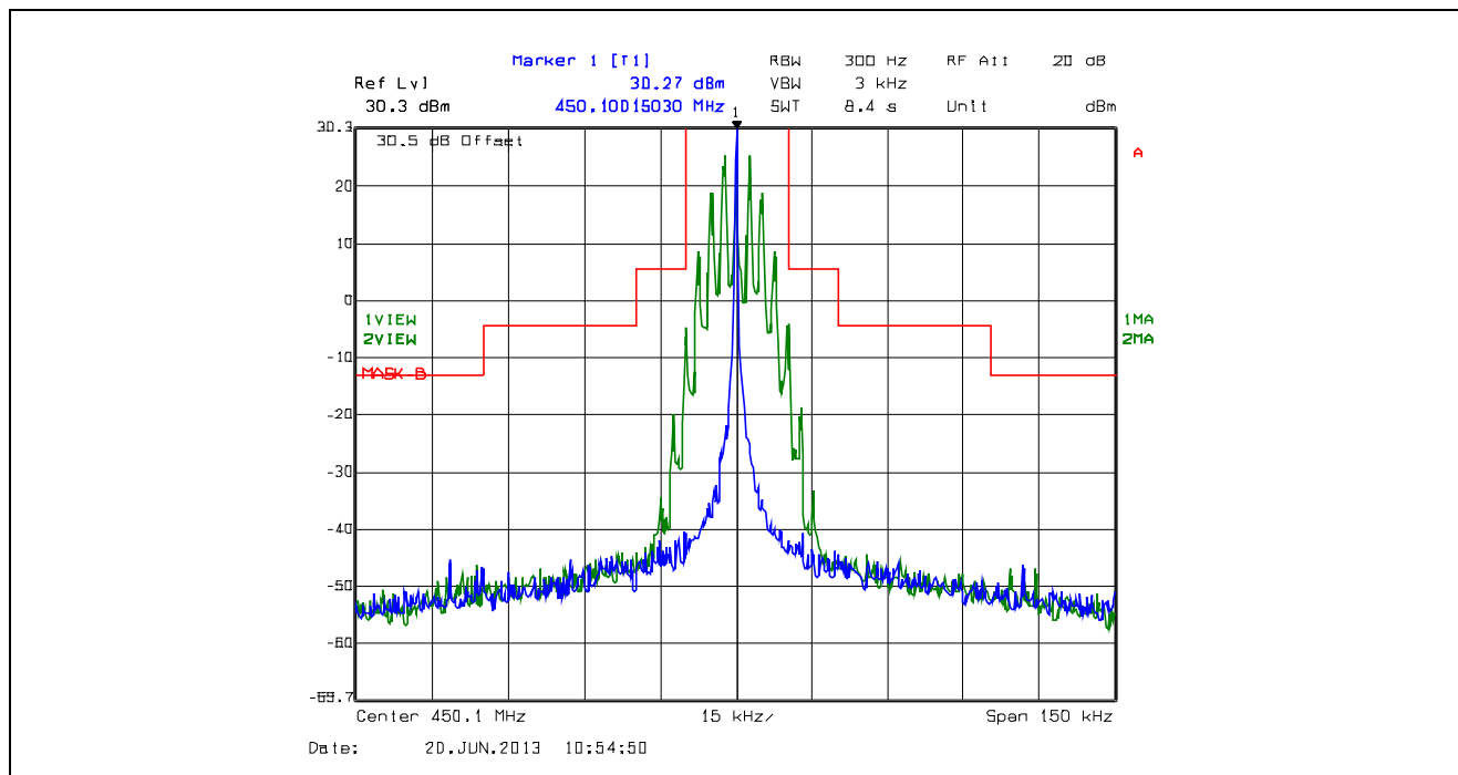
Plot 5.4.4.2.8. Emission Mask B, 25 kHz Channel Spacing, F3E, Low Power, 450.1 MHz
