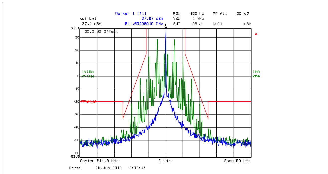
Plot 5.4.4.2.5. Emission Mask D, 12.5 kHz Channel Spacing, F3E, High Power, 511.9 MHz
