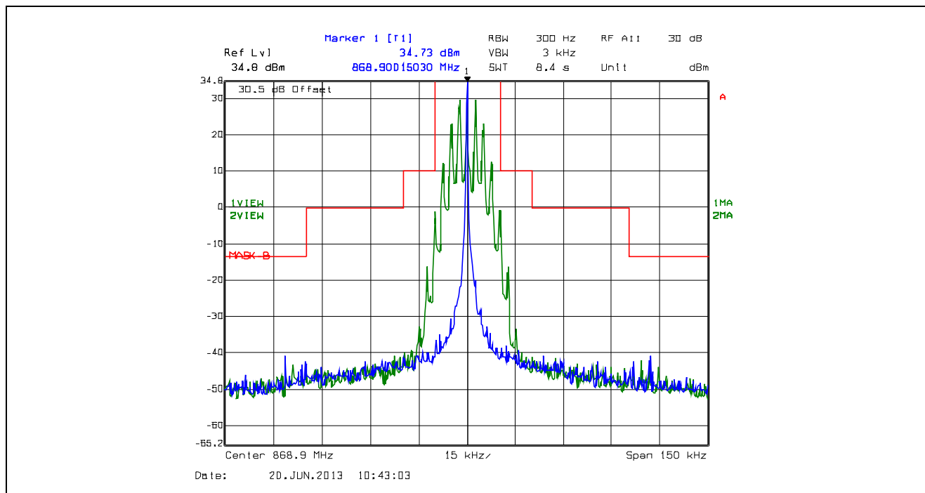
Plot 5.4.4.2.71. Emission Mask B, 25 kHz Channel Spacing, F3E, High Power, 868.9 MHz
