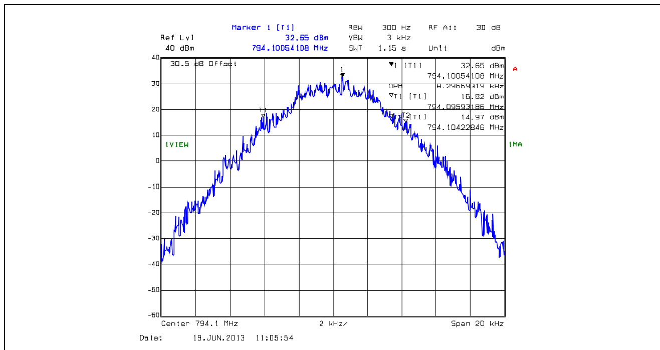
Plot 5.4.4.1.40. 99% Occupied Bandwidth, 12.5 kHz Channel Spacing, F1D, 794.1 MHz
