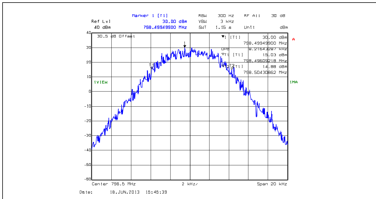
Plot 5.4.4.1.44. 99% Occupied Bandwidth, 12.5 kHz Channel Spacing, F1W, 798.5 MHz
