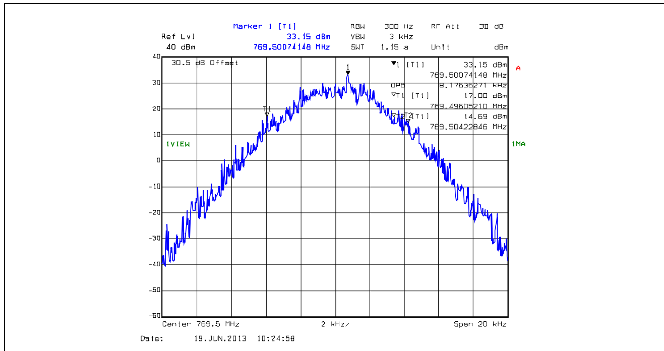
Plot 5.4.4.1.23. 99% Occupied Bandwidth, 12.5 kHz Channel Spacing, F1E, 769.5 MHz
