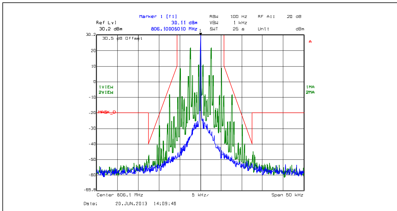
Plot 5.4.4.2.32. Emission Mask D, 12.5 kHz Channel Spacing, F3E, Low Power, 806.1 MHz
