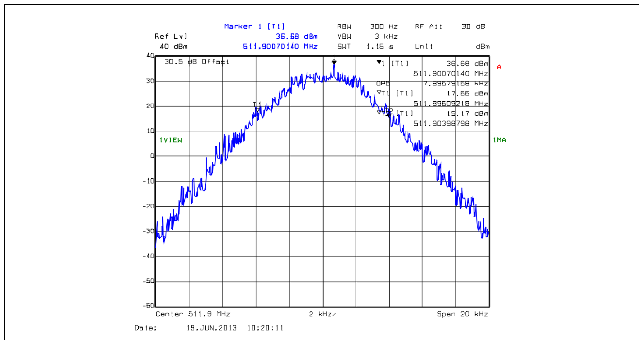
Plot 5.4.4.1.9. 99% Occupied Bandwidth, 12.5 kHz Channel Spacing, F1E, 511.9 MHz
