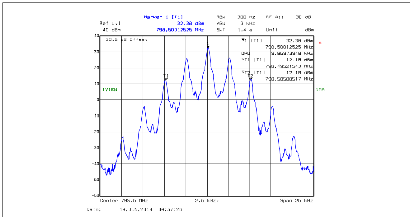
Plot 5.4.4.1.32. 99% Occupied Bandwidth, 12.5 kHz Channel Spacing, F3E, 798.5 MHz
