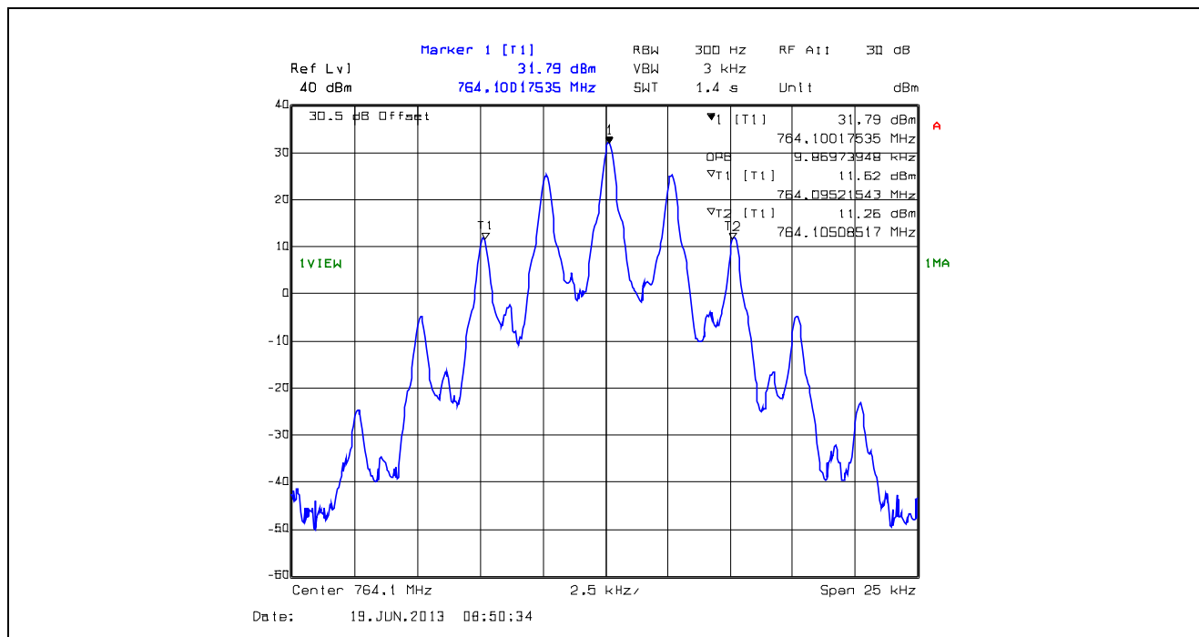
Plot 5.4.4.1.16. 99% Occupied Bandwidth, 12.5 kHz Channel Spacing, F3E, 764.1 MHz
