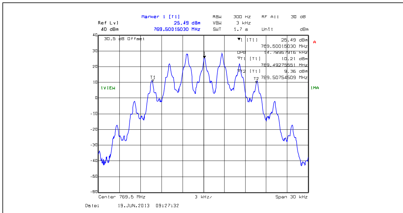
Plot 5.4.4.1.20. 99% Occupied Bandwidth, 25 kHz Channel Spacing, F3E, 769.5MHz
