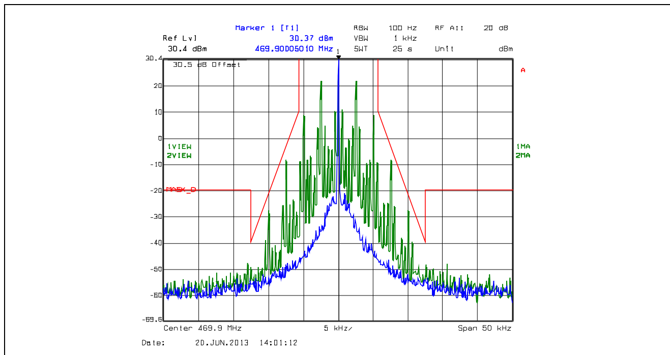
Plot 5.4.4.2.4. Emission Mask D, 12.5 kHz Channel Spacing, F3E, Low Power, 469.9 MHz
