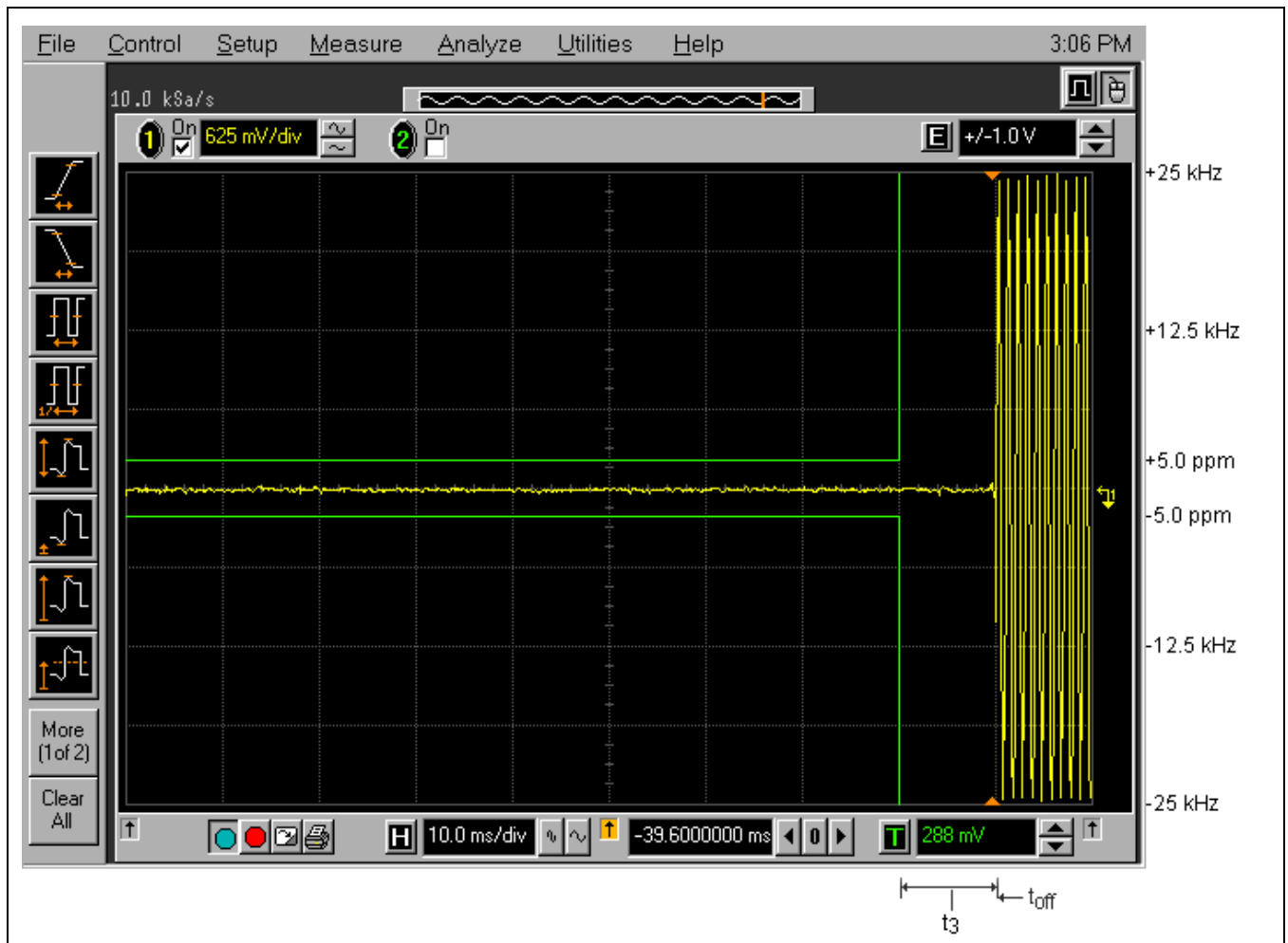
Plot 5.8.4.4. Transient Frequency Behavior on 25 kHz Channels Test Frequency: 450.1 MHz; Power: 5 W; Test Conditions: Switch off condition t_3 , t_{off}
