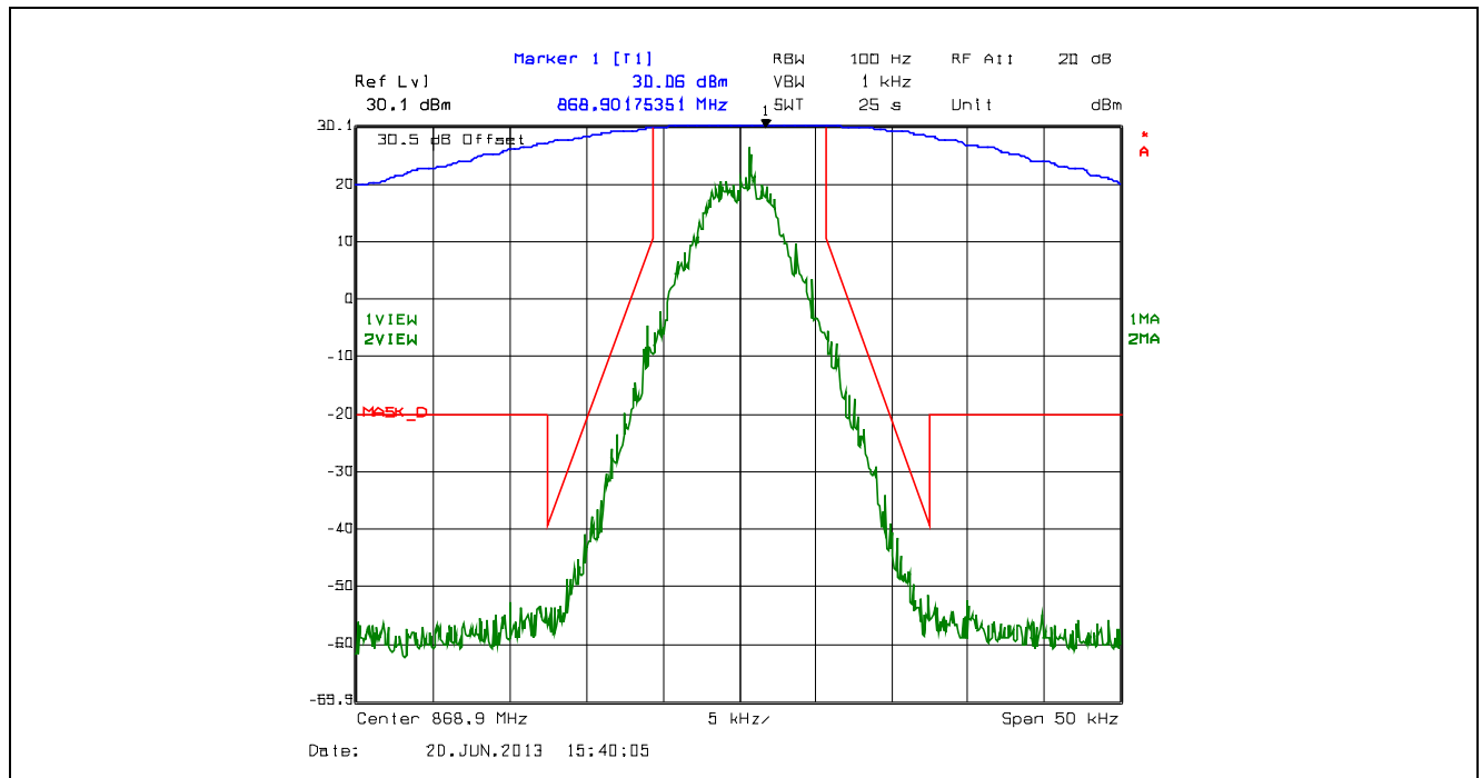
Plot 5.4.4.2.78. Emission Mask D, 12.5 kHz Channel Spacing, F1E, Low Power, 868.9 MHz
