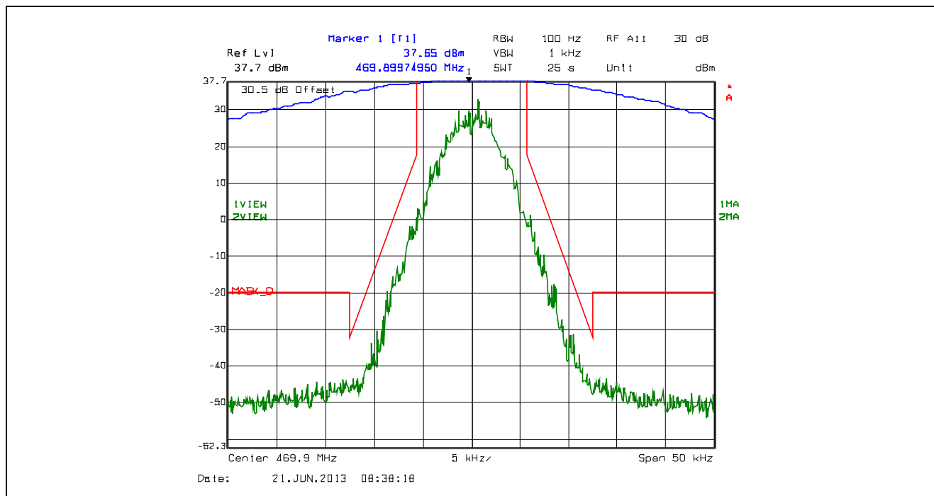
Plot 5.4.4.2.21. Emission Mask D, 12.5 kHz Channel Spacing, F1D, High Power, 469.9 MHz
