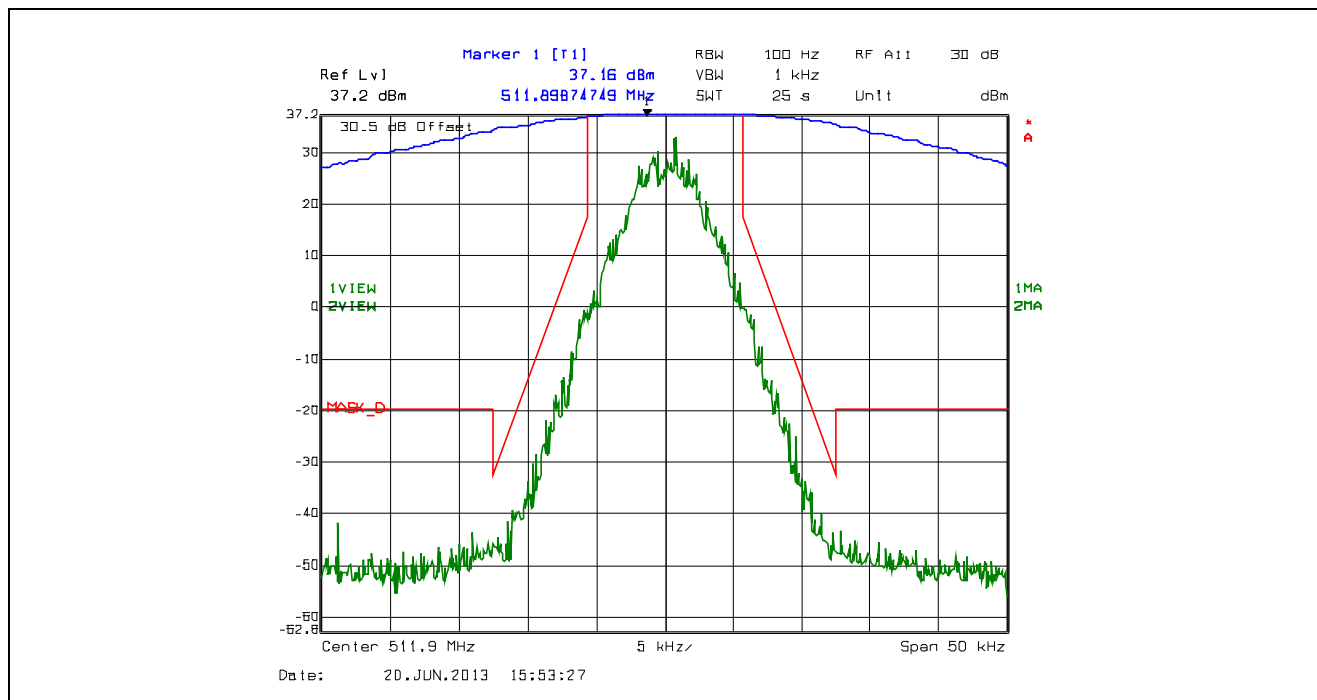
Plot 5.4.4.2.17. Emission Mask D, 12.5 kHz Channel Spacing, F1E, High Power, 511.9 MHz
