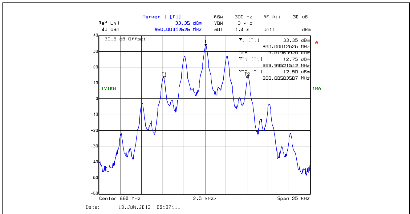
Plot 5.4.4.1.62. 99% Occupied Bandwidth, 12.5 kHz Channel Spacing, F3E, 860.0 MHz
