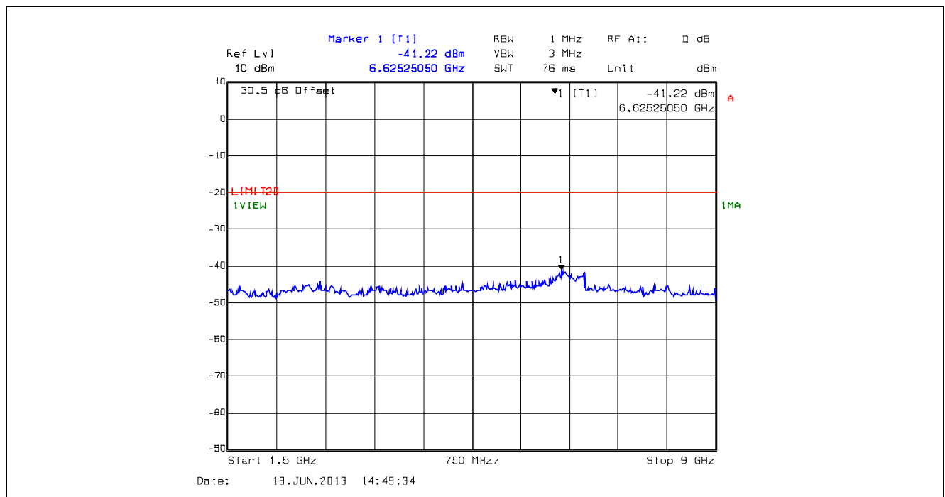
Plot 5.5.4.30. Conducted Transmitter Spurious Emissions, High Power, 798.5 MHz, 1.5 GHz - 9 GHz
