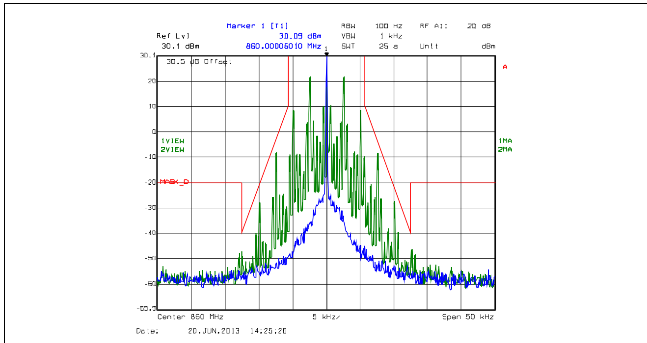
Plot 5.4.4.2.64. Emission Mask D, 12.5 kHz Channel Spacing, F3E, Low Power, 860.0 MHz
