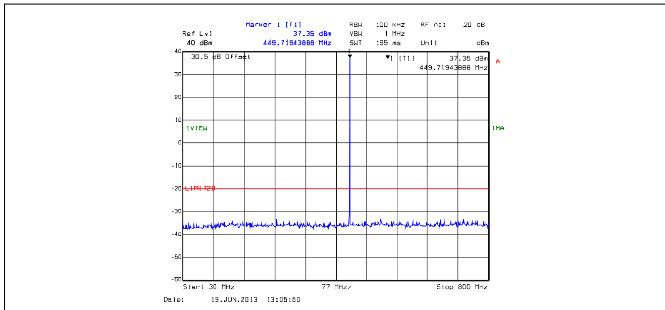
Plot 5.5.4.1. Conducted Transmitter Spurious Emissions, High Power, 450.1 MHz, 30 MHz - 800 MHz
