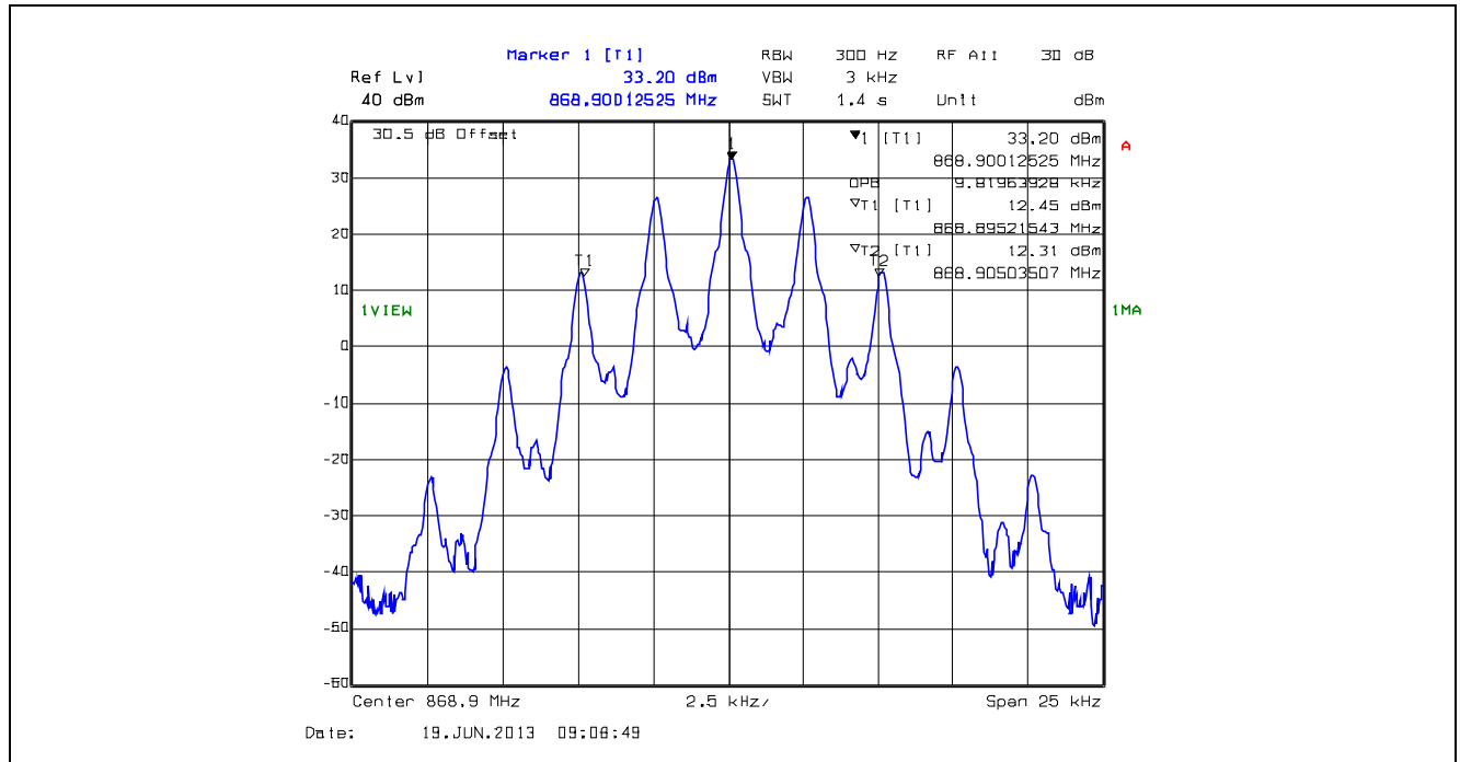
Plot 5.4.4.1.63. 99% Occupied Bandwidth, 12.5 kHz Channel Spacing, F3E, 868.9 MHz
