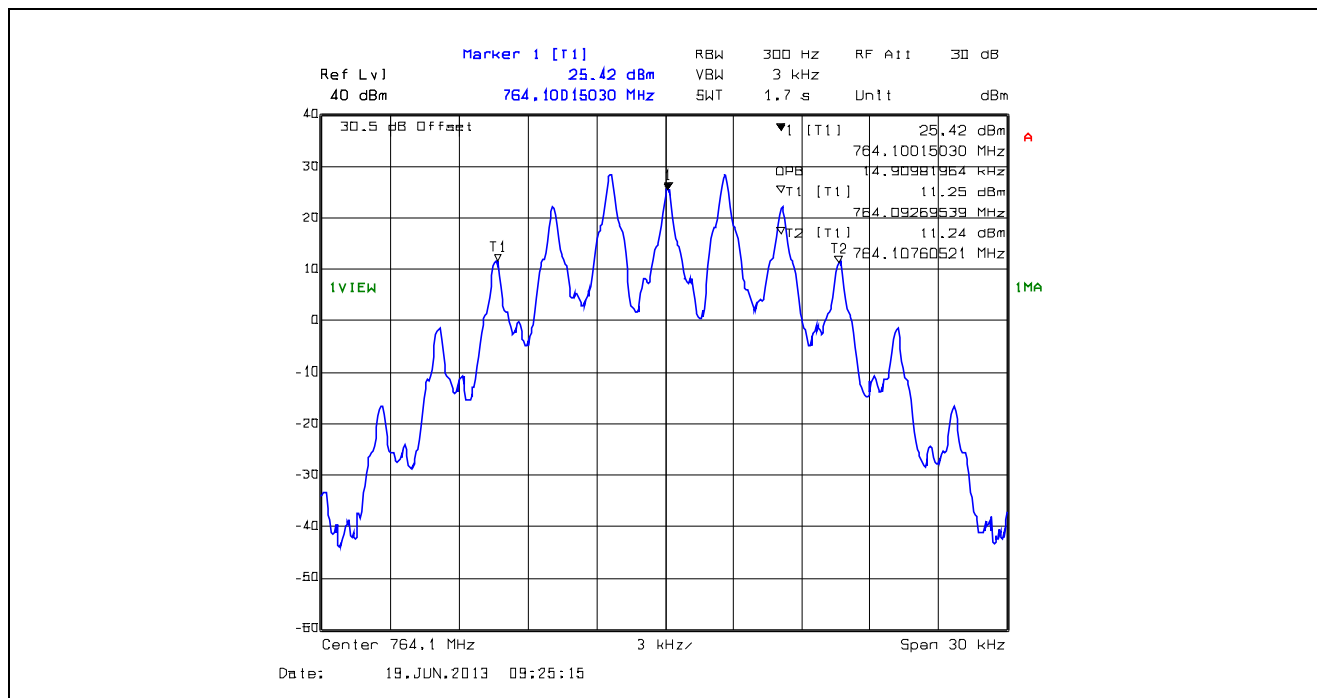
Plot 5.4.4.1.19. 99% Occupied Bandwidth, 25 kHz Channel Spacing, F3E, 764.1 MHz
