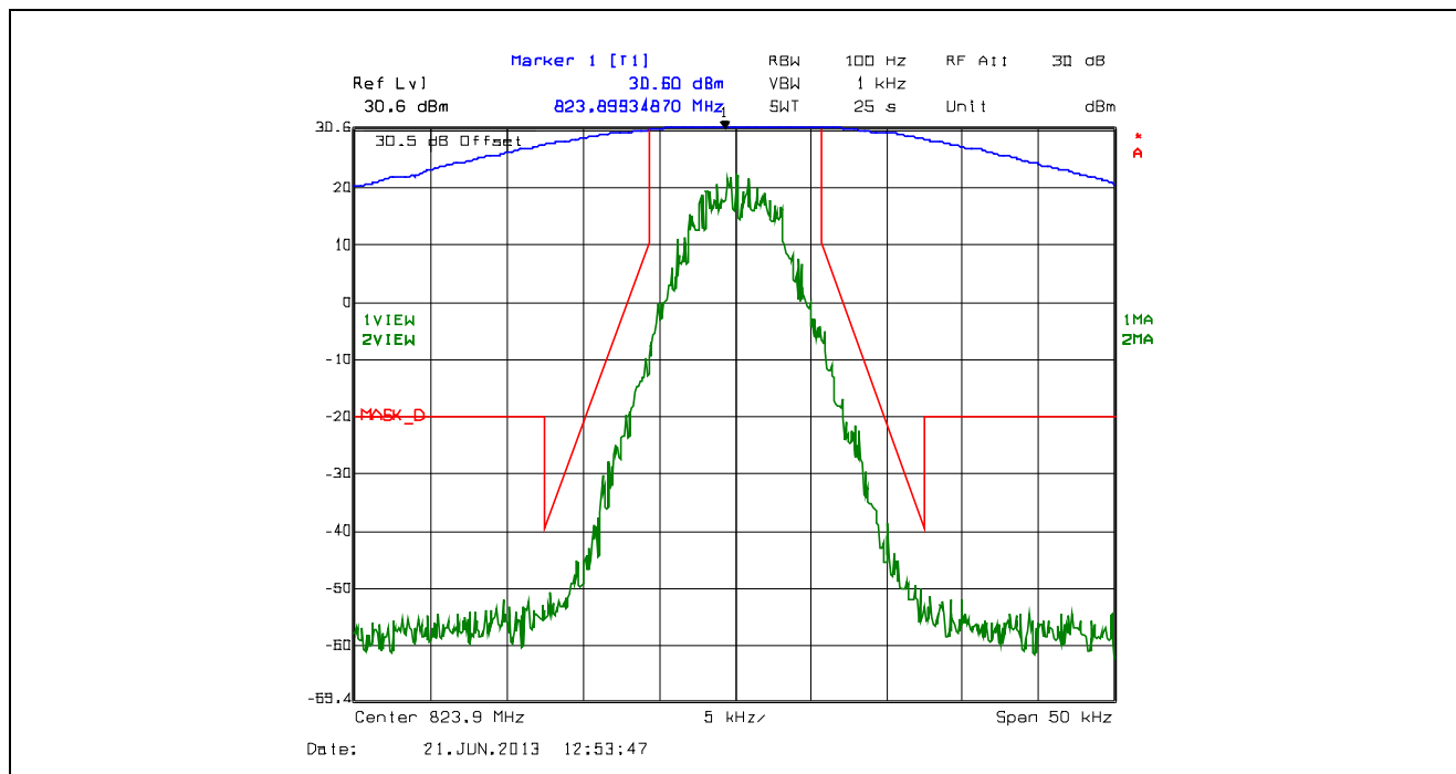
Plot 5.4.4.2.60. Emission Mask D, 12.5 kHz Channel Spacing, F1W, Low Power, 823.9 MHz
