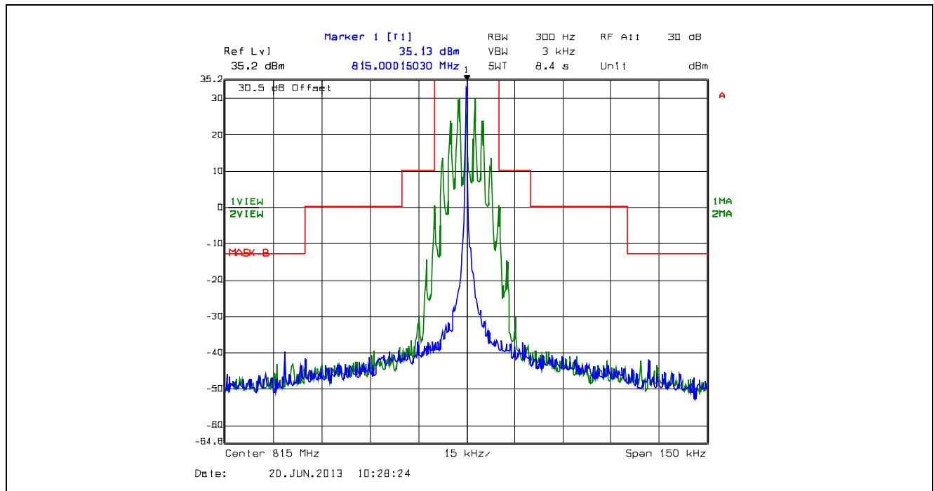
Plot 5.4.4.2.39. Emission Mask B, 25 kHz Channel Spacing, F3E, High Power, 815.0 MHz
