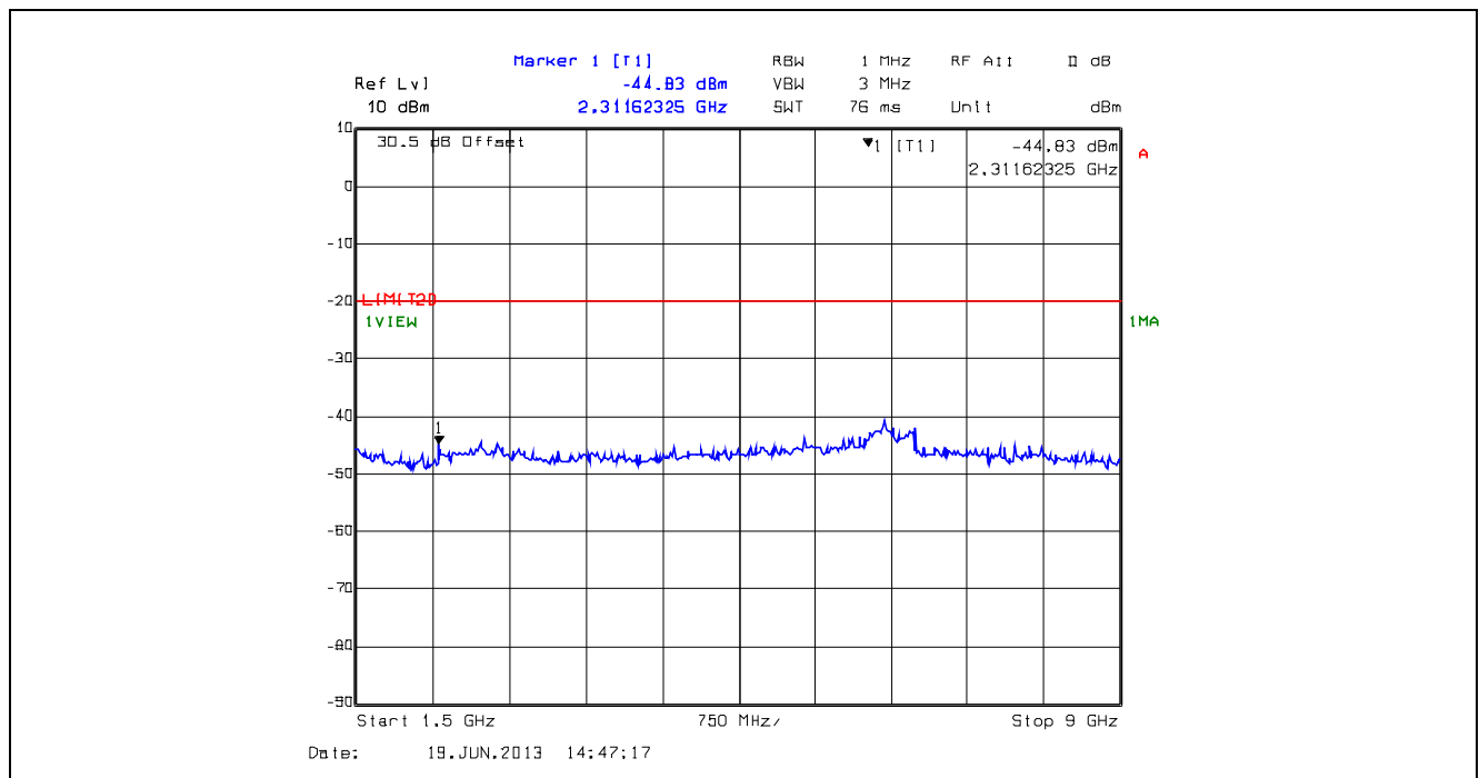
Plot 5.5.4.22. Conducted Transmitter Spurious Emissions, High Power, 774.9 MHz, 1.5 GHz - 9 GHz
