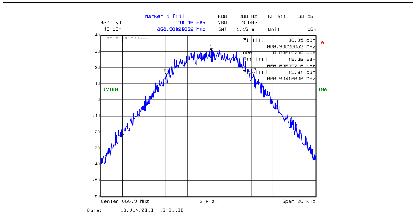
Plot 5.4.4.1.75. 99% Occupied Bandwidth, 12.5 kHz Channel Spacing, F1W, 868.9 MHz
