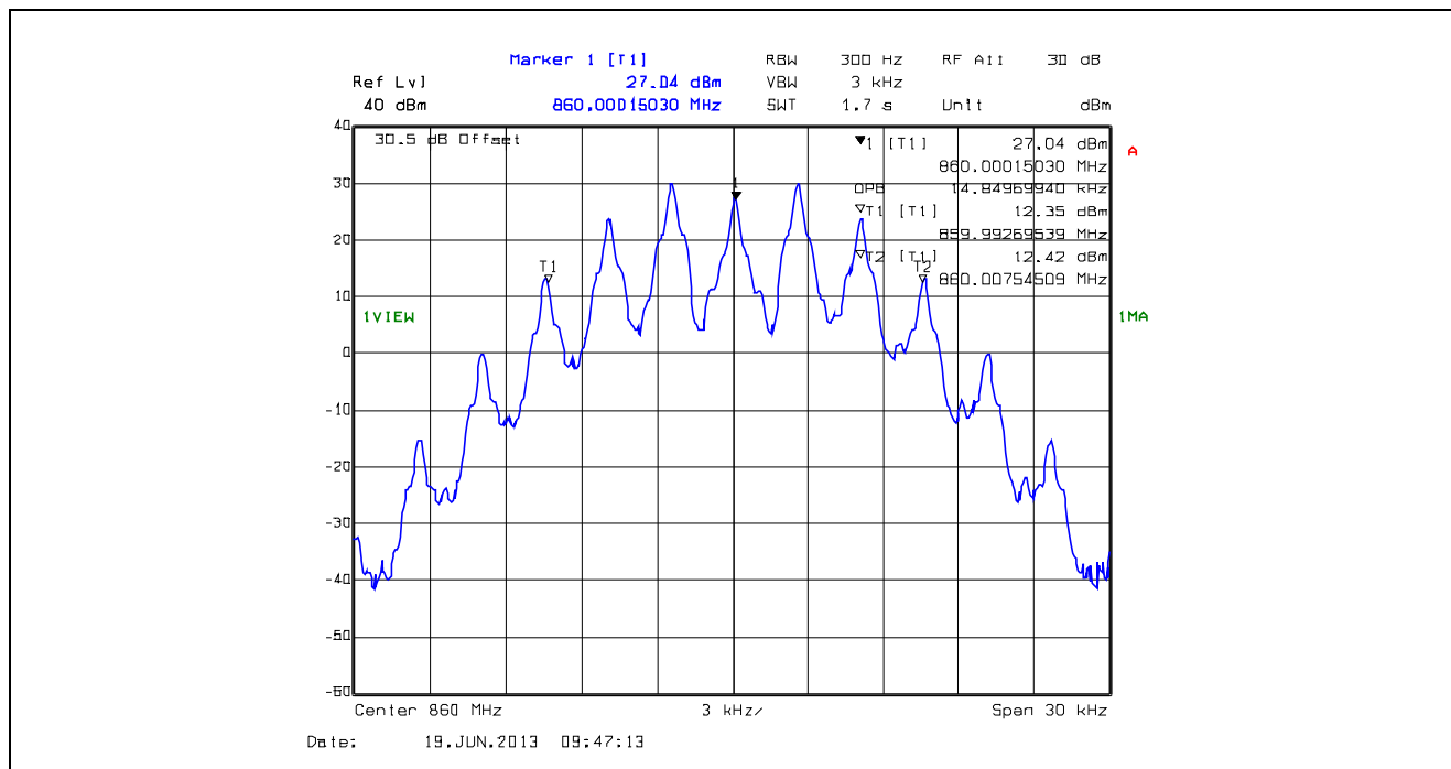
Plot 5.4.4.1.65. 99% Occupied Bandwidth, 25 kHz Channel Spacing, F3E, 860.0 MHz
