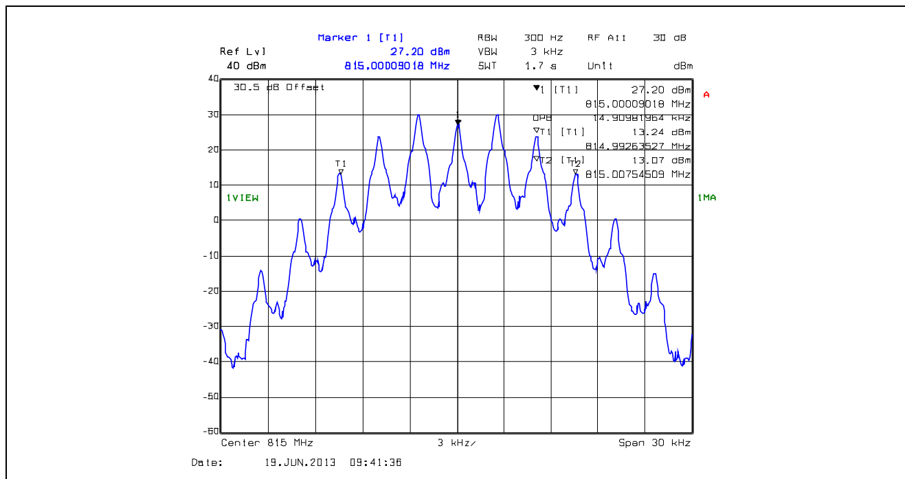
Plot 5.4.4.1.50. 99% Occupied Bandwidth, 25 kHz Channel Spacing, F3E, 815.0MHz
