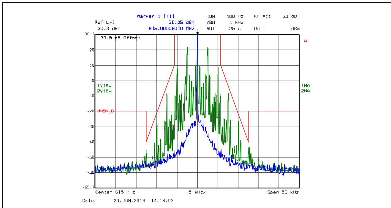
Plot 5.4.4.2.34. Emission Mask D, 12.5 kHz Channel Spacing, F3E, Low Power, 815.0 MHz
