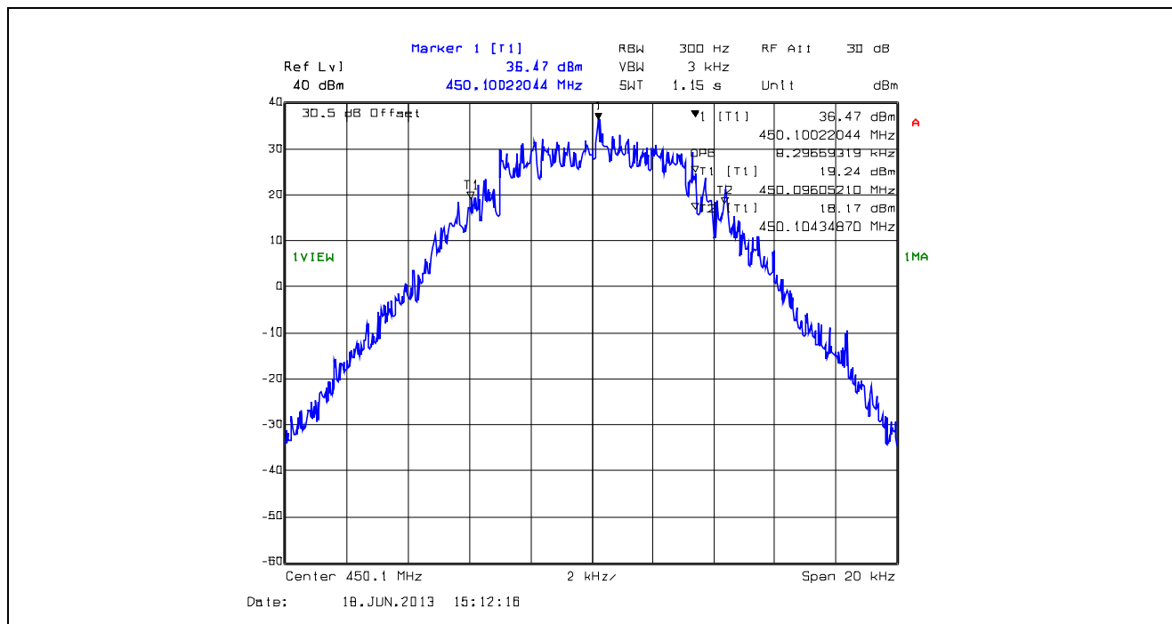
Plot 5.4.4.1.13. 99% Occupied Bandwidth, 12.5 kHz Channel Spacing, F1W, 450.1 MHz
