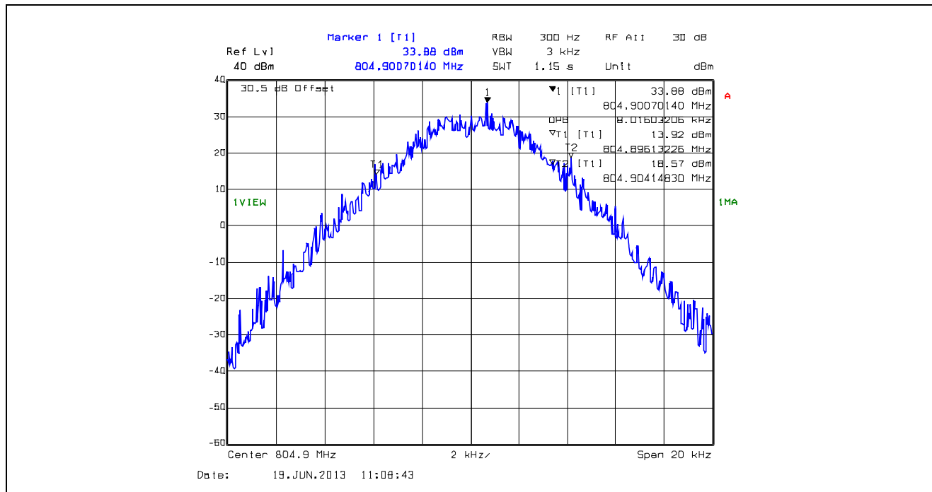
Plot 5.4.4.1.42. 99% Occupied Bandwidth, 12.5 kHz Channel Spacing, F1D, 804.9 MHz
