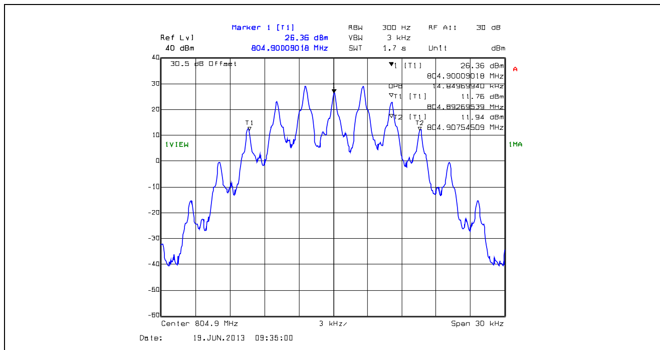
Plot 5.4.4.1.36. 99% Occupied Bandwidth, 25 kHz Channel Spacing, F3E, 804.9 MHz
