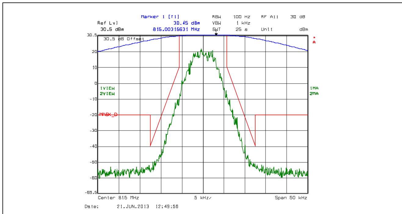
Plot 5.4.4.2.58. Emission Mask D, 12.5 kHz Channel Spacing, F1W, Low Power, 815.0 MHz
