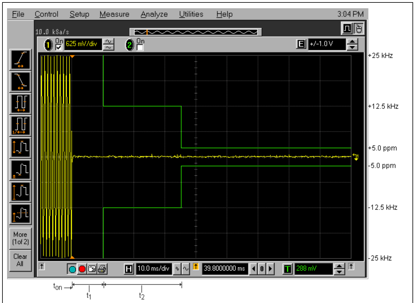
Plot 5.8.4.3. Transient Frequency Behavior on 25 kHz Channels Test Frequency: 450.1 MHz; Power: 5 W; Test Conditions: Switch on condition t_{on} , t_1 , and t_2
