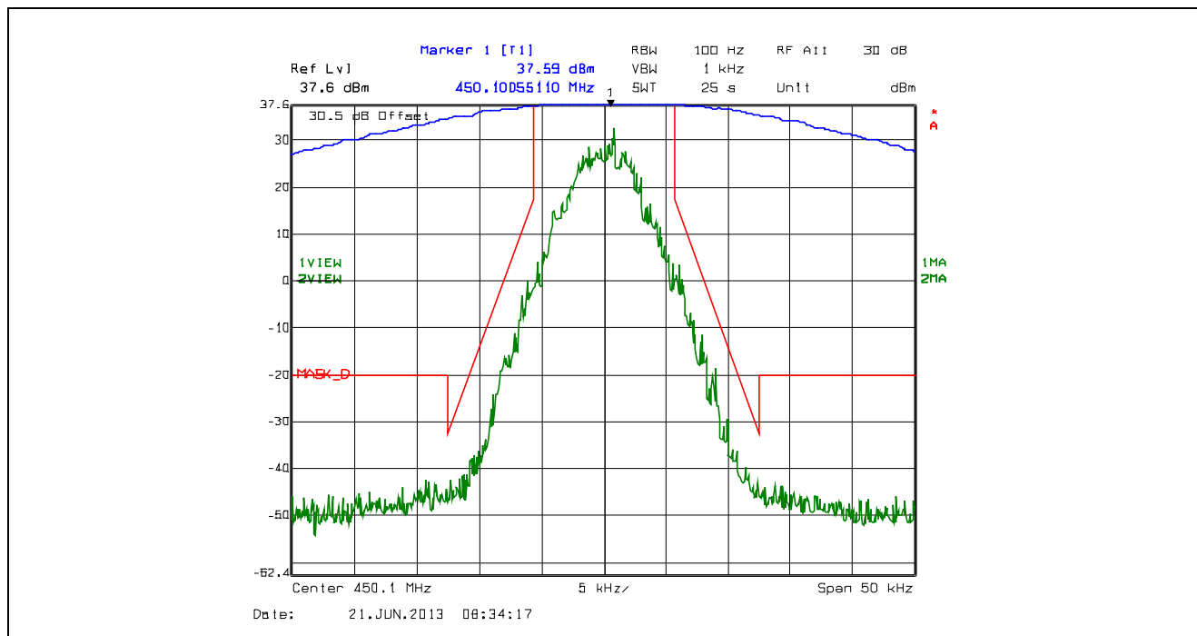
Plot 5.4.4.2.19. Emission Mask D, 12.5 kHz Channel Spacing, F1D, High Power, 450.1 MHz
