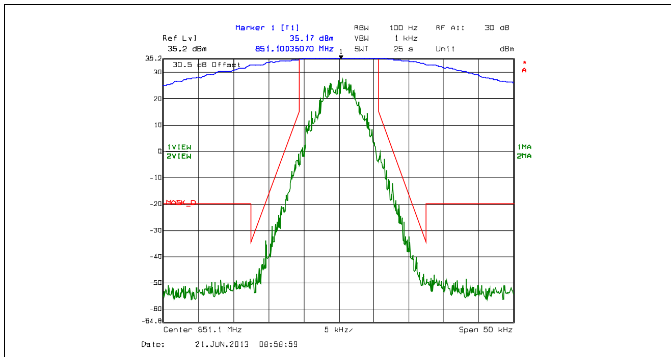
Plot 5.4.4.2.79. Emission Mask D, 12.5 kHz Channel Spacing, F1D, High Power, 851.1 MHz
