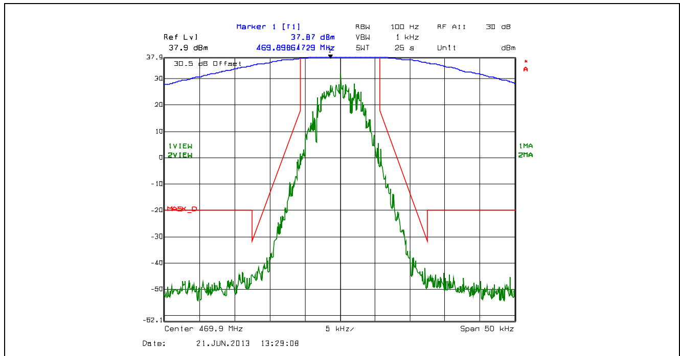
Plot 5.4.4.2.27. Emission Mask D, 12.5 kHz Channel Spacing, F1W, High Power, 469.9 MHz
