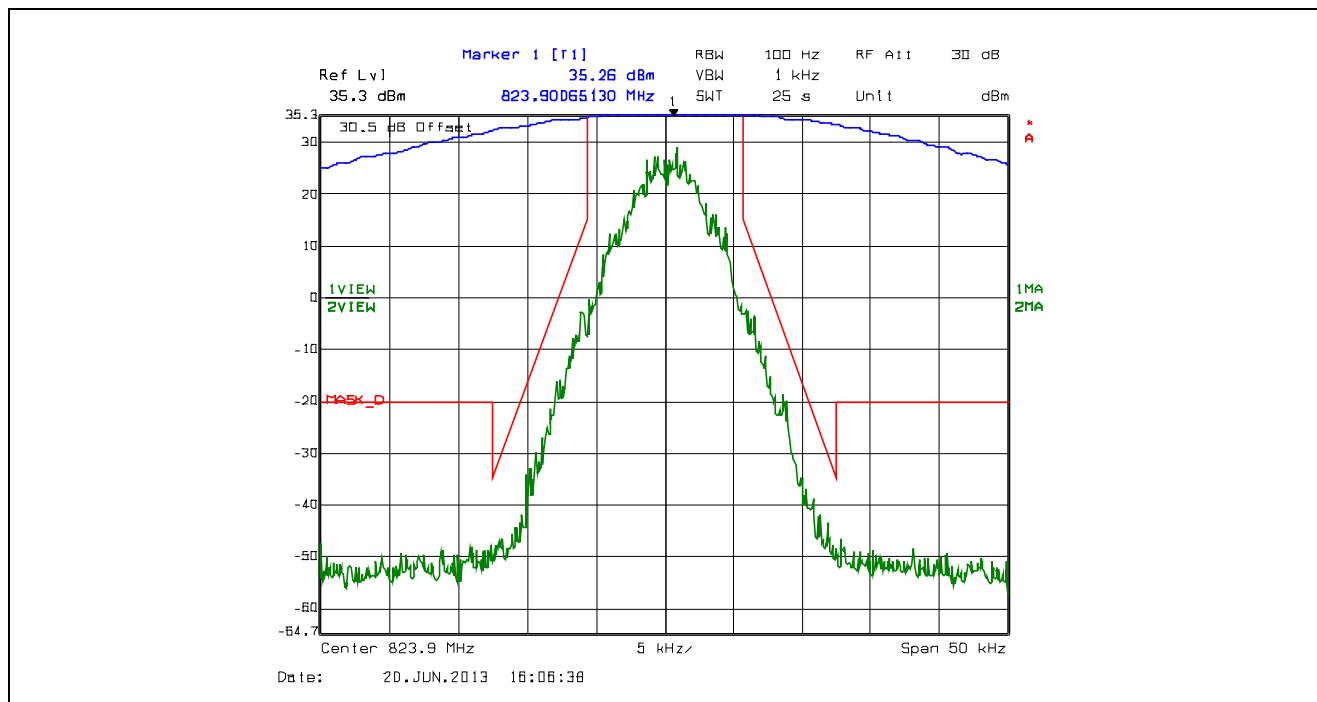
Plot 5.4.4.2.47. Emission Mask D, 12.5 kHz Channel Spacing, F1E, High Power, 823.9 MHz
