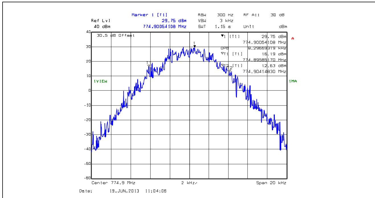
Plot 5.4.4.1.27. 99% Occupied Bandwidth, 12.5 kHz Channel Spacing, F1D, 774.9 MHz
