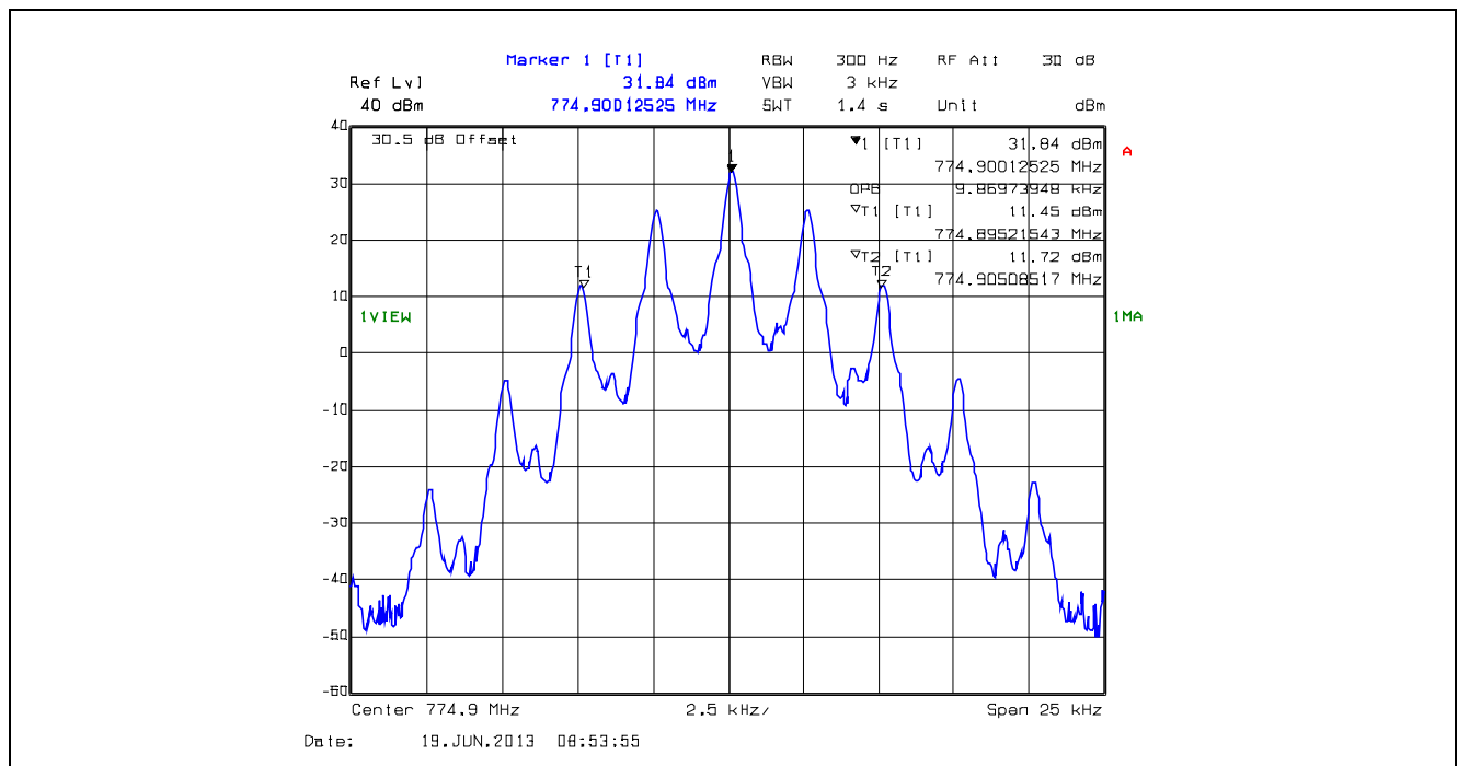
Plot 5.4.4.1.18. 99% Occupied Bandwidth, 12.5 kHz Channel Spacing, F3E, 774.9 MHz
