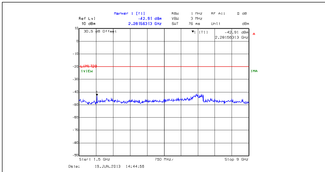
Plot 5.5.4.14. Conducted Transmitter Spurious Emissions, High Power, 764.1 MHz, 1.5 GHz - 9 GHz
