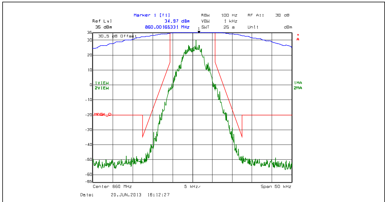
Plot 5.4.4.2.75. Emission Mask D, 12.5 kHz Channel Spacing, F1E, High Power, 860.0 MHz
