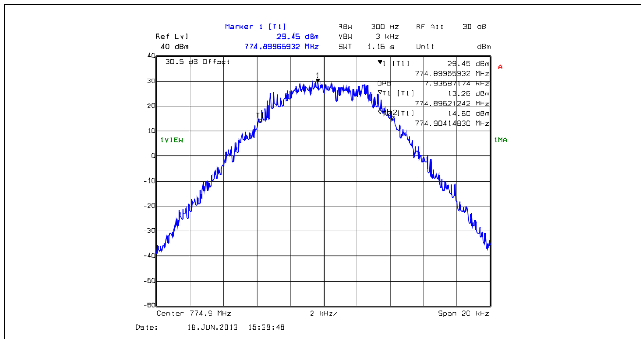
Plot 5.4.4.1.30. 99% Occupied Bandwidth, 12.5 kHz Channel Spacing, F1W, 774.9 MHz
