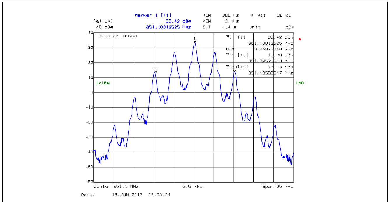
Plot 5.4.4.1.61. 99% Occupied Bandwidth, 12.5 kHz Channel Spacing, F3E, 851.1 MHz
