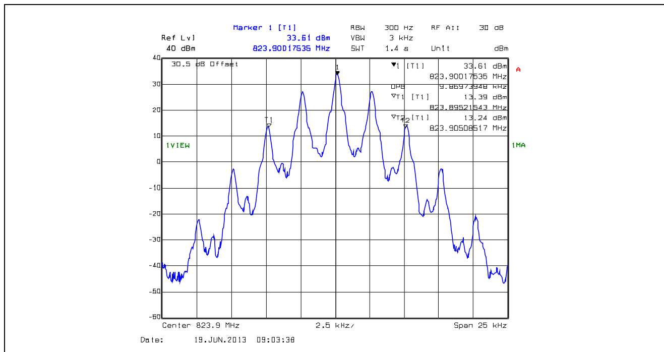
Plot 5.4.4.1.48. 99% Occupied Bandwidth, 12.5 kHz Channel Spacing, F3E, 823.9 MHz
