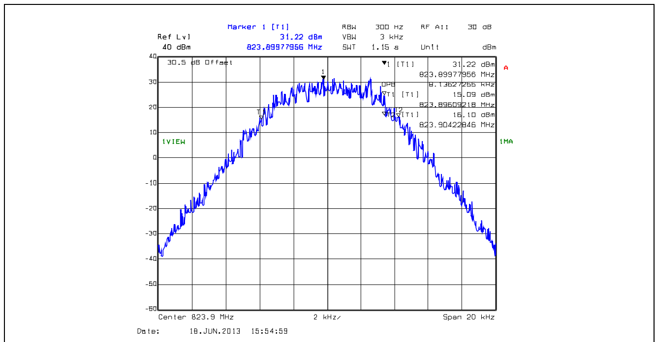
Plot 5.4.4.1.60. 99% Occupied Bandwidth, 12.5 kHz Channel Spacing, F1W, 823.9 MHz
