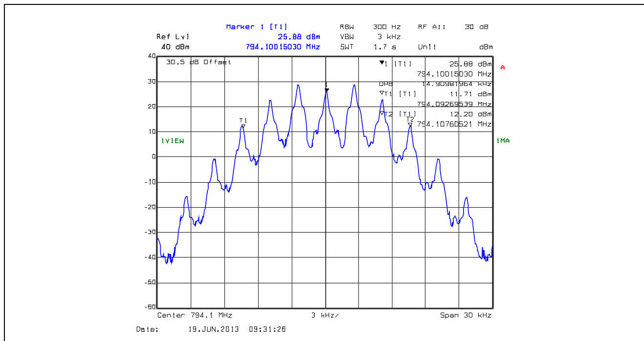
Plot 5.4.4.1.34. 99% Occupied Bandwidth, 25 kHz Channel Spacing, F3E, 794.1MHz
