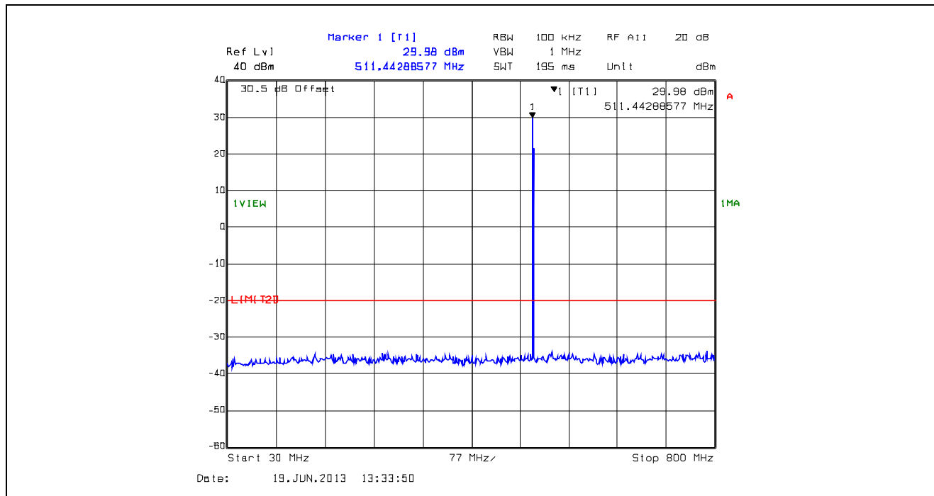
Plot 5.5.4.11. Conducted Transmitter Spurious Emissions, Low Power, 511.9 MHz, 30 MHz - 800 MHz
