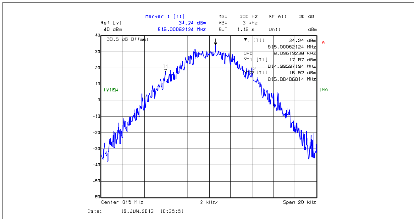
Plot 5.4.4.1.53. 99% Occupied Bandwidth, 12.5 kHz Channel Spacing, F1E, 815.0 MHz
