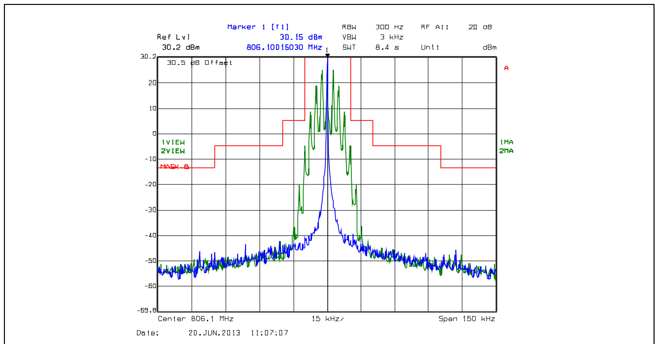
Plot 5.4.4.2.38. Emission Mask B, 25 kHz Channel Spacing, F3E, Low Power, 806.1 MHz
