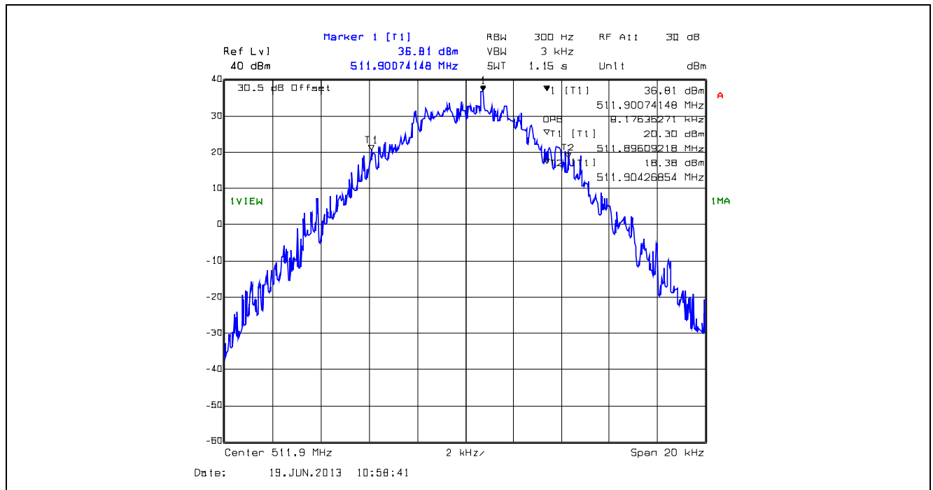
Plot 5.4.4.1.12. 99% Occupied Bandwidth, 12.5 kHz Channel Spacing, F1D, 511.9 MHz
