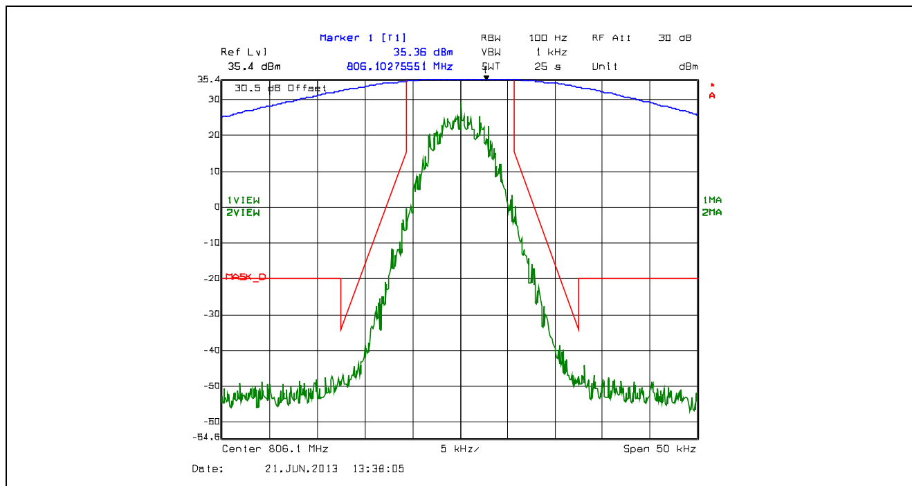
Plot 5.4.4.2.55. Emission Mask D, 12.5 kHz Channel Spacing, F1W, High Power, 806.1 MHz
