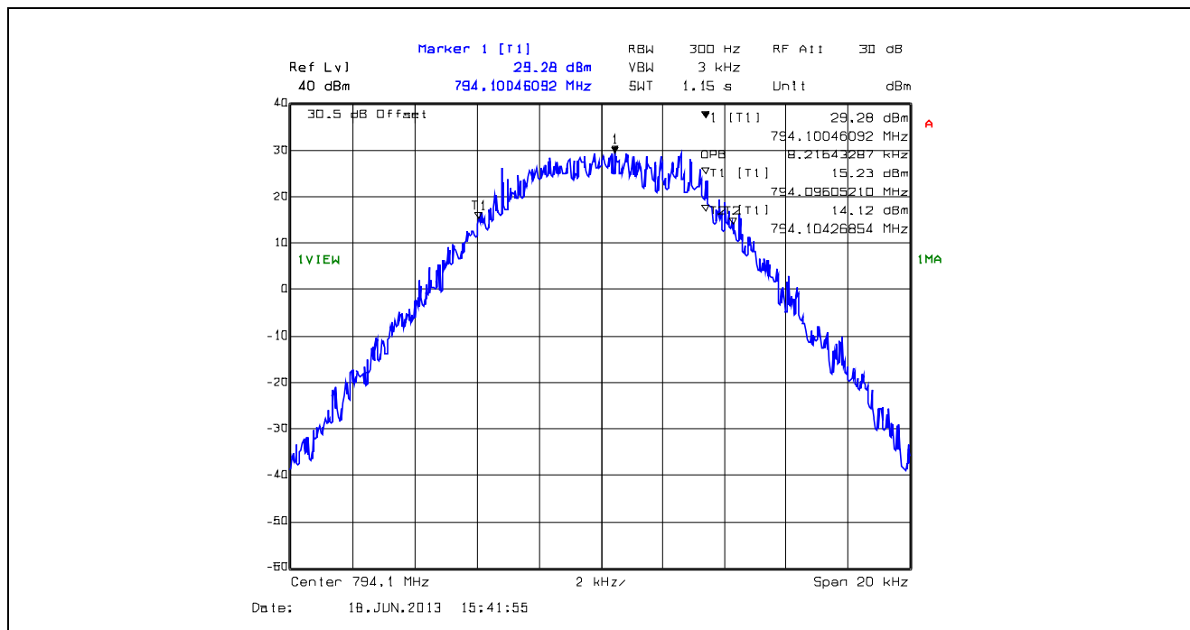
Plot 5.4.4.1.43. 99% Occupied Bandwidth, 12.5 kHz Channel Spacing, F1W, 794.1 MHz
