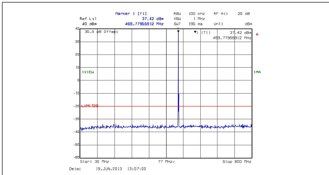
Plot 5.5.4.5. Conducted Transmitter Spurious Emissions, High Power, 469.9 MHz, 30 MHz - 800 MHz
