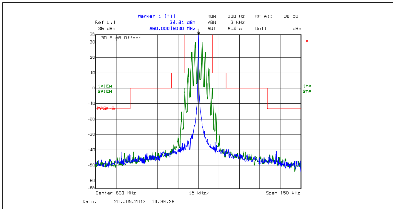
Plot 5.4.4.2.69. Emission Mask B, 25 kHz Channel Spacing, F3E, High Power, 860.0 MHz
