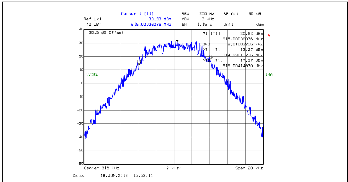
Plot 5.4.4.1.59. 99% Occupied Bandwidth, 12.5 kHz Channel Spacing, F1W, 815.0 MHz
