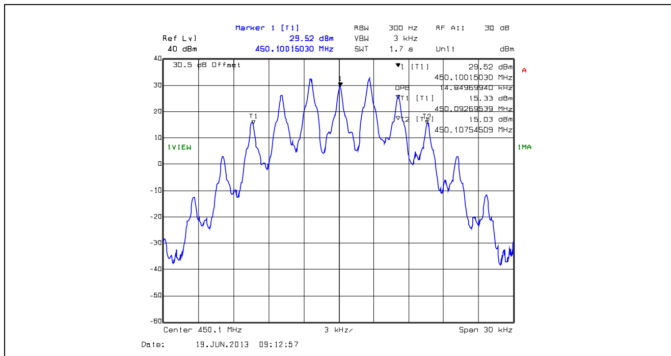
Plot 5.4.4.1.4. 99% Occupied Bandwidth, 25 kHz Channel Spacing, F3E, 450.1 MHz
