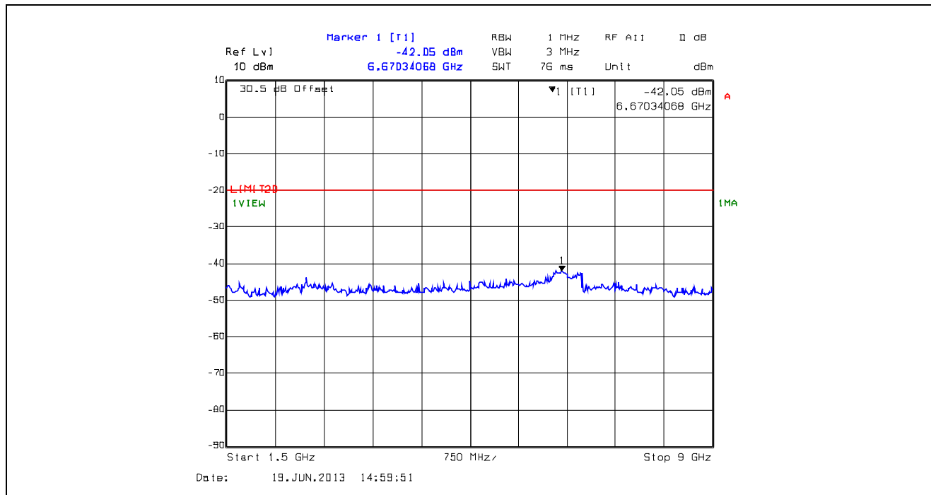
Plot 5.5.4.24. Conducted Transmitter Spurious Emissions, Low Power, 774.9 MHz, 1.5 GHz - 9 GHz
