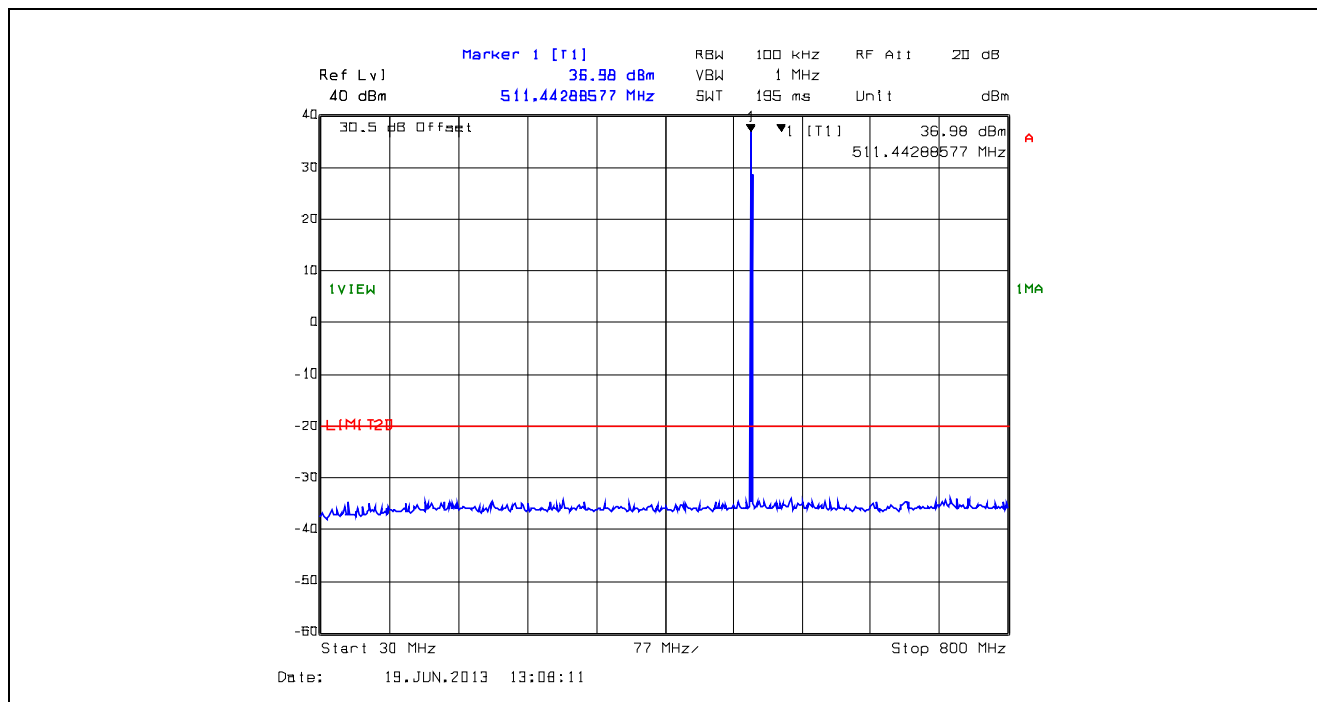
Plot 5.5.4.9. Conducted Transmitter Spurious Emissions, High Power, 511.9 MHz, 30 MHz - 800 MHz
