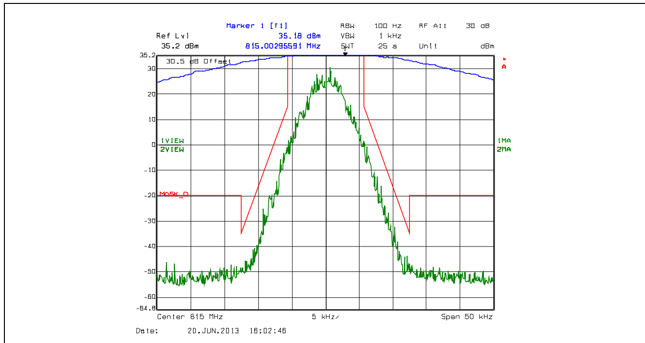
Plot 5.4.4.2.45. Emission Mask D, 12.5 kHz Channel Spacing, F1E, High Power, 815.0 MHz
