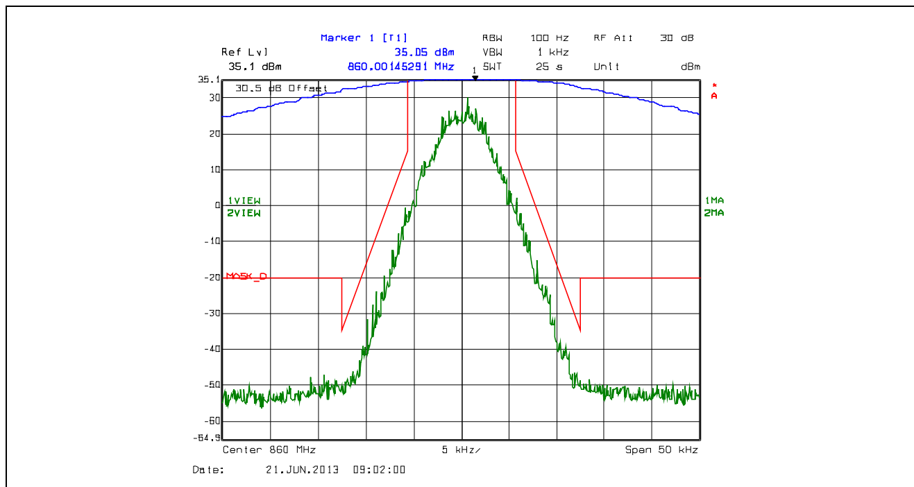
Plot 5.4.4.2.81. Emission Mask D, 12.5 kHz Channel Spacing, F1D, High Power, 860.0 MHz
