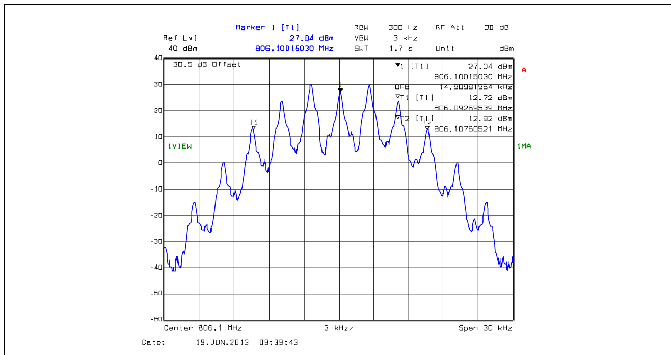
Plot 5.4.4.1.49. 99% Occupied Bandwidth, 25 kHz Channel Spacing, F3E, 806.1 MHz
