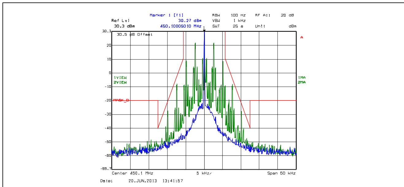
Plot 5.4.4.2.2. Emission Mask D, 12.5 kHz Channel Spacing, F3E, Low Power, 450.1 MHz
