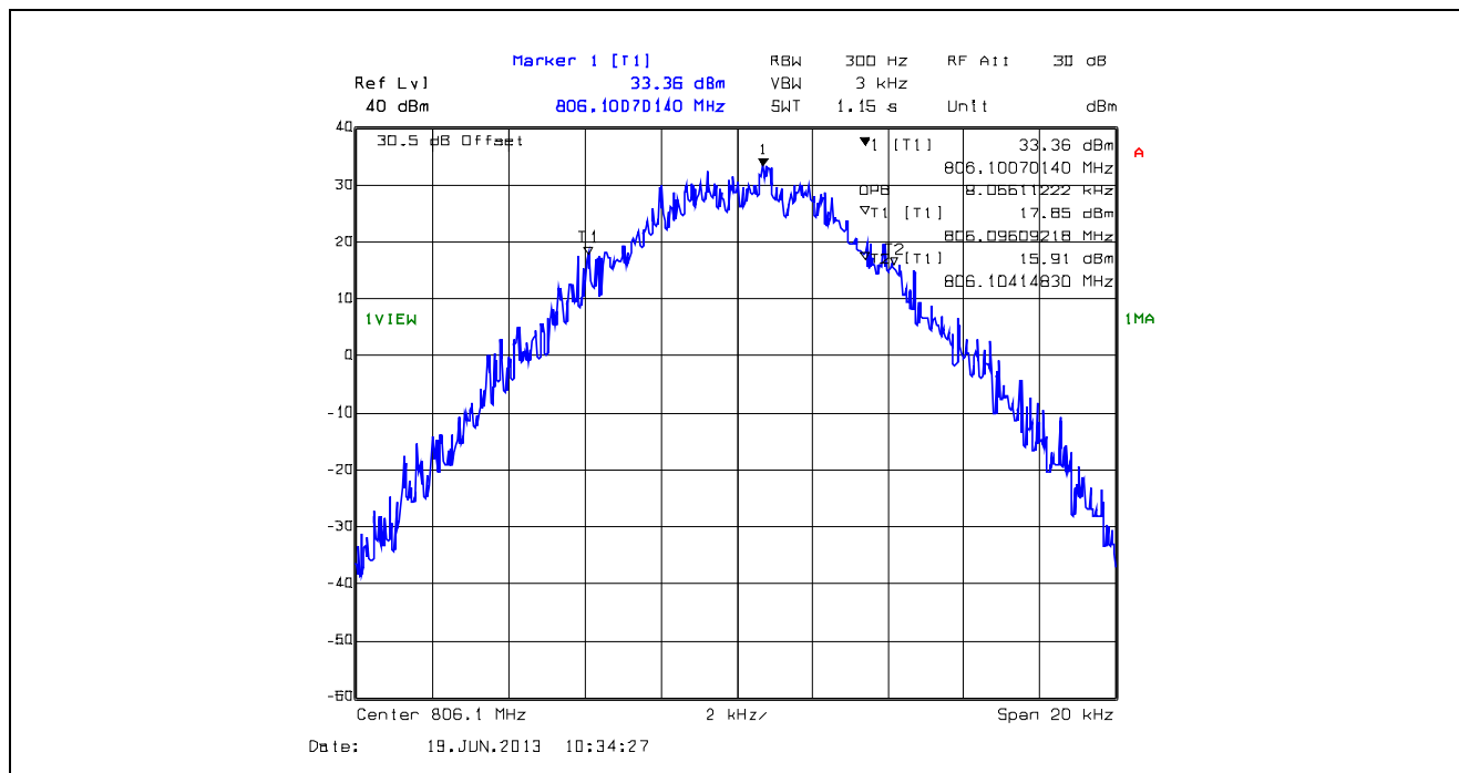
Plot 5.4.4.1.52. 99% Occupied Bandwidth, 12.5 kHz Channel Spacing, F1E, 806.1 MHz
