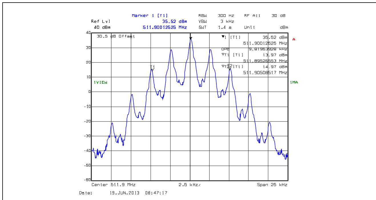
Plot 5.4.4.1.3. 99% Occupied Bandwidth, 12.5 kHz Channel Spacing, F3E, 511.9 MHz
