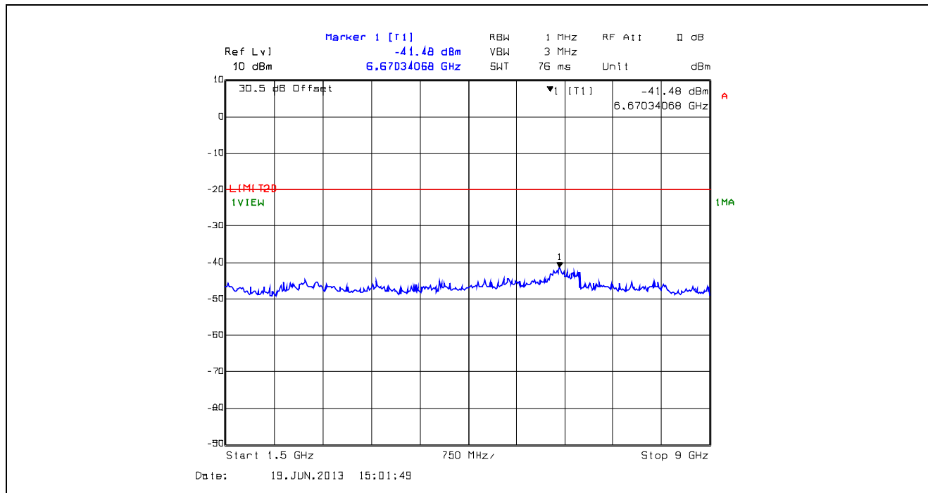
Plot 5.5.4.32. Conducted Transmitter Spurious Emissions, Low Power, 798.5 MHz, 1.5 GHz - 9 GHz
