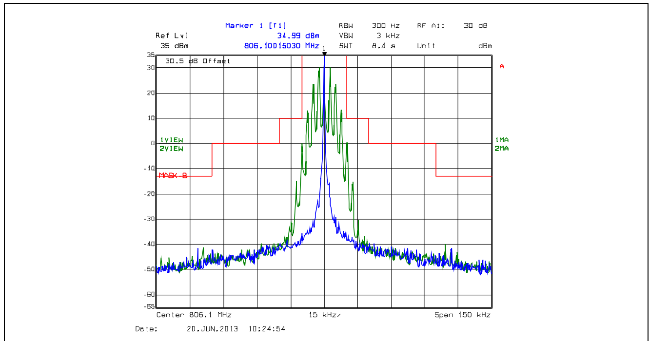
Plot 5.4.4.2.37. Emission Mask B, 25 kHz Channel Spacing, F3E, High Power, 806.1 MHz
