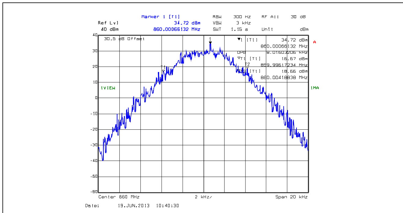
Plot 5.4.4.1.68. 99% Occupied Bandwidth, 12.5 kHz Channel Spacing, F1E, 860.0 MHz
