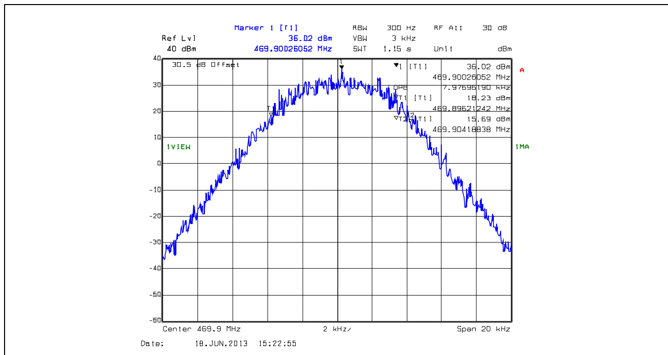
Plot 5.4.4.1.14. 99% Occupied Bandwidth, 12.5 kHz Channel Spacing, F1W, 469.9 MHz
