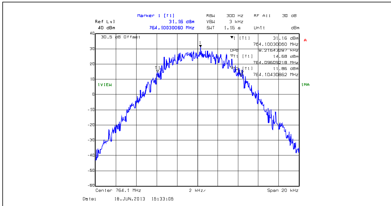
Plot 5.4.4.1.28. 99% Occupied Bandwidth, 12.5 kHz Channel Spacing, F1W, 764.1 MHz
