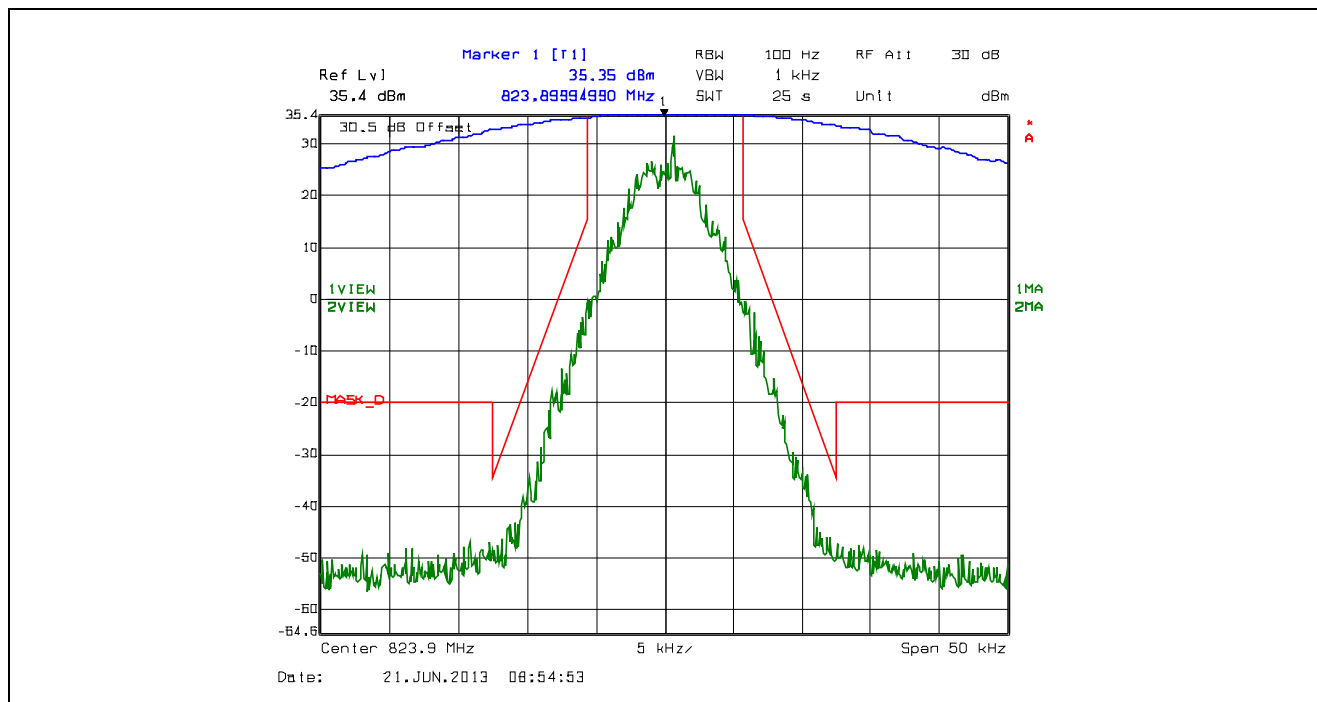
Plot 5.4.4.2.53. Emission Mask D, 12.5 kHz Channel Spacing, F1D, High Power, 823.9 MHz
