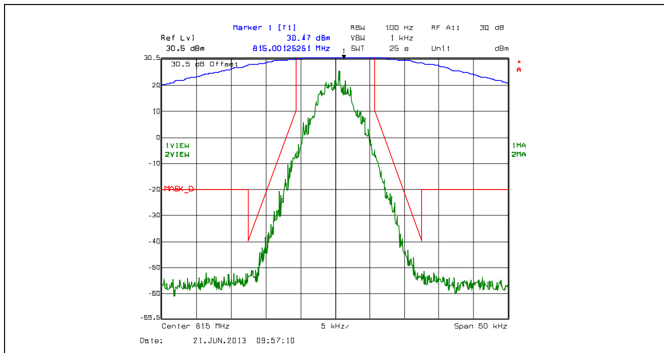
Plot 5.4.4.2.52. Emission Mask D, 12.5 kHz Channel Spacing, F1D, Low Power, 815.0 MHz
