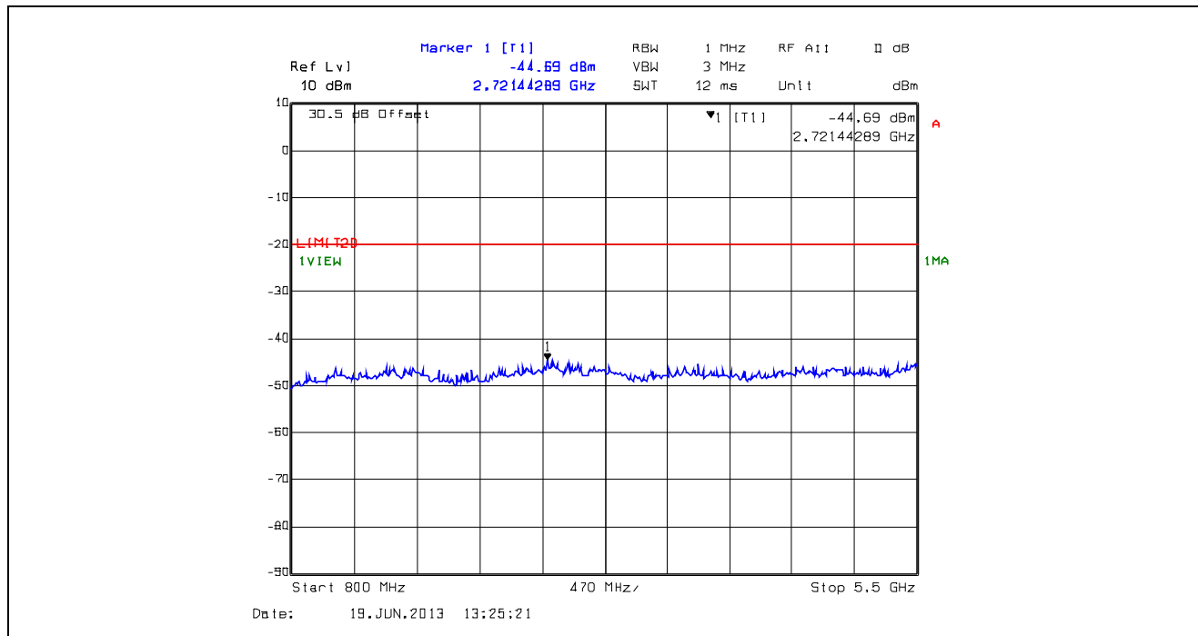
Plot 5.5.4.12. Conducted Transmitter Spurious Emissions, Low Power, 511.9 MHz, 800 MHz - 5.5 GHz
