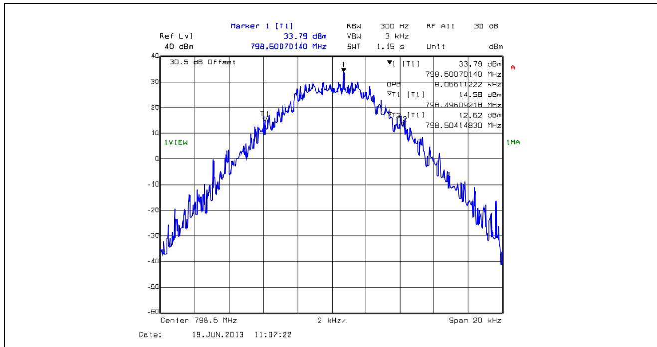
Plot 5.4.4.1.41. 99% Occupied Bandwidth, 12.5 kHz Channel Spacing, F1D, 798.5 MHz
