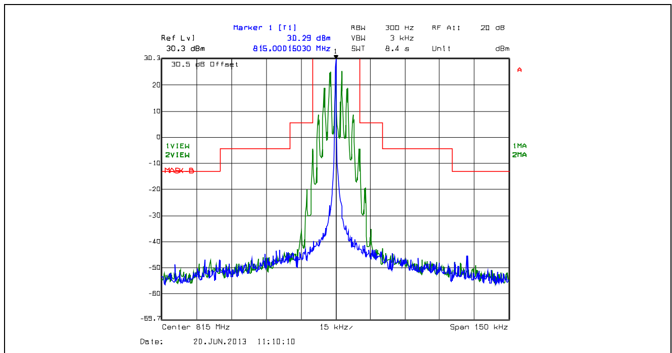
Plot 5.4.4.2.40. Emission Mask B, 25 kHz Channel Spacing, F3E, Low Power, 815.0 MHz
