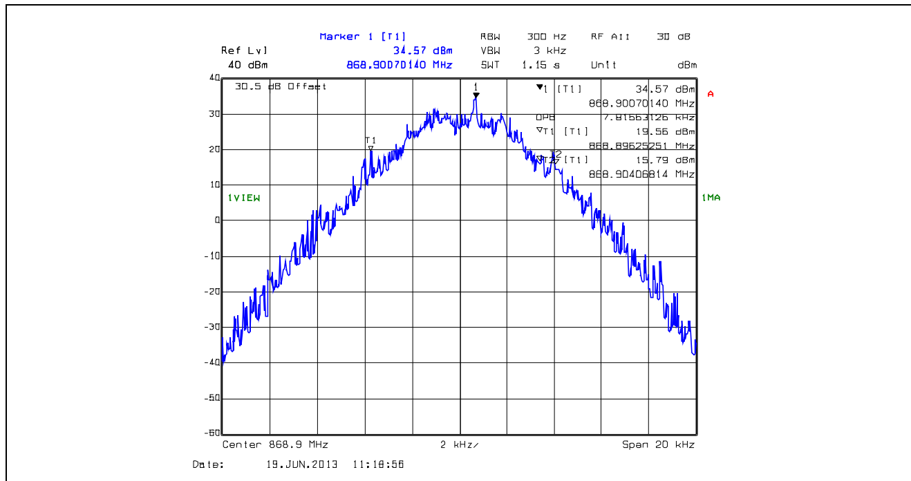
Plot 5.4.4.1.72. 99% Occupied Bandwidth, 12.5 kHz Channel Spacing, F1D, 868.9 MHz
