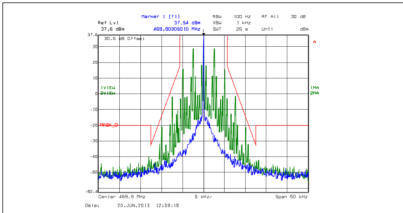
Plot 5.4.4.2.3. Emission Mask D, 12.5 kHz Channel Spacing, F3E, High Power, 469.9 MHz
