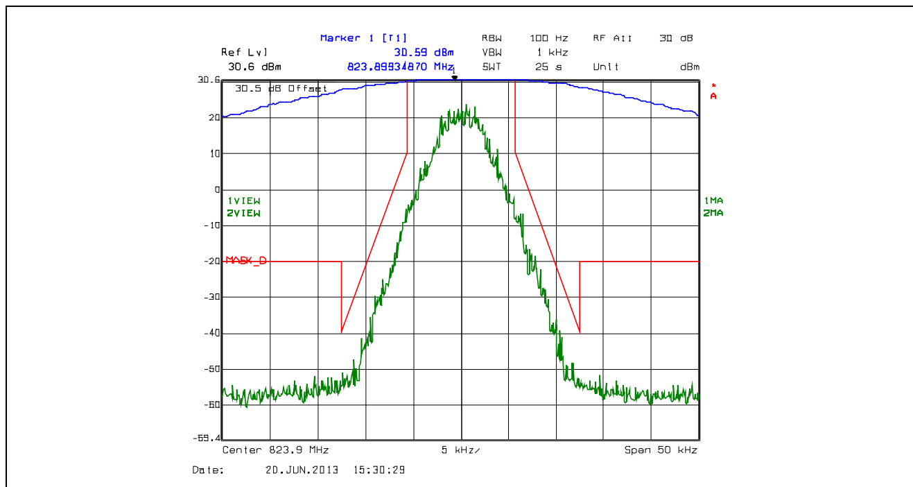
Plot 5.4.4.2.48. Emission Mask D, 12.5 kHz Channel Spacing, F1E, Low Power, 823.9 MHz
