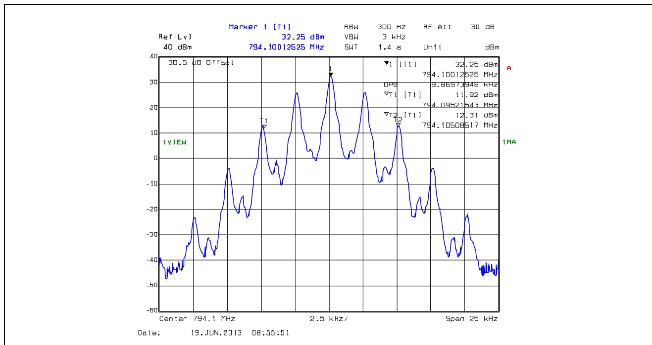
Plot 5.4.4.1.31. 99% Occupied Bandwidth, 12.5 kHz Channel Spacing, F3E, 794.1 MHz
