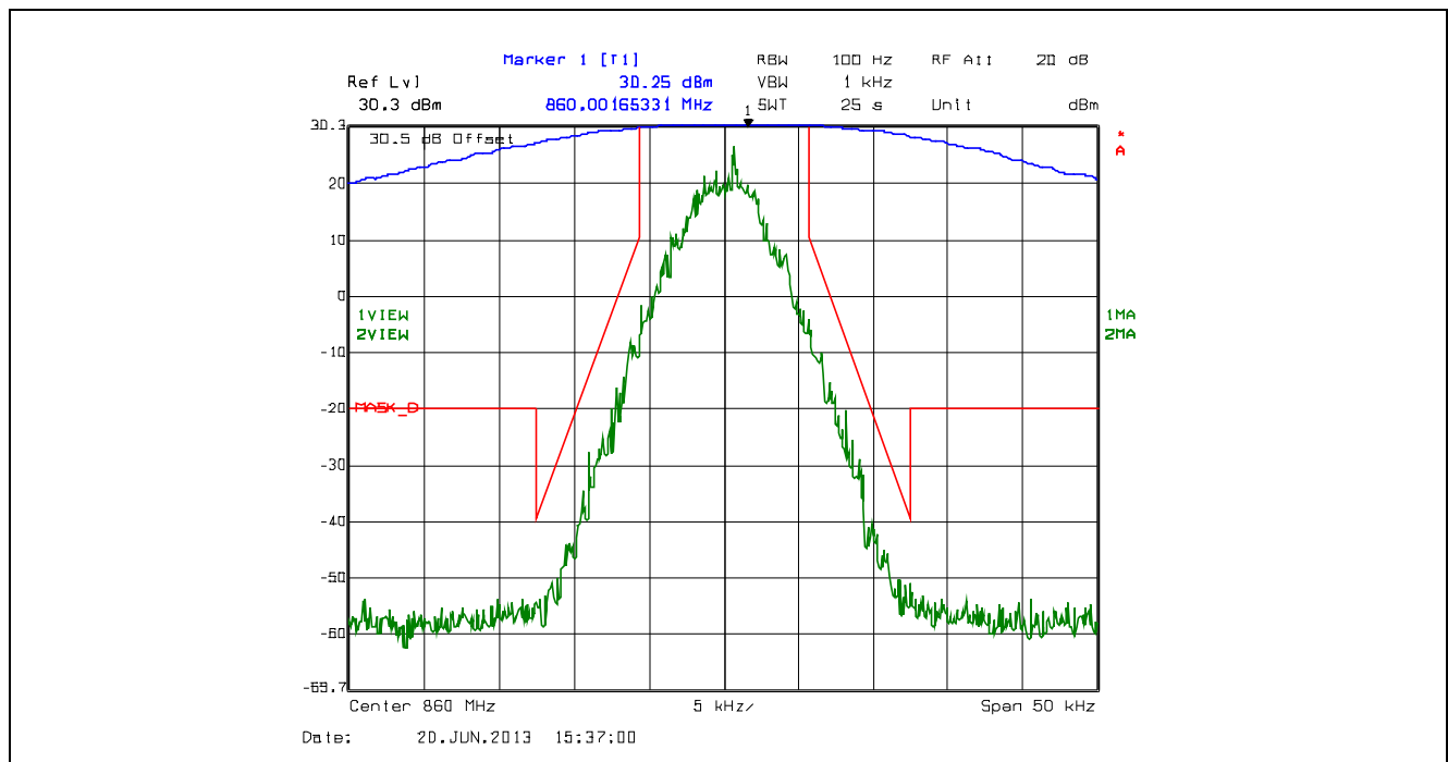
Plot 5.4.4.2.76. Emission Mask D, 12.5 kHz Channel Spacing, F1E, Low Power, 860.0 MHz
