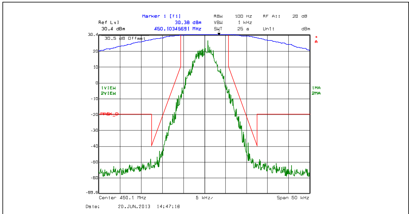
Plot 5.4.4.2.14. Emission Mask D, 12.5 kHz Channel Spacing, F1E, Low Power, 450.1 MHz
