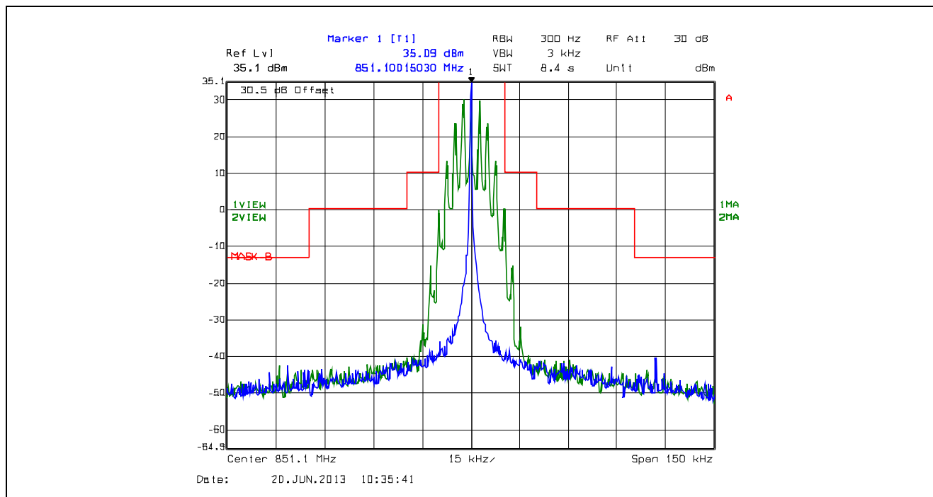
Plot 5.4.4.2.67. Emission Mask B, 25 kHz Channel Spacing, F3E, High Power, 851.1 MHz
