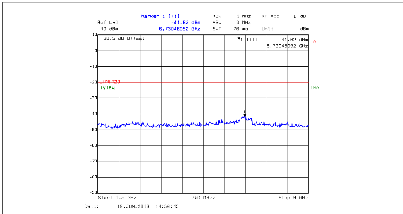
Plot 5.5.4.20. Conducted Transmitter Spurious Emissions, Low Power, 769.5 MHz, 1.5 GHz - 9 GHz
