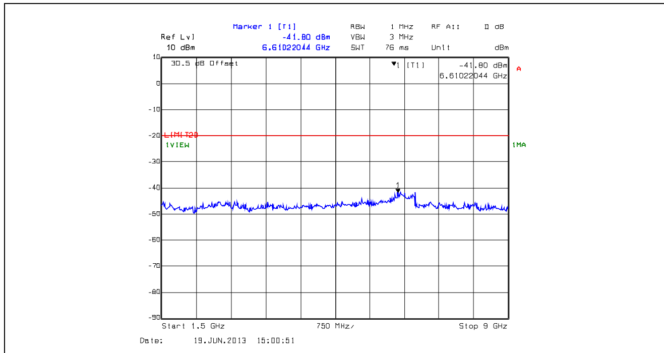
Plot 5.5.4.28. Conducted Transmitter Spurious Emissions, Low Power, 794.1 MHz, 1.5 GHz - 9 GHz
