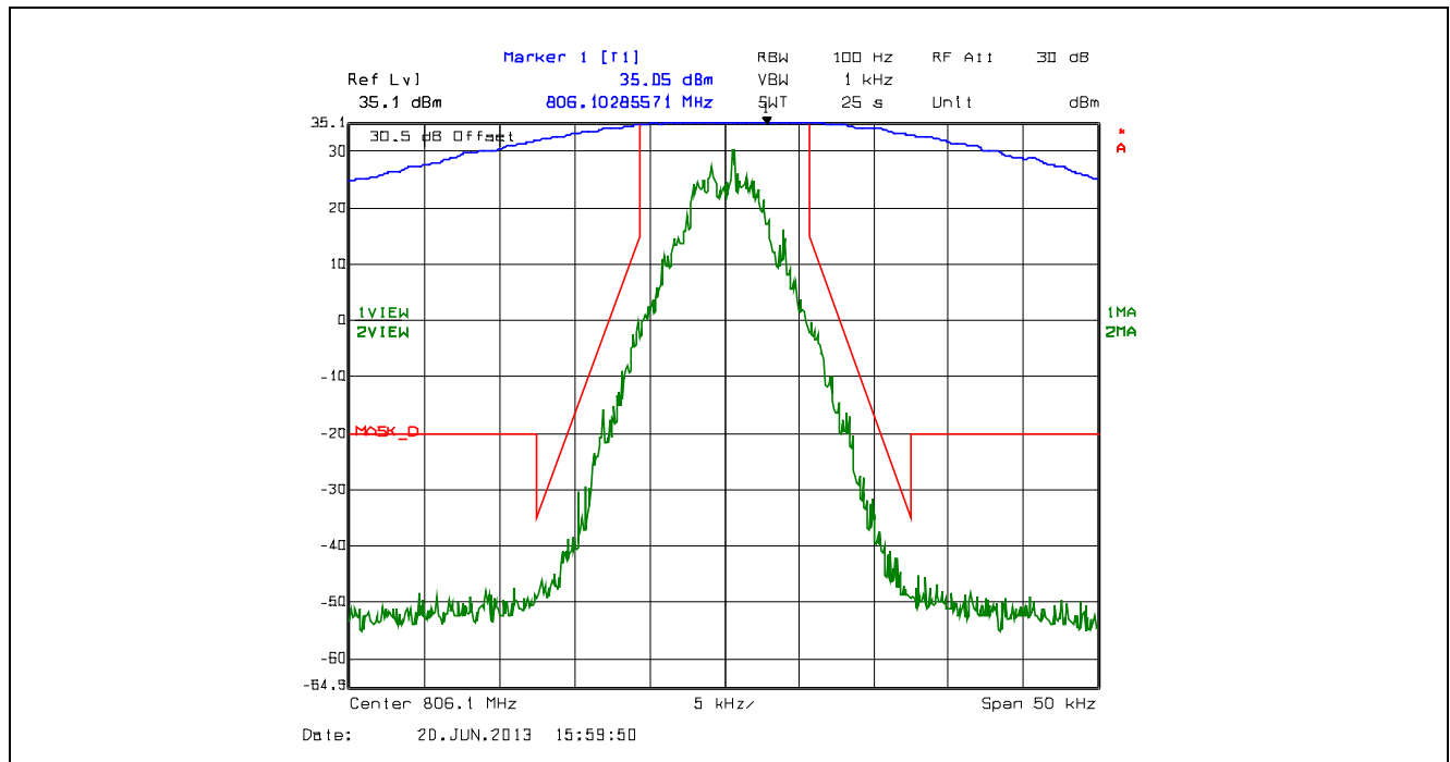
Plot 5.4.4.2.43. Emission Mask D, 12.5 kHz Channel Spacing, F1E, High Power, 806.1 MHz
