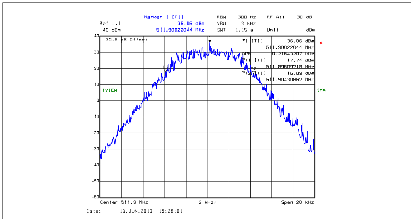
Plot 5.4.4.1.15. 99% Occupied Bandwidth, 12.5 kHz Channel Spacing, F1W, 511.9 MHz
