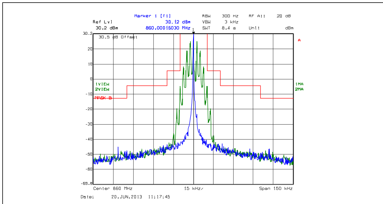
Plot 5.4.4.2.70. Emission Mask B, 25 kHz Channel Spacing, F3E, Low Power, 860.0 MHz
