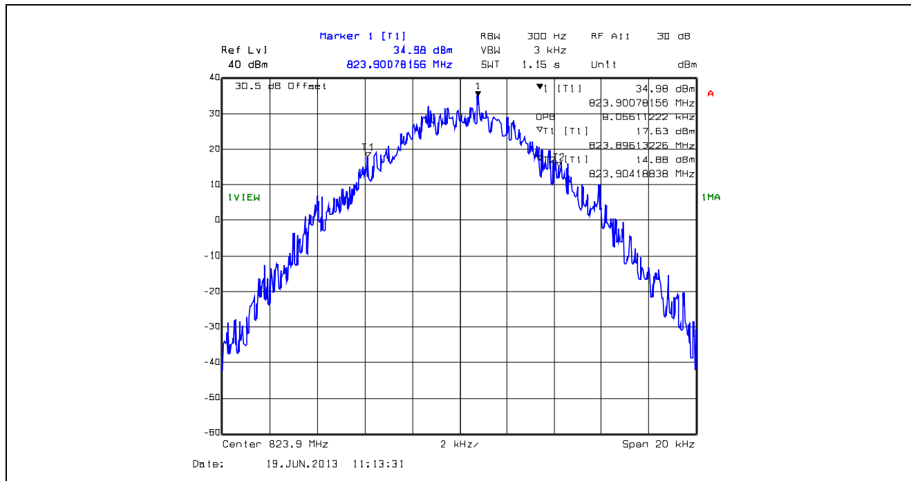
Plot 5.4.4.1.57. 99% Occupied Bandwidth, 12.5 kHz Channel Spacing, F1D, 823.9 MHz
