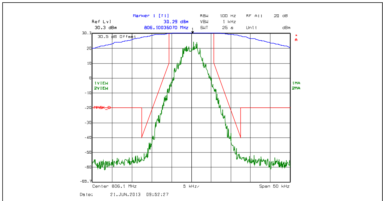
Plot 5.4.4.2.50. Emission Mask D, 12.5 kHz Channel Spacing, F1D, Low Power, 806.1 MHz
