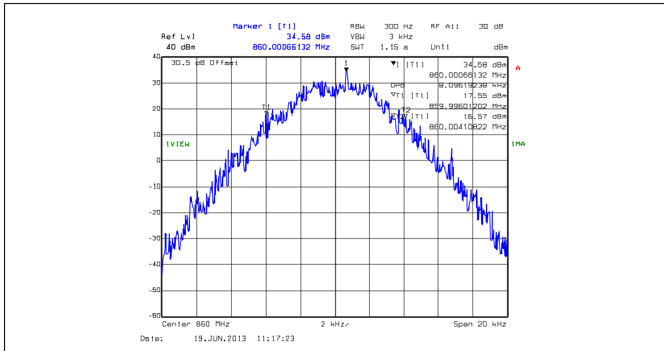
Plot 5.4.4.1.71. 99% Occupied Bandwidth, 12.5 kHz Channel Spacing, F1D, 860.0 MHz
