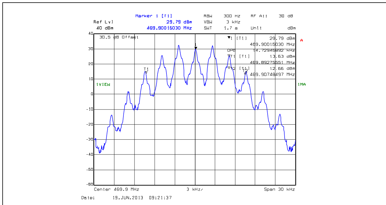
Plot 5.4.4.1.5. 99% Occupied Bandwidth, 25 kHz Channel Spacing, F3E, 469.9 MHz
