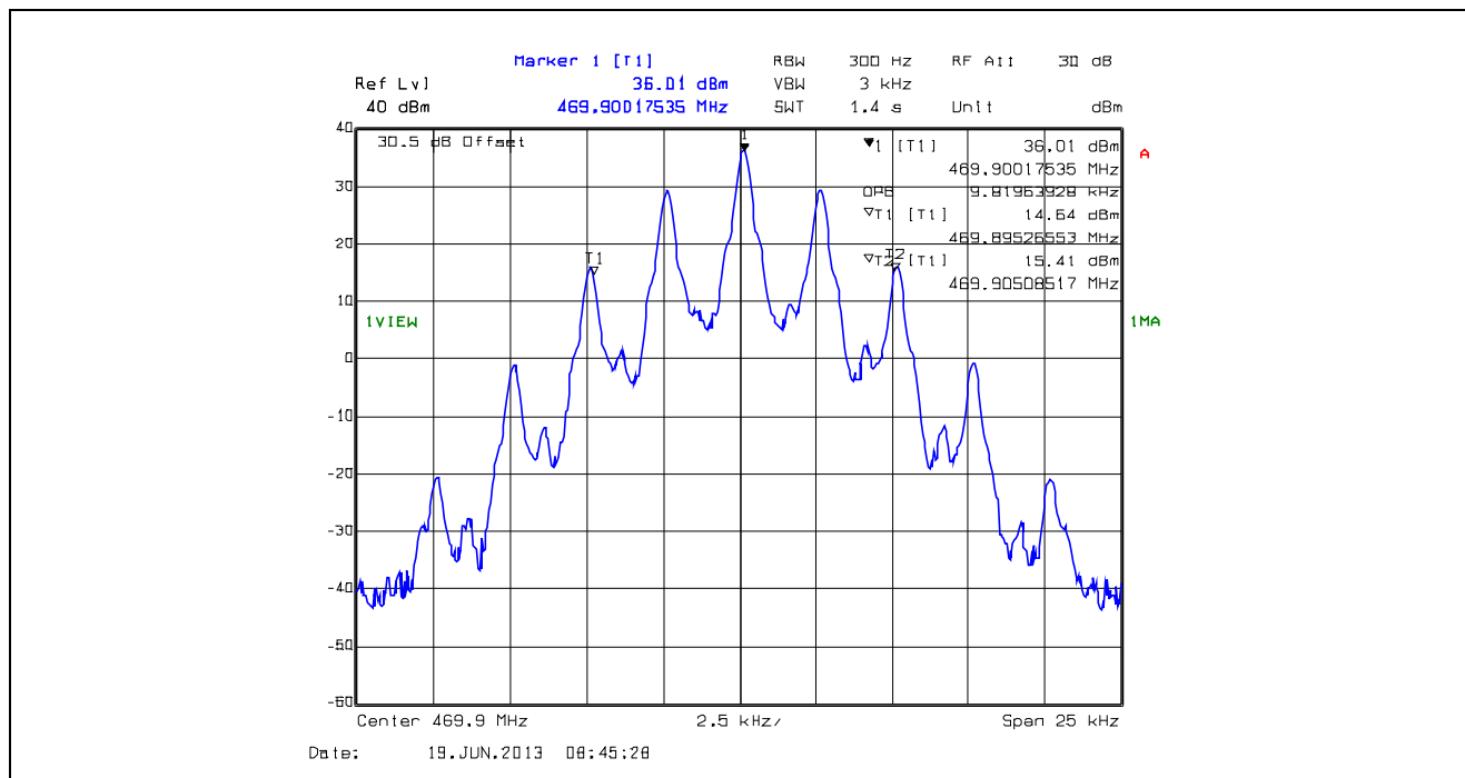
Plot 5.4.4.1.2. 99% Occupied Bandwidth, 12.5 kHz Channel Spacing, F3E, 469.9 MHz
