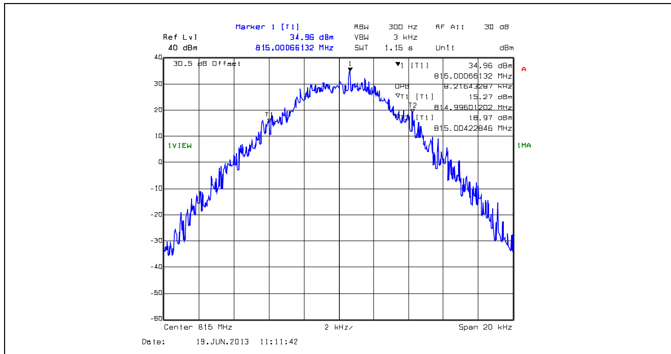
Plot 5.4.4.1.56. 99% Occupied Bandwidth, 12.5 kHz Channel Spacing, F1D, 815.0 MHz
