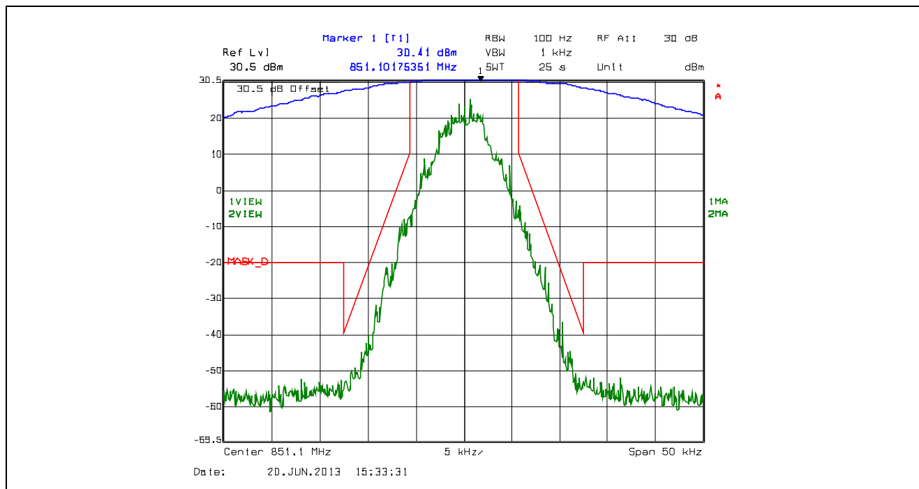
Plot 5.4.4.2.74. Emission Mask D, 12.5 kHz Channel Spacing, F1E, Low Power, 851.1 MHz
