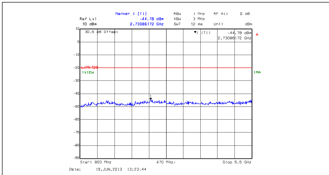
Plot 5.5.4.8. Conducted Transmitter Spurious Emissions, Low Power, 469.9 MHz, 800 MHz - 5.5 GHz
