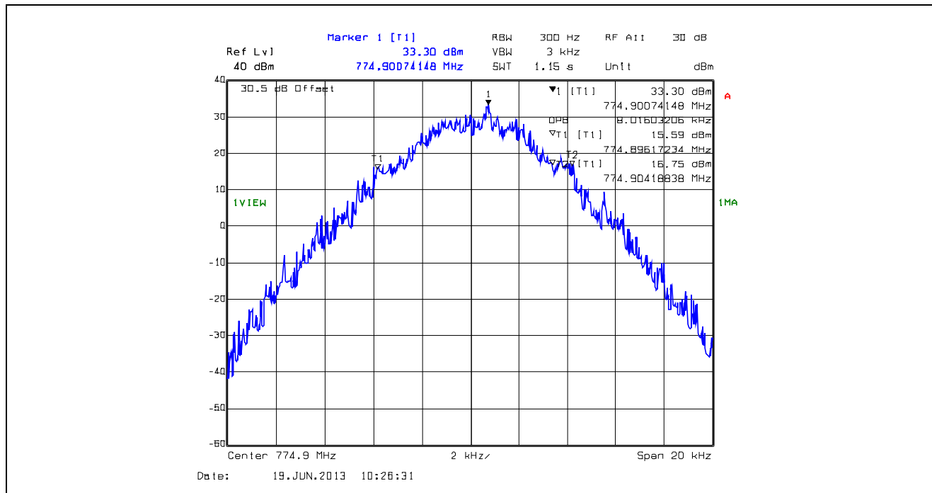
Plot 5.4.4.1.24. 99% Occupied Bandwidth, 12.5 kHz Channel Spacing, F1E, 774.9 MHz
