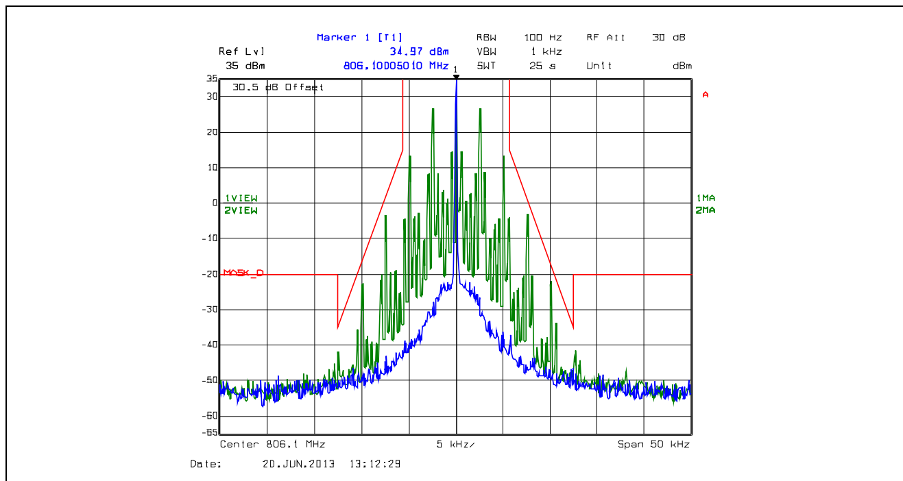
Plot 5.4.4.2.31. Emission Mask D, 12.5 kHz Channel Spacing, F3E, High Power, 806.1 MHz
