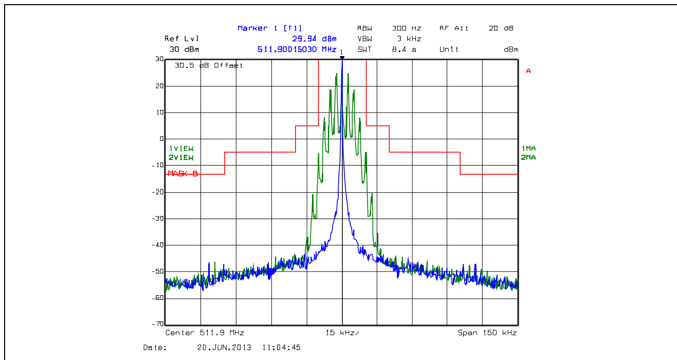
Plot 5.4.4.2.12. Emission Mask B, 25 kHz Channel Spacing, F3E, Low Power, 511.9 MHz
