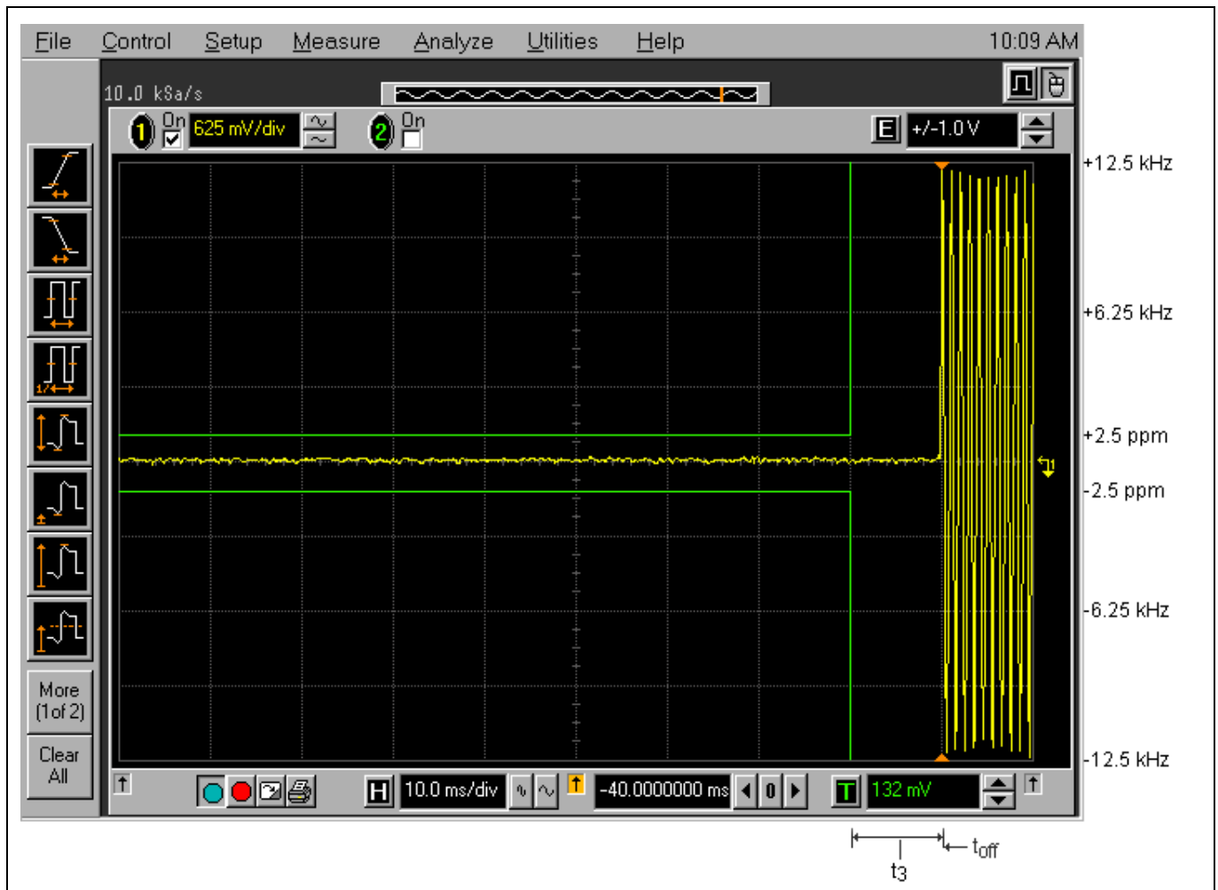
Plot 5.8.4.2. Transient Frequency Behavior on 12.5 kHz Channels Test Frequency: 450.1 MHz; Power: 5 W; Test Conditions: Switch off condition t_3 , t_{off}
