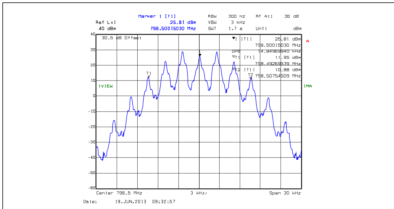
Plot 5.4.4.1.35. 99% Occupied Bandwidth, 25 kHz Channel Spacing, F3E, 798.5 MHz
