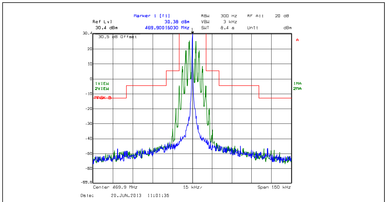
Plot 5.4.4.2.10. Emission Mask B, 25 kHz Channel Spacing, F3E, Low Power, 469.9 MHz
