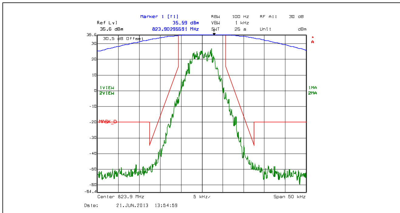
Plot 5.4.4.2.59. Emission Mask D, 12.5 kHz Channel Spacing, F1W, High Power, 823.9 MHz
