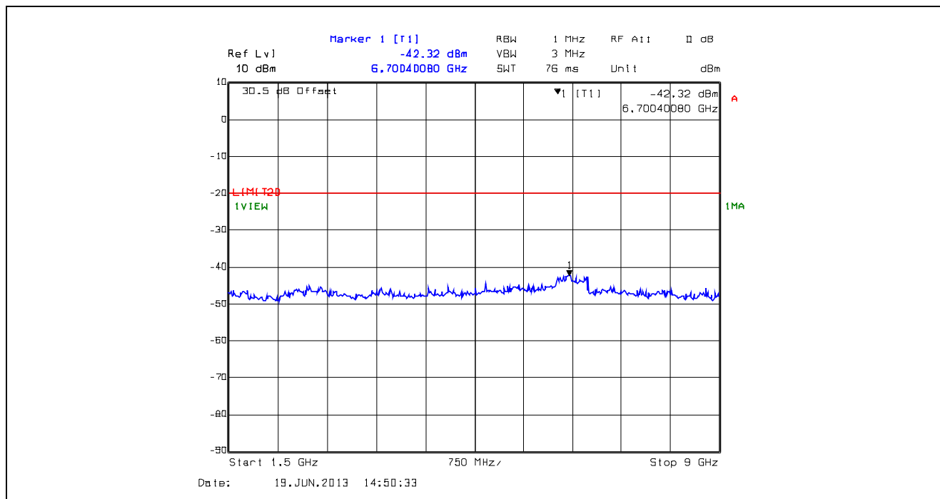
Plot 5.5.4.34. Conducted Transmitter Spurious Emissions, High Power, 804.9 MHz, 1.5 GHz - 9 GHz
