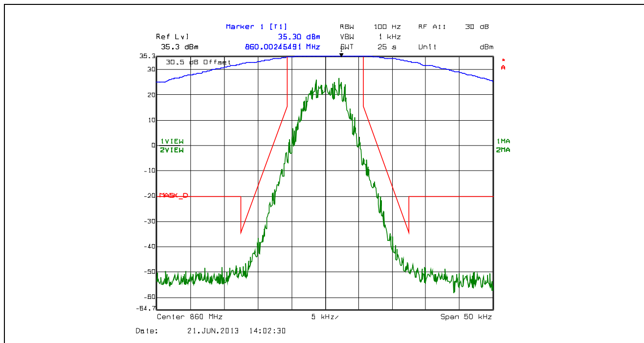
Plot 5.4.4.2.87. Emission Mask D, 12.5 kHz Channel Spacing, F1W, High Power, 860.0 MHz
