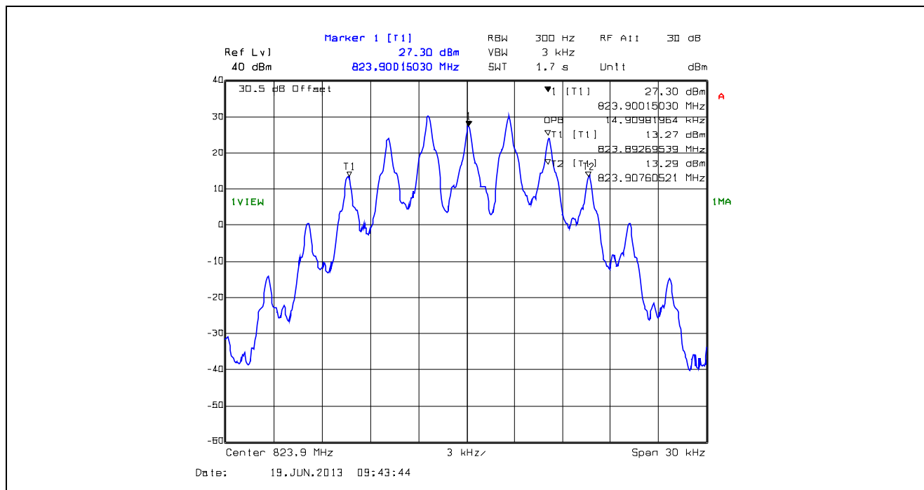
Plot 5.4.4.1.51. 99% Occupied Bandwidth, 25 kHz Channel Spacing, F3E, 823.9 MHz
