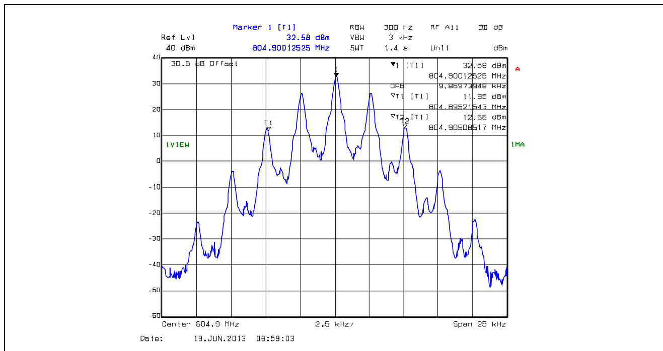
Plot 5.4.4.1.33. 99% Occupied Bandwidth, 12.5 kHz Channel Spacing, F3E, 804.9 MHz
