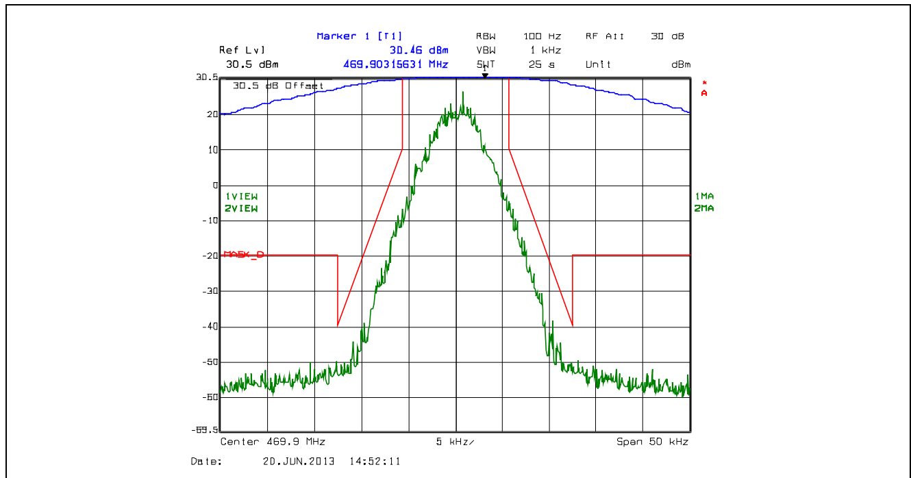
Plot 5.4.4.2.16. Emission Mask D, 12.5 kHz Channel Spacing, F1E, Low Power, 469.9 MHz
