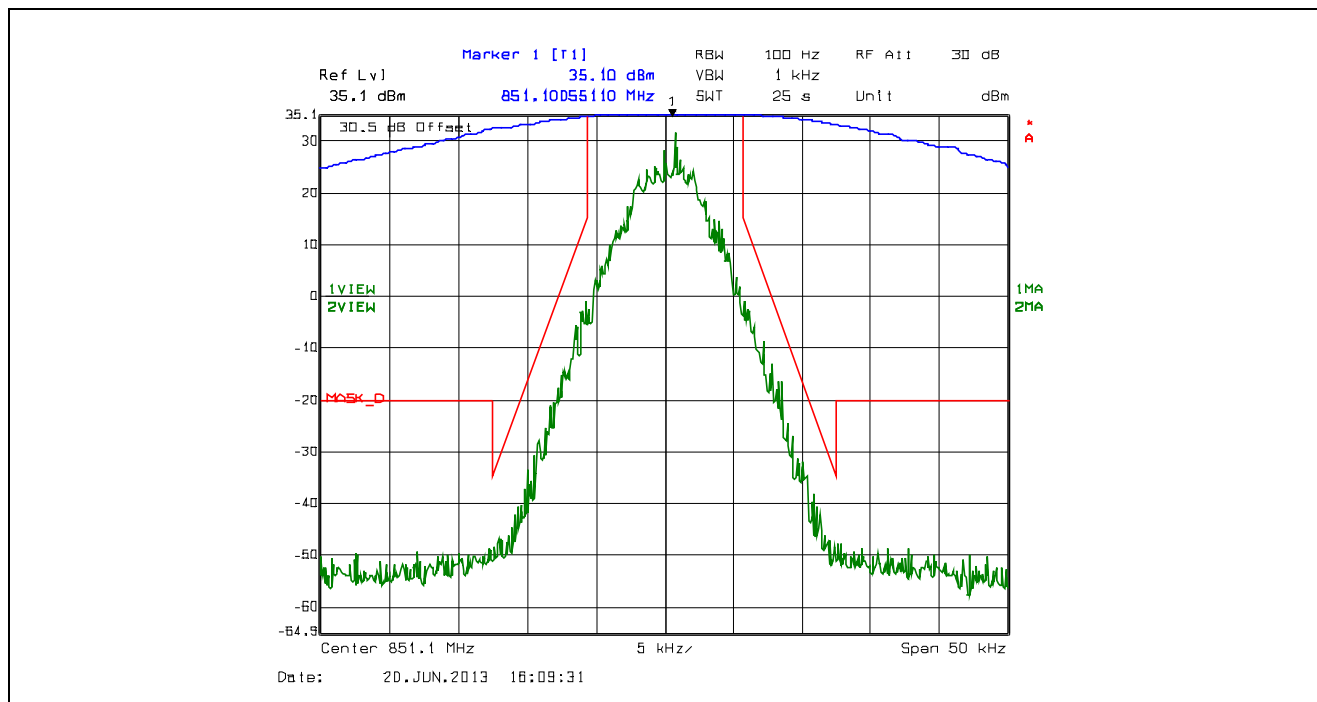
Plot 5.4.4.2.73. Emission Mask D, 12.5 kHz Channel Spacing, F1E, High Power, 851.1 MHz
