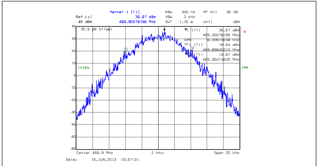
Plot 5.4.4.1.11. 99% Occupied Bandwidth, 12.5 kHz Channel Spacing, F1D, 469.9 MHz
