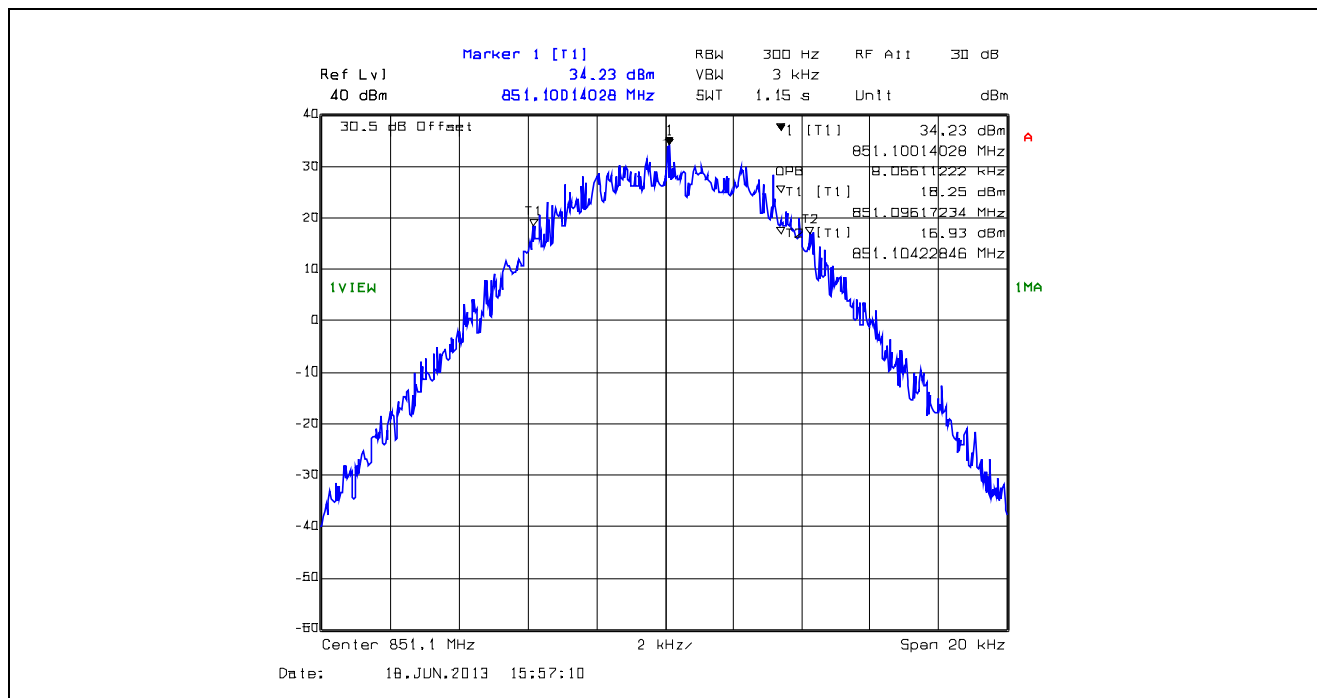
Plot 5.4.4.1.73. 99% Occupied Bandwidth, 12.5 kHz Channel Spacing, F1W, 851.1 MHz
