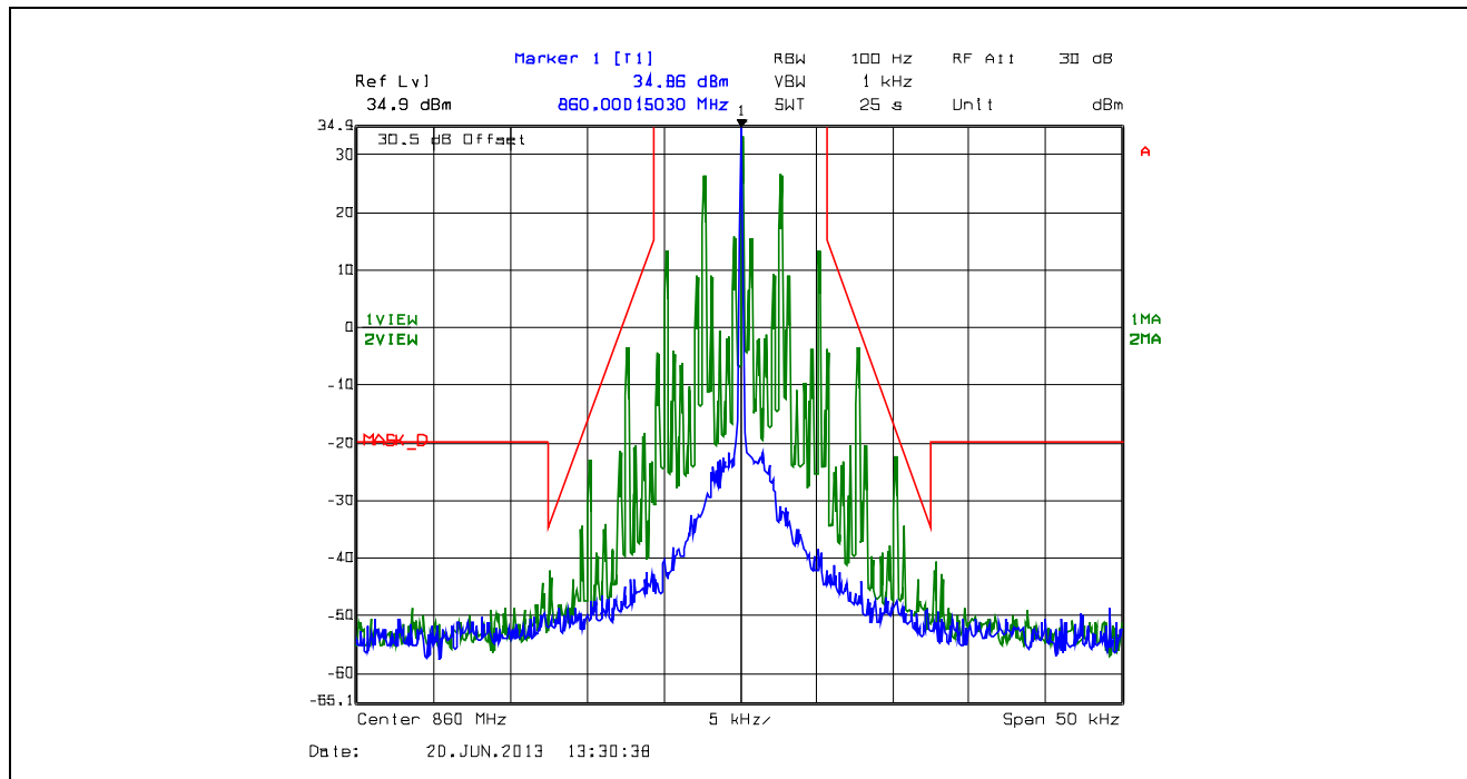
Plot 5.4.4.2.63. Emission Mask D, 12.5 kHz Channel Spacing, F3E, High Power, 860.0 MHz
