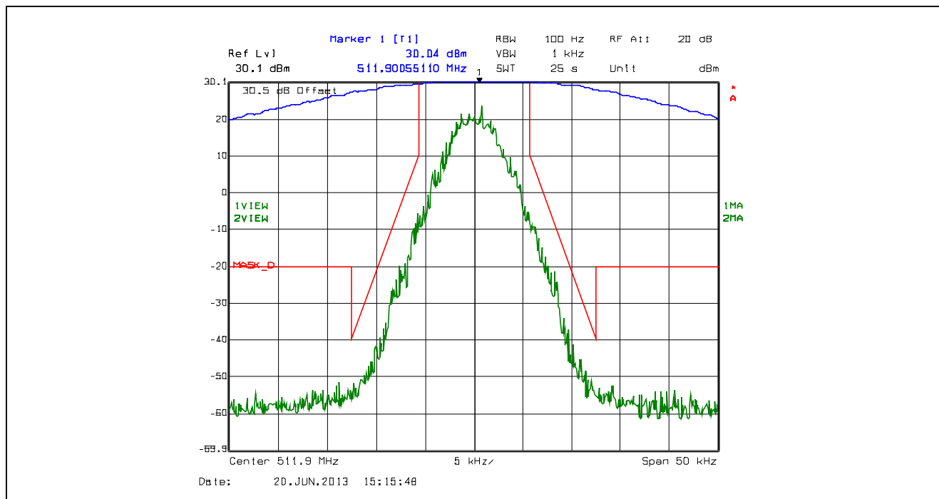
Plot 5.4.4.2.18. Emission Mask D, 12.5 kHz Channel Spacing, F1E, Low Power, 511.9 MHz
