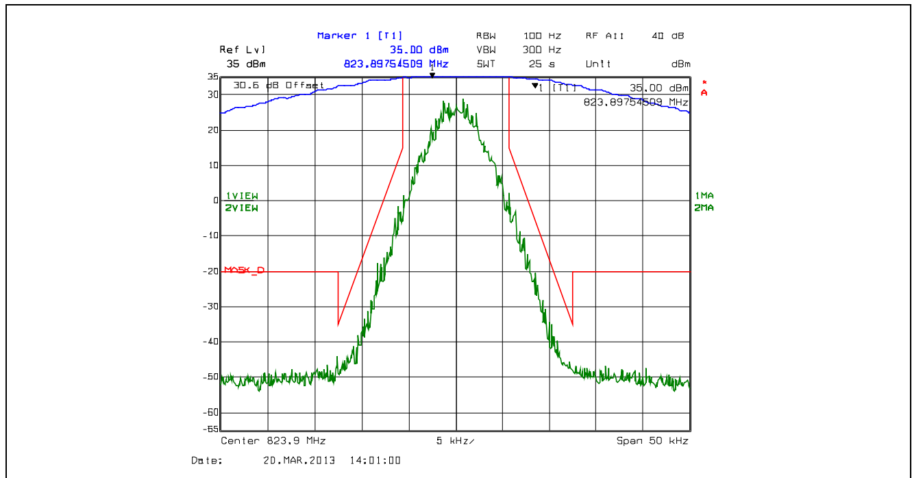
Plot 5.4.4.2.49. Emission Mask D, 12.5 kHz Channel Spacing, F1D, High Power, 823.9 MHz
