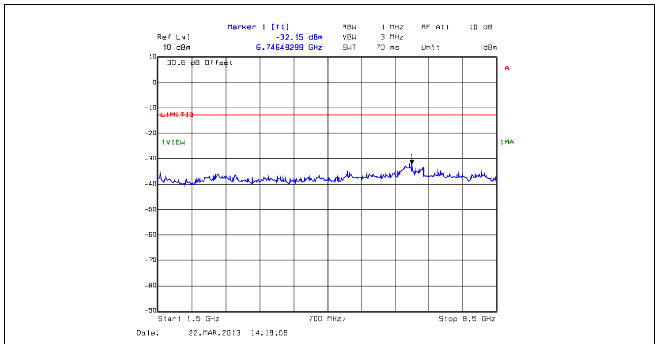
Plot 5.5.4.24. Conducted Transmitter Spurious Emissions, Low Power, 774.9 MHz, 1.5 GHz - 8.5 GHz
