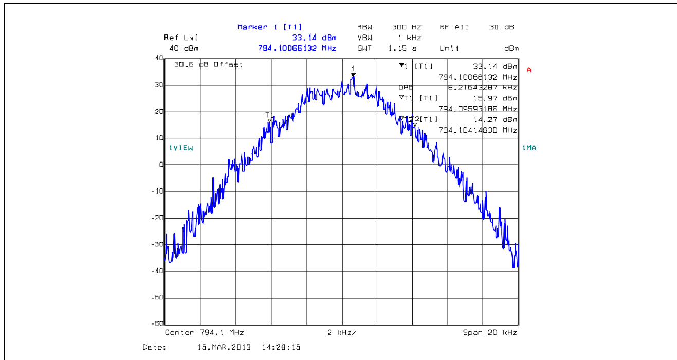
Plot 5.4.4.1.35. 99% Occupied Bandwidth, 12.5 kHz Channel Spacing, F1E, 794.1 MHz
