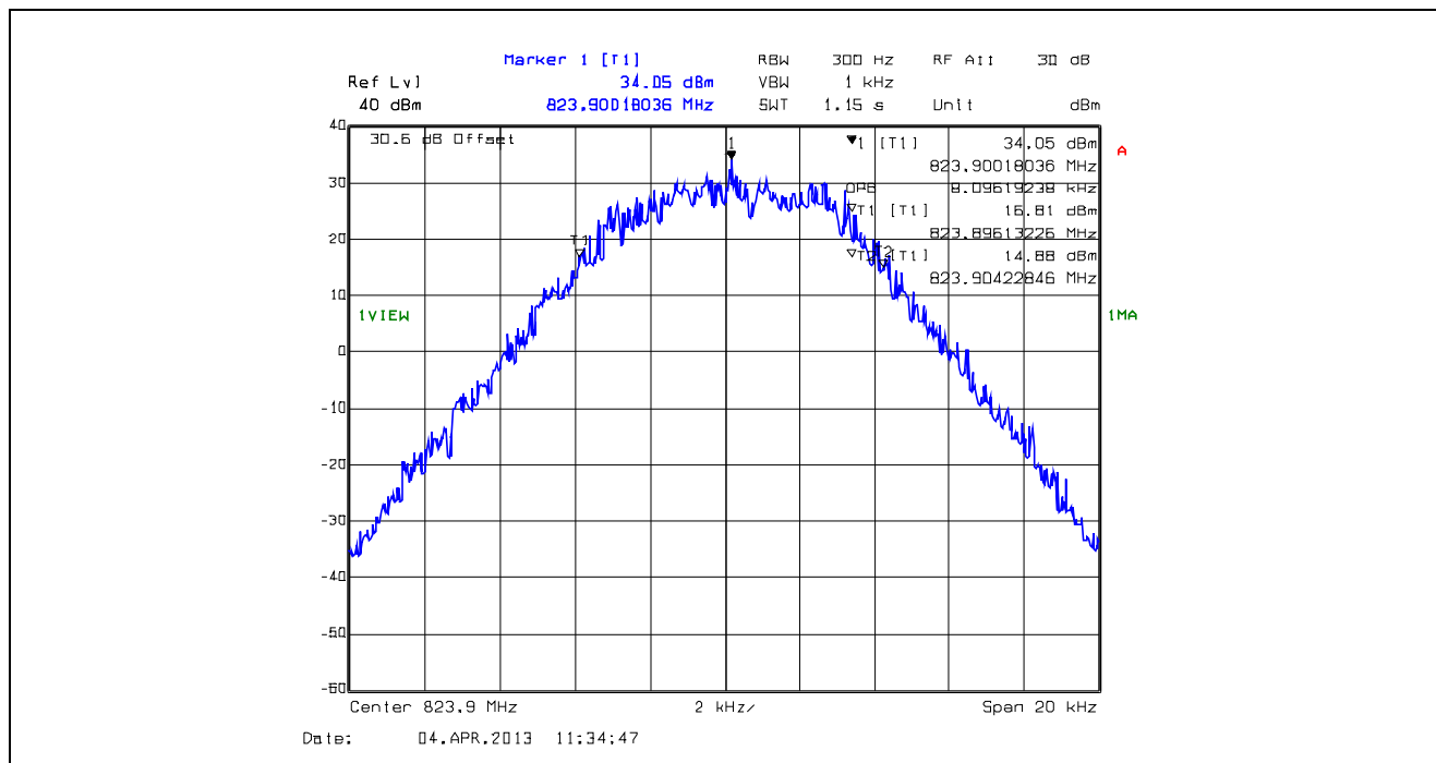
Plot 5.4.4.1.58. 99% Occupied Bandwidth, 12.5 kHz Channel Spacing, F1W, 823.9 MHz
