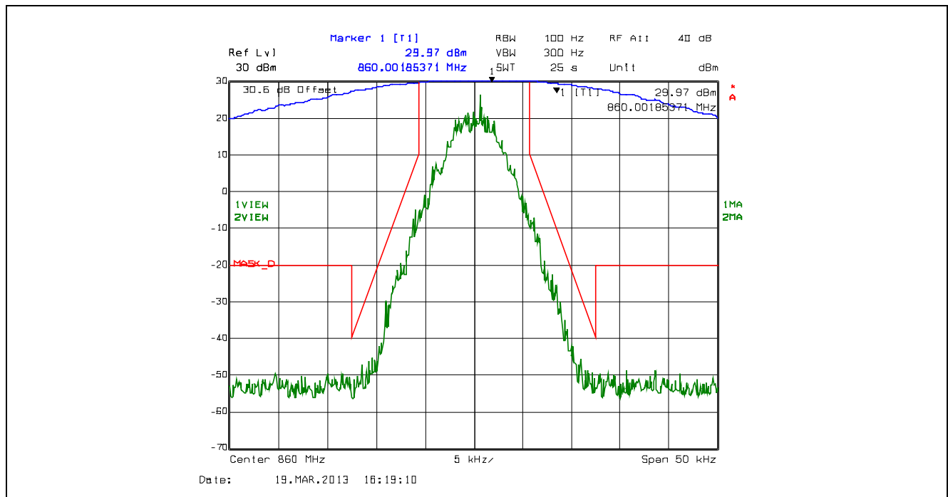
Plot 5.4.4.2.72. Emission Mask D, 12.5 kHz Channel Spacing, F1E, Low Power, 860.0 MHz
