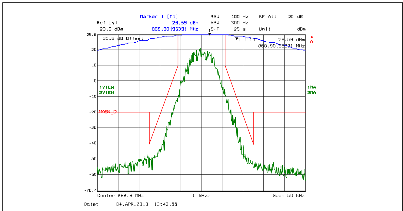
Plot 5.4.4.2.86. Emission Mask D, 12.5 kHz Channel Spacing, F1W, Low Power, 868.9 MHz
