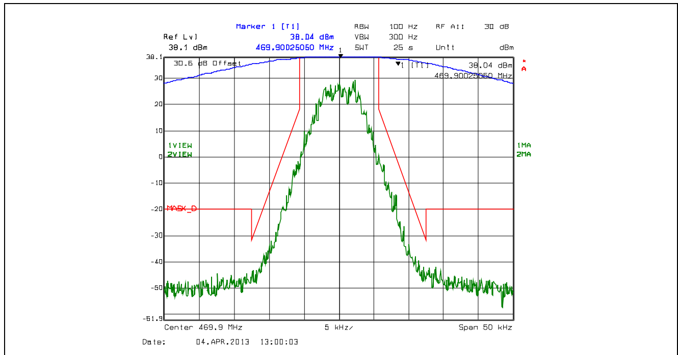
Plot 5.4.4.2.25. Emission Mask D, 12.5 kHz Channel Spacing, F1W, High Power, 469.9 MHz
