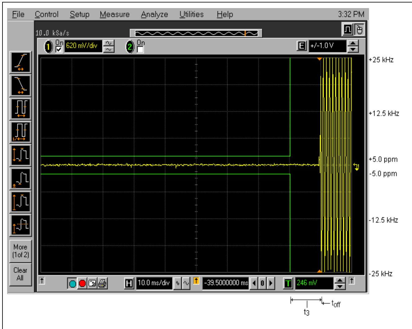
Plot 5.8.4.4. Transient Frequency Behavior on 25 kHz Channels Test Frequency: 406.2 MHz; Power: 5 W; Test Conditions: Switch off condition t_3 , t_{off}
