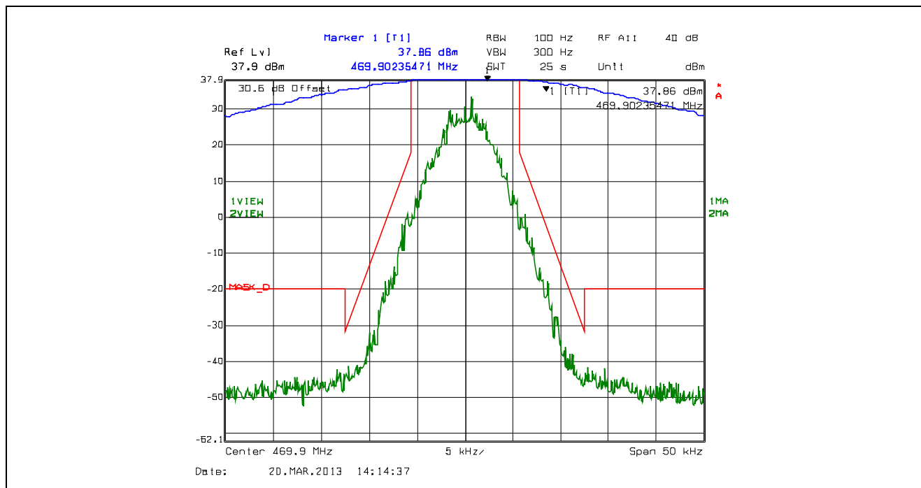
Plot 5.4.4.2.19. Emission Mask D, 12.5 kHz Channel Spacing, F1D, High Power, 469.9 MHz
