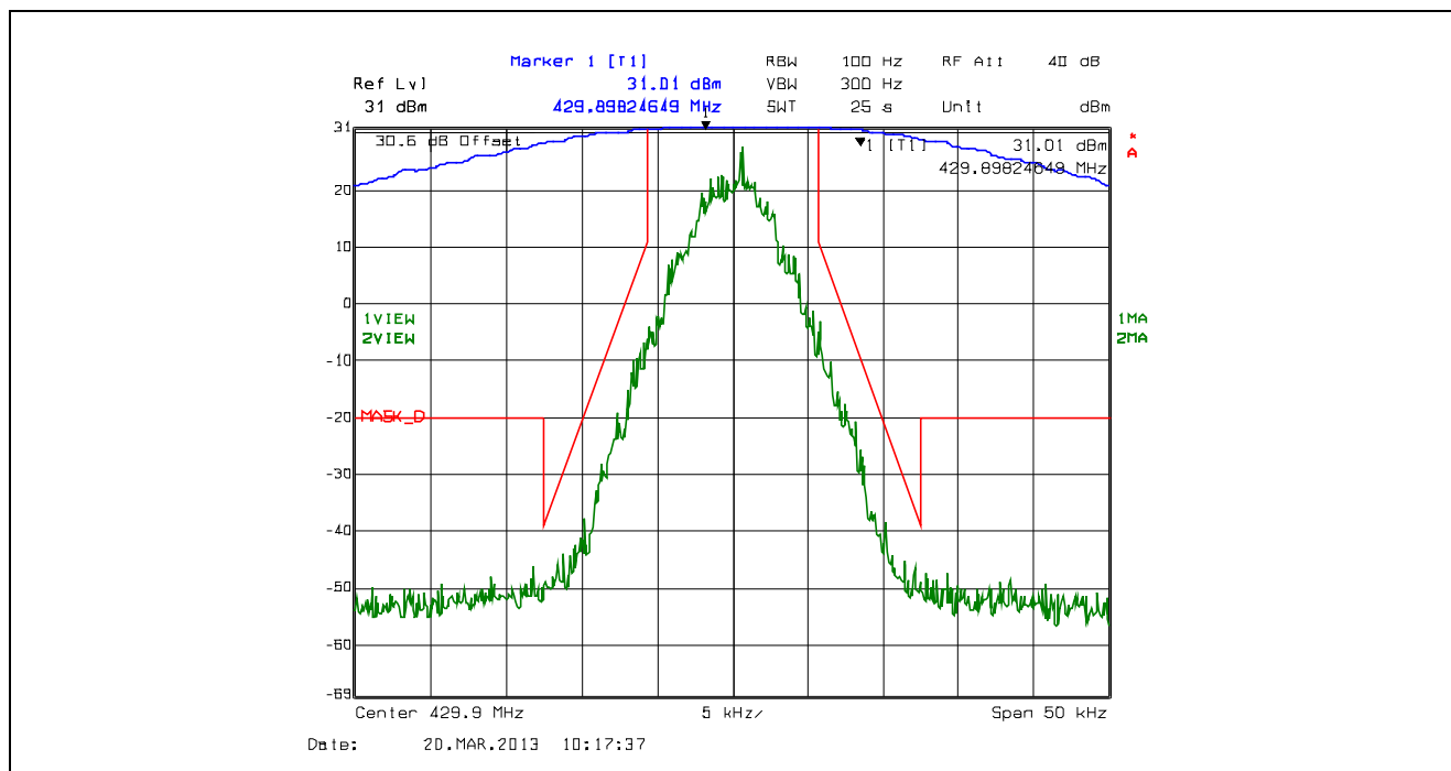
Plot 5.4.4.2.12. Emission Mask D, 12.5 kHz Channel Spacing, F1E, Low Power, 429.9 MHz
