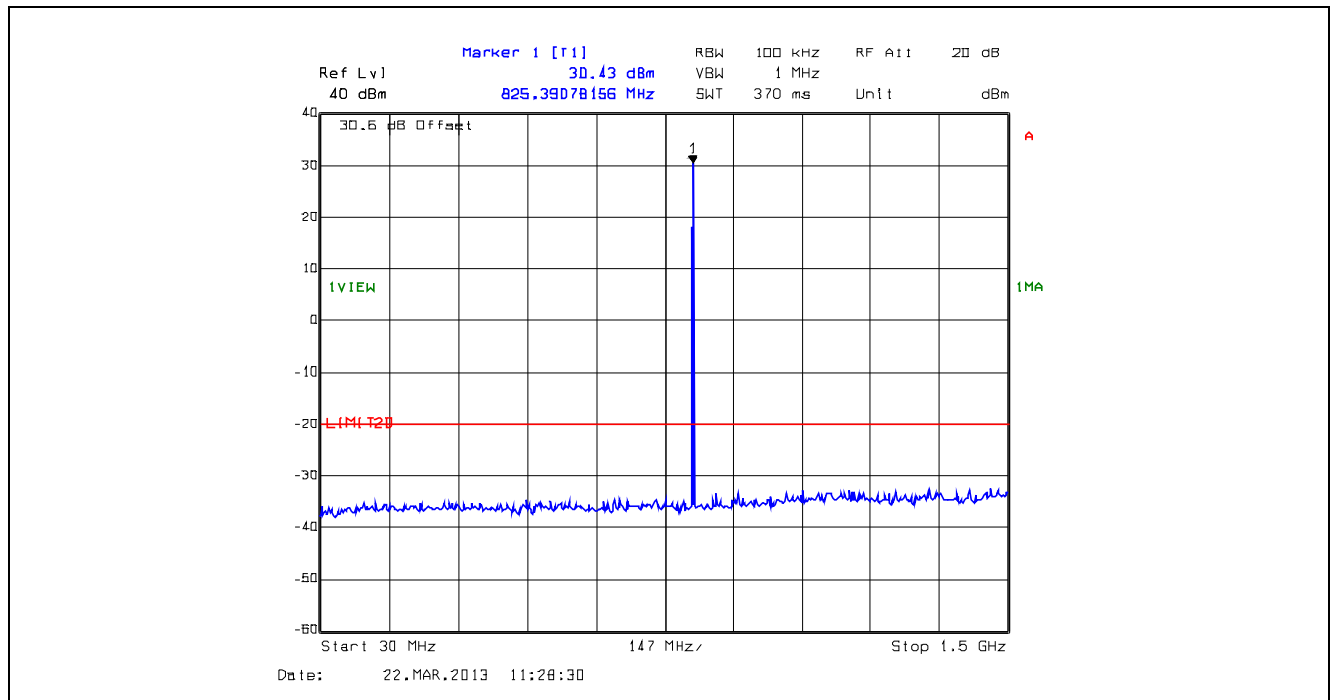
Plot 5.5.4.47. Conducted Transmitter Spurious Emissions, Low Power, 823.9 MHz, 30 MHz - 1.5 GHz
