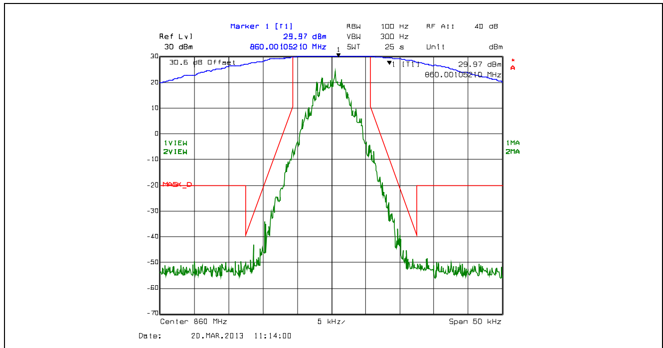
Plot 5.4.4.2.78. Emission Mask D, 12.5 kHz Channel Spacing, F1D, Low Power, 860.0 MHz
