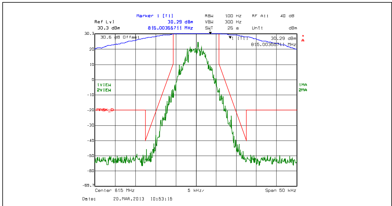
Plot 5.4.4.2.48. Emission Mask D, 12.5 kHz Channel Spacing, F1D, Low Power, 815.0 MHz
