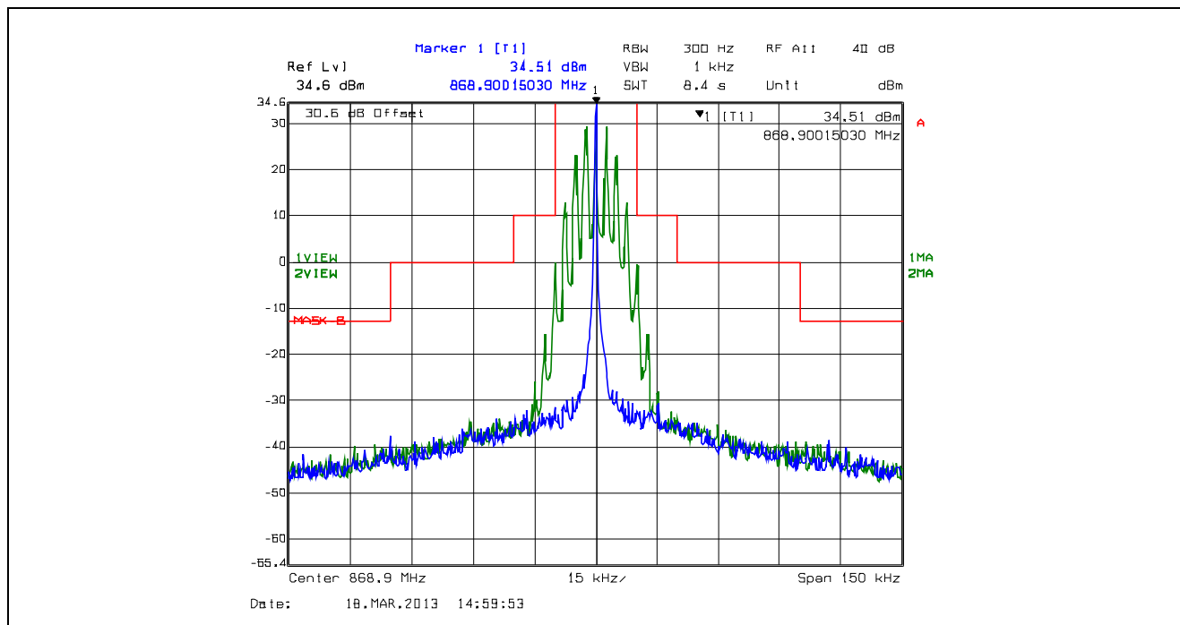
Plot 5.4.4.2.67. Emission Mask B, 25 kHz Channel Spacing, F3E, High Power, 868.9 MHz
