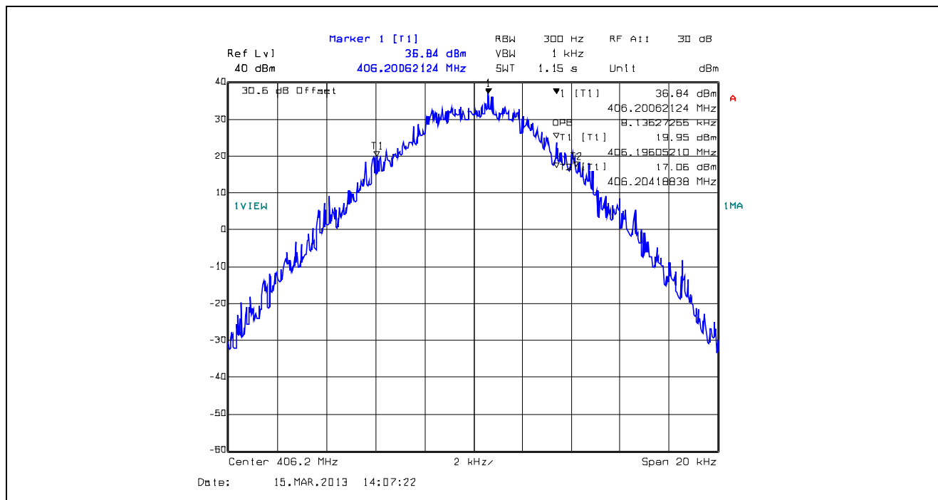
Plot 5.4.4.1.5. 99% Occupied Bandwidth, 12.5 kHz Channel Spacing, F1E, 406.2 MHz
