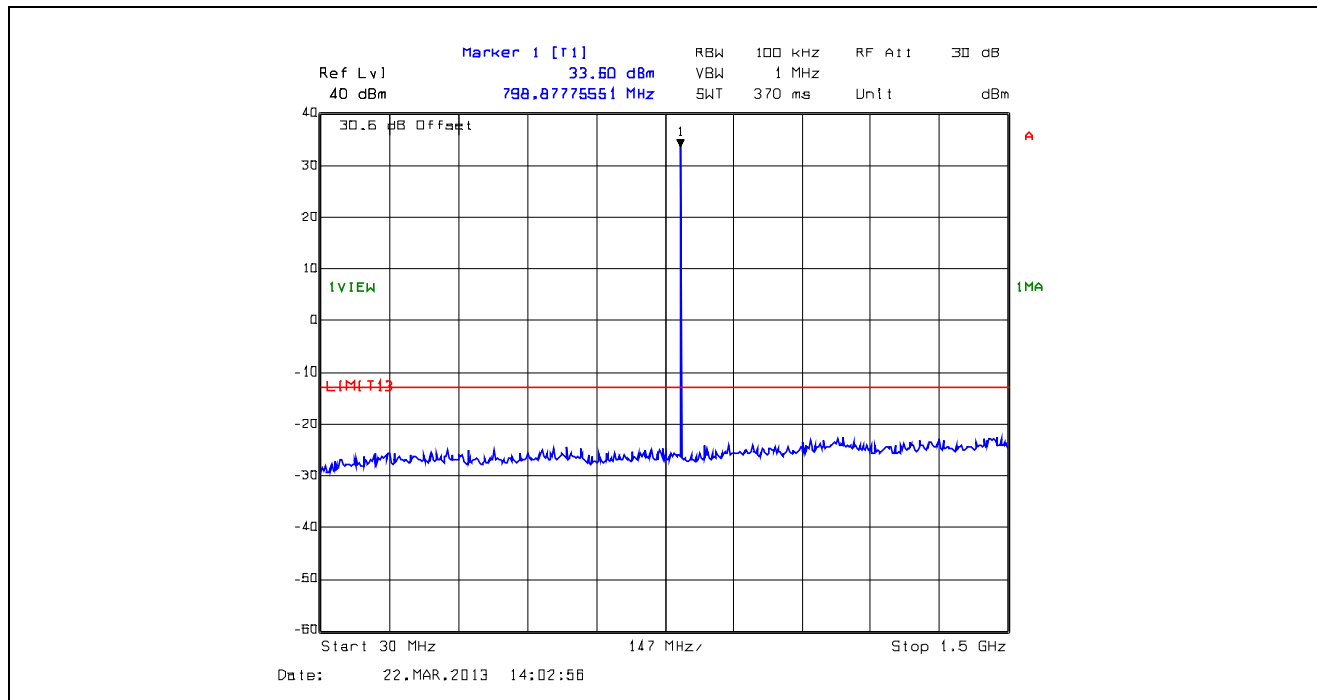
Plot 5.5.4.29. Conducted Transmitter Spurious Emissions, High Power, 798.5 MHz, 30 MHz - 1.5 GHz
