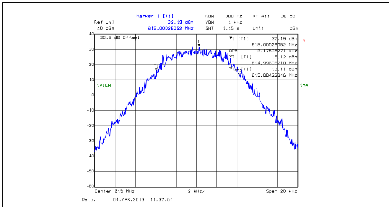
Plot 5.4.4.1.57. 99% Occupied Bandwidth, 12.5 kHz Channel Spacing, F1W, 815.0 MHz
