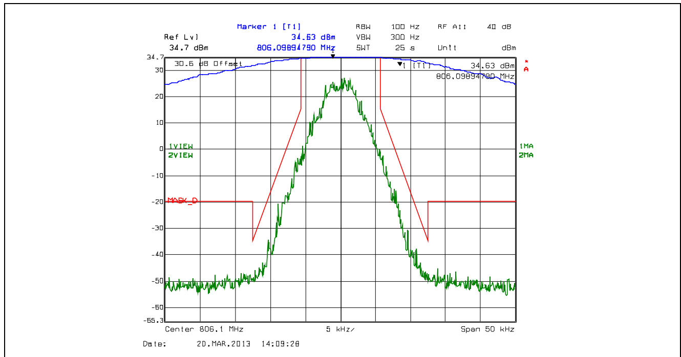
Plot 5.4.4.2.45. Emission Mask D, 12.5 kHz Channel Spacing, F1D, High Power, 806.1 MHz
