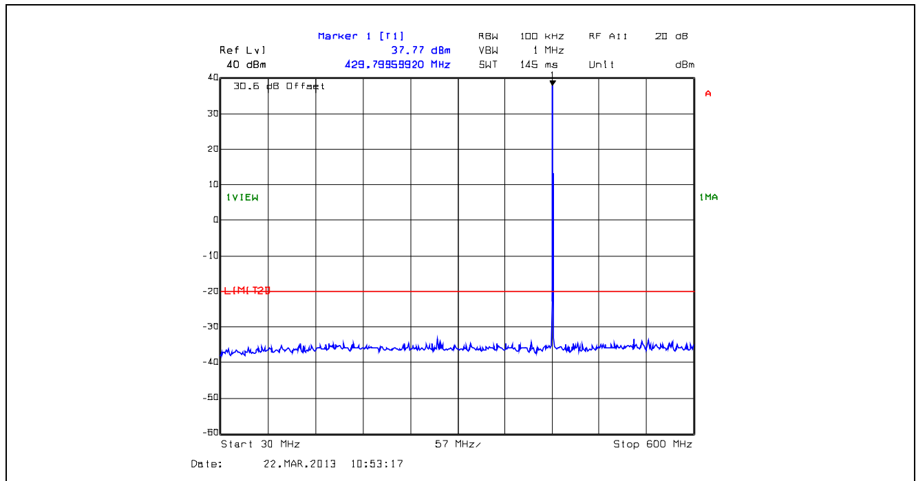
Plot 5.5.4.5. Conducted Transmitter Spurious Emissions, High Power, 429.9 MHz, 30 MHz - 600 MHz
