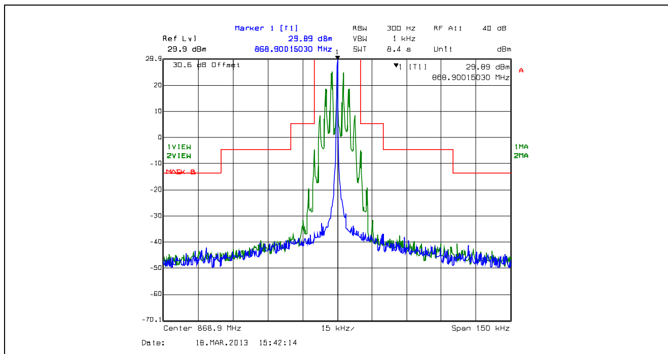
Plot 5.4.4.2.68. Emission Mask B, 25 kHz Channel Spacing, F3E, Low Power, 868.9 MHz
