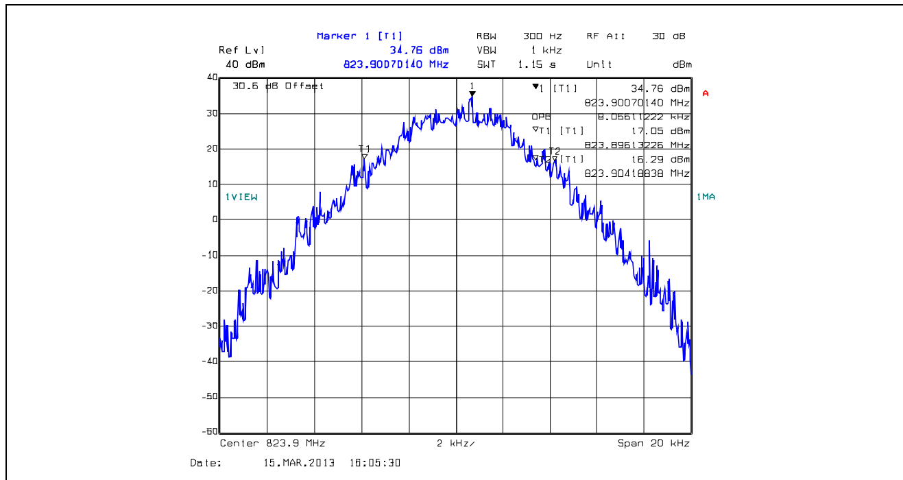
Plot 5.4.4.1.55. 99% Occupied Bandwidth, 12.5 kHz Channel Spacing, F1D, 823.9 MHz
