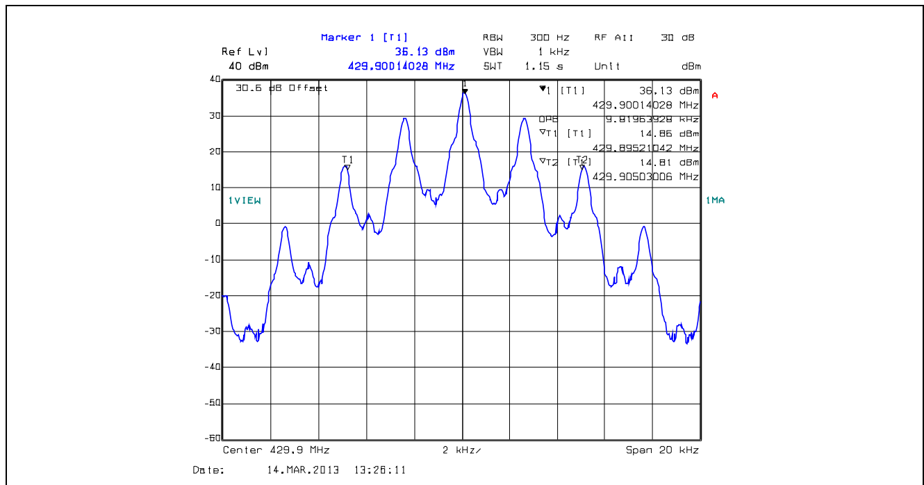
Plot 5.4.4.1.2. 99% Occupied Bandwidth, 12.5 kHz Channel Spacing, F3E, 429.9 MHz
