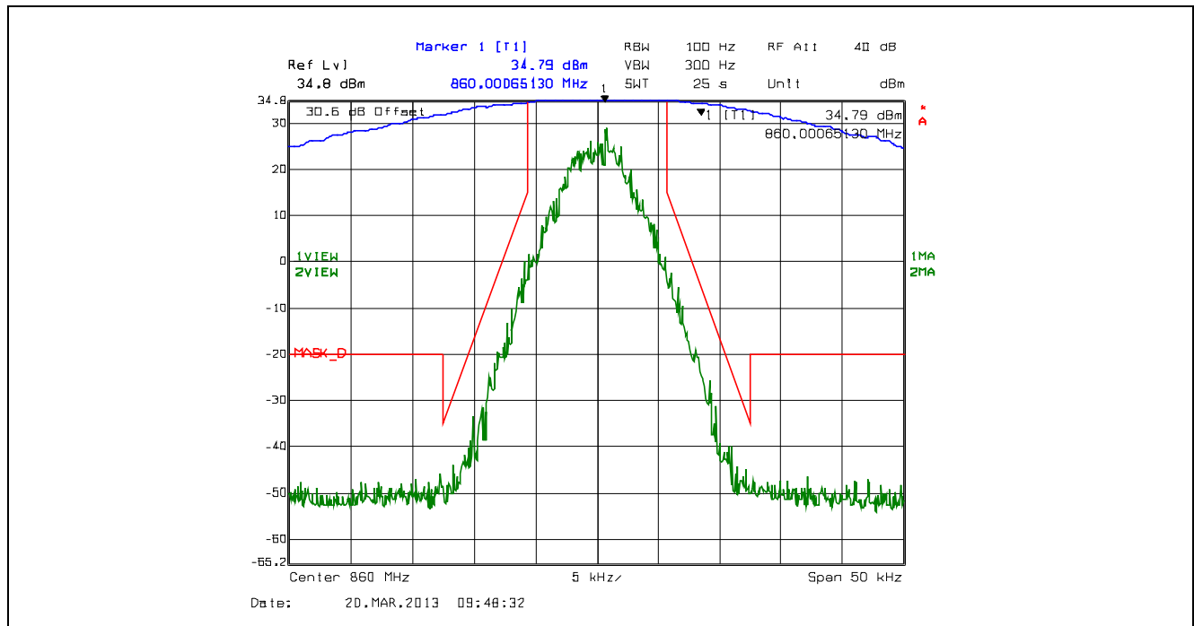
Plot 5.4.4.2.71. Emission Mask D, 12.5 kHz Channel Spacing, F1E, High Power, 860.0 MHz
