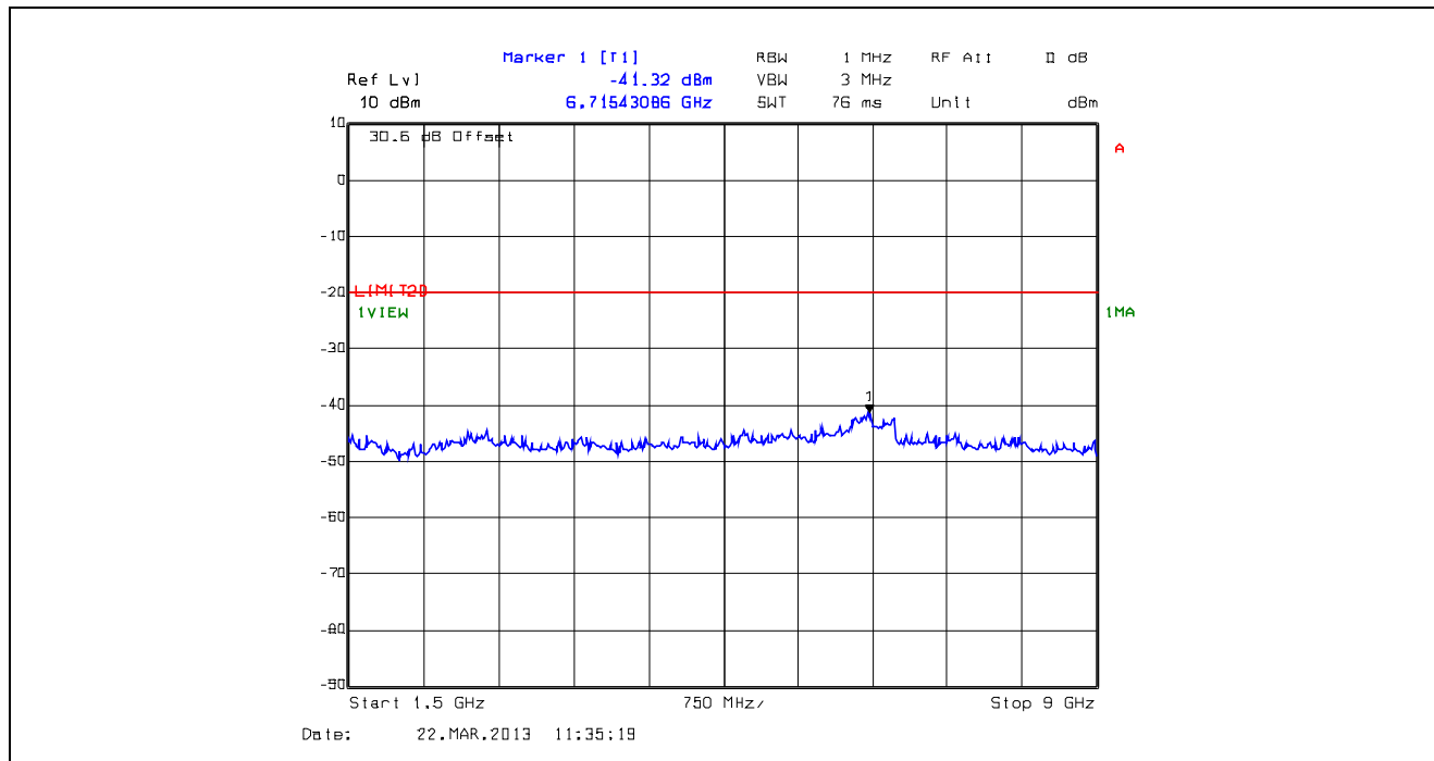
Plot 5.5.4.40. Conducted Transmitter Spurious Emissions, Low Power, 806.1 MHz, 1.5 GHz - 9 GHz
