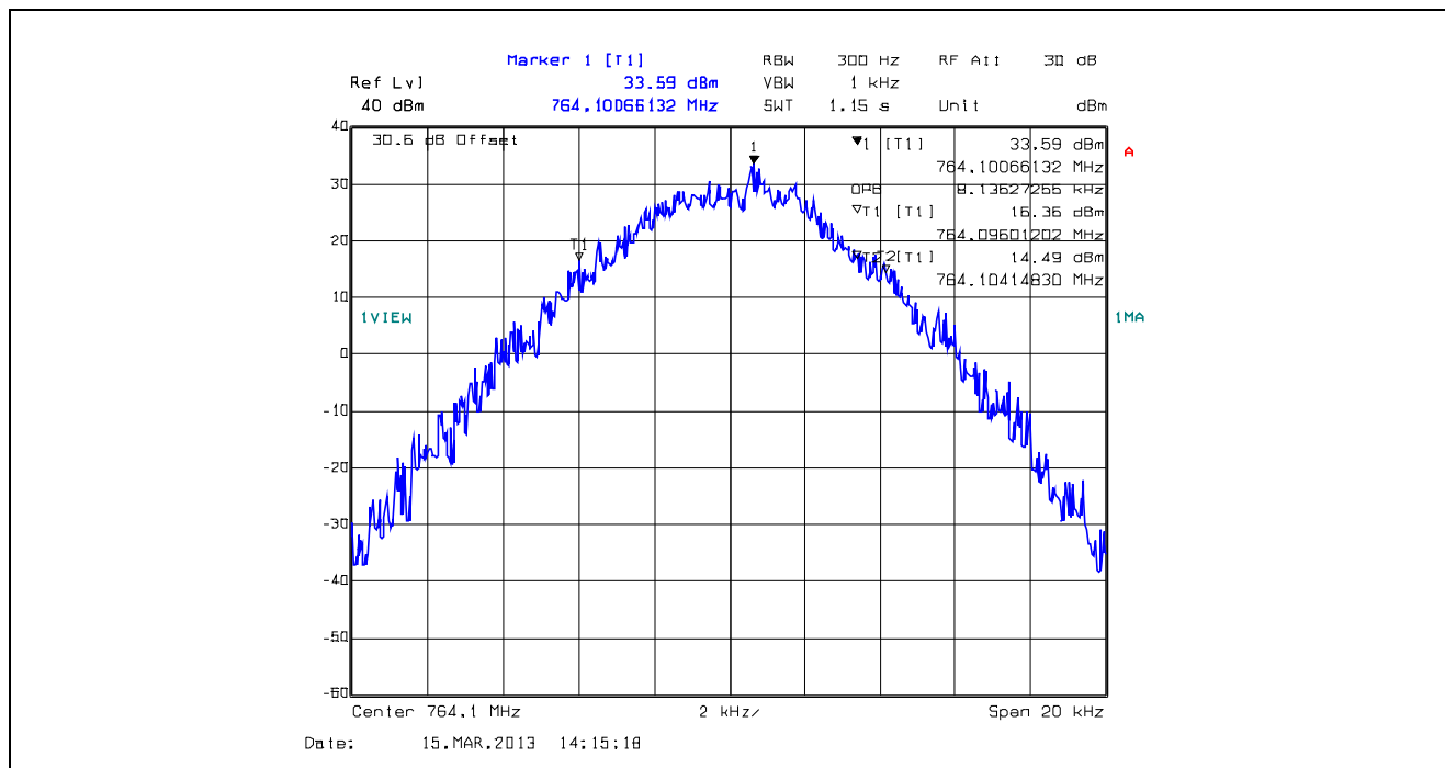
Plot 5.4.4.1.20. 99% Occupied Bandwidth, 12.5 kHz Channel Spacing, F1E, 764.1 MHz
