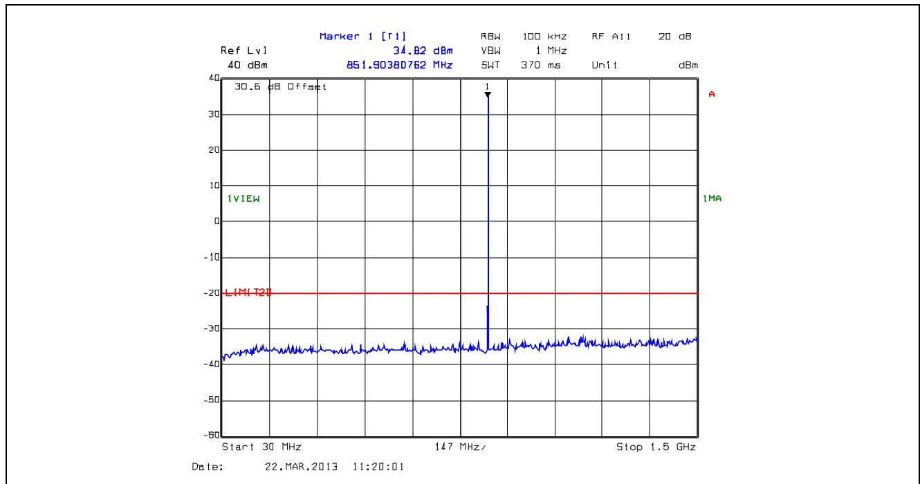
Plot 5.5.4.49. Conducted Transmitter Spurious Emissions, High Power, 851.1 MHz, 30 MHz - 1.5 GHz
