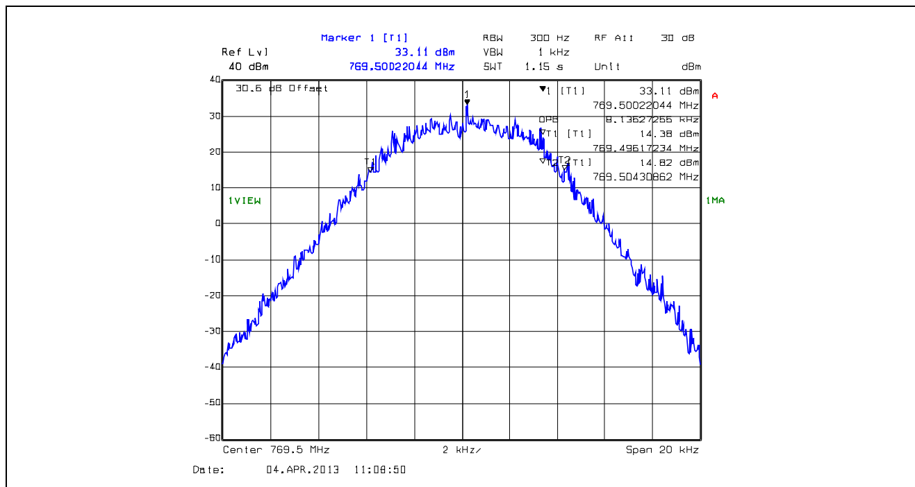
Plot 5.4.4.1.27. 99% Occupied Bandwidth, 12.5 kHz Channel Spacing, F1W, 769.5 MHz
