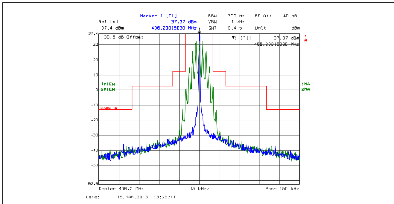
Plot 5.4.4.2.7. Emission Mask B, 25 kHz Channel Spacing, F3E, High Power, 406.2 MHz
