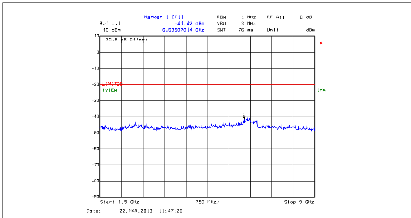
Plot 5.5.4.42. Conducted Transmitter Spurious Emissions, High Power, 815.0 MHz, 1.5 GHz - 9 GHz
