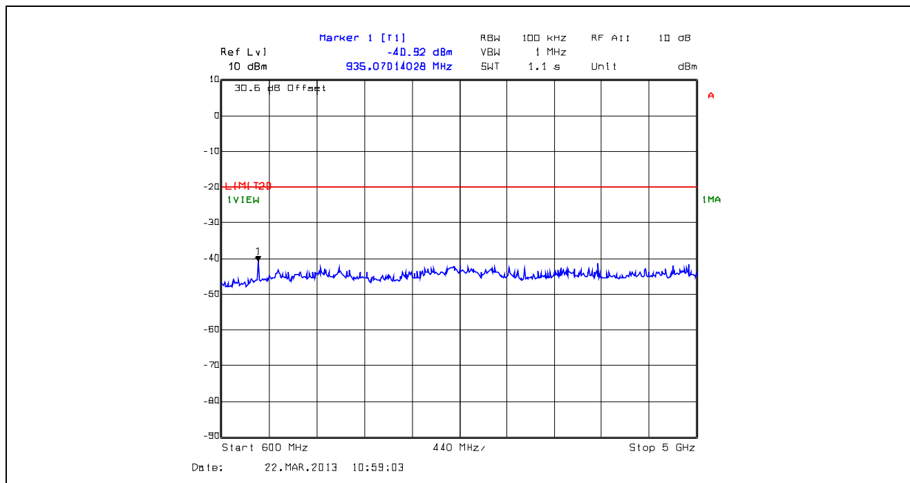
Plot 5.5.4.10. Conducted Transmitter Spurious Emissions, High Power, 469.9 MHz, 600 MHz - 5 GHz
