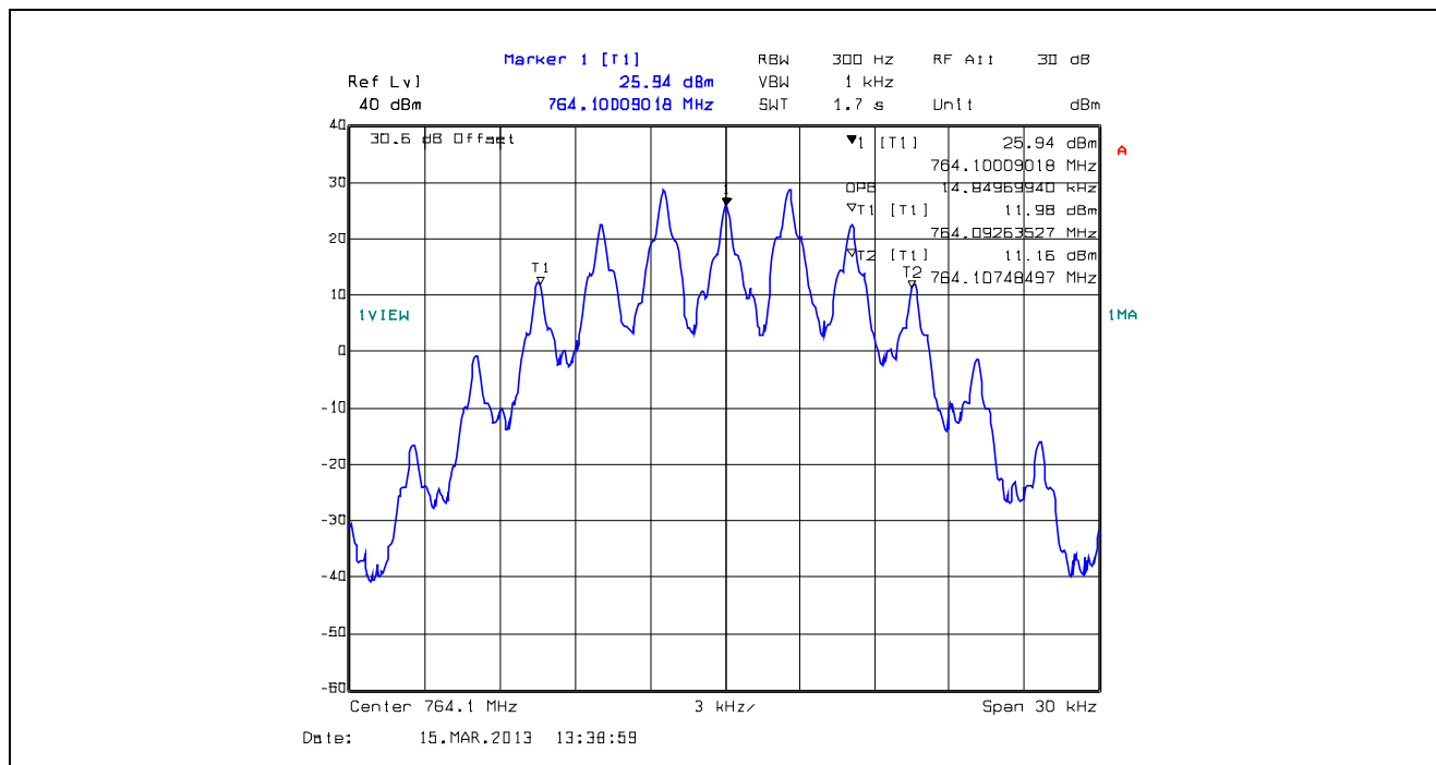
Plot 5.4.4.1.17. 99% Occupied Bandwidth, 25 kHz Channel Spacing, F3E, 764.1 MHz
