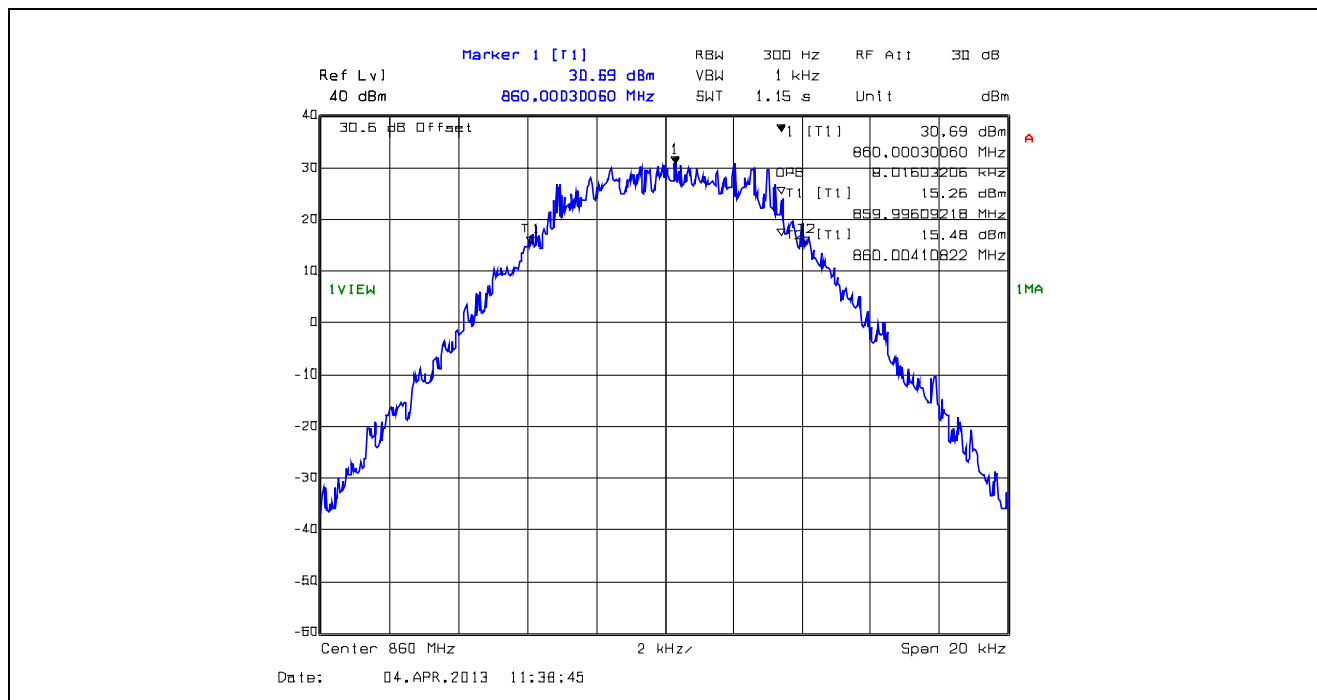
Plot 5.4.4.1.72. 99% Occupied Bandwidth, 12.5 kHz Channel Spacing, F1W, 860.0 MHz
