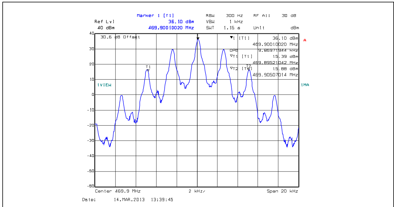
Plot 5.4.4.1.3. 99% Occupied Bandwidth, 12.5 kHz Channel Spacing, F3E, 469.9 MHz
