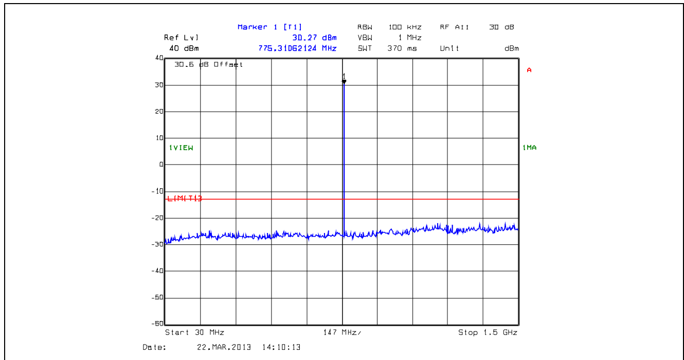
Plot 5.5.4.23. Conducted Transmitter Spurious Emissions, Low Power, 774.9 MHz, 30 MHz - 1.5 GHz
