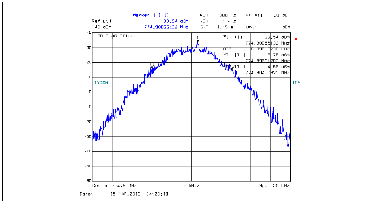
Plot 5.4.4.1.22. 99% Occupied Bandwidth, 12.5 kHz Channel Spacing, F1E, 774.9 MHz
