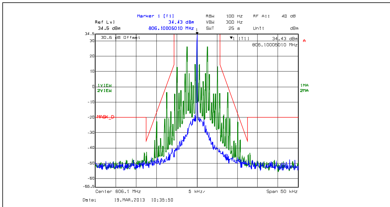
Plot 5.4.4.2.27. Emission Mask D, 12.5 kHz Channel Spacing, F3E, High Power, 806.1 MHz
