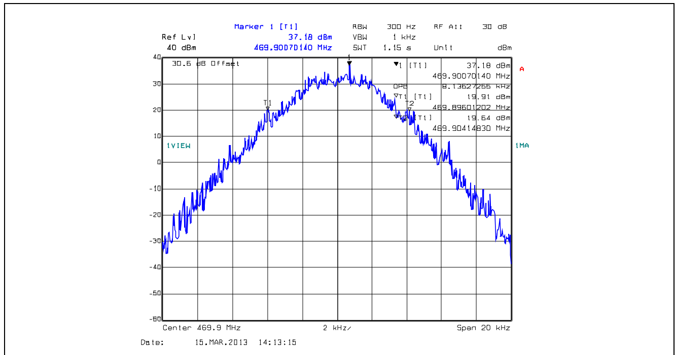
Plot 5.4.4.1.7. 99% Occupied Bandwidth, 12.5 kHz Channel Spacing, F1E, 469.9 MHz
