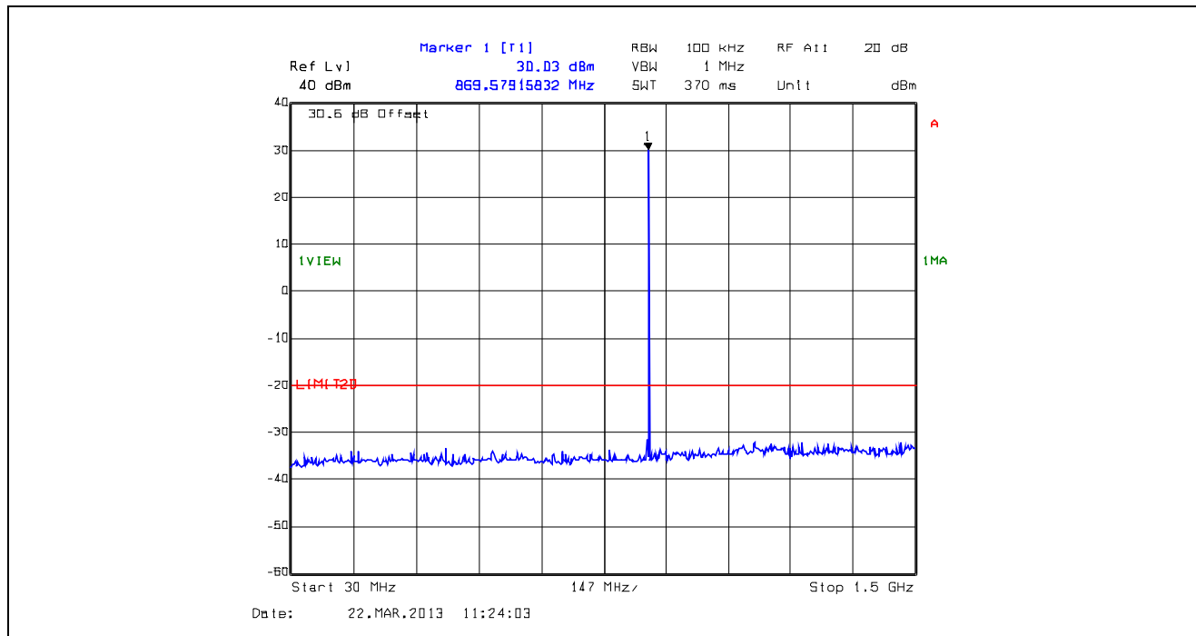
Plot 5.5.4.59. Conducted Transmitter Spurious Emissions, Low Power, 868.9 MHz, 30 MHz - 1.5 GHz
