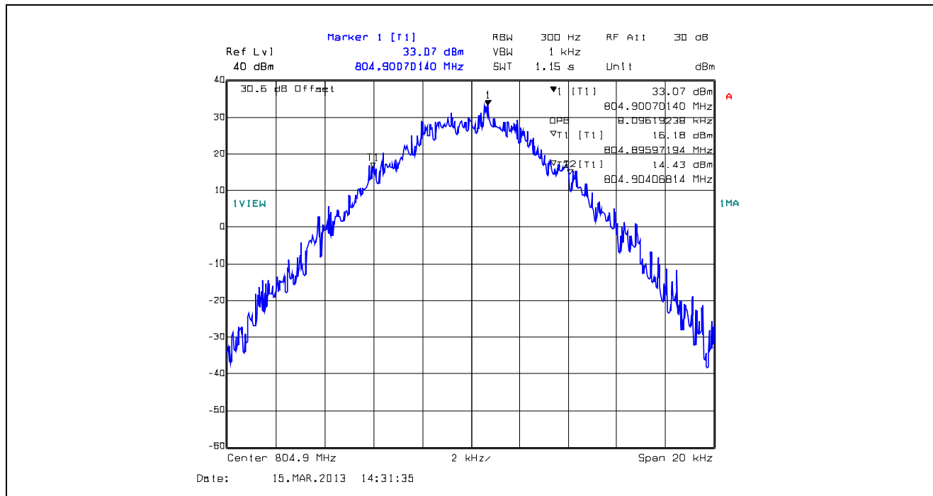
Plot 5.4.4.1.37. 99% Occupied Bandwidth, 12.5 kHz Channel Spacing, F1E, 804.9 MHz
