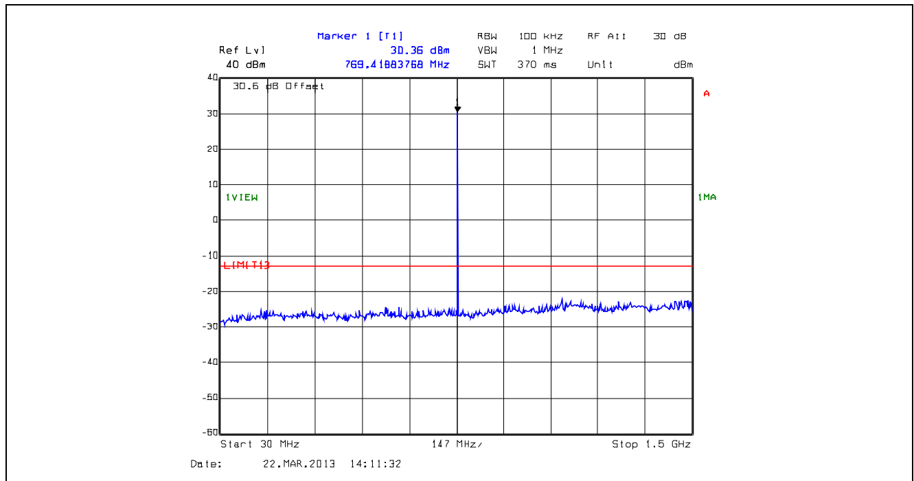
Plot 5.5.4.19. Conducted Transmitter Spurious Emissions, Low Power, 769.5 MHz, 30 MHz - 1.5 GHz
