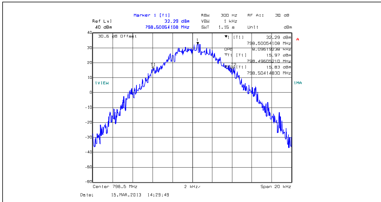
Plot 5.4.4.1.36. 99% Occupied Bandwidth, 12.5 kHz Channel Spacing, F1E, 798.5 MHz
