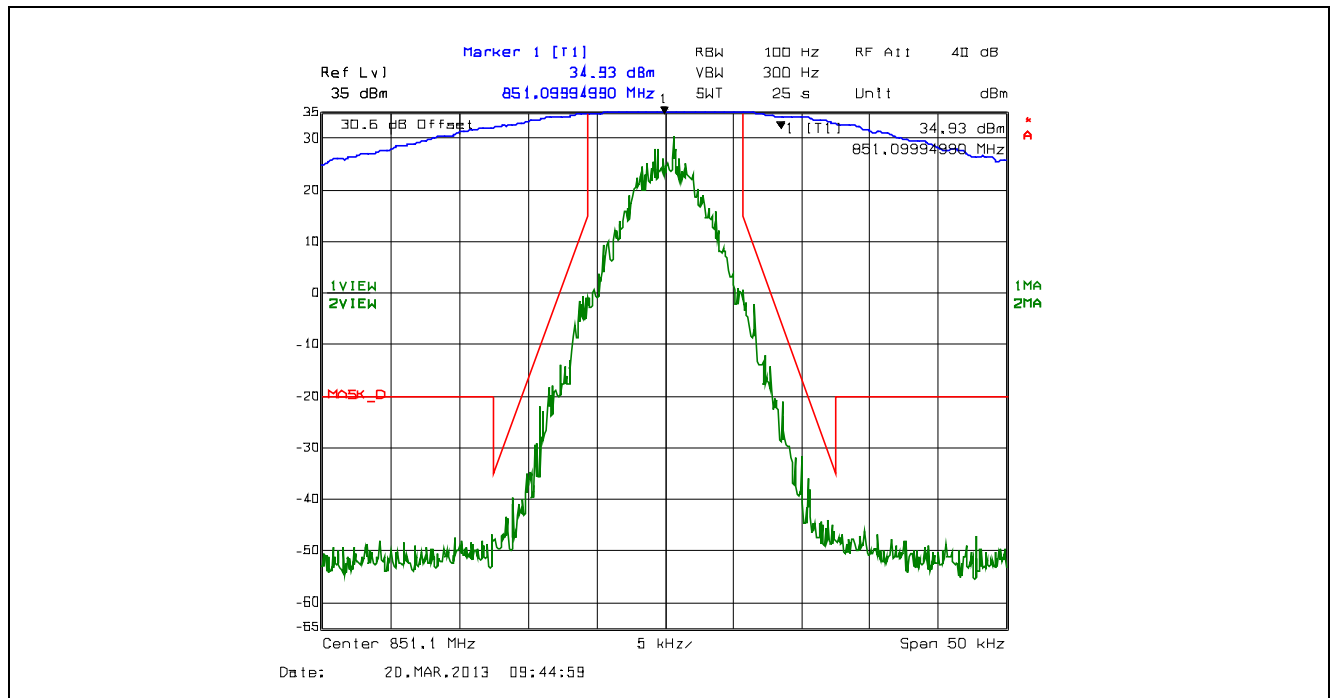
Plot 5.4.4.2.69. Emission Mask D, 12.5 kHz Channel Spacing, F1E, High Power, 851.1 MHz
