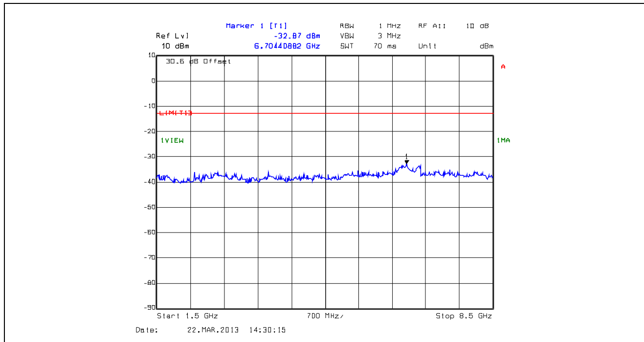
Plot 5.5.4.14. Conducted Transmitter Spurious Emissions, High Power, 764.1 MHz, 1.5 GHz - 8.5 GHz
