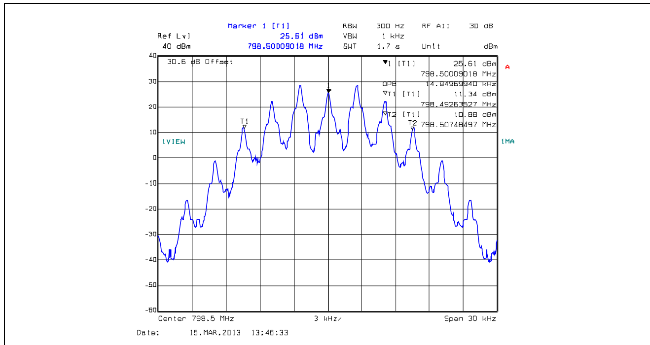
Plot 5.4.4.1.33. 99% Occupied Bandwidth, 25 kHz Channel Spacing, F3E, 798.5 MHz
