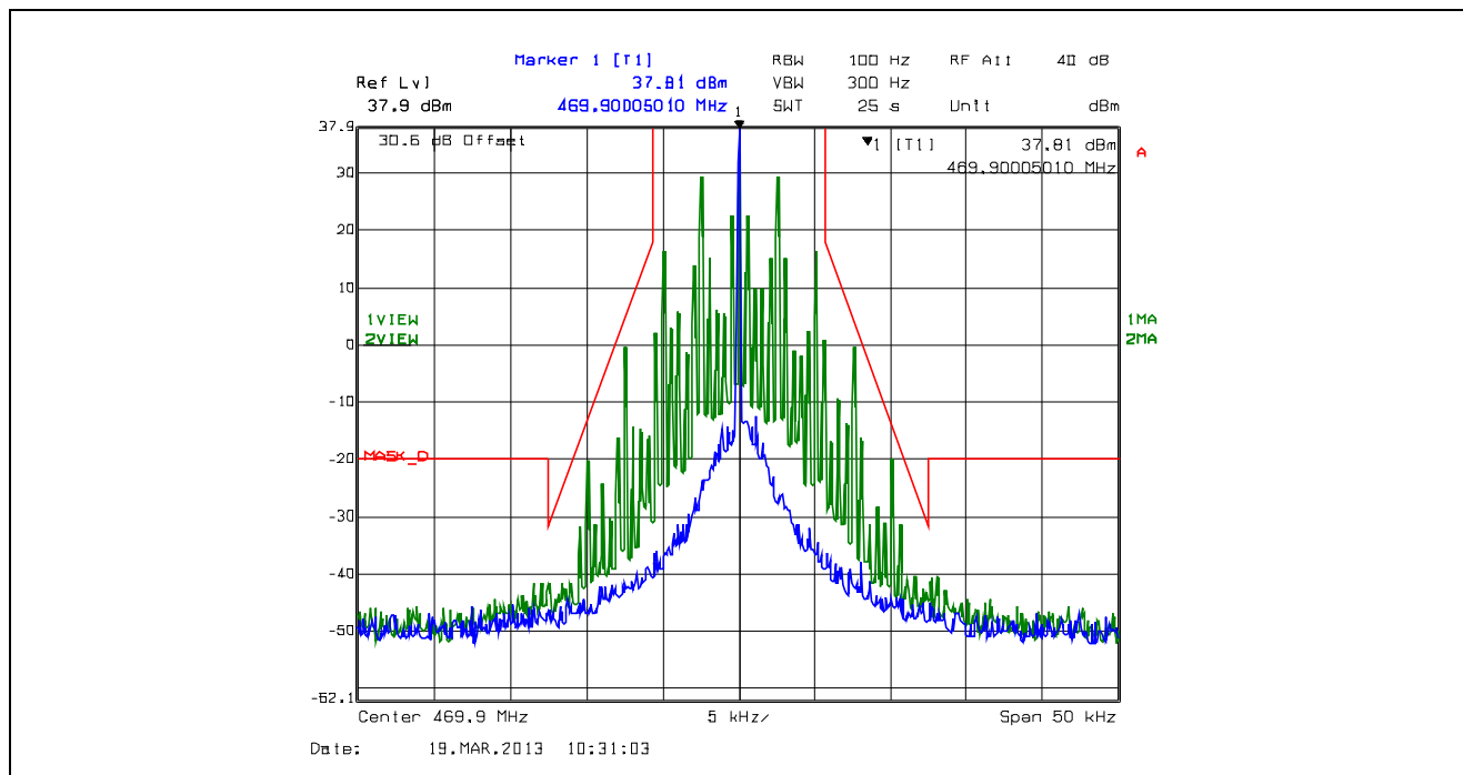
Plot 5.4.4.2.5. Emission Mask D, 12.5 kHz Channel Spacing, F3E, High Power, 469.9 MHz
