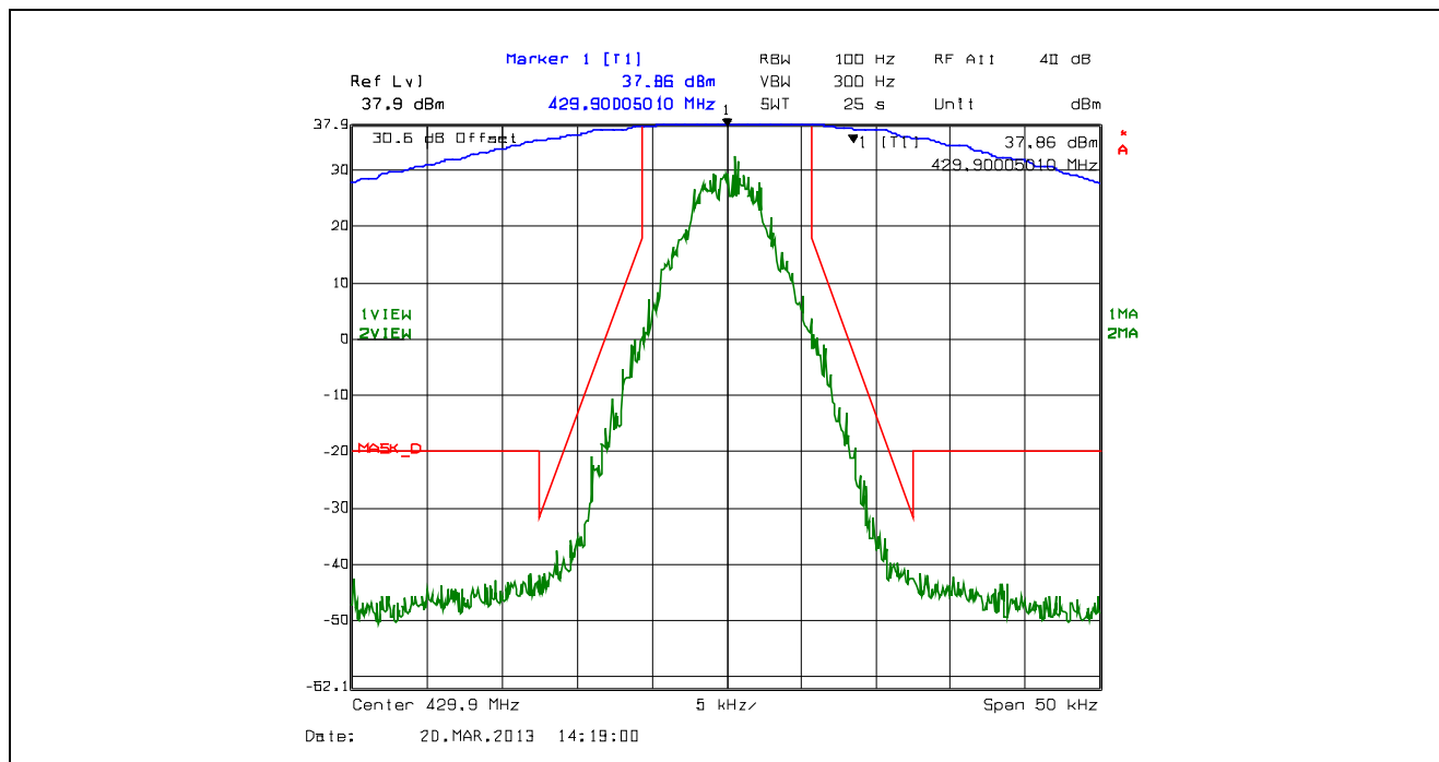
Plot 5.4.4.2.17. Emission Mask D, 12.5 kHz Channel Spacing, F1D, High Power, 429.9 MHz
