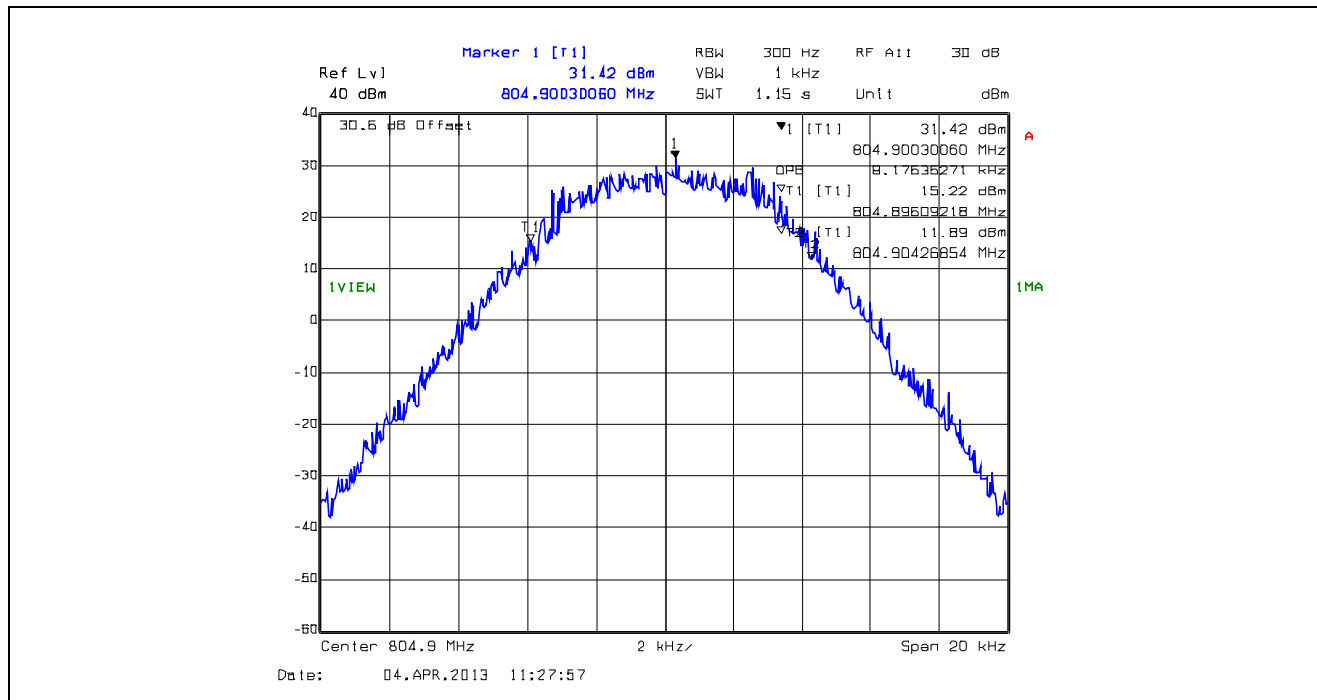
Plot 5.4.4.1.43. 99% Occupied Bandwidth, 12.5 kHz Channel Spacing, F1W, 804.9 MHz
