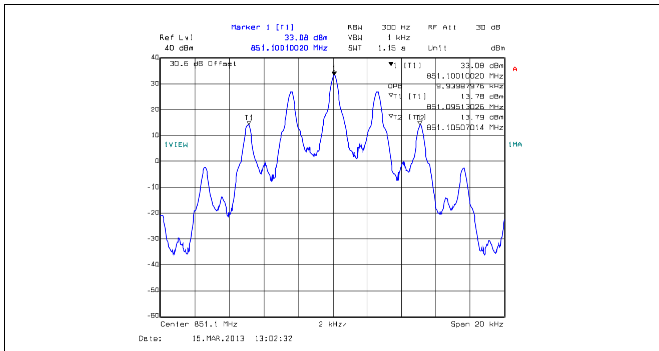
Plot 5.4.4.1.59. 99% Occupied Bandwidth, 12.5 kHz Channel Spacing, F3E, 851.1 MHz
