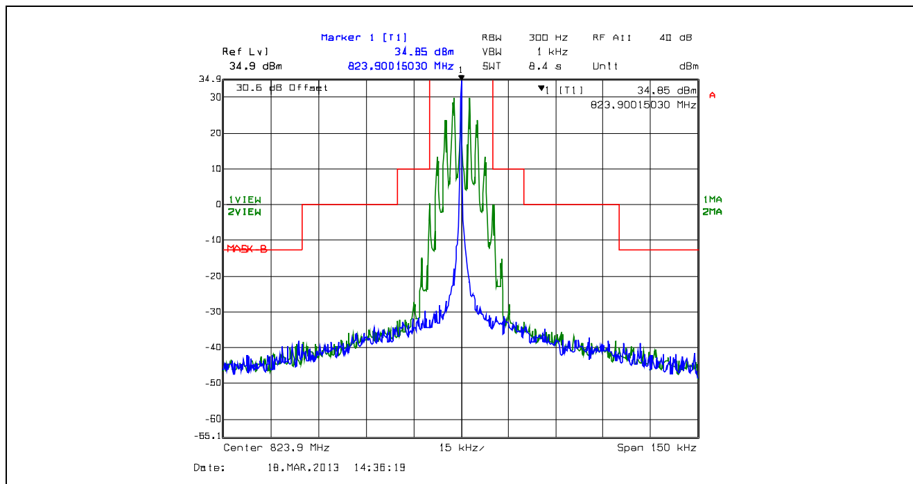
Plot 5.4.4.2.37. Emission Mask B, 25 kHz Channel Spacing, F3E, High Power, 823.9 MHz
