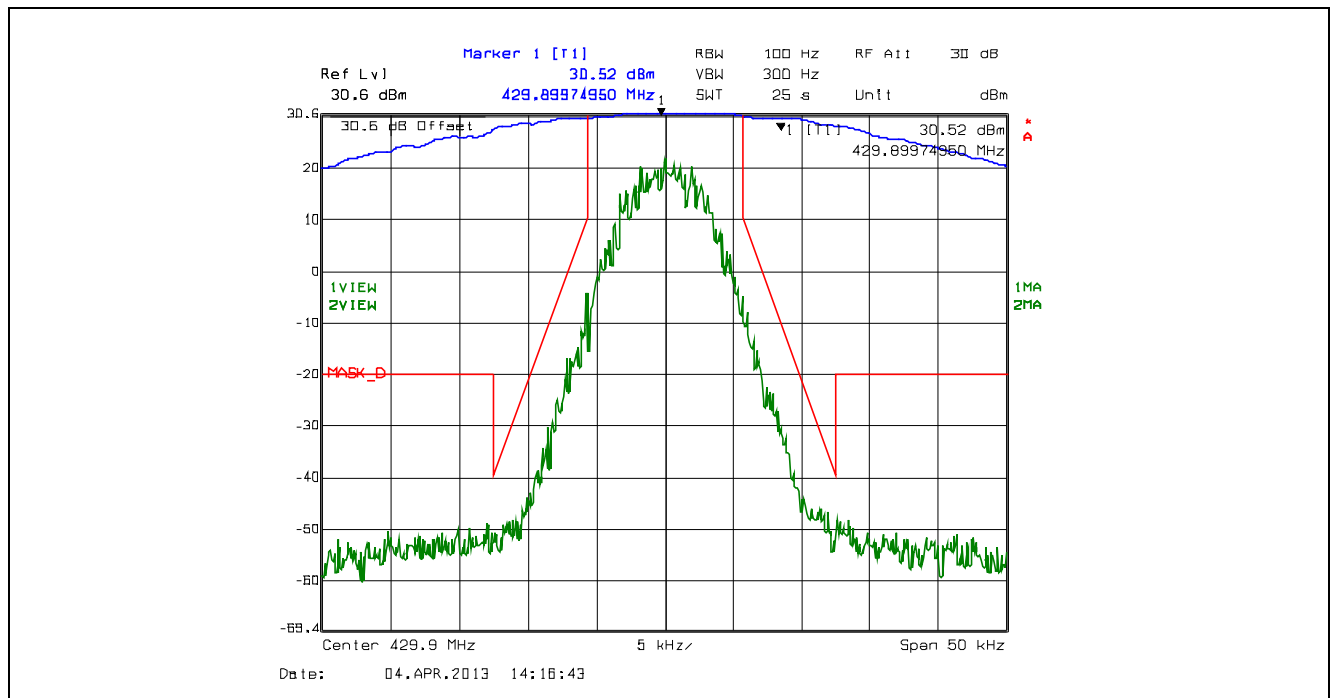
Plot 5.4.4.2.24. Emission Mask D, 12.5 kHz Channel Spacing, F1W, Low Power, 429.9 MHz
