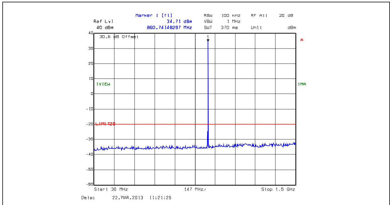
Plot 5.5.4.53. Conducted Transmitter Spurious Emissions, High Power, 860.0 MHz, 30 MHz - 1.5 GHz
