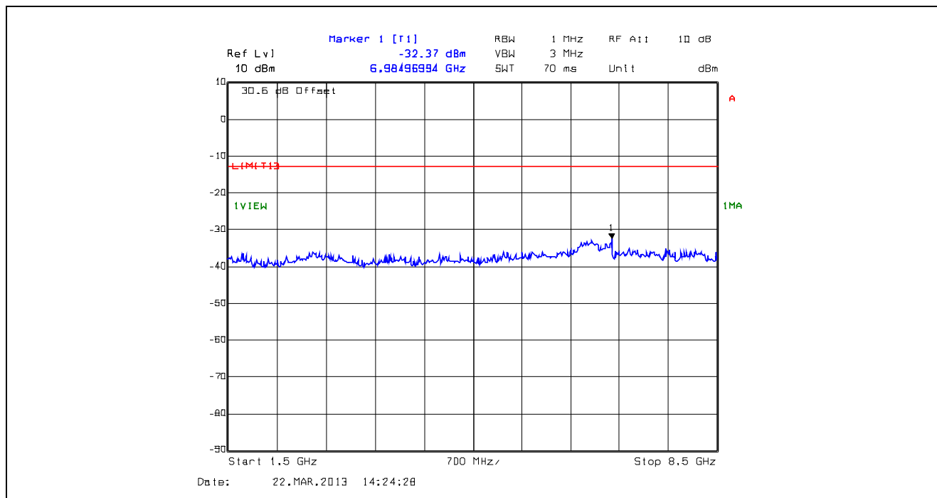
Plot 5.5.4.34. Conducted Transmitter Spurious Emissions, High Power, 804.9 MHz, 1.5 GHz - 8.5 GHz
