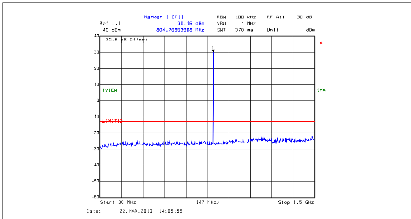
Plot 5.5.4.35. Conducted Transmitter Spurious Emissions, Low Power, 804.9 MHz, 30 MHz - 1.5 GHz
