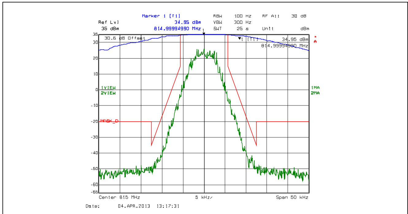
Plot 5.4.4.2.53. Emission Mask D, 12.5 kHz Channel Spacing, F1W, High Power, 815.0 MHz
