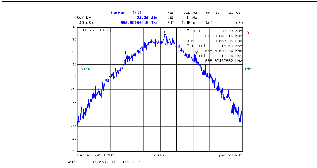
Plot 5.4.4.1.67. 99% Occupied Bandwidth, 12.5 kHz Channel Spacing, F1E, 868.9 MHz
