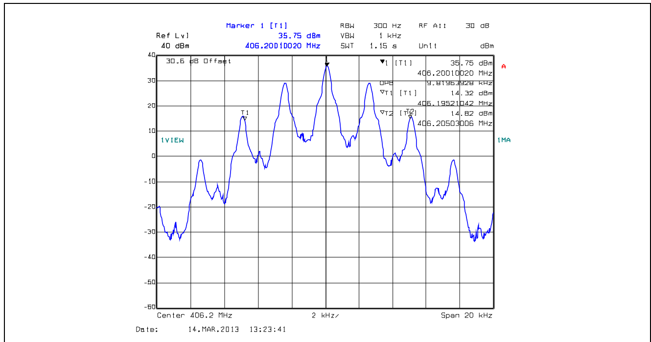
Plot 5.4.4.1.1. 99% Occupied Bandwidth, 12.5 kHz Channel Spacing, F3E, 406.2 MHz
