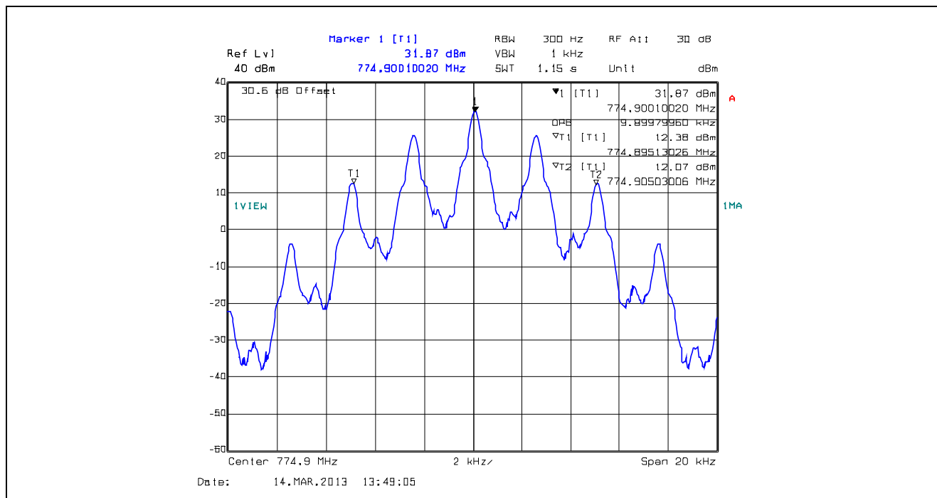
Plot 5.4.4.1.16. 99% Occupied Bandwidth, 12.5 kHz Channel Spacing, F3E, 774.9 MHz
