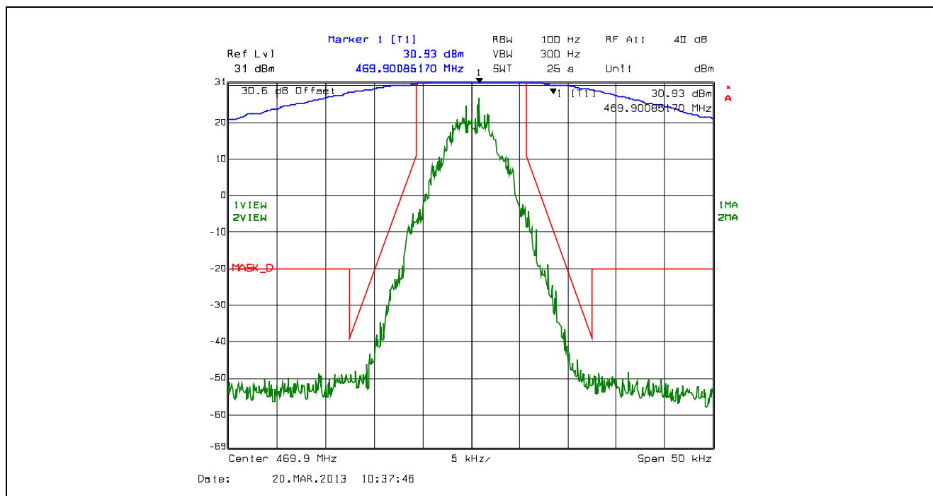
Plot 5.4.4.2.20. Emission Mask D, 12.5 kHz Channel Spacing, F1D, Low Power, 469.9 MHz
