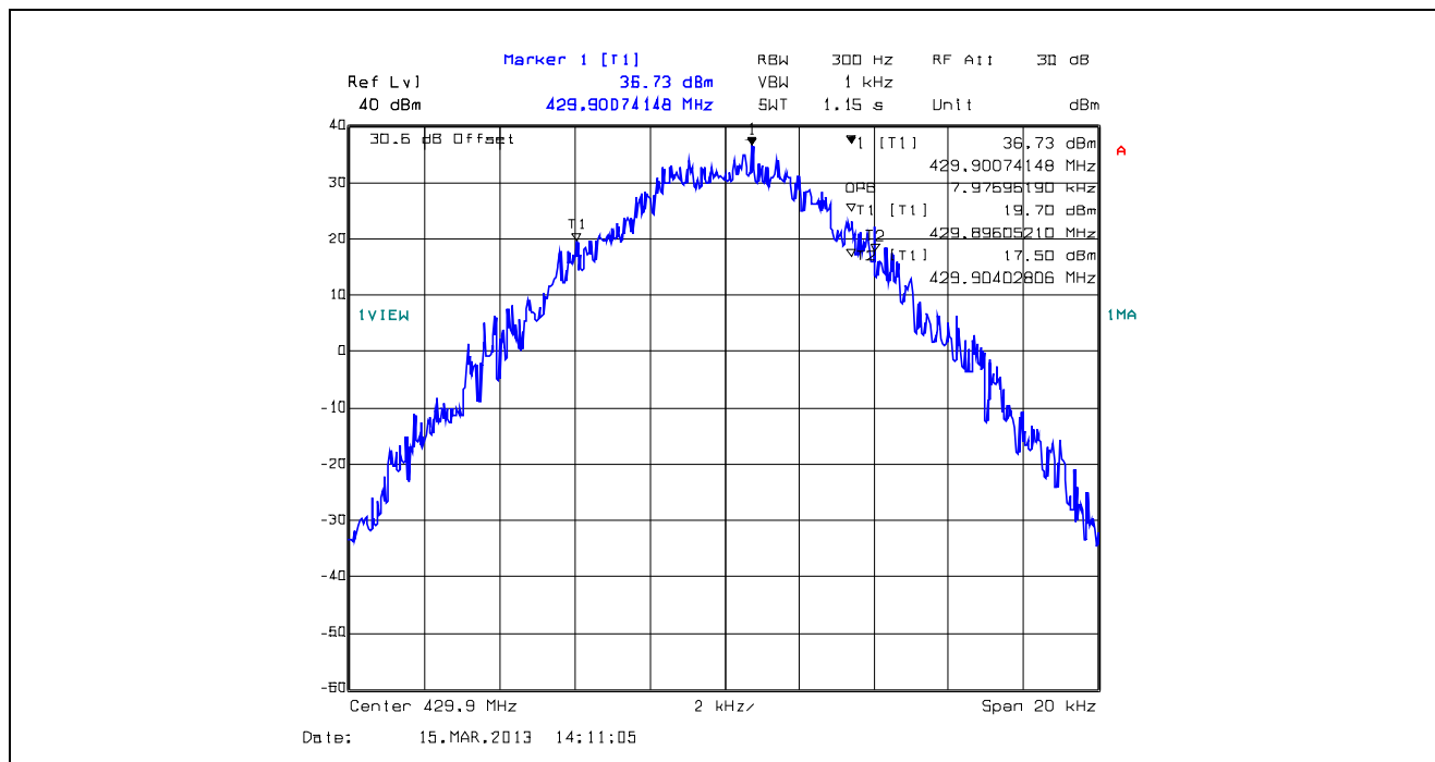
Plot 5.4.4.1.6. 99% Occupied Bandwidth, 12.5 kHz Channel Spacing, F1E, 429.9 MHz
