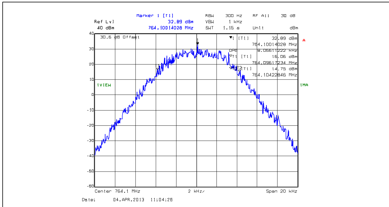
Plot 5.4.4.1.26. 99% Occupied Bandwidth, 12.5 kHz Channel Spacing, F1W, 764.1 MHz
