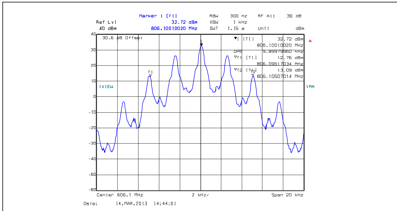
Plot 5.4.4.1.44. 99% Occupied Bandwidth, 12.5 kHz Channel Spacing, F3E, 806.1 MHz
