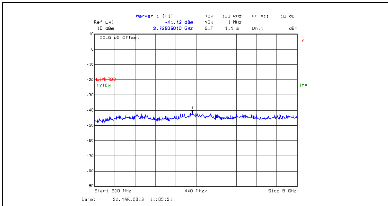
Plot 5.5.4.12. Conducted Transmitter Spurious Emissions, Low Power, 469.9 MHz, 600 MHz - 5 GHz
