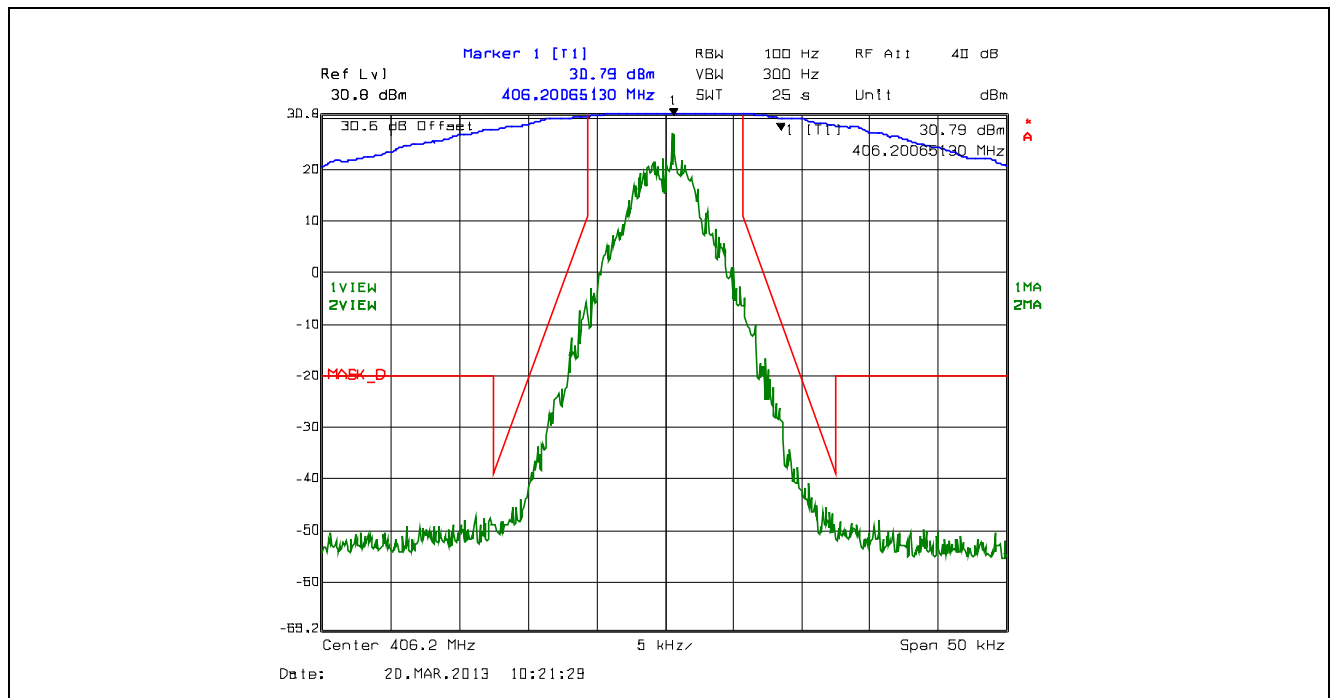
Plot 5.4.4.2.10. Emission Mask D, 12.5 kHz Channel Spacing, F1E, Low Power, 406.2 MHz
