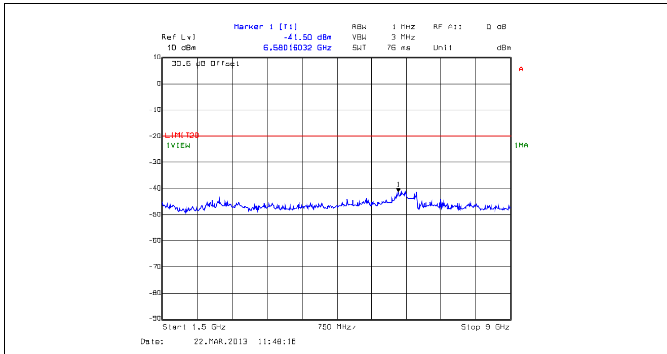
Plot 5.5.4.38. Conducted Transmitter Spurious Emissions, High Power, 806.1 MHz, 1.5 GHz - 9 GHz
