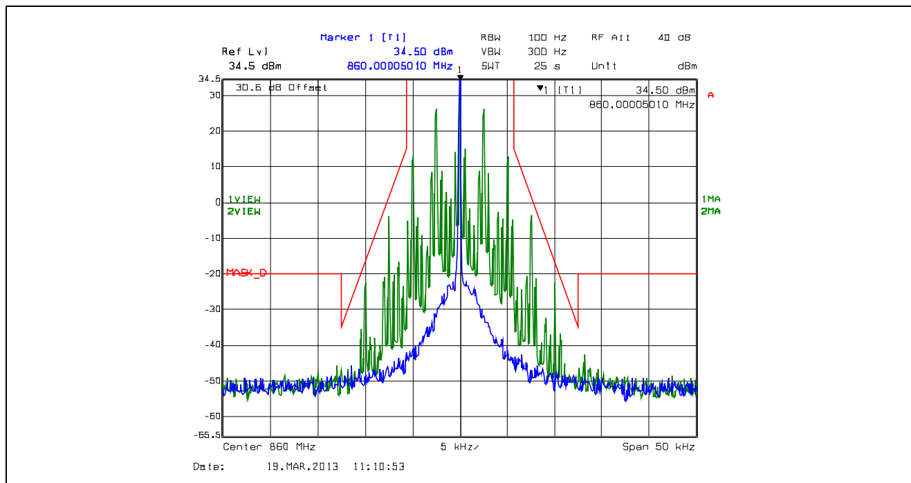
Plot 5.4.4.2.59. Emission Mask D, 12.5 kHz Channel Spacing, F3E, High Power, 860.0 MHz
