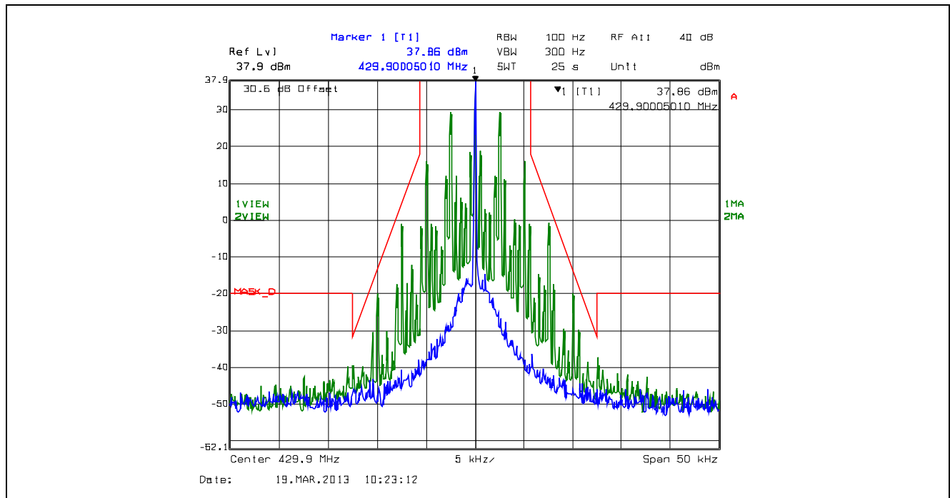
Plot 5.4.4.2.3. Emission Mask D, 12.5 kHz Channel Spacing, F3E, High Power, 429.9 MHz
