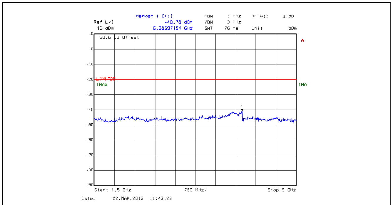
Plot 5.5.4.54. Conducted Transmitter Spurious Emissions, High Power, 860.0 MHz, 1.5 GHz - 9 GHz
