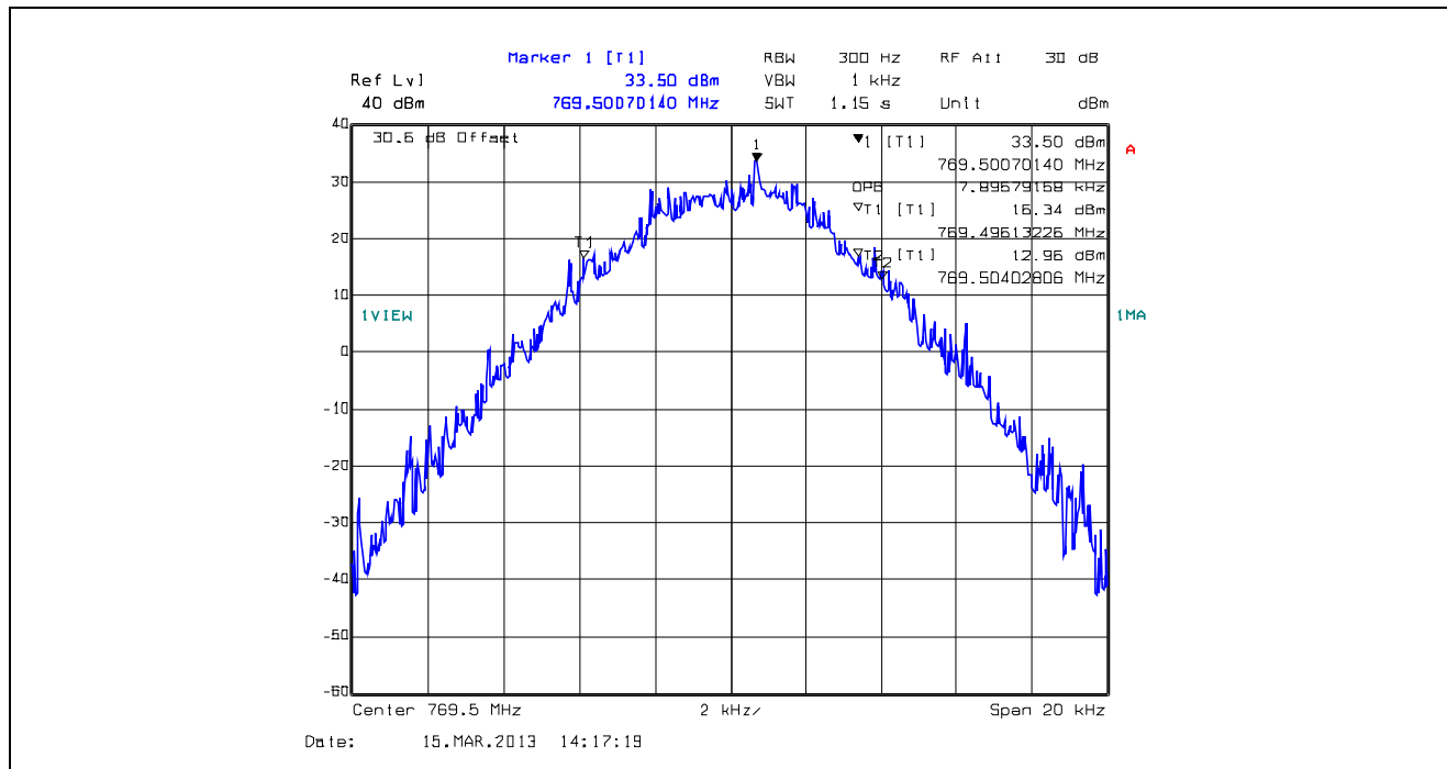
Plot 5.4.4.1.21. 99% Occupied Bandwidth, 12.5 kHz Channel Spacing, F1E, 769.5 MHz
