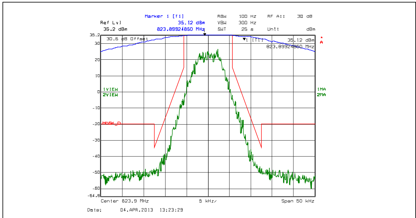
Plot 5.4.4.2.55. Emission Mask D, 12.5 kHz Channel Spacing, F1W, High Power, 823.9 MHz
