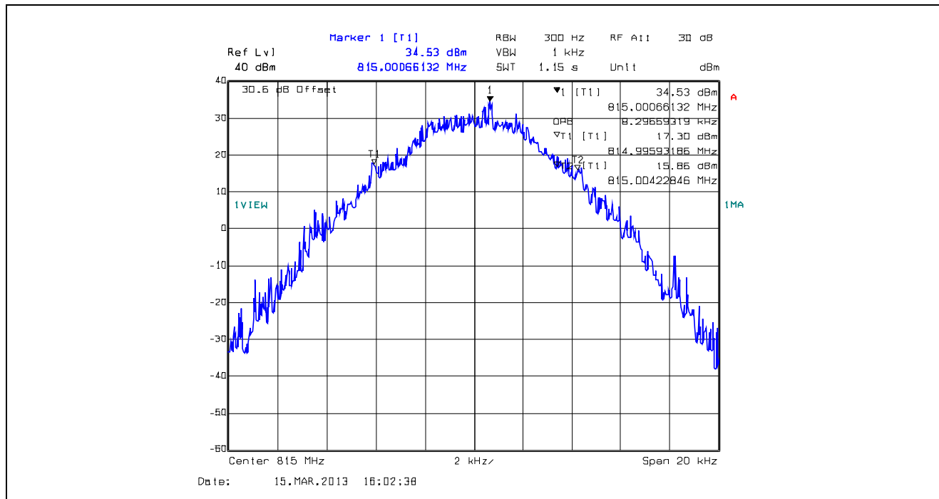
Plot 5.4.4.1.54. 99% Occupied Bandwidth, 12.5 kHz Channel Spacing, F1D, 815.0 MHz
