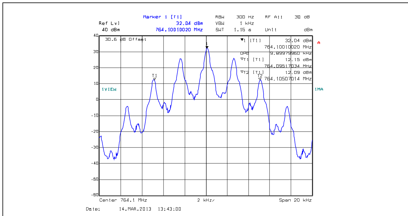
Plot 5.4.4.1.14. 99% Occupied Bandwidth, 12.5 kHz Channel Spacing, F3E, 764.1 MHz
