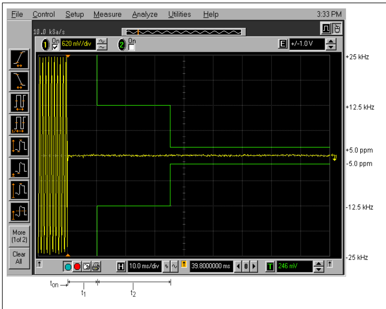
Plot 5.8.4.3. Transient Frequency Behavior on 25 kHz Channels Test Frequency: 406.2 MHz; Power: 5 W; Test Conditions: Switch on condition t_{on} , t_1 , and t_2
