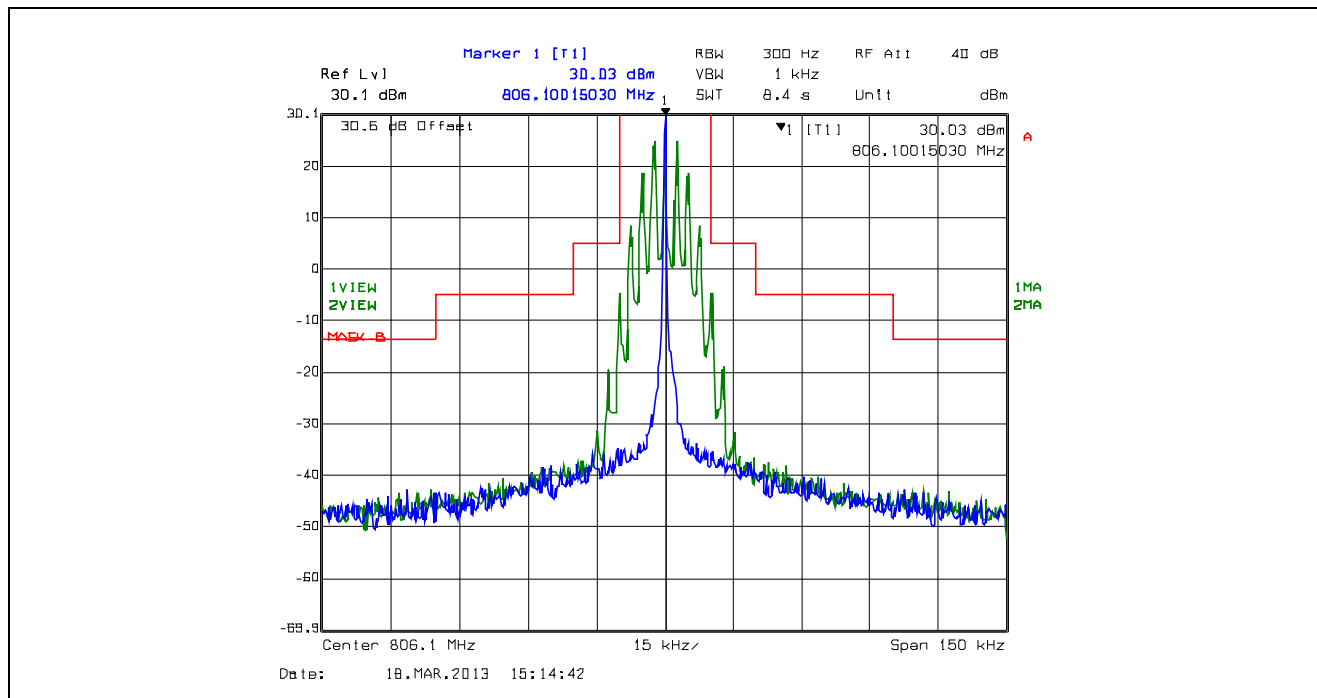
Plot 5.4.4.2.34. Emission Mask B, 25 kHz Channel Spacing, F3E, Low Power, 806.1 MHz
