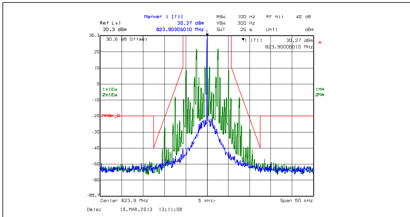
Plot 5.4.4.2.32. Emission Mask D, 12.5 kHz Channel Spacing, F3E, Low Power, 823.9 MHz
