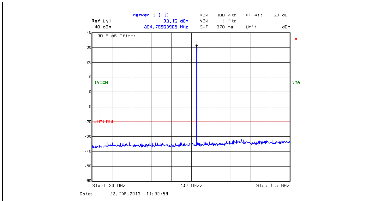
Plot 5.5.4.39. Conducted Transmitter Spurious Emissions, Low Power, 806.1 MHz, 30 MHz - 1.5 GHz
