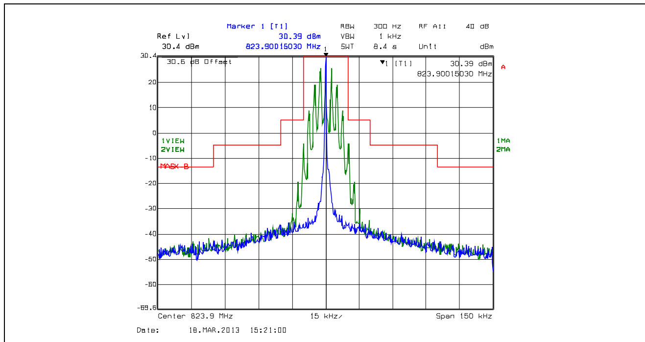
Plot 5.4.4.2.38. Emission Mask B, 25 kHz Channel Spacing, F3E, Low Power, 823.9 MHz
