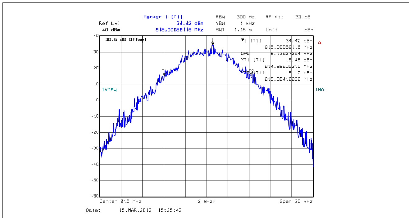
Plot 5.4.4.1.51. 99% Occupied Bandwidth, 12.5 kHz Channel Spacing, F1E, 815.0 MHz
