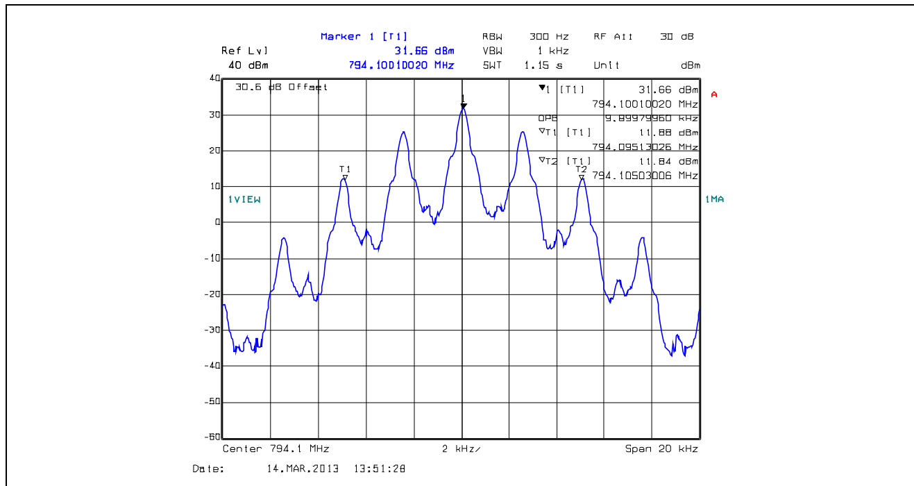
Plot 5.4.4.1.29. 99% Occupied Bandwidth, 12.5 kHz Channel Spacing, F3E, 794.1 MHz
