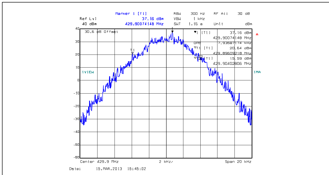
Plot 5.4.4.1.9. 99% Occupied Bandwidth, 12.5 kHz Channel Spacing, F1D, 429.9 MHz
