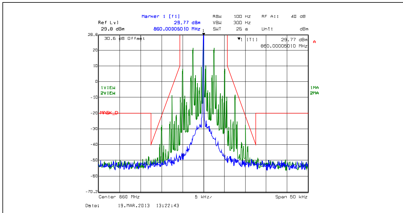
Plot 5.4.4.2.60. Emission Mask D, 12.5 kHz Channel Spacing, F3E, Low Power, 860.0 MHz
