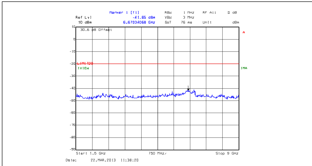
Plot 5.5.4.52. Conducted Transmitter Spurious Emissions, Low Power, 851.1 MHz, 1.5 GHz - 9 GHz
