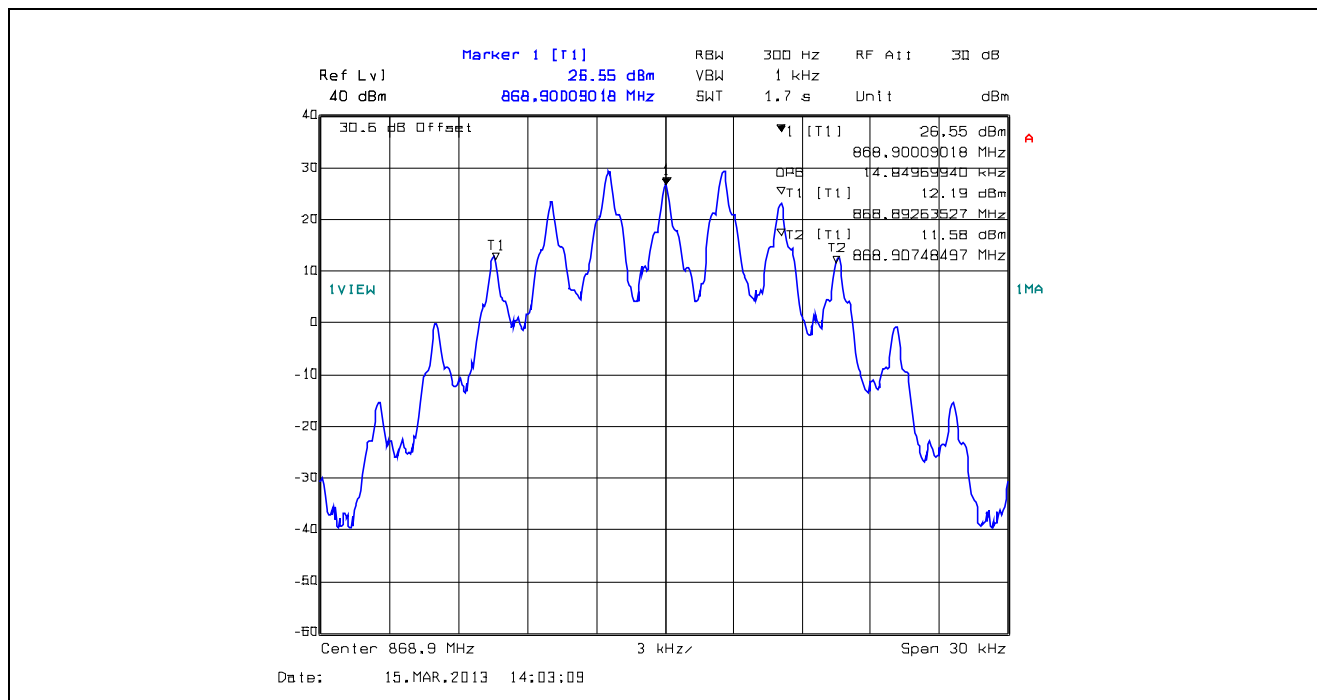
Plot 5.4.4.1.64. 99% Occupied Bandwidth, 25 kHz Channel Spacing, F3E, 868.9 MHz
