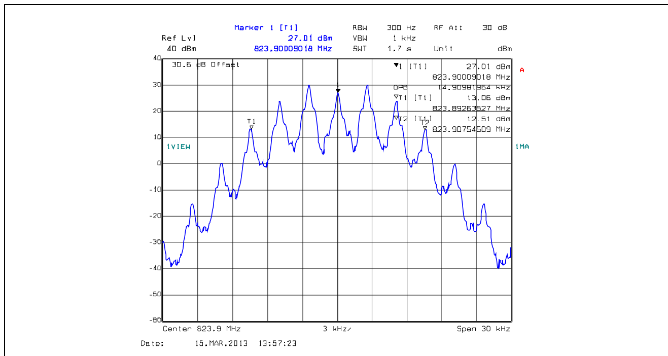
Plot 5.4.4.1.49. 99% Occupied Bandwidth, 25 kHz Channel Spacing, F3E, 823.9 MHz
