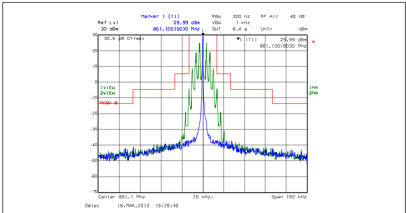
Plot 5.4.4.2.64. Emission Mask B, 25 kHz Channel Spacing, F3E, Low Power, 851.1 MHz
