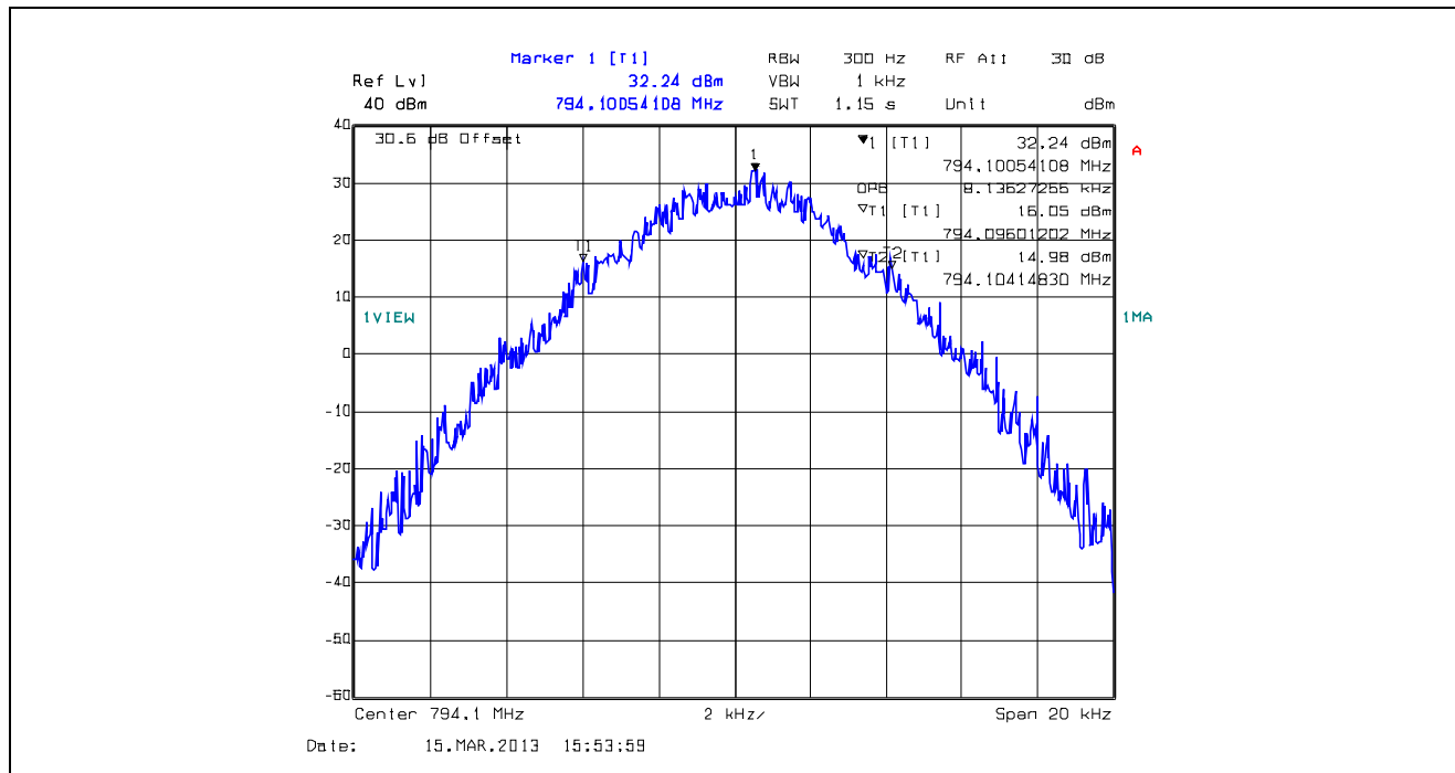
Plot 5.4.4.1.38. 99% Occupied Bandwidth, 12.5 kHz Channel Spacing, F1D, 794.1 MHz
