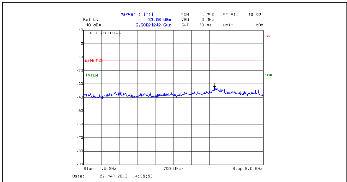
Plot 5.5.4.26. Conducted Transmitter Spurious Emissions, High Power, 794.1 MHz, 1.5 GHz - 8.5 GHz
