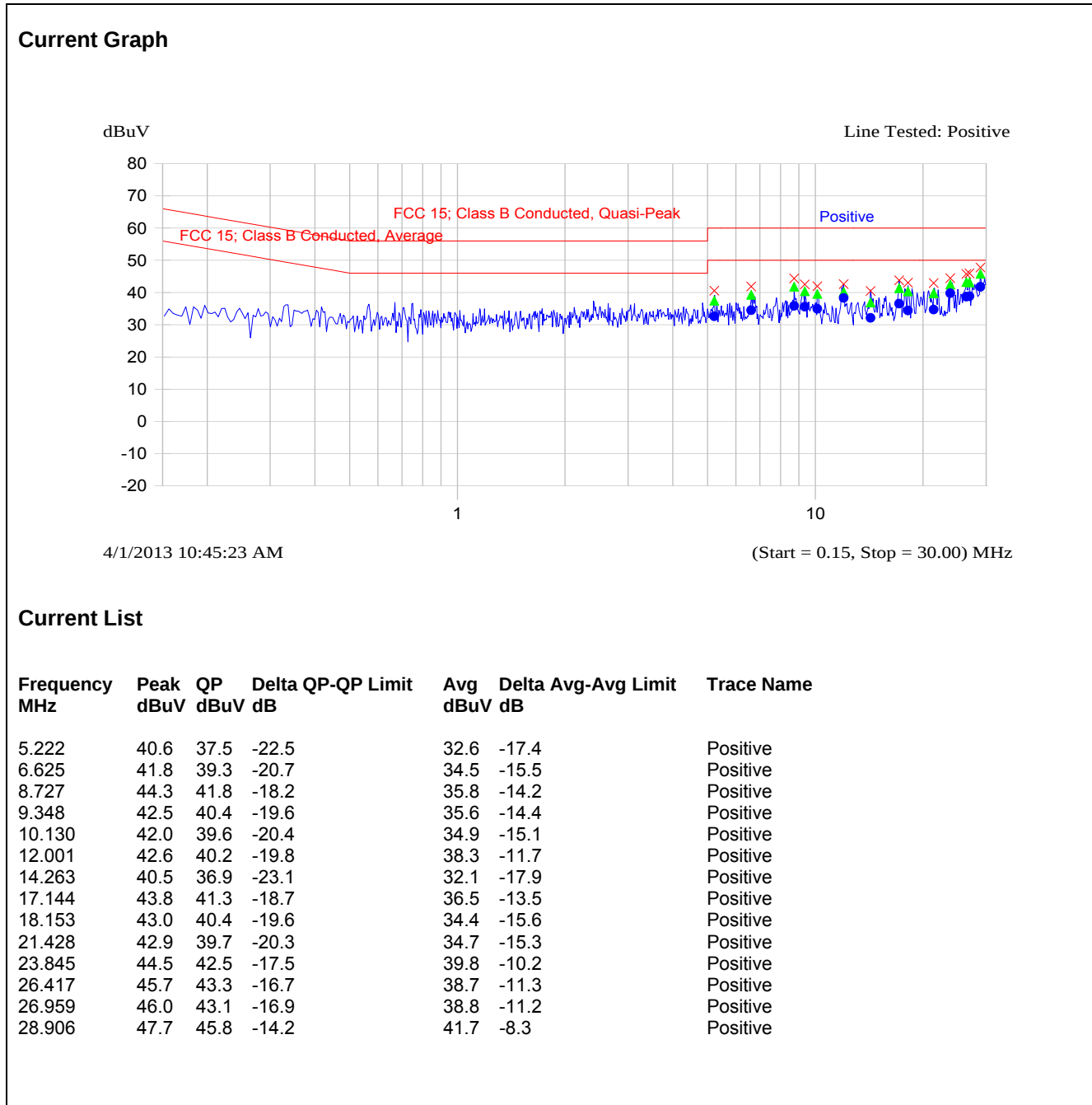
Plot 5.11.3.1. Power Line Conducted Emissions (Tx Mode) Line Voltage: 7.5 VDC; Line Tested: Positive
