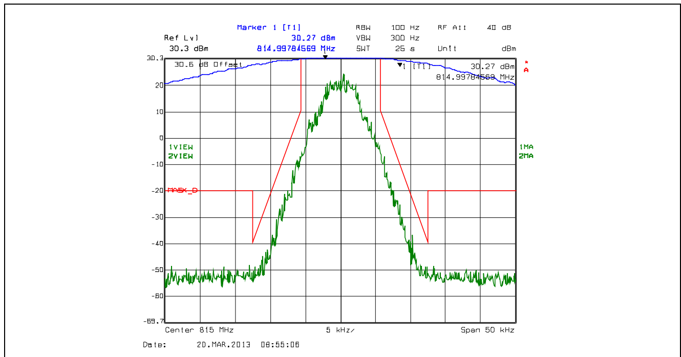
Plot 5.4.4.2.42. Emission Mask D, 12.5 kHz Channel Spacing, F1E, Low Power, 815.0 MHz
