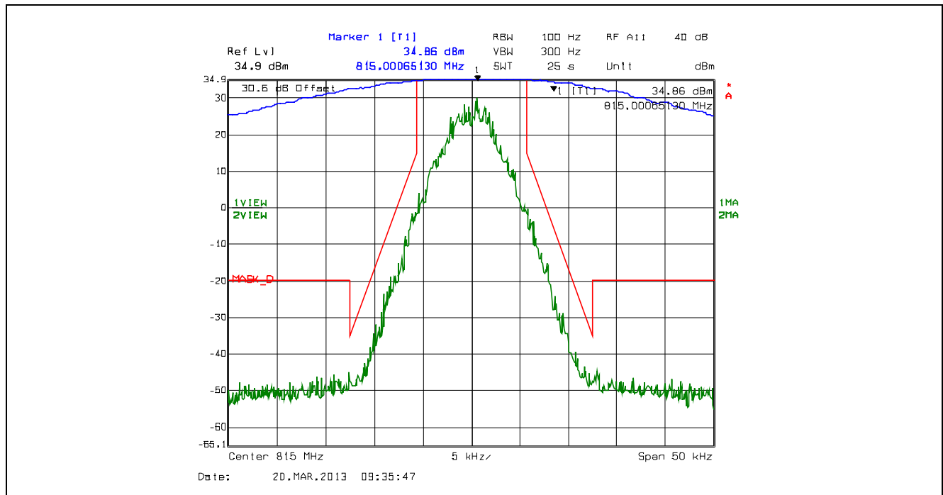
Plot 5.4.4.2.41. Emission Mask D, 12.5 kHz Channel Spacing, F1E, High Power, 815.0 MHz
