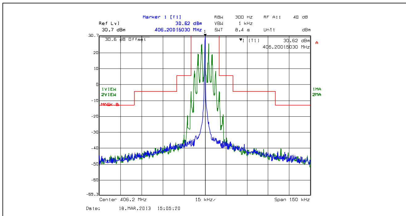
Plot 5.4.4.2.8. Emission Mask B, 25 kHz Channel Spacing, F3E, Low Power, 406.2 MHz
