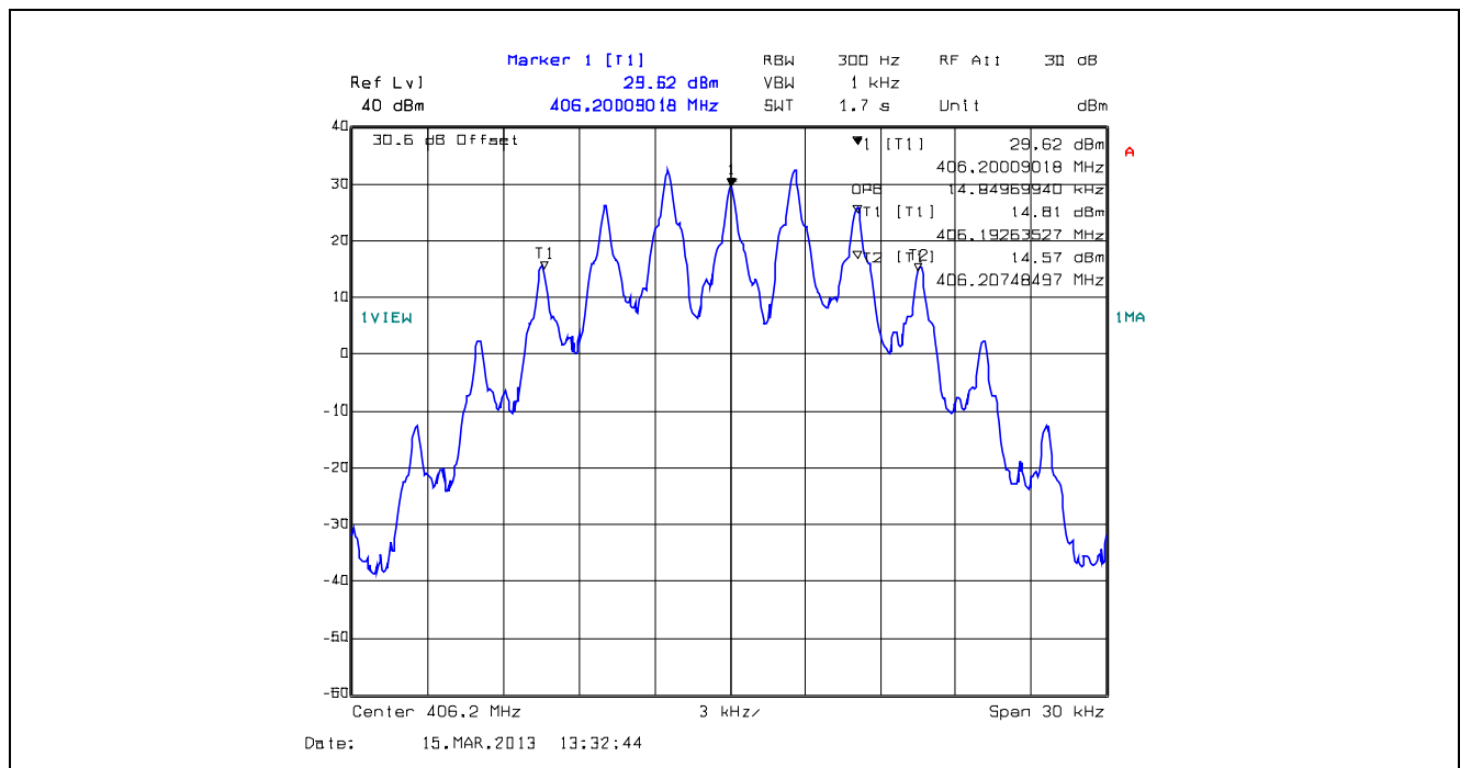
Plot 5.4.4.1.4. 99% Occupied Bandwidth, 25 kHz Channel Spacing, F3E, 406.2 MHz
