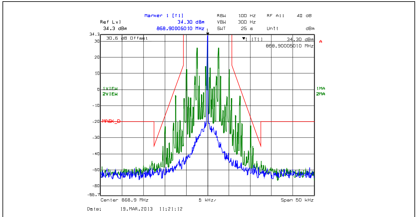
Plot 5.4.4.2.61. Emission Mask D, 12.5 kHz Channel Spacing, F3E, High Power, 868.9 MHz
