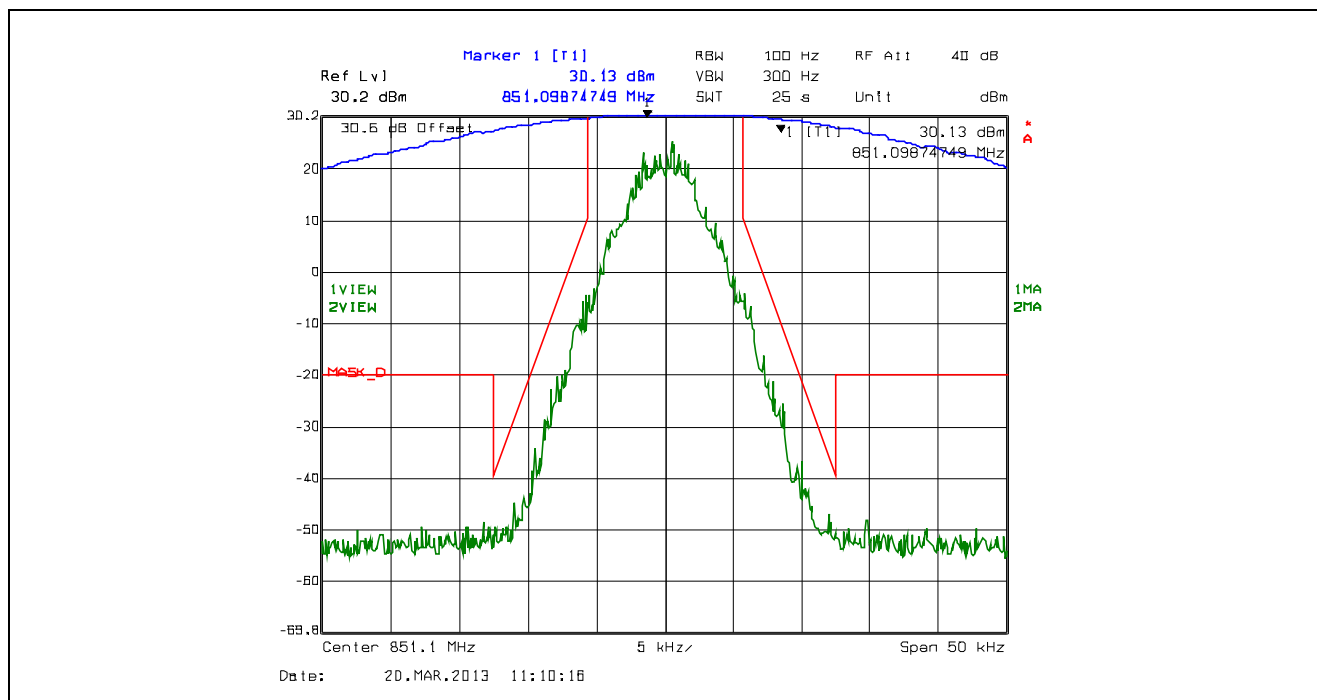
Plot 5.4.4.2.76. Emission Mask D, 12.5 kHz Channel Spacing, F1D, Low Power, 851.1 MHz
