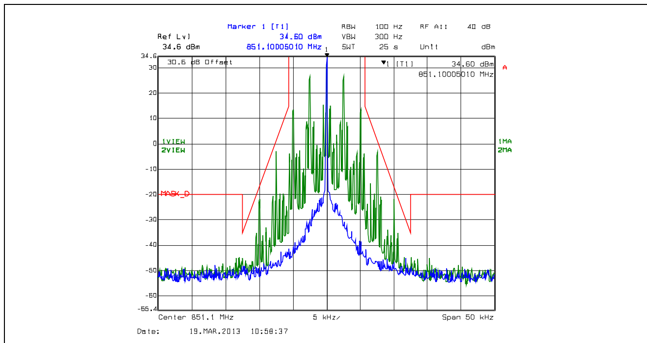
Plot 5.4.4.2.57. Emission Mask D, 12.5 kHz Channel Spacing, F3E, High Power, 851.1 MHz
