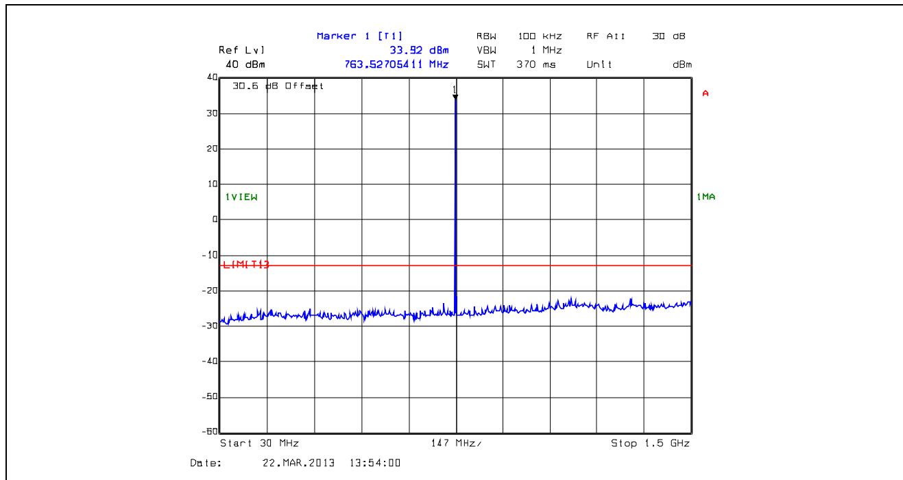
Plot 5.5.4.13. Conducted Transmitter Spurious Emissions, High Power, 764.1 MHz, 30 MHz - 1.5 GHz
