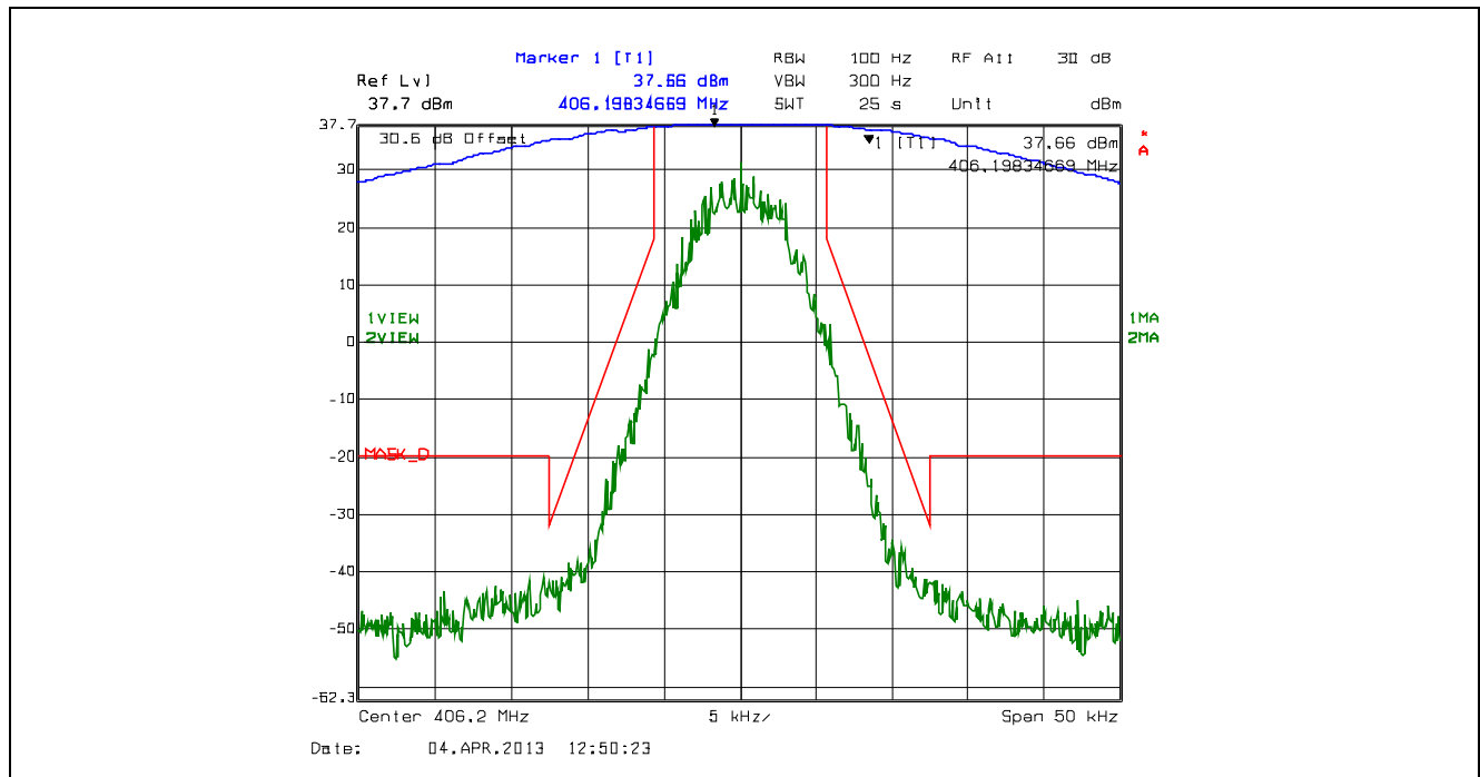
Plot 5.4.4.2.21. Emission Mask D, 12.5 kHz Channel Spacing, F1W, High Power, 406.2 MHz
