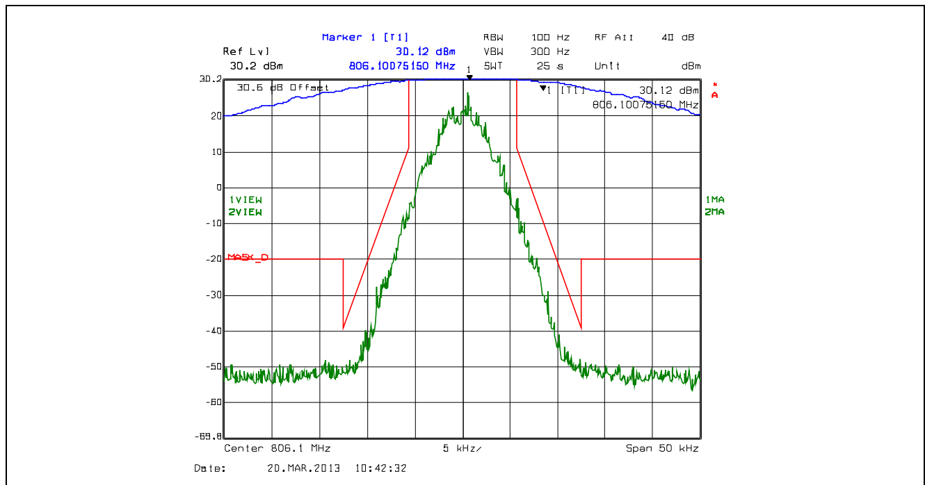
Plot 5.4.4.2.46. Emission Mask D, 12.5 kHz Channel Spacing, F1D, Low Power, 806.1 MHz
