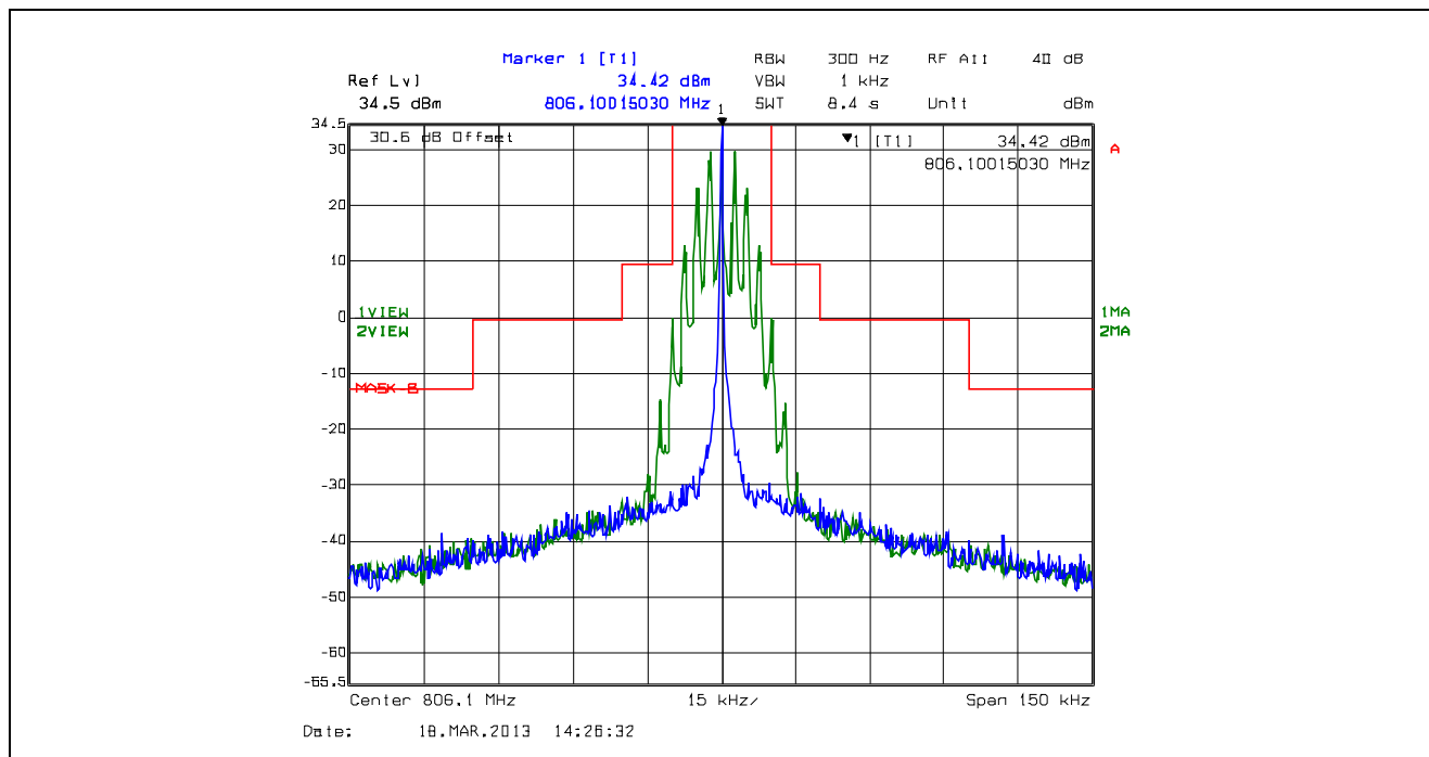
Plot 5.4.4.2.33. Emission Mask B, 25 kHz Channel Spacing, F3E, High Power, 806.1 MHz
