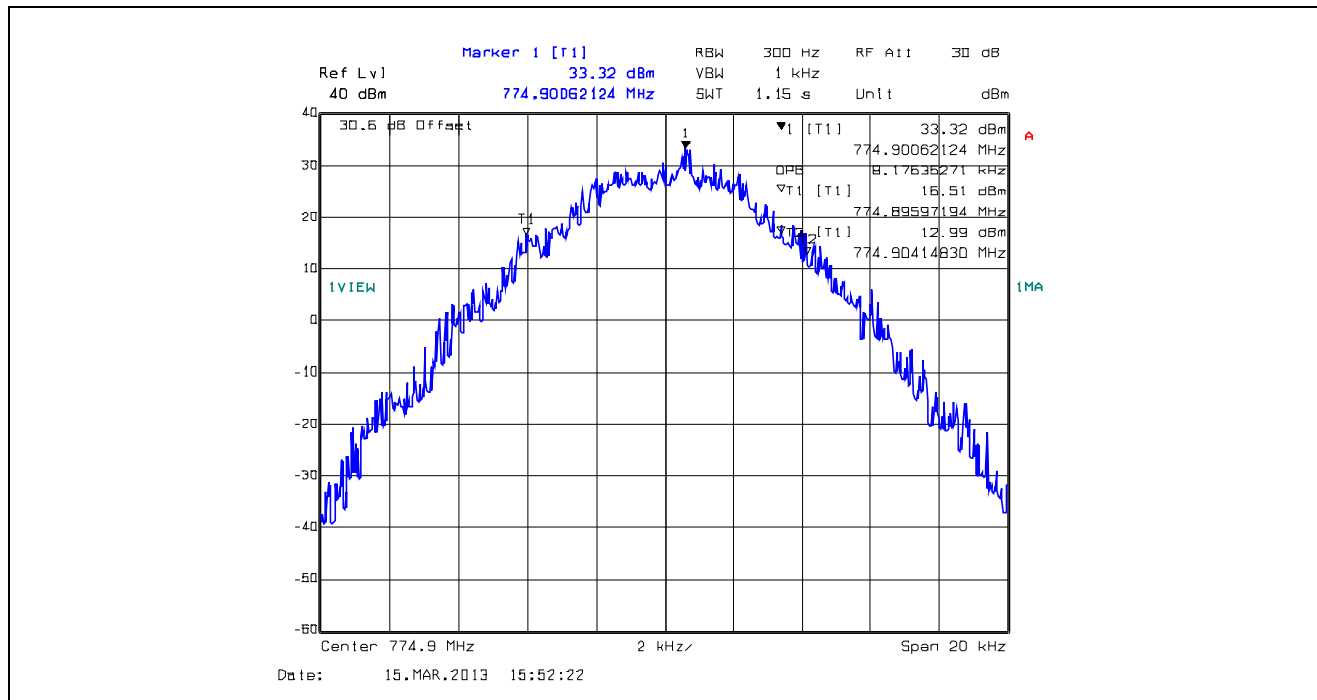
Plot 5.4.4.1.25. 99% Occupied Bandwidth, 12.5 kHz Channel Spacing, F1D, 774.9 MHz
