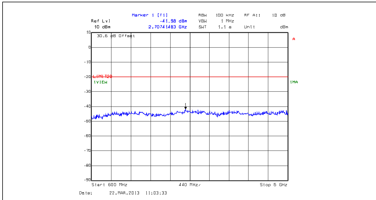
Plot 5.5.4.4. Conducted Transmitter Spurious Emissions, Low Power, 406.2 MHz, 600 MHz -5 GHz
