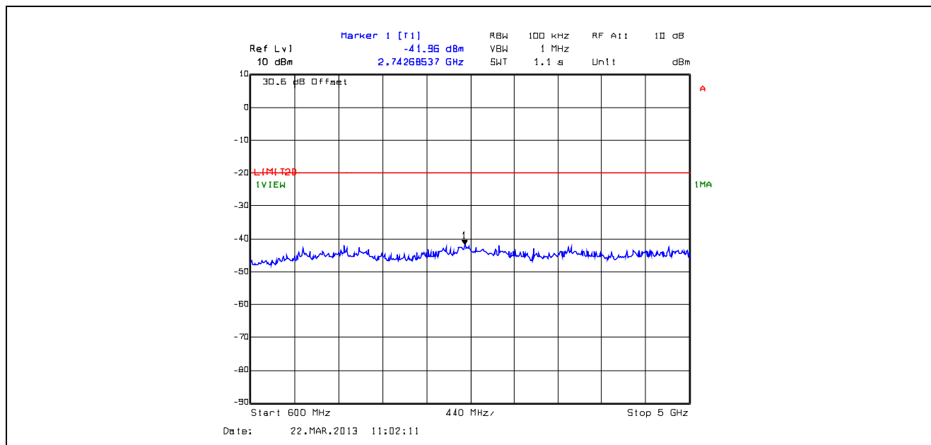
Plot 5.5.4.2. Conducted Transmitter Spurious Emissions, High Power, 406.2 MHz, 600 MHz - 5 GHz
