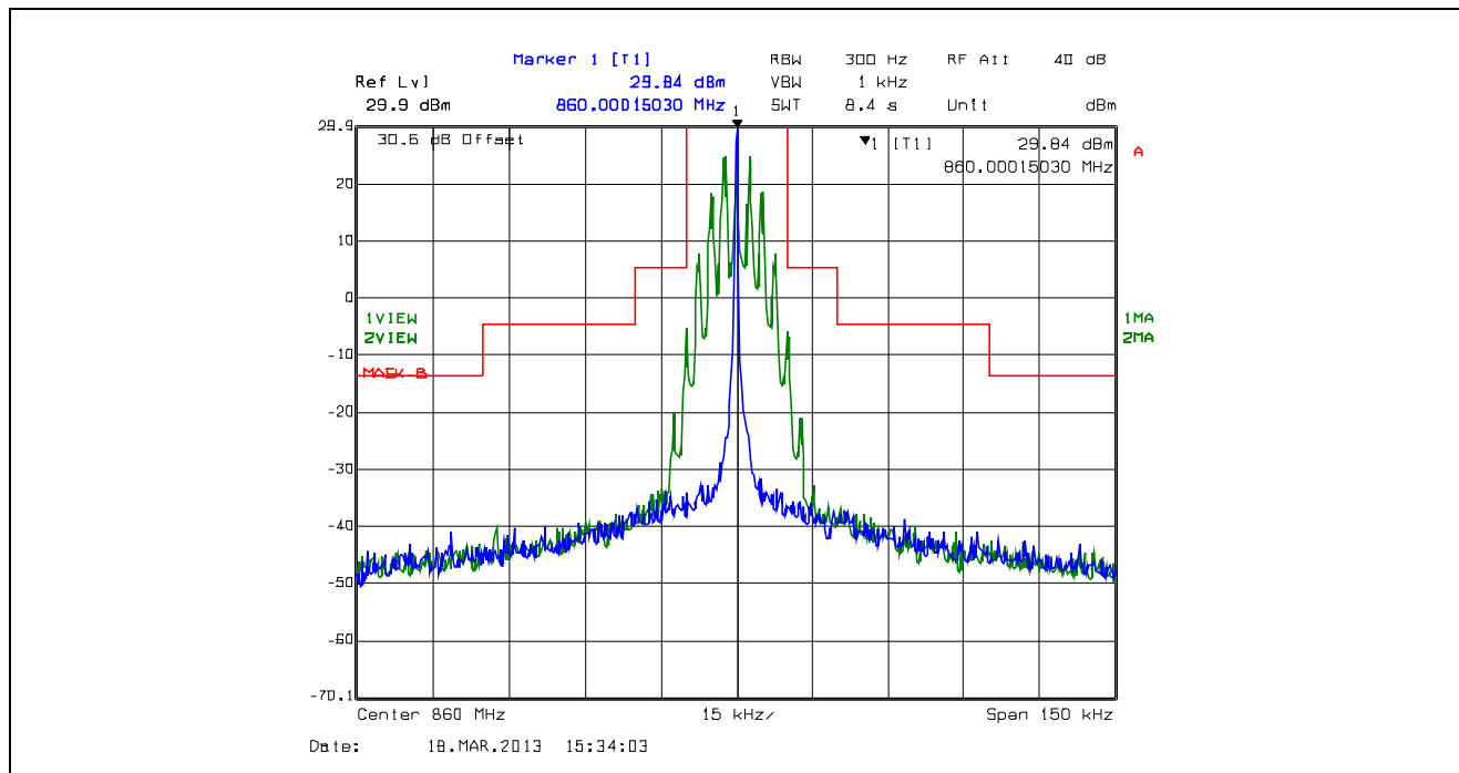
Plot 5.4.4.2.66. Emission Mask B, 25 kHz Channel Spacing, F3E, Low Power, 860.0 MHz
