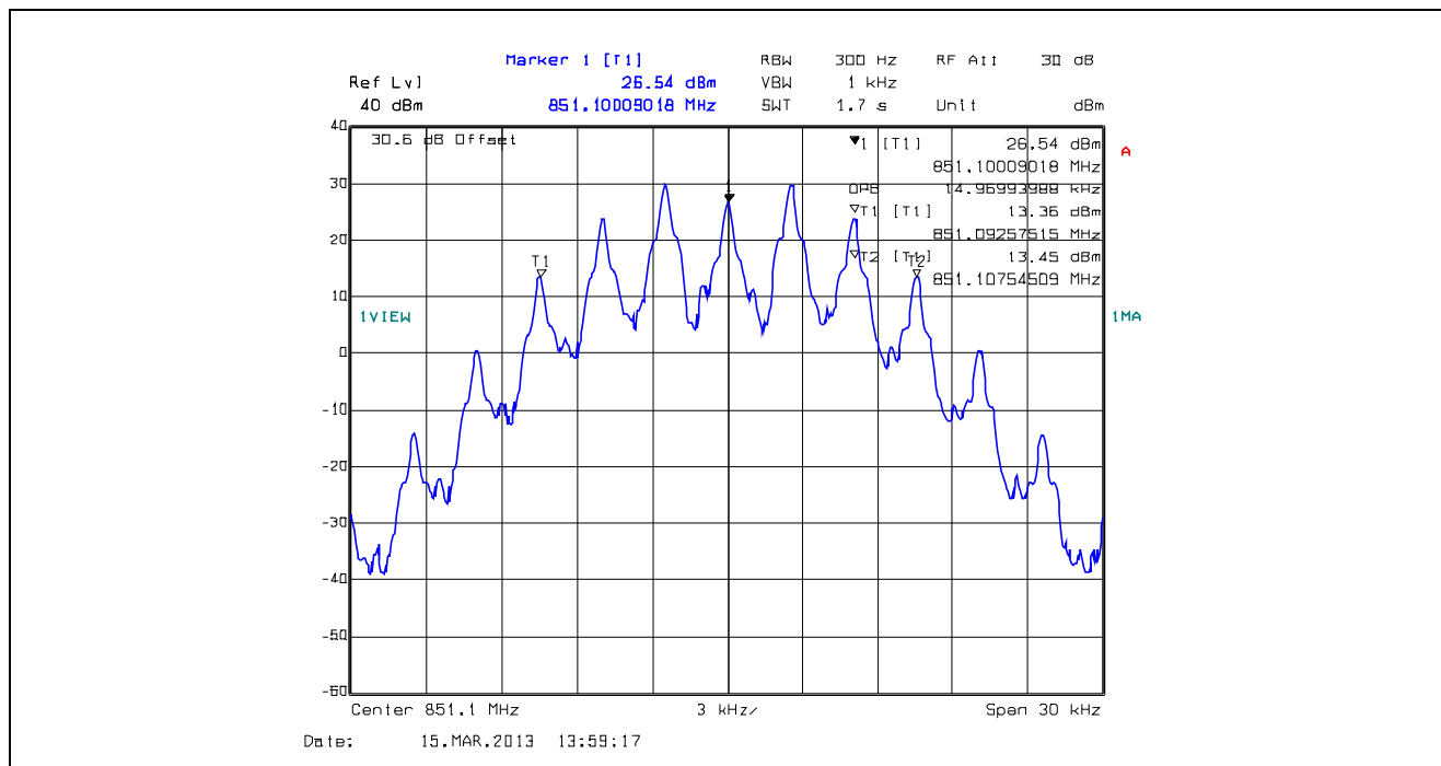
Plot 5.4.4.1.62. 99% Occupied Bandwidth, 25 kHz Channel Spacing, F3E, 851.1 MHz
