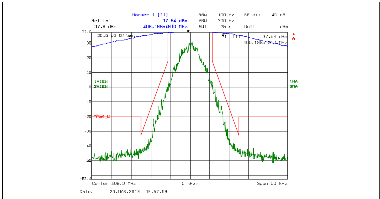
Plot 5.4.4.2.9. Emission Mask D, 12.5 kHz Channel Spacing, F1E, High Power, 406.2 MHz
