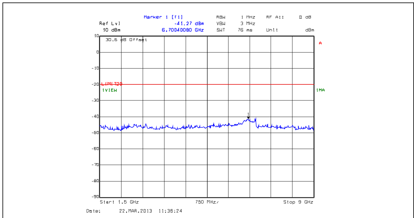
Plot 5.5.4.44. Conducted Transmitter Spurious Emissions, Low Power, 815.0 MHz, 1.5 GHz - 9 GHz
