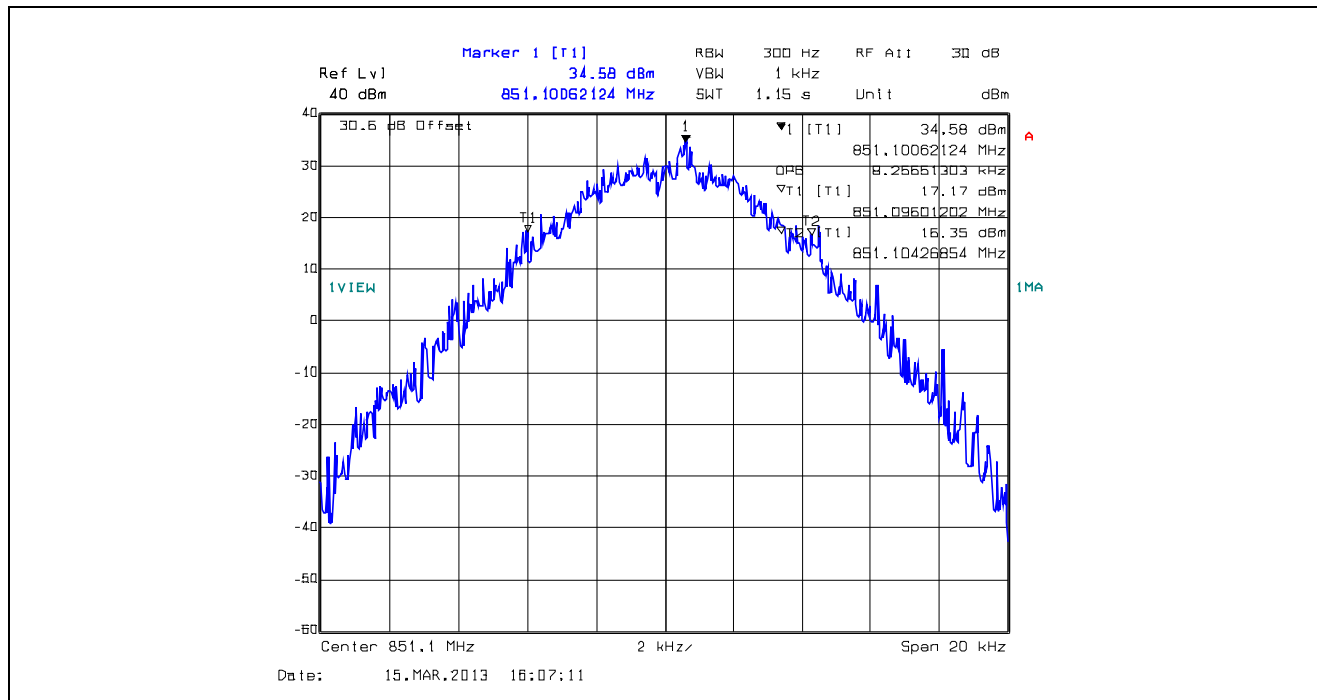
Plot 5.4.4.1.68. 99% Occupied Bandwidth, 12.5 kHz Channel Spacing, F1D, 851.1 MHz
