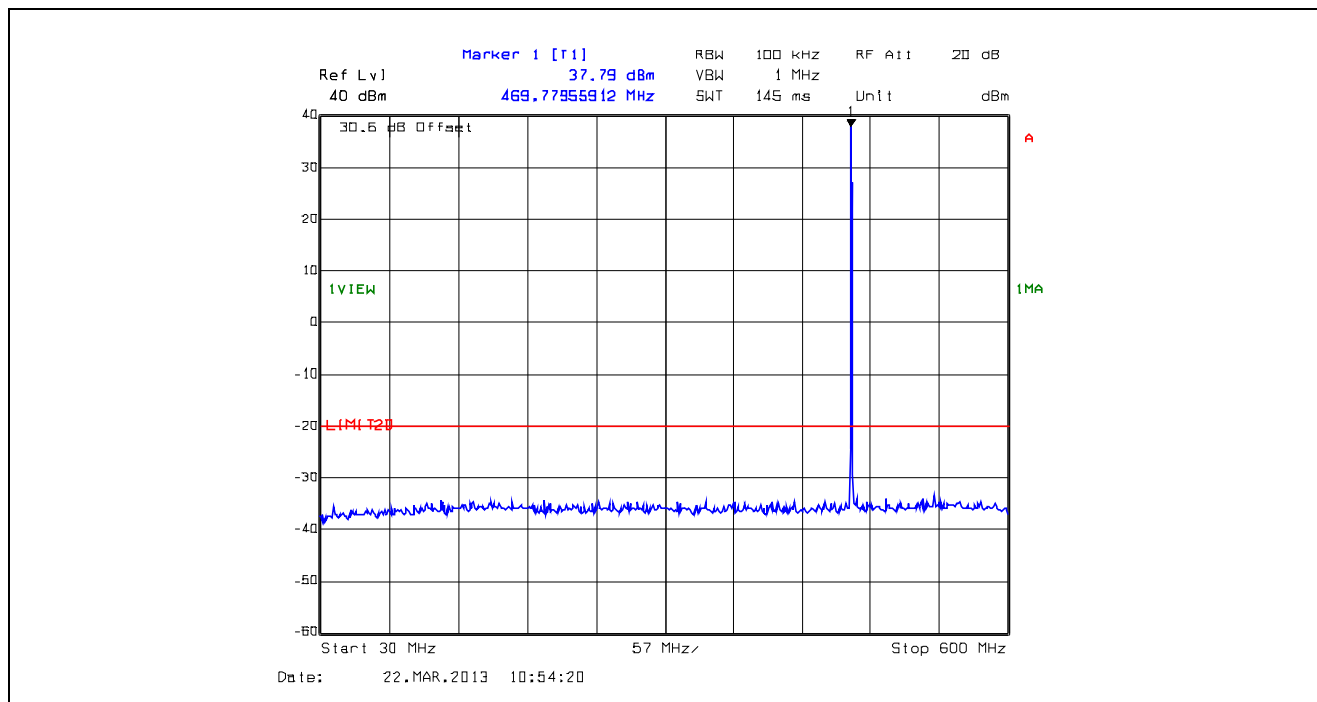
Plot 5.5.4.9. Conducted Transmitter Spurious Emissions, High Power, 469.9 MHz, 30 MHz - 600 MHz
