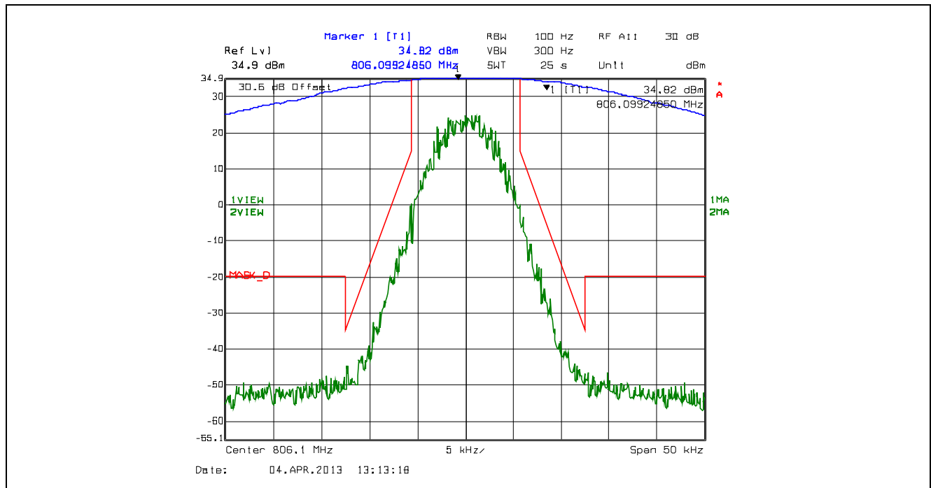
Plot 5.4.4.2.51. Emission Mask D, 12.5 kHz Channel Spacing, F1W, High Power, 806.1 MHz
