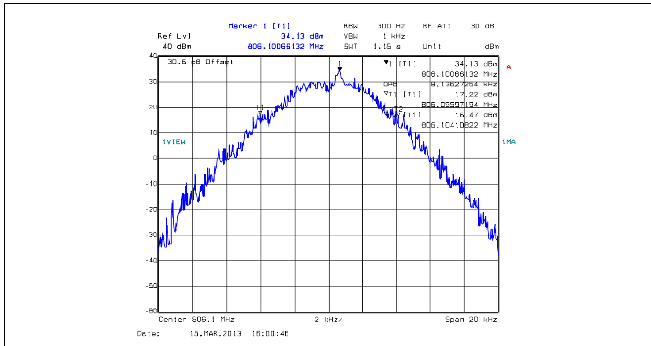
Plot 5.4.4.1.53. 99% Occupied Bandwidth, 12.5 kHz Channel Spacing, F1D, 806.1 MHz
