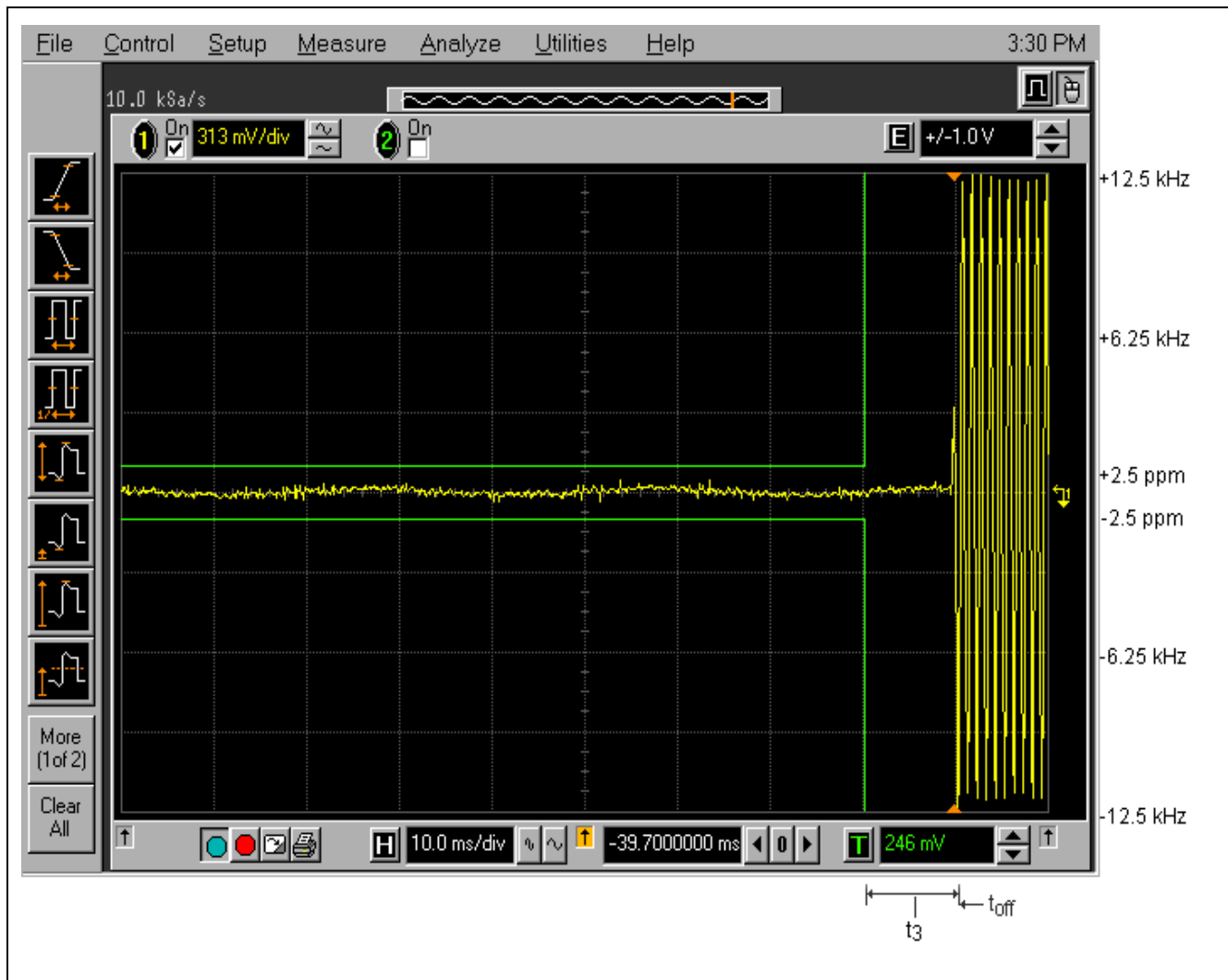
Plot 5.8.4.2. Transient Frequency Behavior on 12.5 kHz Channels Test Frequency: 406.2 MHz; Power: 5 W; Test Conditions: Switch off condition t_3 , t_{off}
