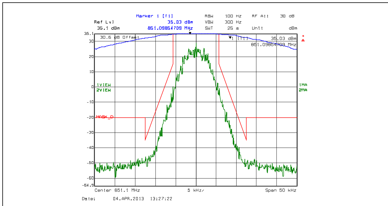
Plot 5.4.4.2.81. Emission Mask D, 12.5 kHz Channel Spacing, F1W, High Power, 851.1 MHz
