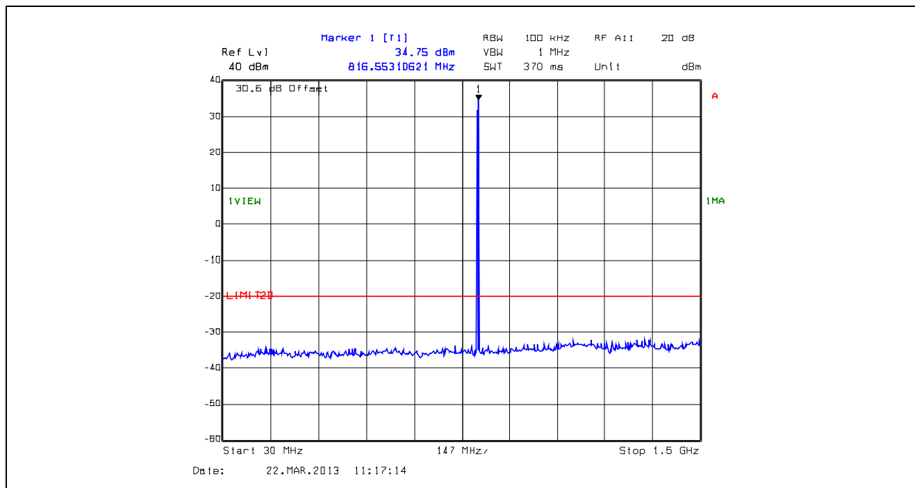
Plot 5.5.4.41. Conducted Transmitter Spurious Emissions, High Power, 815.0 MHz, 30 MHz - 1.5 GHz
