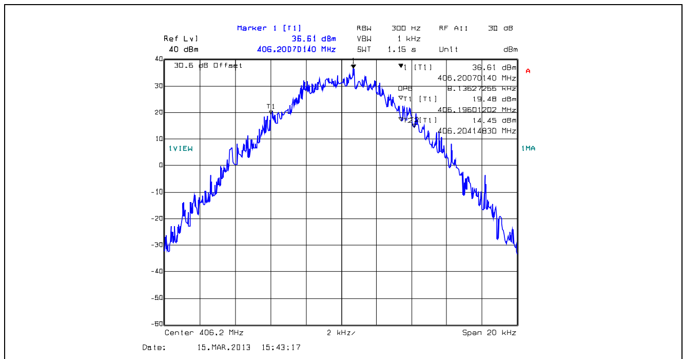
Plot 5.4.4.1.8. 99% Occupied Bandwidth, 12.5 kHz Channel Spacing, F1D, 406.2 MHz
