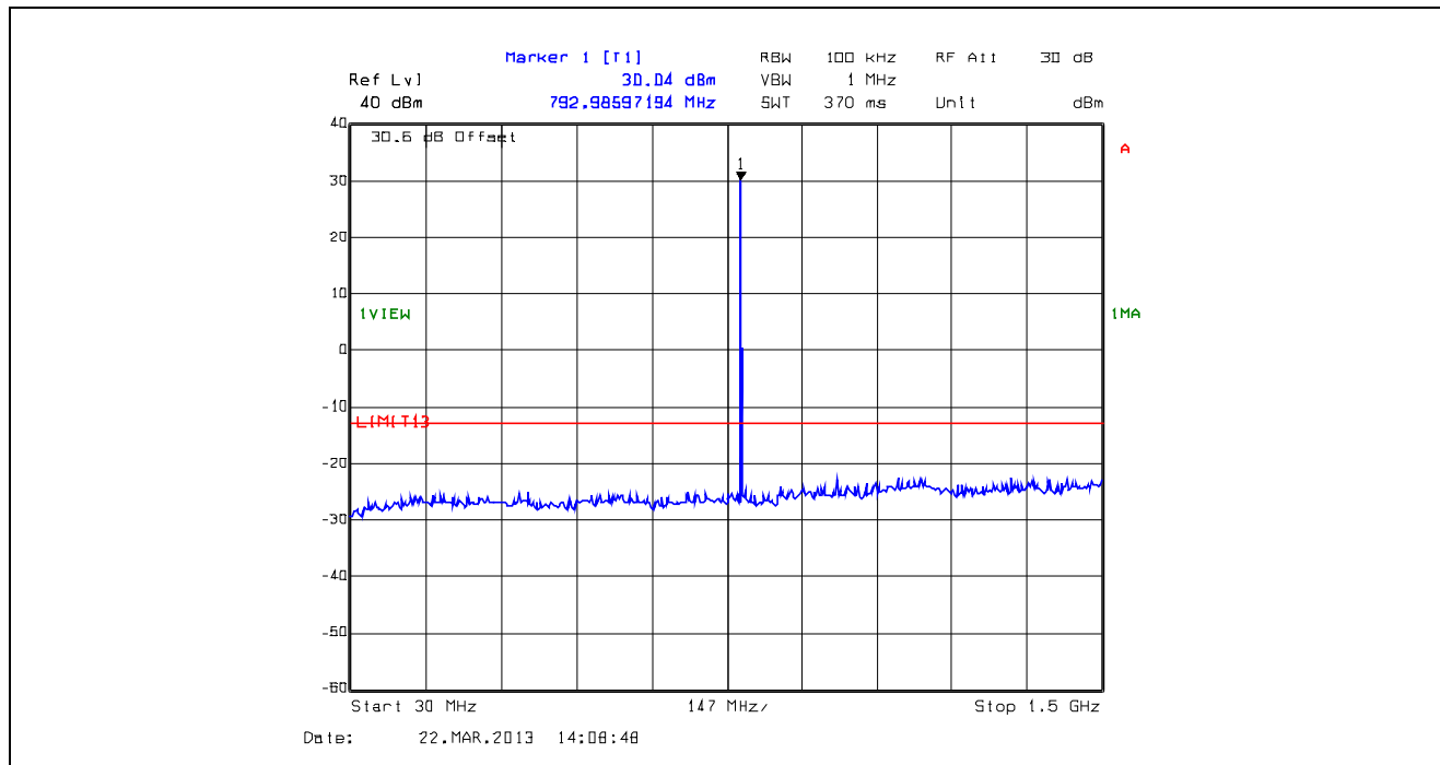
Plot 5.5.4.27. Conducted Transmitter Spurious Emissions, Low Power, 794.1 MHz, 30 MHz - 1.5 GHz
