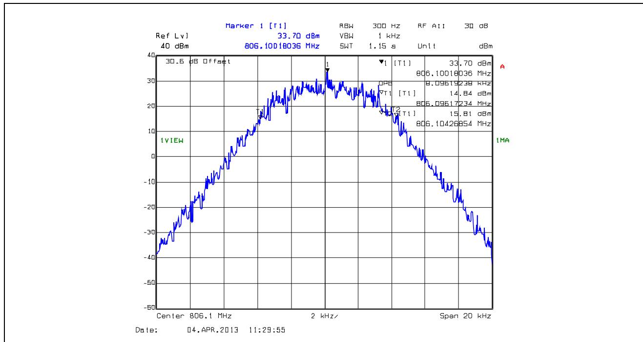
Plot 5.4.4.1.56. 99% Occupied Bandwidth, 12.5 kHz Channel Spacing, F1W, 806.1 MHz
