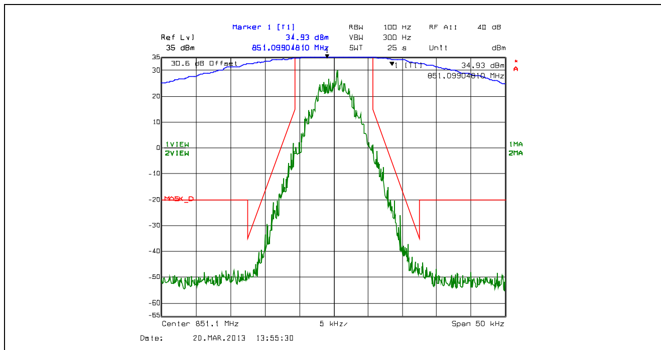
Plot 5.4.4.2.75. Emission Mask D, 12.5 kHz Channel Spacing, F1D, High Power, 851.1 MHz
