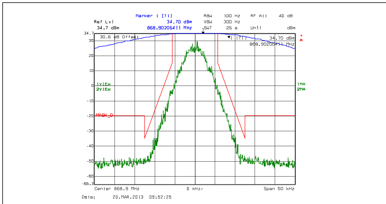
Plot 5.4.4.2.73. Emission Mask D, 12.5 kHz Channel Spacing, F1E, High Power, 868.9 MHz
