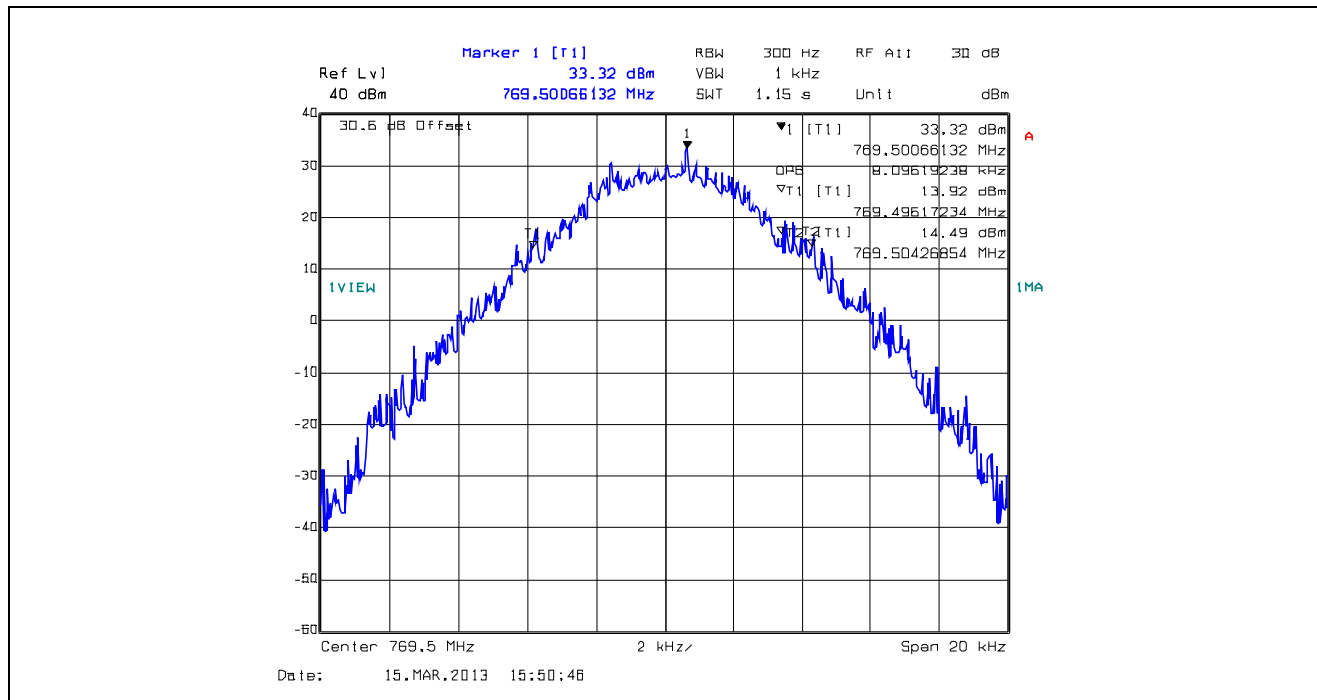
Plot 5.4.4.1.24. 99% Occupied Bandwidth, 12.5 kHz Channel Spacing, F1D, 769.5 MHz
