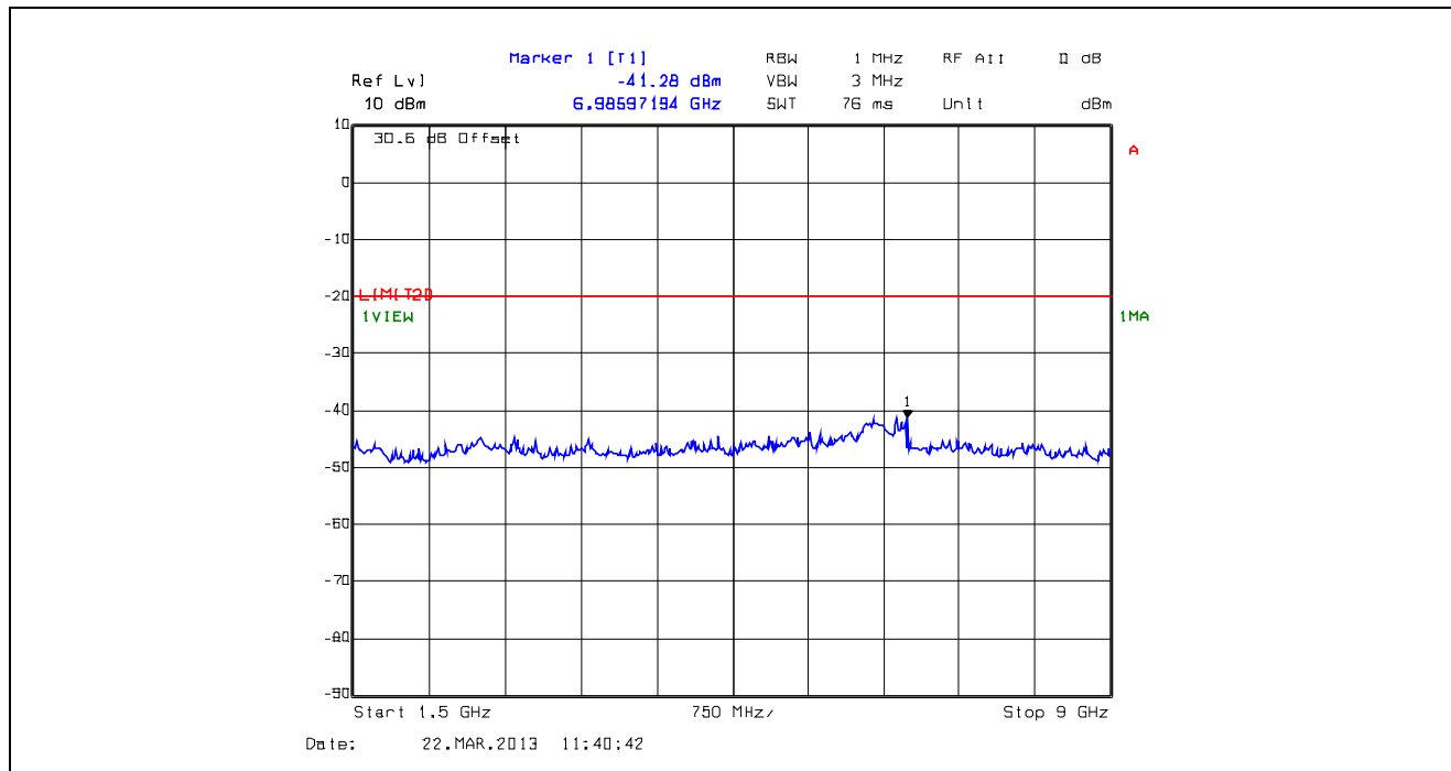
Plot 5.5.4.60. Conducted Transmitter Spurious Emissions, Low Power, 868.9 MHz, 1.5 GHz - 9 GHz
