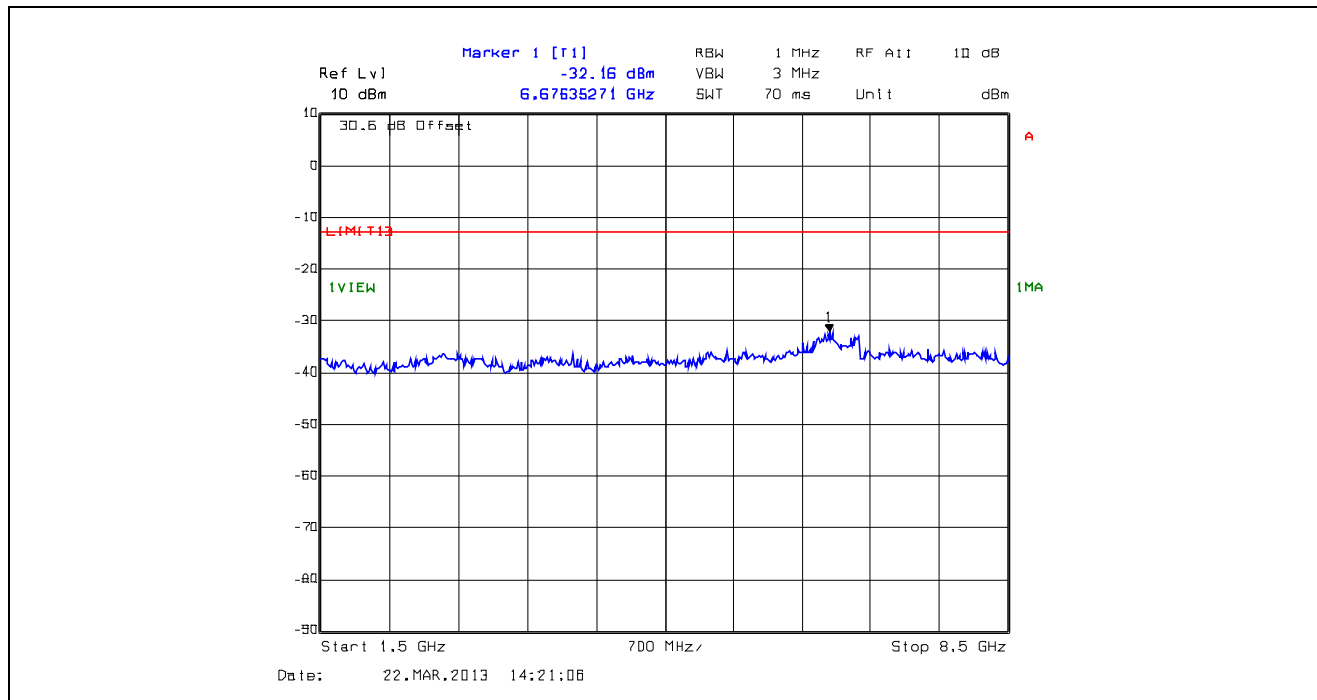
Plot 5.5.4.28. Conducted Transmitter Spurious Emissions, Low Power, 794.1 MHz, 1.5 GHz - 8.5 GHz
