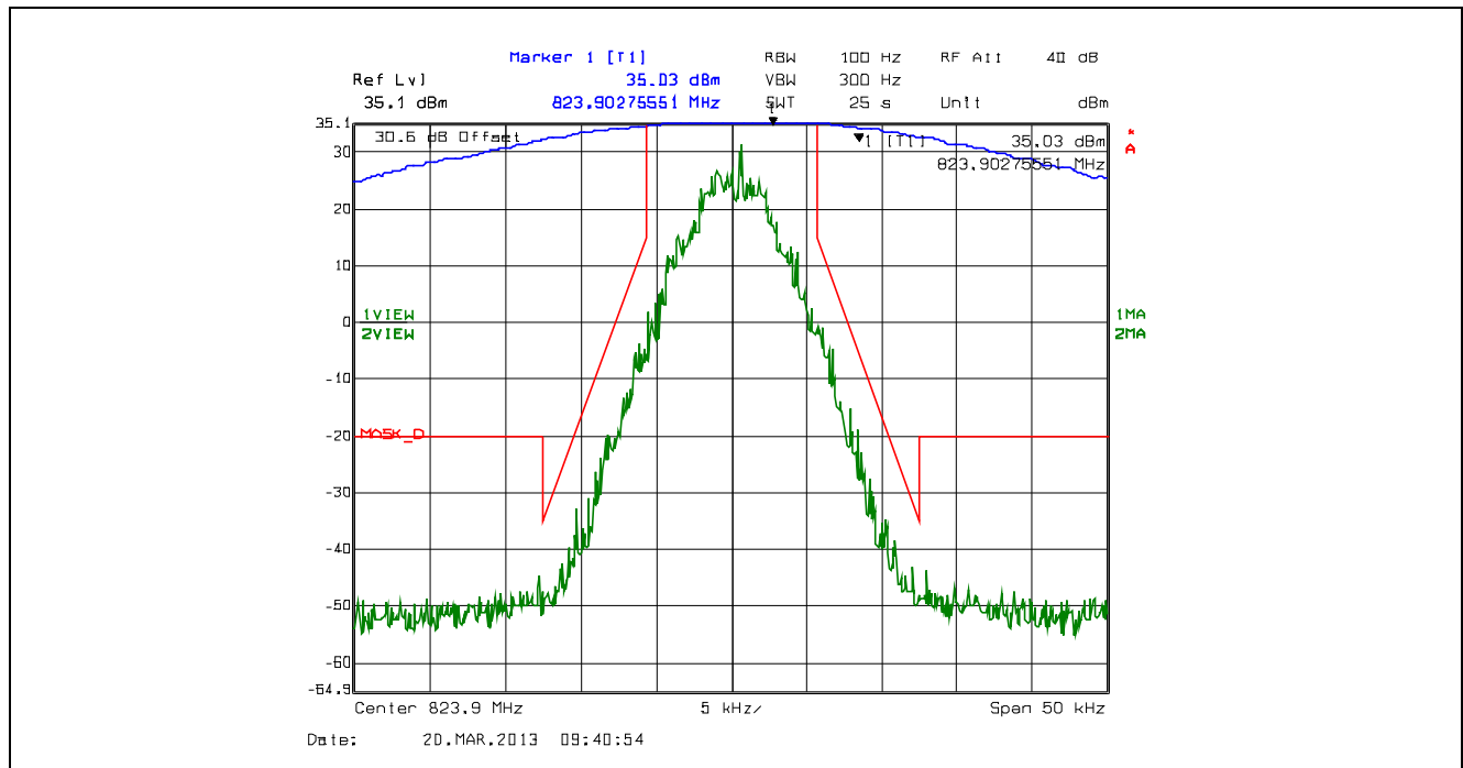
Plot 5.4.4.2.43. Emission Mask D, 12.5 kHz Channel Spacing, F1E, High Power, 823.9 MHz
