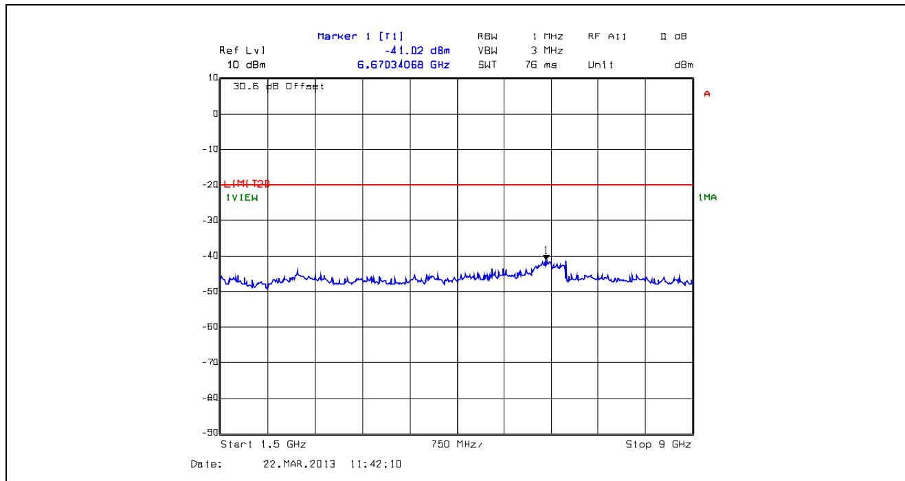
Plot 5.5.458. Conducted Transmitter Spurious Emissions, High Power, 868.9 MHz, 1.5 GHz - 9 GHz
