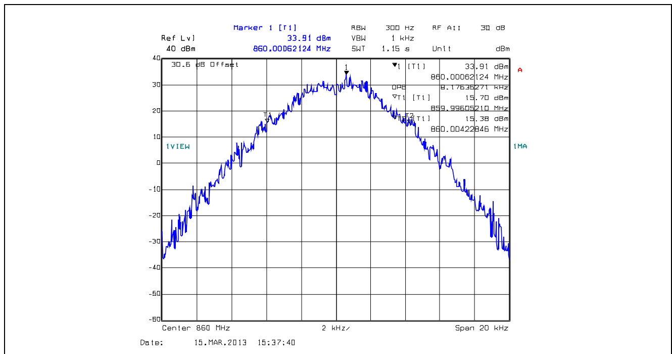
Plot 5.4.4.1.66. 99% Occupied Bandwidth, 12.5 kHz Channel Spacing, F1E, 860.0 MHz
