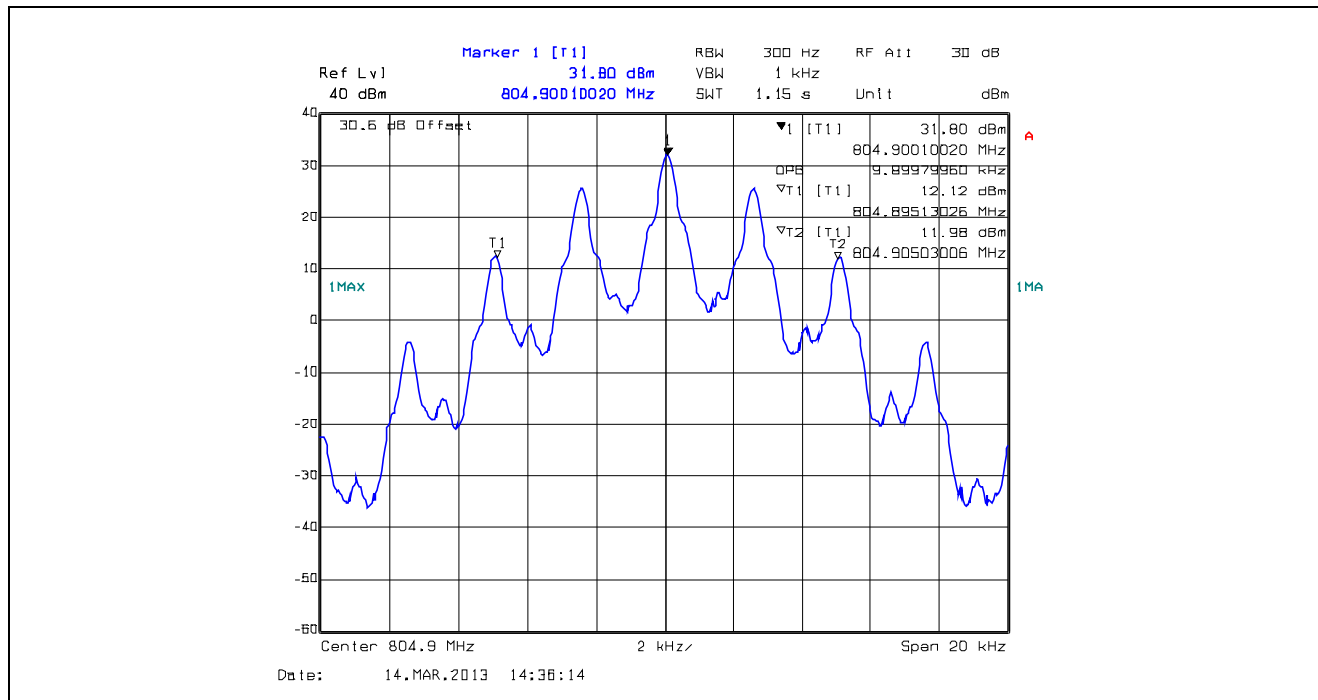
Plot 5.4.4.1.31. 99% Occupied Bandwidth, 12.5 kHz Channel Spacing, F3E, 804.9 MHz
