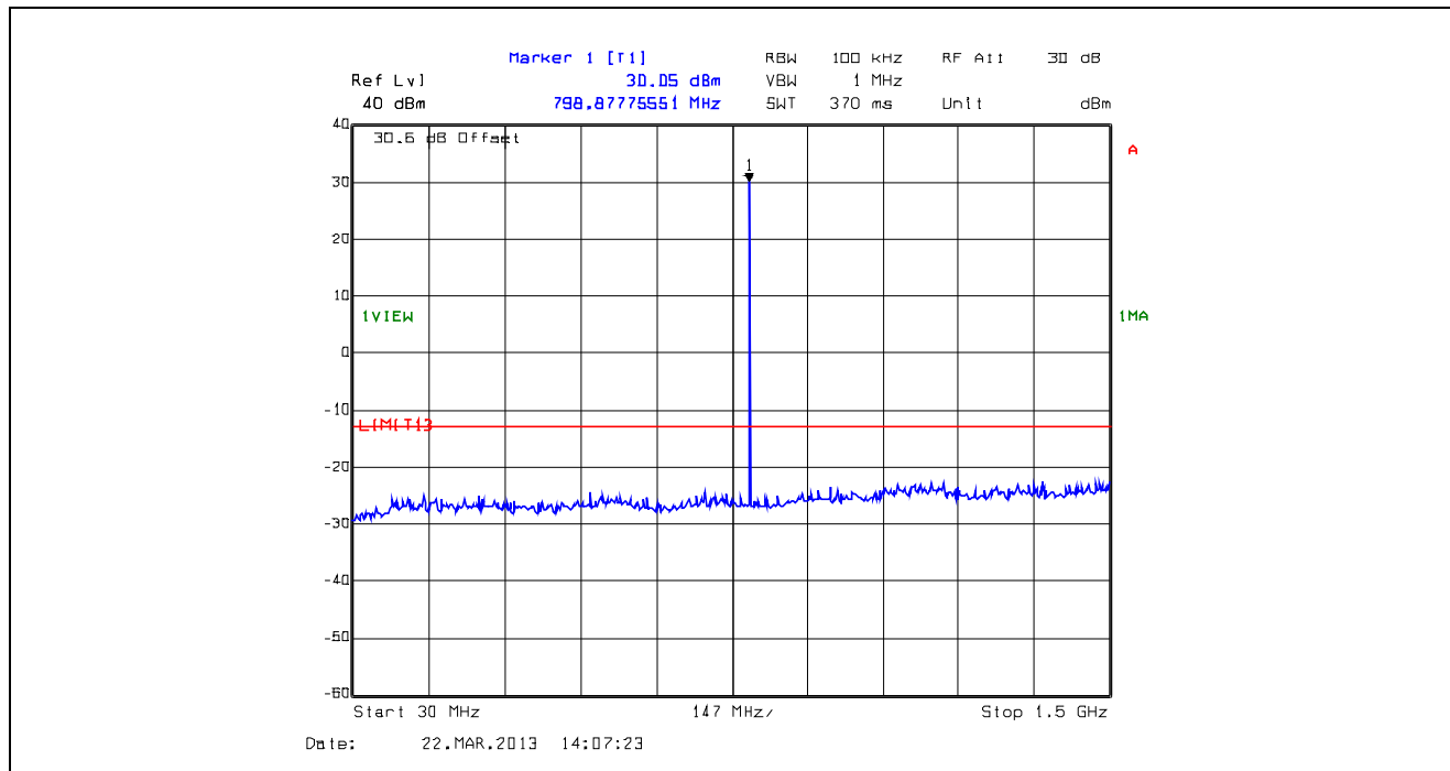
Plot 5.5.4.31. Conducted Transmitter Spurious Emissions, Low Power, 798.5 MHz, 30 MHz - 1.5 GHz
