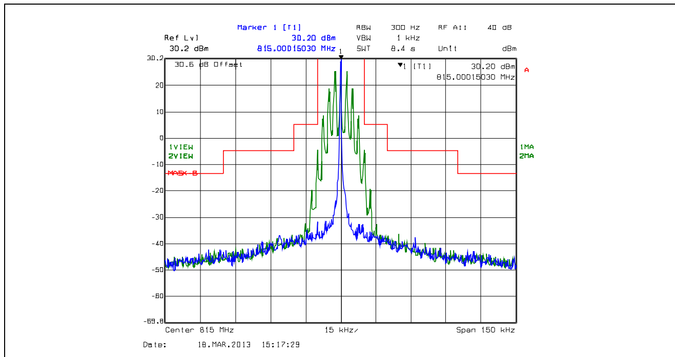
Plot 5.4.4.2.36. Emission Mask B, 25 kHz Channel Spacing, F3E, Low Power, 815.0 MHz
