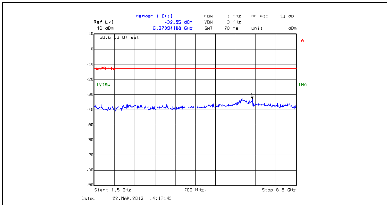
Plot 5.5.4.16. Conducted Transmitter Spurious Emissions, Low Power, 764.1 MHz, 1.5 GHz - 8.5 GHz
