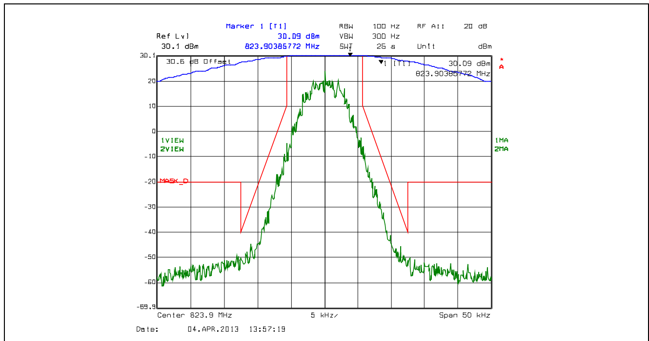
Plot 5.4.4.2.56. Emission Mask D, 12.5 kHz Channel Spacing, F1W, Low Power, 823.9 MHz
