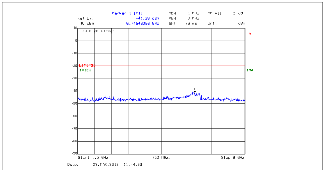
Plot 5.5.4.50. Conducted Transmitter Spurious Emissions, High Power, 851.1 MHz, 1.5 GHz - 9 GHz
