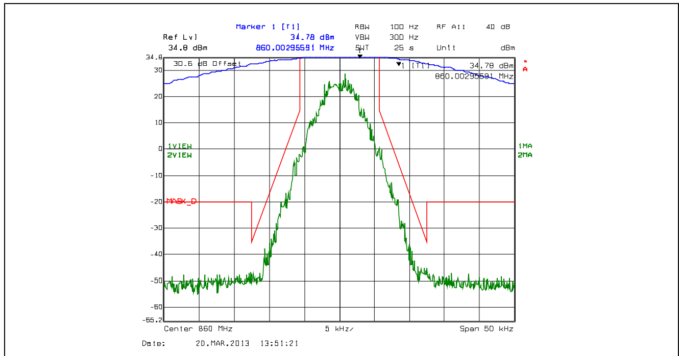
Plot 5.4.4.2.77. Emission Mask D, 12.5 kHz Channel Spacing, F1D, High Power, 860.0 MHz
