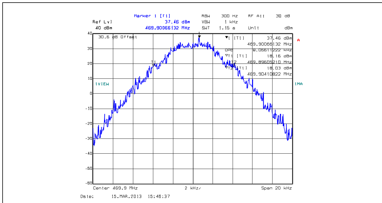
Plot 5.4.4.1.10. 99% Occupied Bandwidth, 12.5 kHz Channel Spacing, F1D, 469.9 MHz
