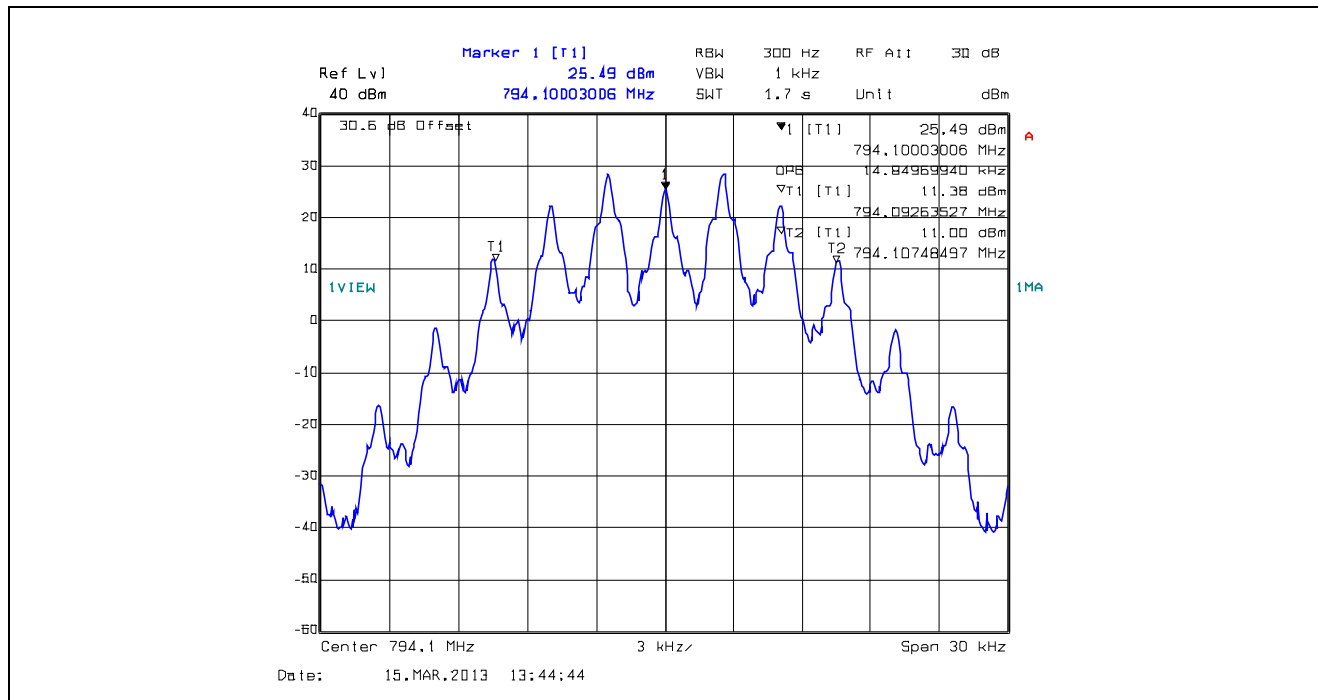
Plot 5.4.4.1.32. 99% Occupied Bandwidth, 25 kHz Channel Spacing, F3E, 794.1MHz
