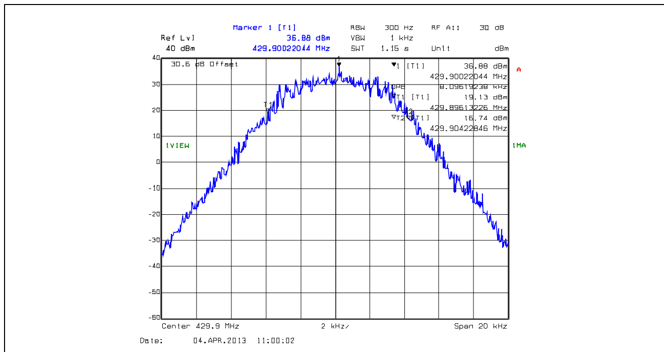
Plot 5.4.4.1.12. 99% Occupied Bandwidth, 12.5 kHz Channel Spacing, F1W, 429.9 MHz
