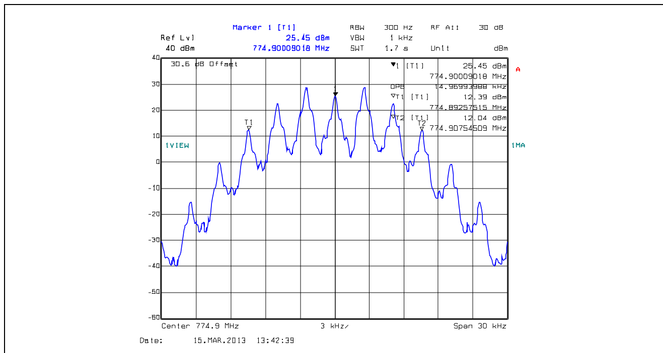
Plot 5.4.4.1.19. 99% Occupied Bandwidth, 25 kHz Channel Spacing, F3E, 774.9MHz
