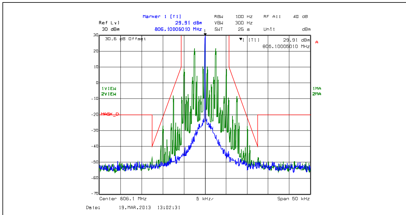
Plot 5.4.4.2.28. Emission Mask D, 12.5 kHz Channel Spacing, F3E, Low Power, 806.1 MHz
