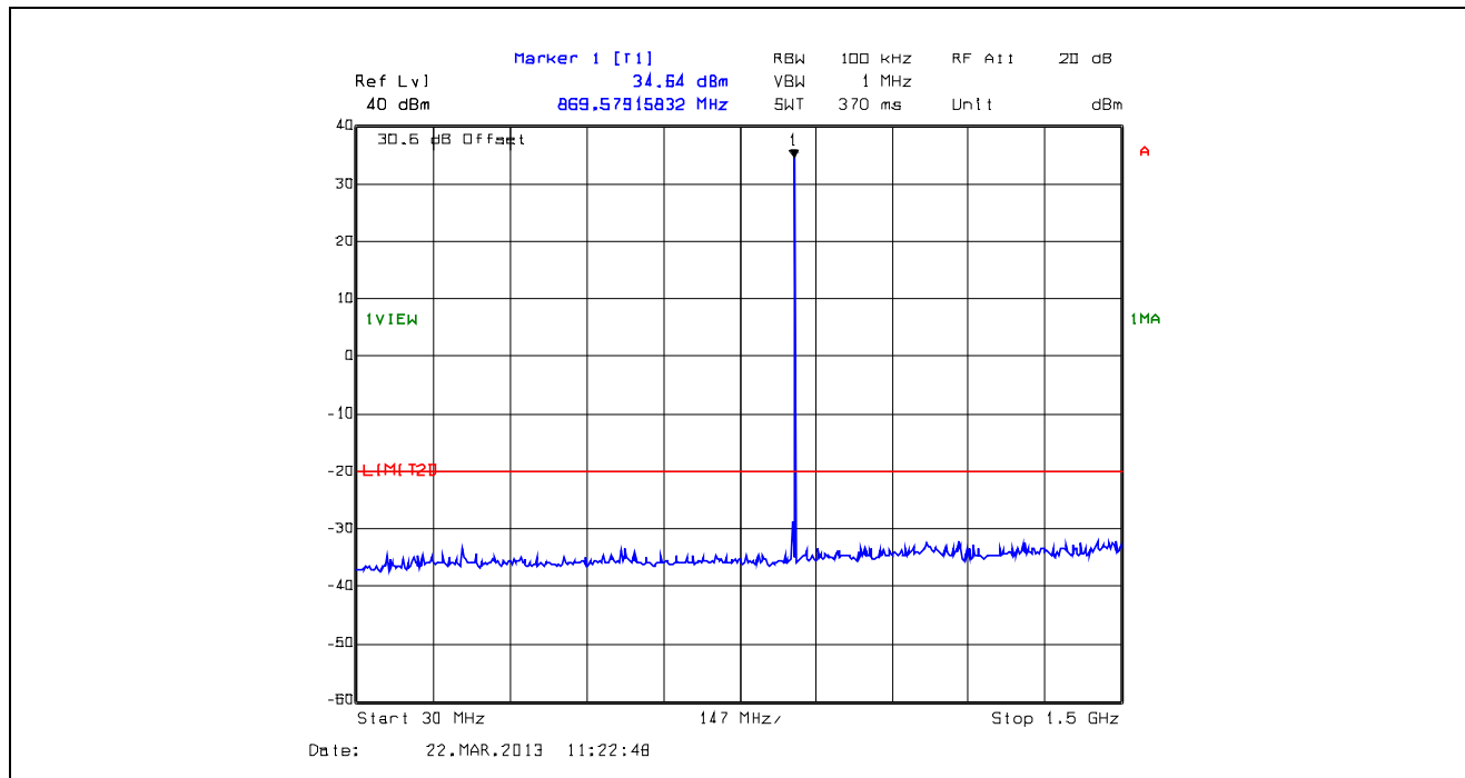
Plot 5.5.457. Conducted Transmitter Spurious Emissions, High Power, 868.9 MHz, 30 MHz - 1.5 GHz
