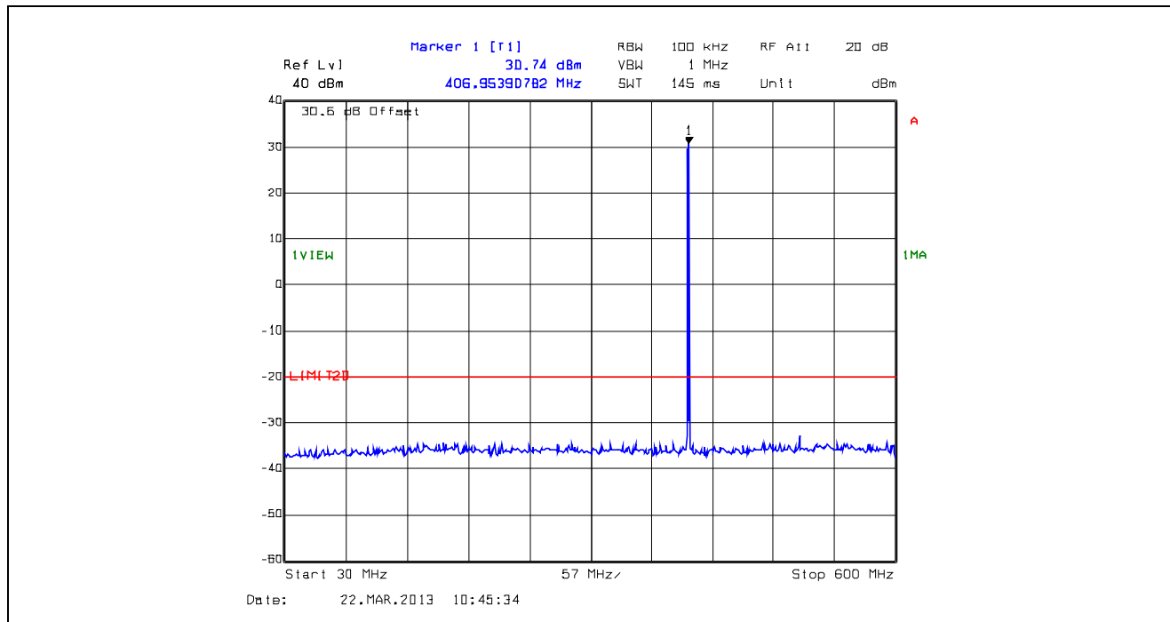
Plot 5.5.4.3. Conducted Transmitter Spurious Emissions, Low Power, 406.2 MHz, 30 MHz - 600 MHz
