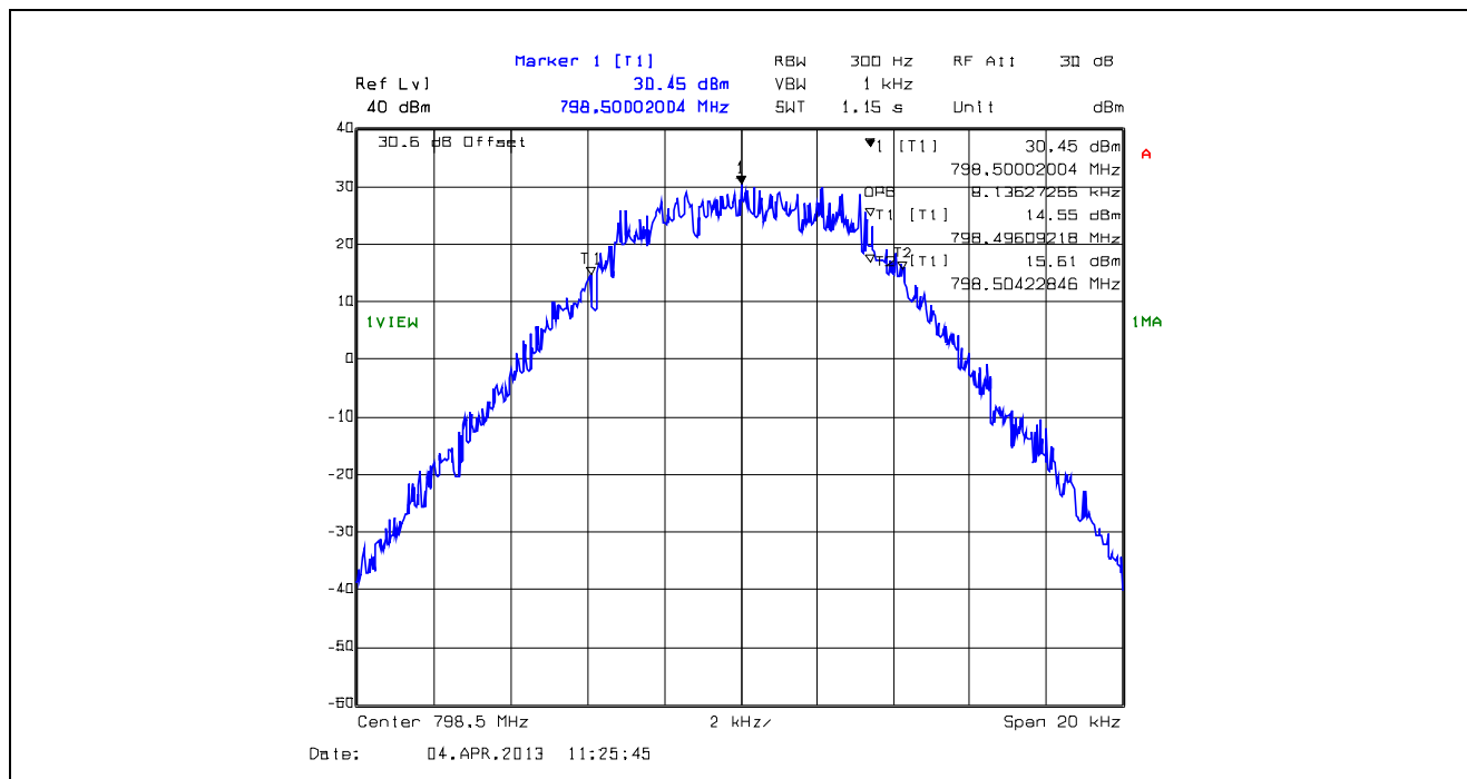
Plot 5.4.4.1.42. 99% Occupied Bandwidth, 12.5 kHz Channel Spacing, F1W, 798.5 MHz
