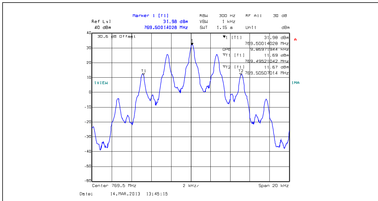
Plot 5.4.4.1.15. 99% Occupied Bandwidth, 12.5 kHz Channel Spacing, F3E, 769.5 MHz
