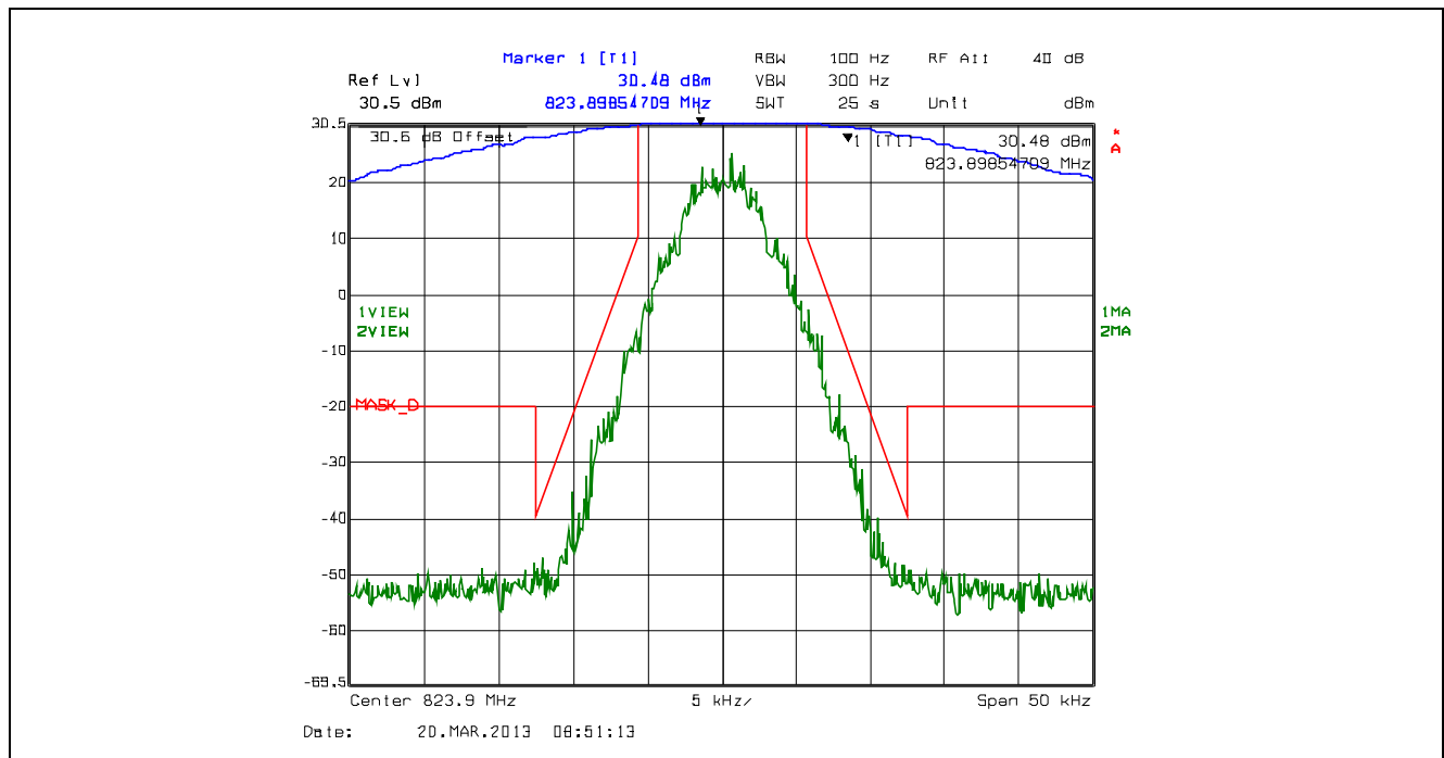
Plot 5.4.4.2.44. Emission Mask D, 12.5 kHz Channel Spacing, F1E, Low Power, 823.9 MHz
