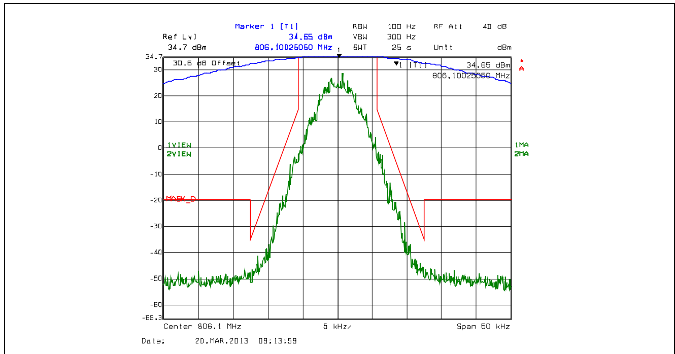
Plot 5.4.4.2.39. Emission Mask D, 12.5 kHz Channel Spacing, F1E, High Power, 806.1 MHz
