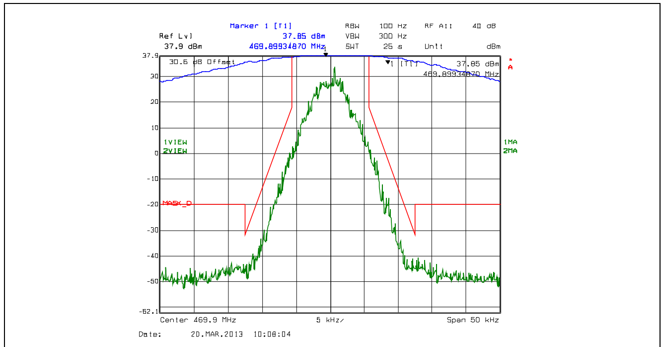
Plot 5.4.4.2.13. Emission Mask D, 12.5 kHz Channel Spacing, F1E, High Power, 469.9 MHz
