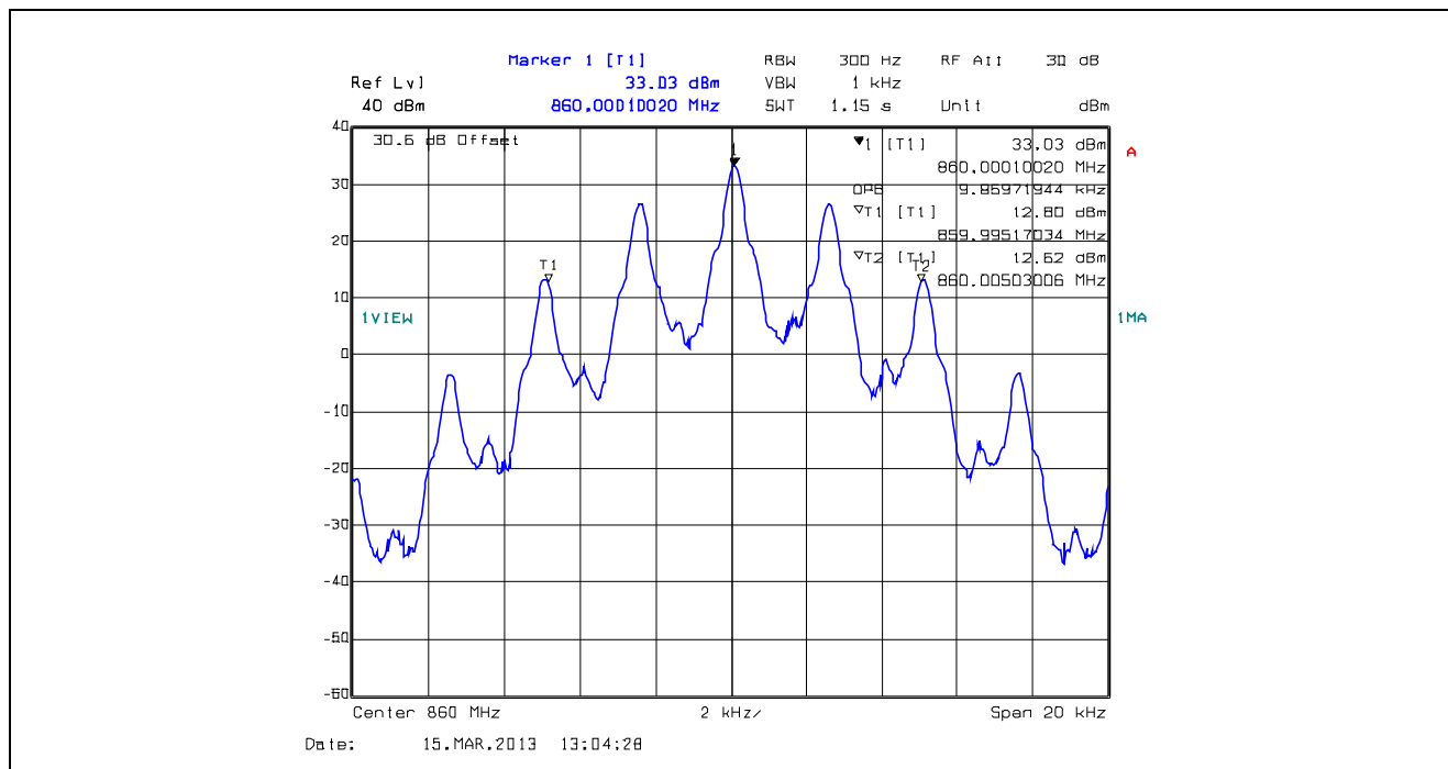
Plot 5.4.4.1.60. 99% Occupied Bandwidth, 12.5 kHz Channel Spacing, F3E, 860.0 MHz
