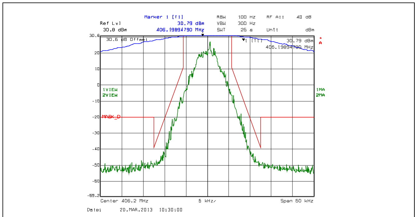
Plot 5.4.4.2.16. Emission Mask D, 12.5 kHz Channel Spacing, F1D, Low Power, 406.2 MHz
