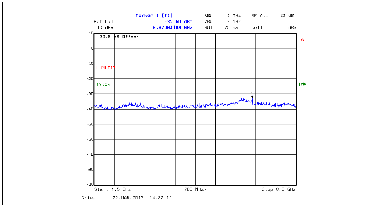
Plot 5.5.4.32. Conducted Transmitter Spurious Emissions, Low Power, 798.5 MHz, 1.5 GHz - 8.5 GHz
