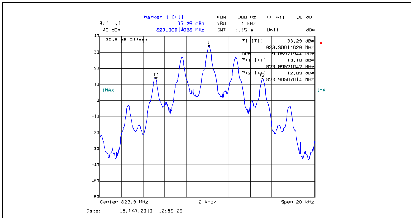
Plot 5.4.4.1.46. 99% Occupied Bandwidth, 12.5 kHz Channel Spacing, F3E, 823.9 MHz
