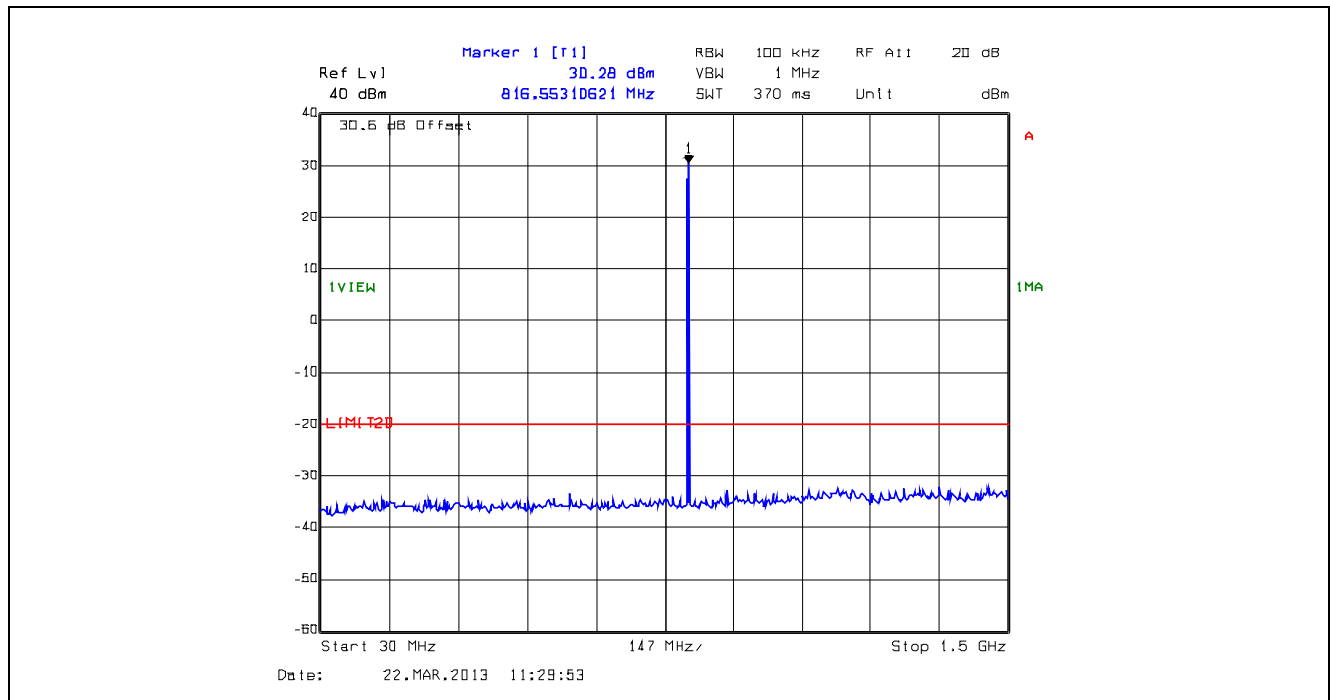
Plot 5.5.4.43. Conducted Transmitter Spurious Emissions, Low Power, 815.0 MHz, 30 MHz - 1.5 GHz
