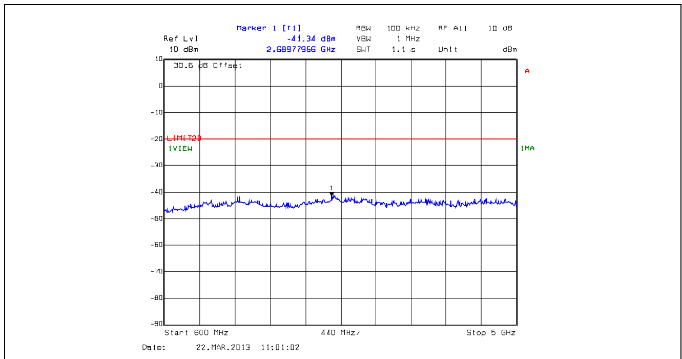
Plot 5.5.4.6. Conducted Transmitter Spurious Emissions, High Power, 429.9 MHz, 600 MHz -5 GHz
