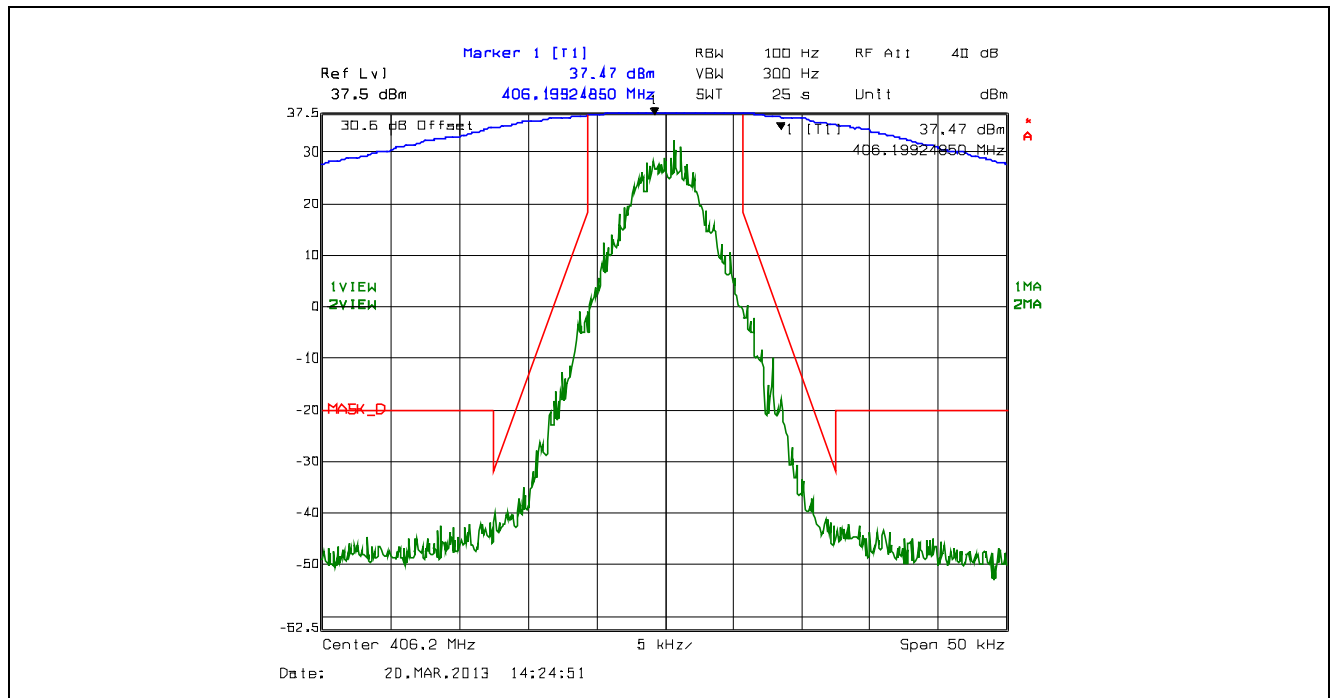
Plot 5.4.4.2.15. Emission Mask D, 12.5 kHz Channel Spacing, F1D, High Power, 406.2 MHz
