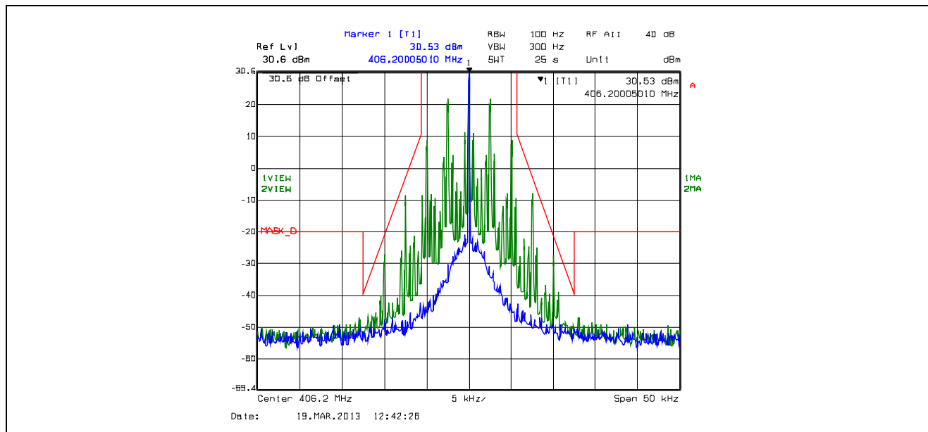
Plot 5.4.4.2.2. Emission Mask D, 12.5 kHz Channel Spacing, F3E, Low Power, 406.2 MHz
