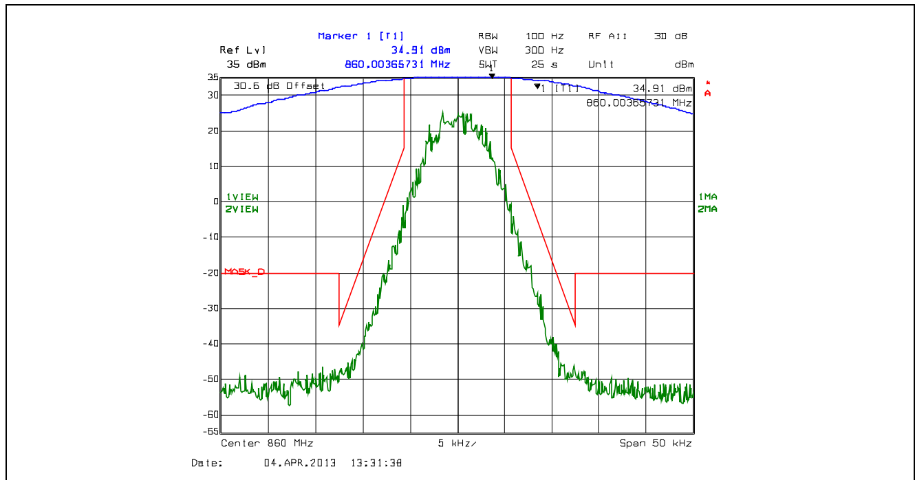
Plot 5.4.4.2.83. Emission Mask D, 12.5 kHz Channel Spacing, F1W, High Power, 860.0 MHz
