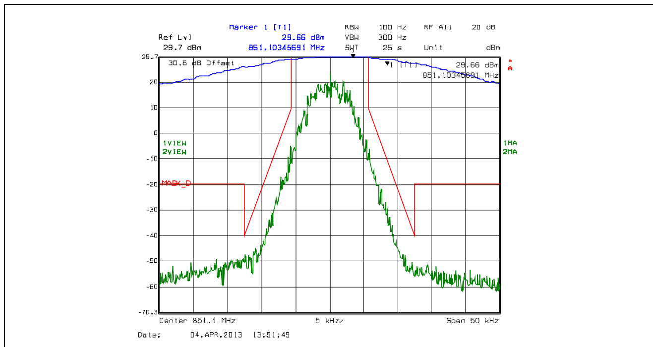
Plot 5.4.4.2.82. Emission Mask D, 12.5 kHz Channel Spacing, F1W, Low Power, 851.1 MHz
