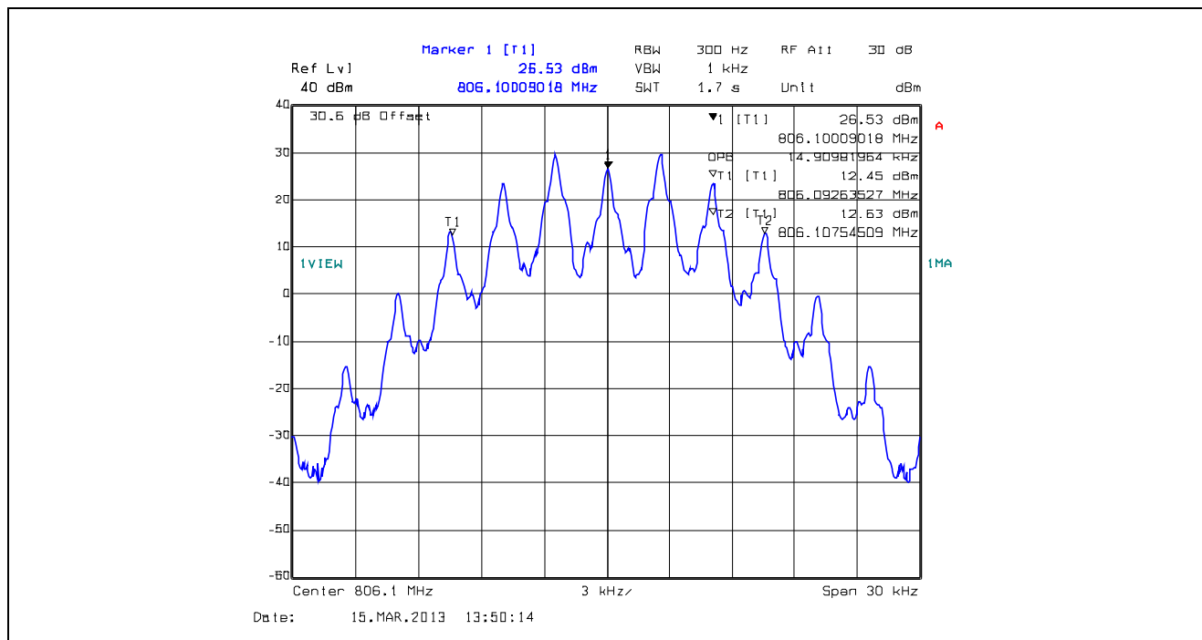
Plot 5.4.4.1.47. 99% Occupied Bandwidth, 25 kHz Channel Spacing, F3E, 806.1 MHz
