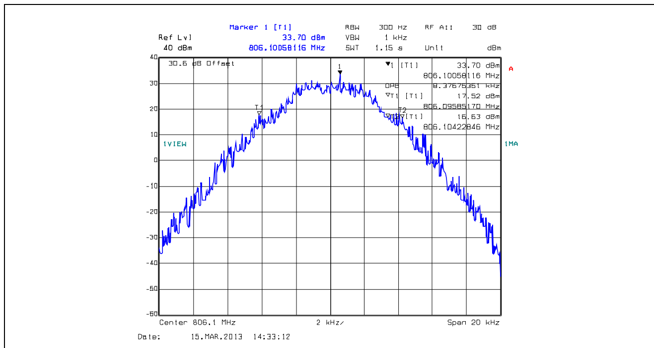
Plot 5.4.4.1.50. 99% Occupied Bandwidth, 12.5 kHz Channel Spacing, F1E, 806.1 MHz
