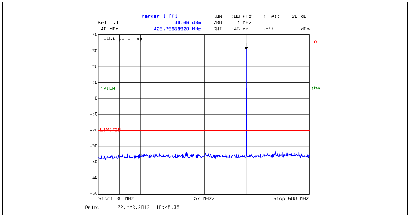
Plot 5.5.4.7. Conducted Transmitter Spurious Emissions, Low Power, 429.9 MHz, 30 MHz - 600 MHz
