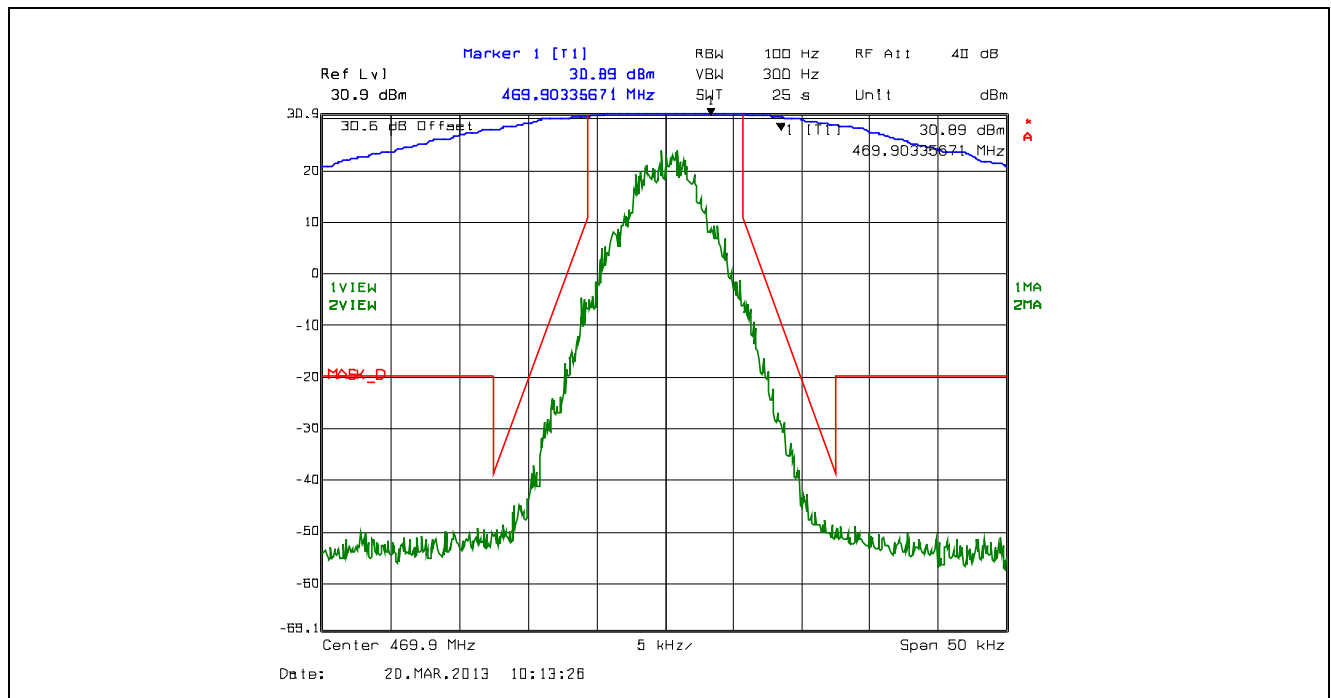
Plot 5.4.4.2.14. Emission Mask D, 12.5 kHz Channel Spacing, F1E, Low Power, 469.9 MHz
