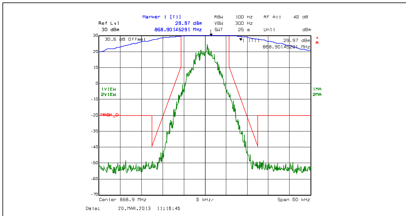
Plot 5.4.4.2.80. Emission Mask D, 12.5 kHz Channel Spacing, F1D, Low Power, 868.9 MHz
