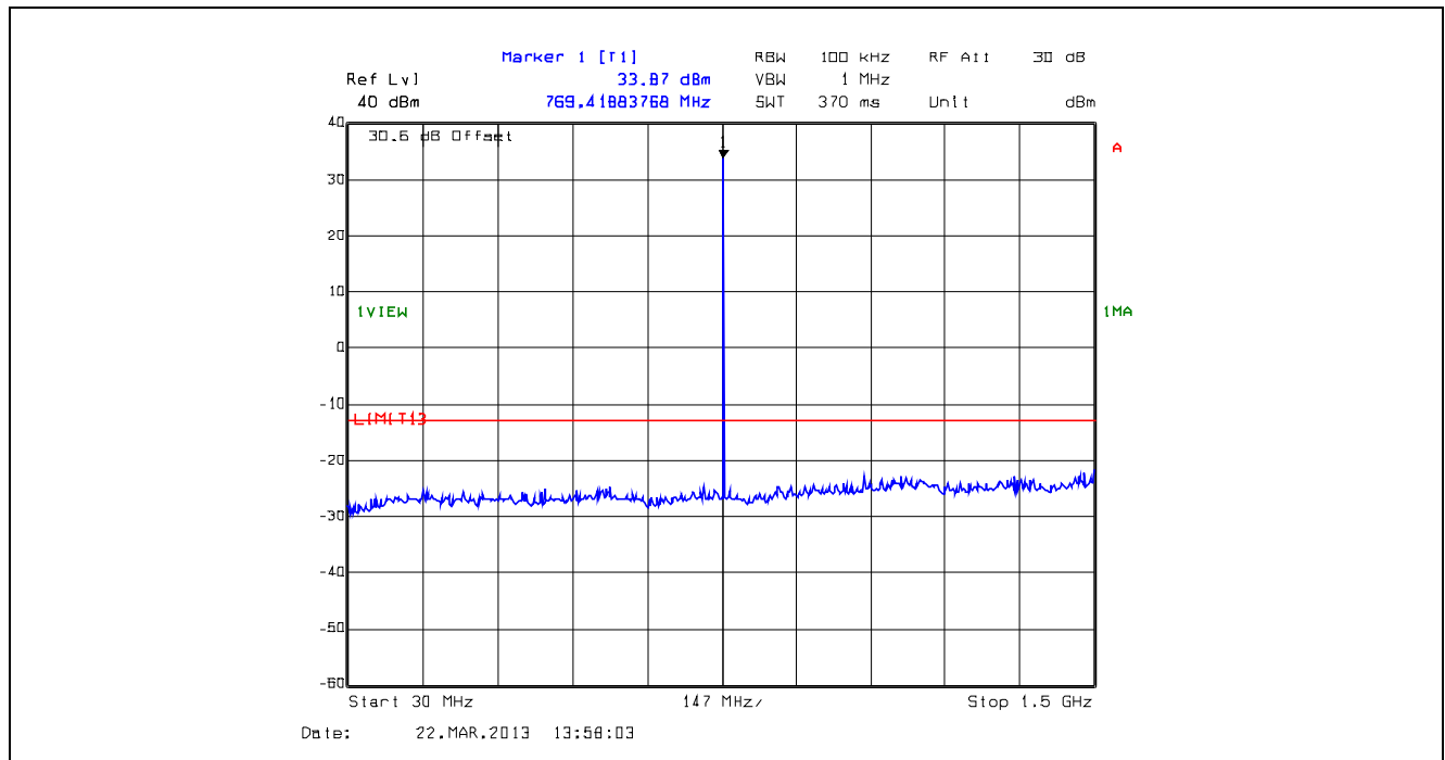
Plot 5.5.4.17. Conducted Transmitter Spurious Emissions, High Power, 769.5 MHz, 30 MHz - 1.5 GHz
