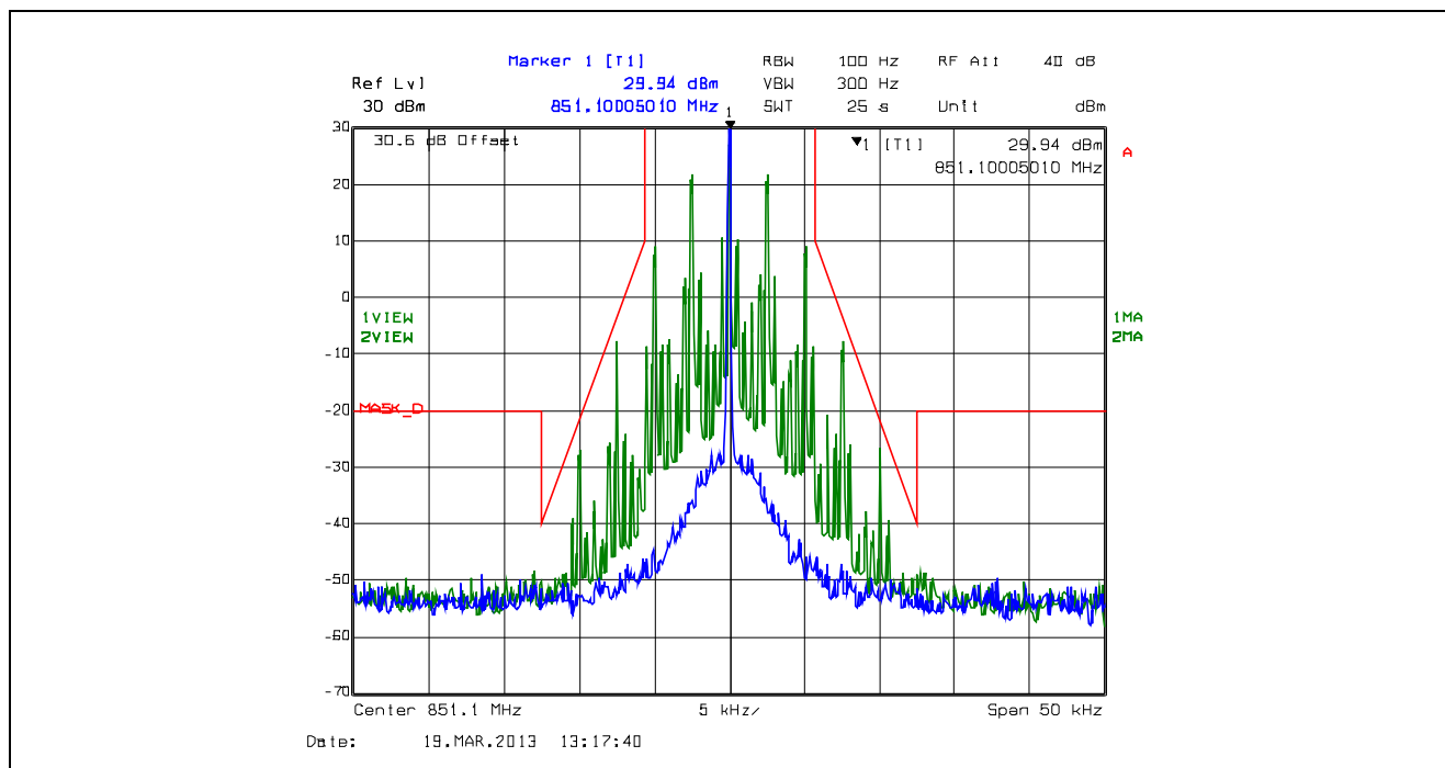
Plot 5.4.4.2.58. Emission Mask D, 12.5 kHz Channel Spacing, F3E, Low Power, 851.1 MHz
