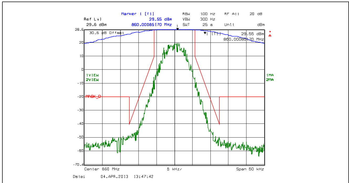
Plot 5.4.4.2.84. Emission Mask D, 12.5 kHz Channel Spacing, F1W, Low Power, 860.0 MHz
