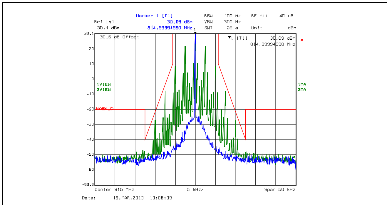
Plot 5.4.4.2.30. Emission Mask D, 12.5 kHz Channel Spacing, F3E, Low Power, 815.0 MHz
