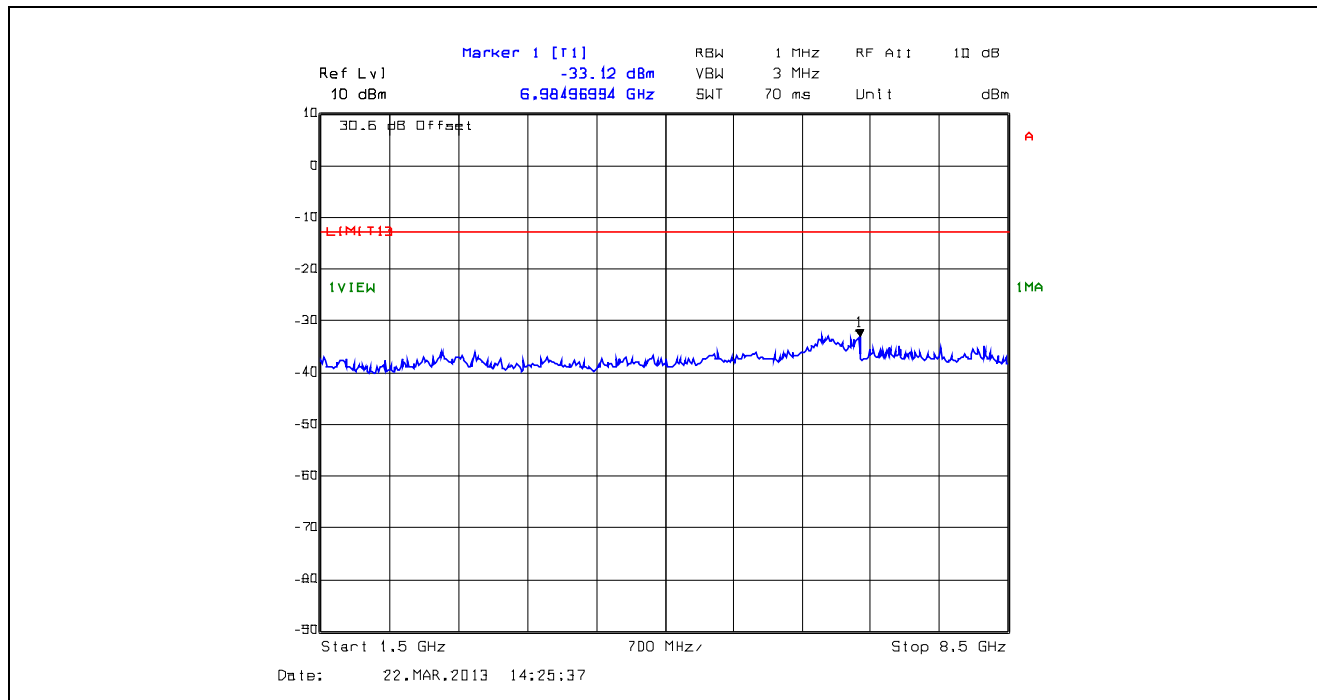
Plot 5.5.4.30. Conducted Transmitter Spurious Emissions, High Power, 798.5 MHz, 1.5 GHz - 8.5 GHz
