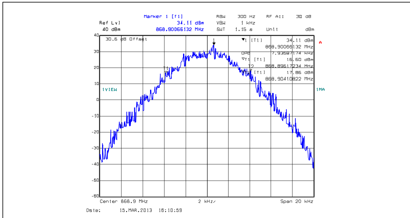
Plot 5.4.4.1.70. 99% Occupied Bandwidth, 12.5 kHz Channel Spacing, F1D, 868.9 MHz
