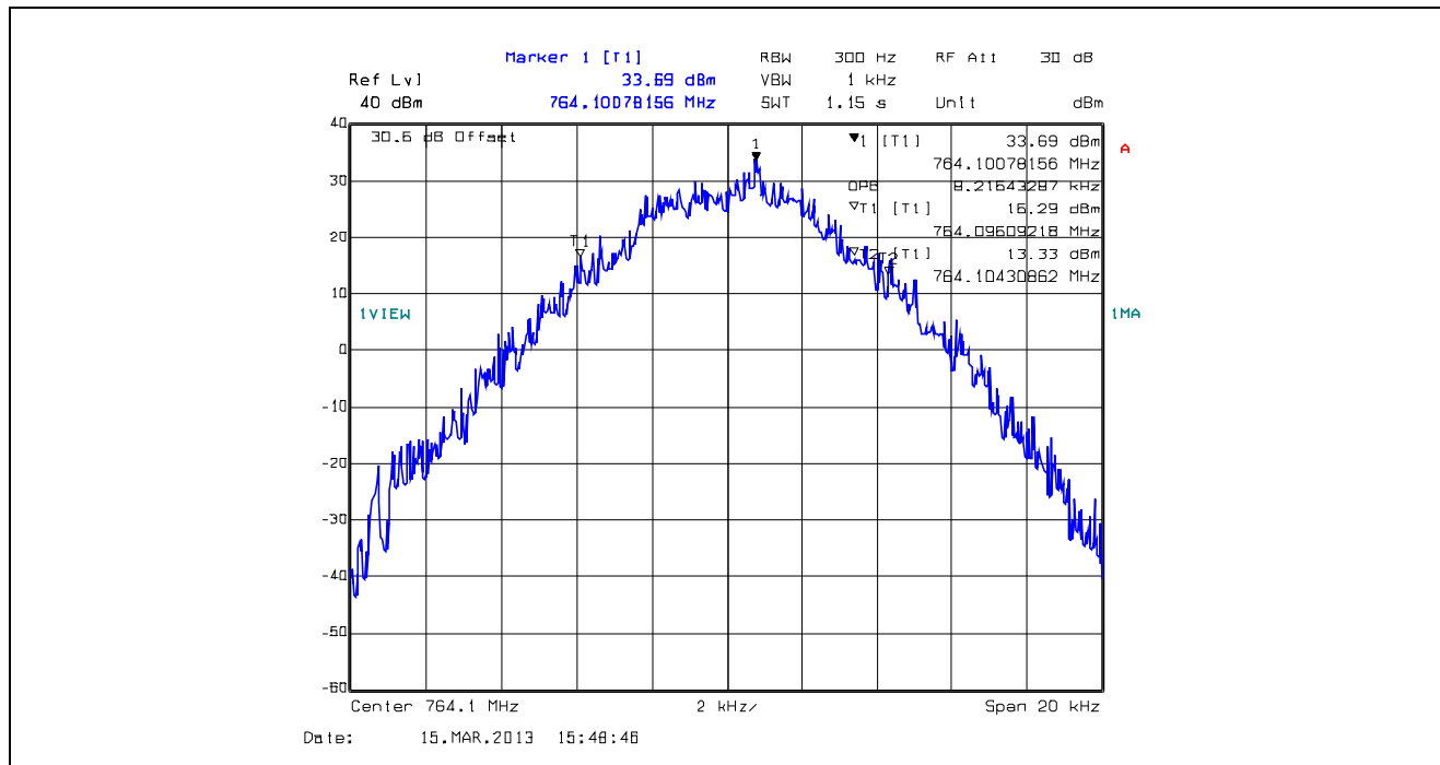
Plot 5.4.4.1.23. 99% Occupied Bandwidth, 12.5 kHz Channel Spacing, F1D, 764.1 MHz
