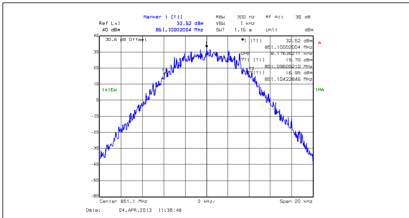
Plot 5.4.4.1.71. 99% Occupied Bandwidth, 12.5 kHz Channel Spacing, F1W, 851.1 MHz
