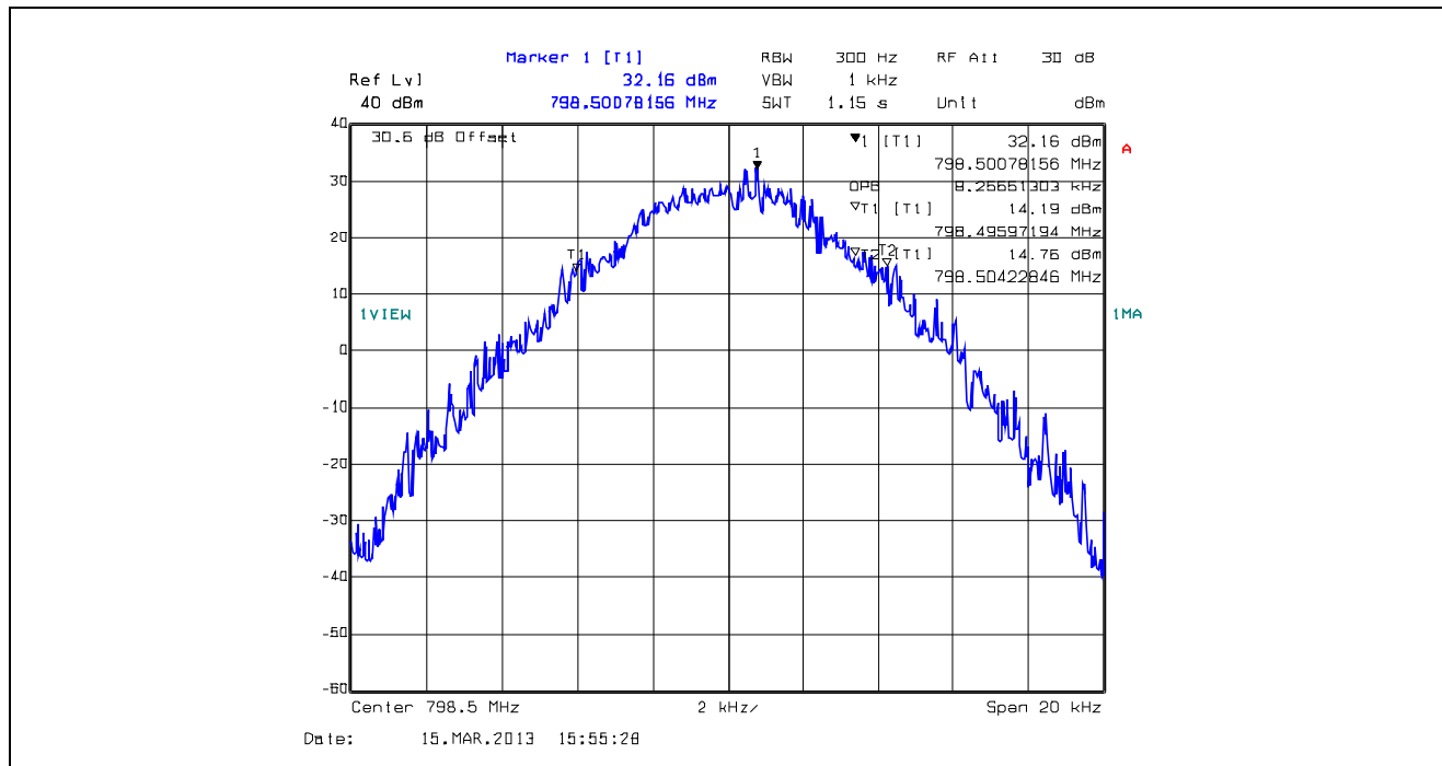
Plot 5.4.4.1.39. 99% Occupied Bandwidth, 12.5 kHz Channel Spacing, F1D, 798.5 MHz
