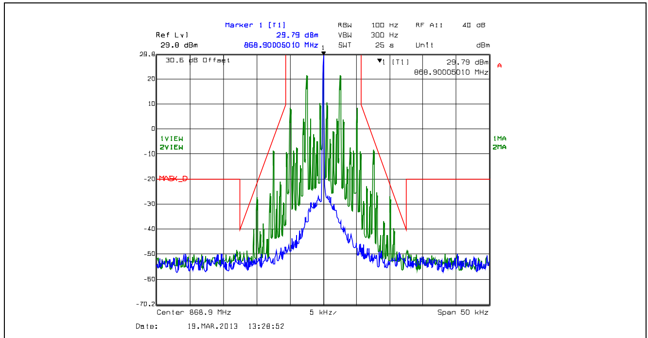
Plot 5.4.4.2.62. Emission Mask D, 12.5 kHz Channel Spacing, F3E, Low Power, 868.9 MHz
