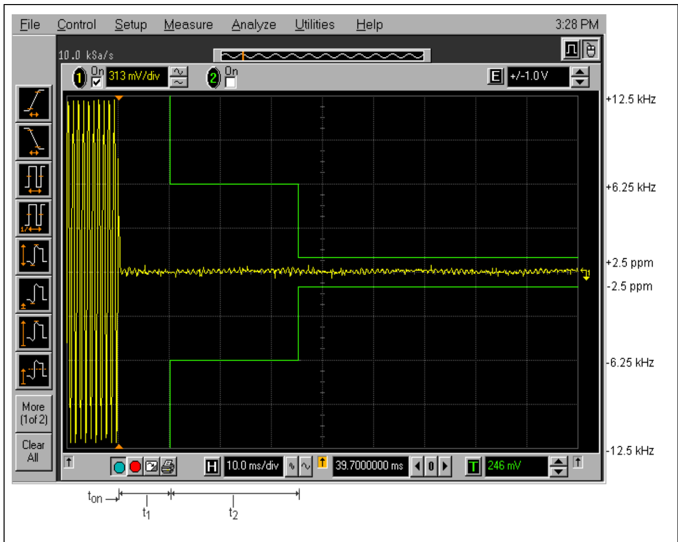
Plot 5.8.4.1. Transient Frequency Behavior on 12.5 kHz Channels Test Frequency: 406.2 MHz; Power: 5 W; Test Conditions: Switch on condition t_{on} , t_1 , and t_2
