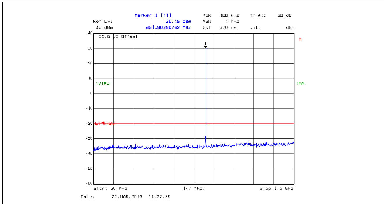
Plot 5.5.4.51. Conducted Transmitter Spurious Emissions, Low Power, 851.1 MHz, 30 MHz - 1.5 GHz
