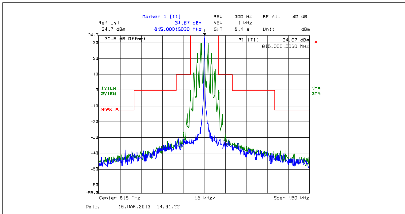
Plot 5.4.4.2.35. Emission Mask B, 25 kHz Channel Spacing, F3E, High Power, 815.0 MHz
