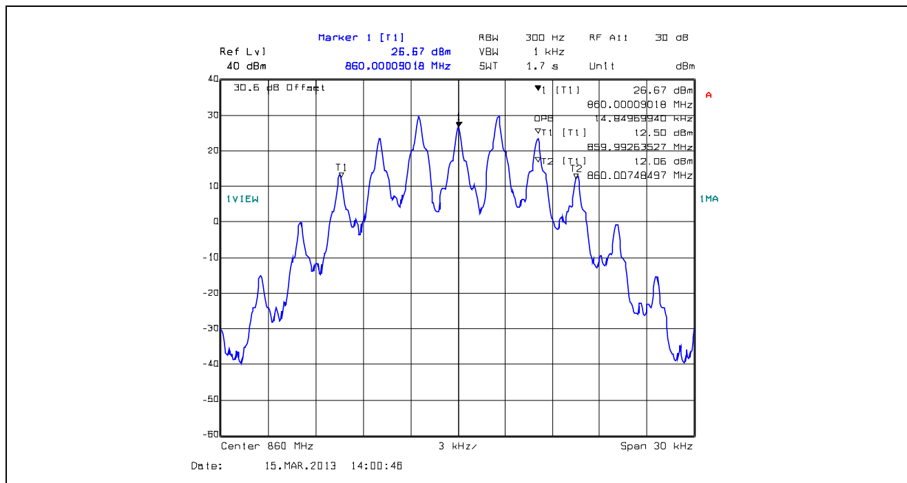
Plot 5.4.4.1.63. 99% Occupied Bandwidth, 25 kHz Channel Spacing, F3E, 860.0 MHz
