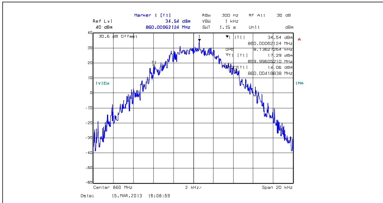
Plot 5.4.4.1.69. 99% Occupied Bandwidth, 12.5 kHz Channel Spacing, F1D, 860.0 MHz
