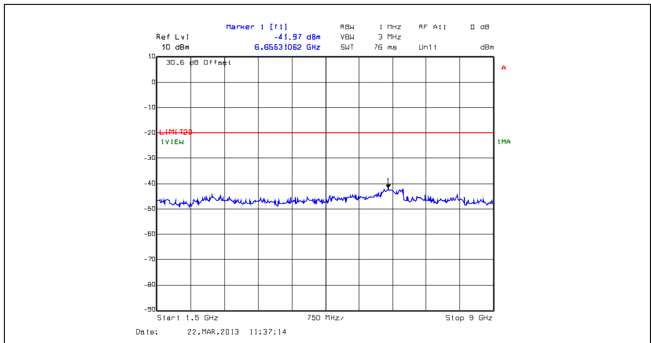
Plot 5.5.4.48. Conducted Transmitter Spurious Emissions, Low Power, 823.9 MHz, 1.5 GHz - 9 GHz
