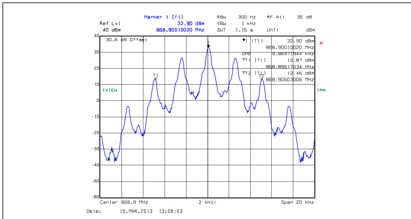
Plot 5.4.4.1.61. 99% Occupied Bandwidth, 12.5 kHz Channel Spacing, F3E, 868.9 MHz
