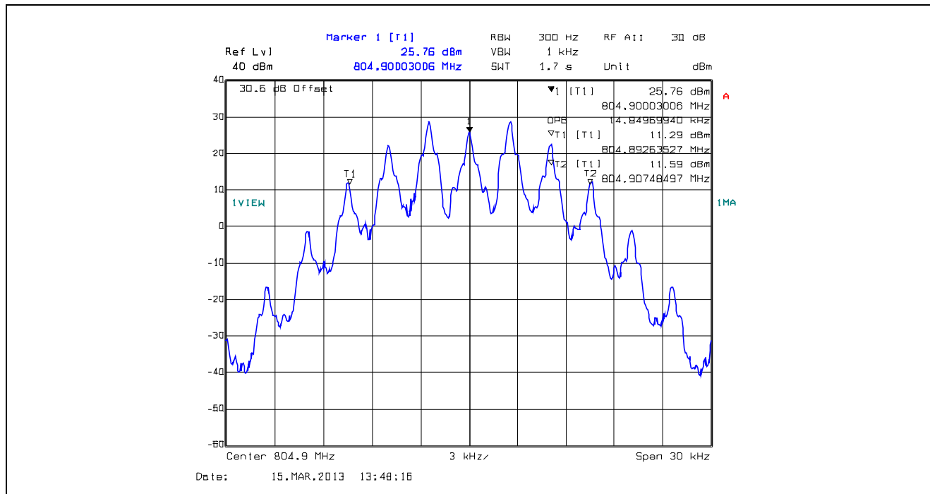
Plot 5.4.4.1.34. 99% Occupied Bandwidth, 25 kHz Channel Spacing, F3E, 804.9 MHz
