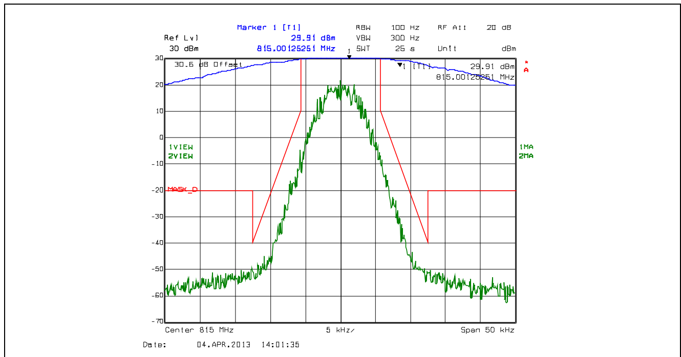
Plot 5.4.4.2.54. Emission Mask D, 12.5 kHz Channel Spacing, F1W, Low Power, 815.0 MHz
