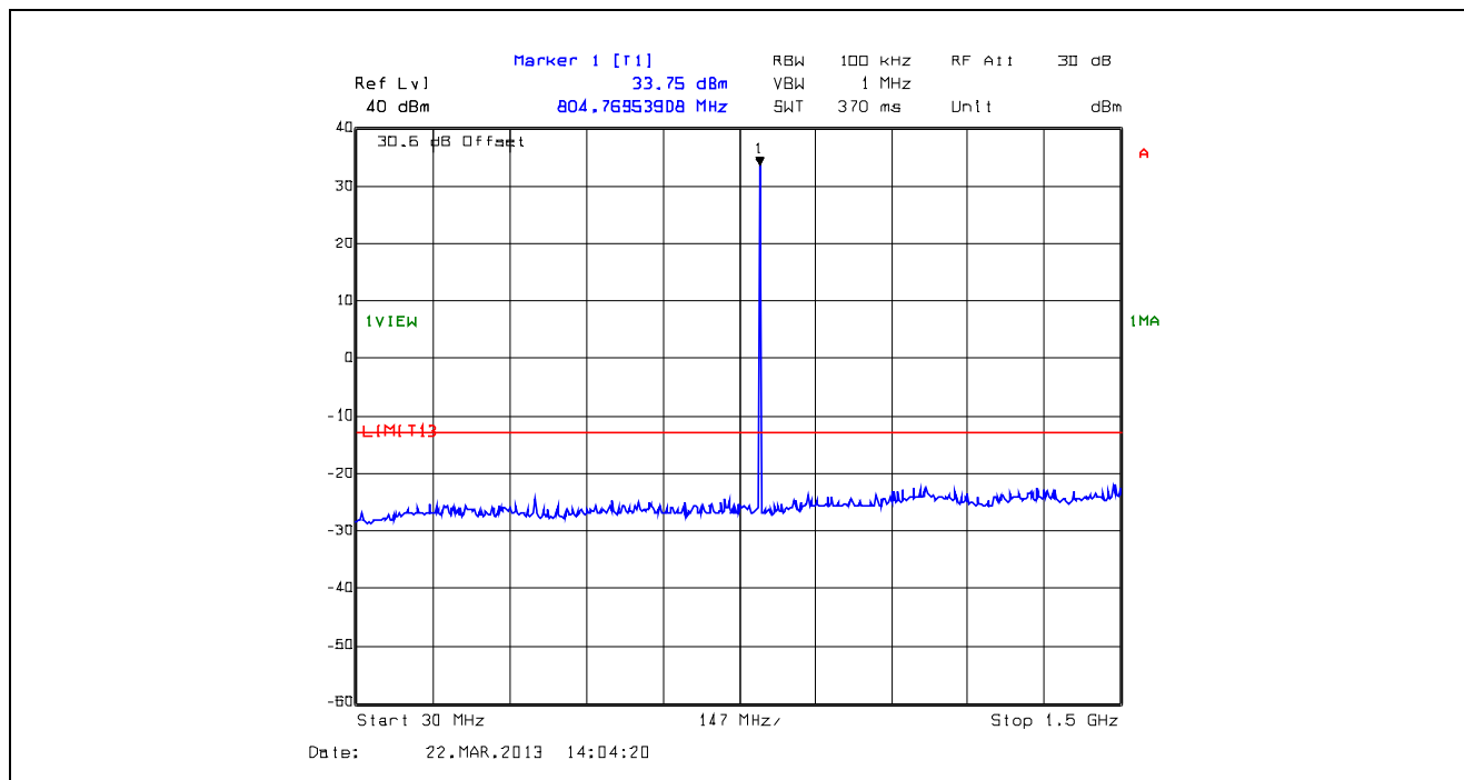
Plot 5.5.4.33. Conducted Transmitter Spurious Emissions, High Power, 804.9 MHz, 30 MHz - 1.5 GHz
