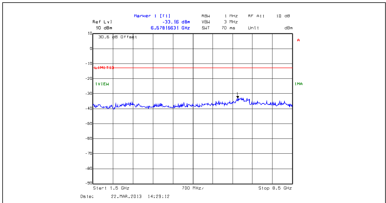
Plot 5.5.4.18. Conducted Transmitter Spurious Emissions, High Power, 769.5 MHz, 1.5 GHz - 8.5 GHz
