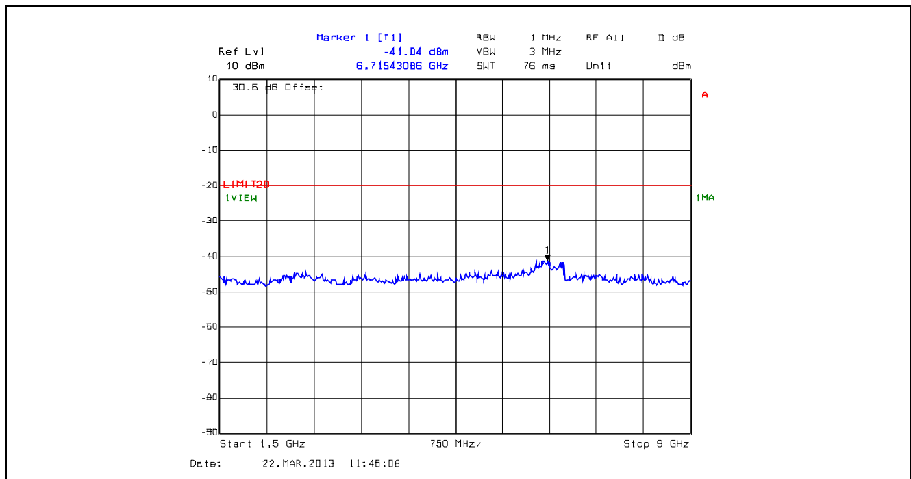
Plot 5.5.4.46. Conducted Transmitter Spurious Emissions, High Power, 823.9 MHz, 1.5 GHz - 9 GHz
