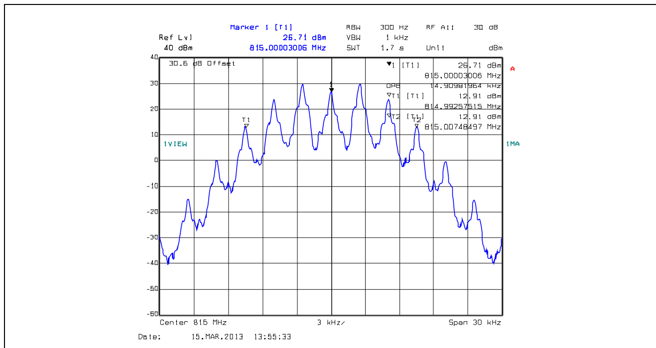
Plot 5.4.4.1.48. 99% Occupied Bandwidth, 25 kHz Channel Spacing, F3E, 815.0MHz
