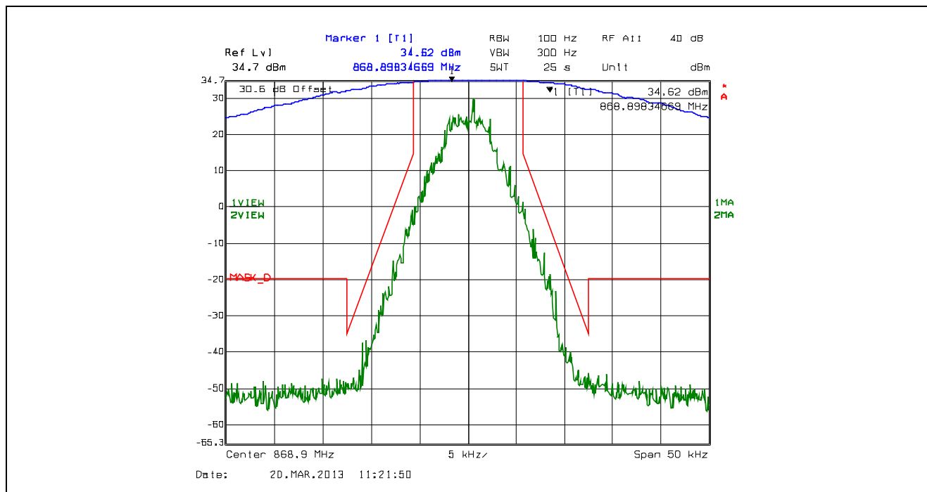
Plot 5.4.4.2.79. Emission Mask D, 12.5 kHz Channel Spacing, F1D, High Power, 868.9 MHz
