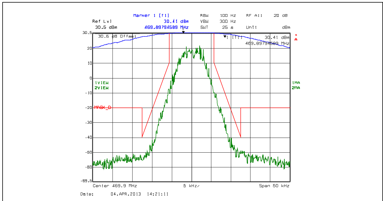
Plot 5.4.4.2.26. Emission Mask D, 12.5 kHz Channel Spacing, F1W, Low Power, 469.9 MHz
