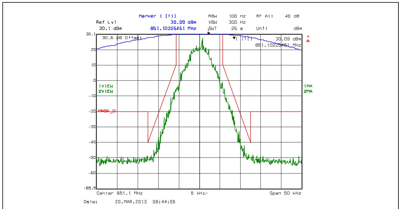
Plot 5.4.4.2.70. Emission Mask D, 12.5 kHz Channel Spacing, F1E, Low Power, 851.1 MHz
