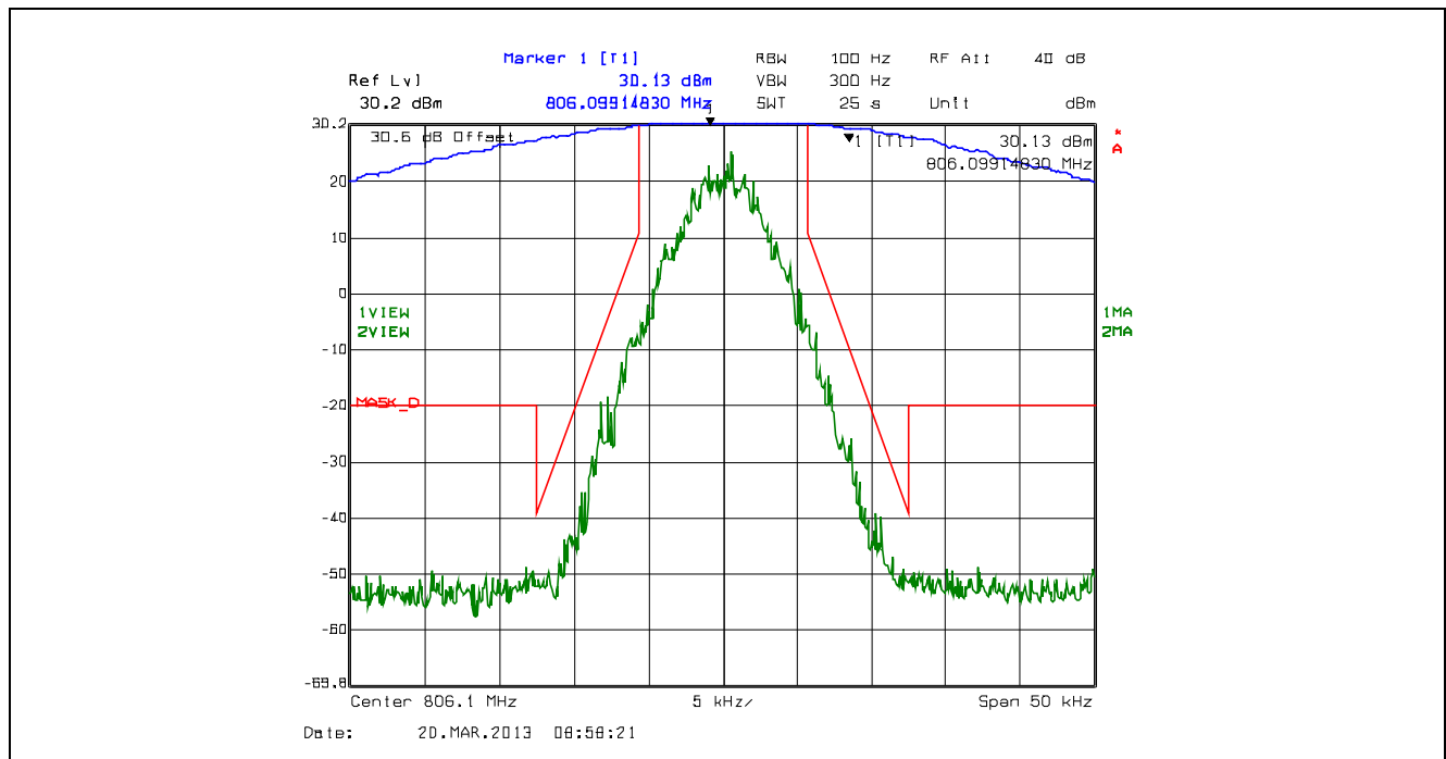
Plot 5.4.4.2.40. Emission Mask D, 12.5 kHz Channel Spacing, F1E, Low Power, 806.1 MHz
