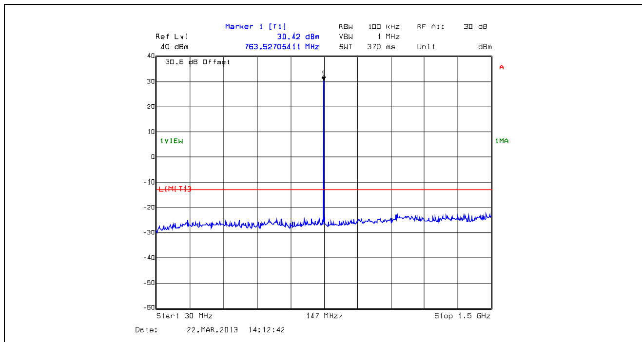
Plot 5.5.4.15. Conducted Transmitter Spurious Emissions, Low Power, 764.1 MHz, 30 MHz - 1.5 GHz
