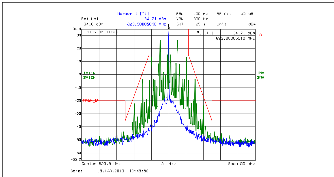
Plot 5.4.4.2.31. Emission Mask D, 12.5 kHz Channel Spacing, F3E, High Power, 823.9 MHz
