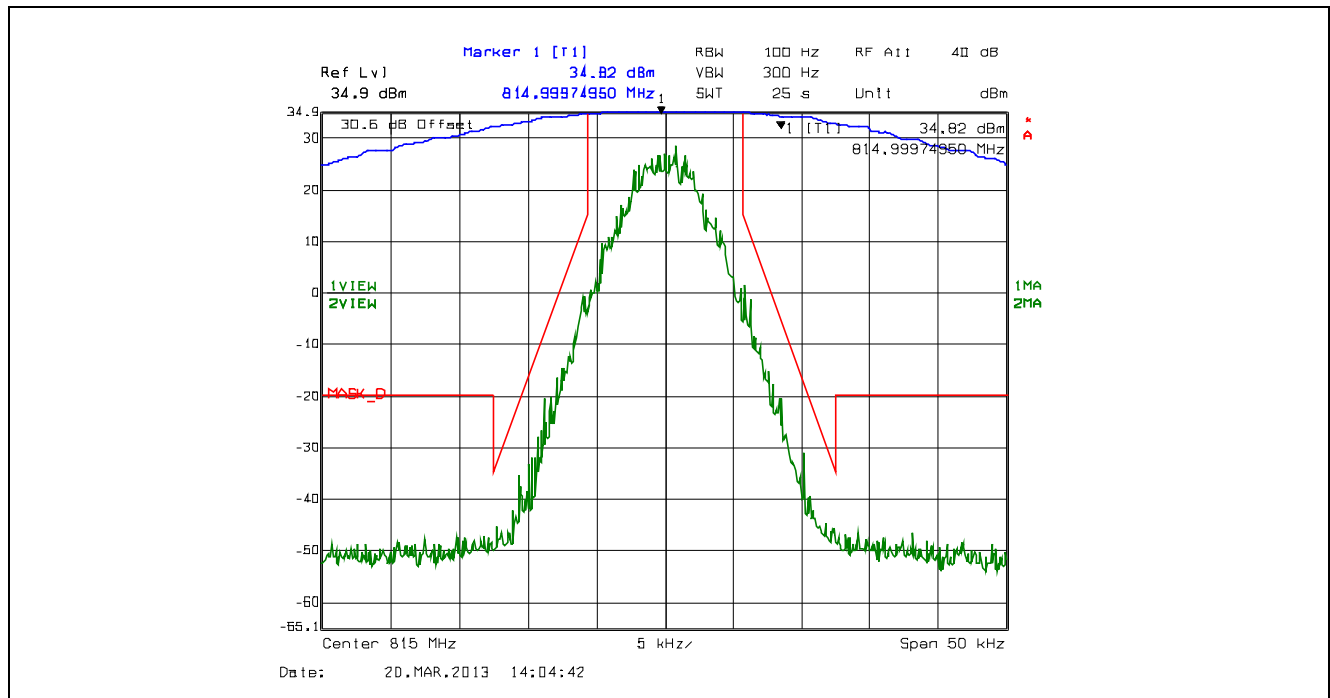
Plot 5.4.4.2.47. Emission Mask D, 12.5 kHz Channel Spacing, F1D, High Power, 815.0 MHz
