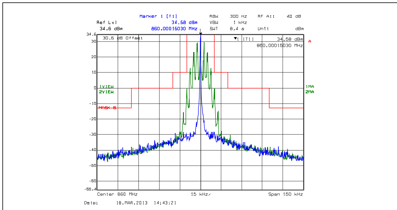
Plot 5.4.4.2.65. Emission Mask B, 25 kHz Channel Spacing, F3E, High Power, 860.0 MHz
