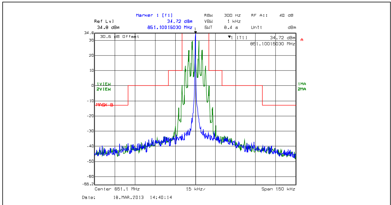
Plot 5.4.4.2.63. Emission Mask B, 25 kHz Channel Spacing, F3E, High Power, 851.1 MHz
