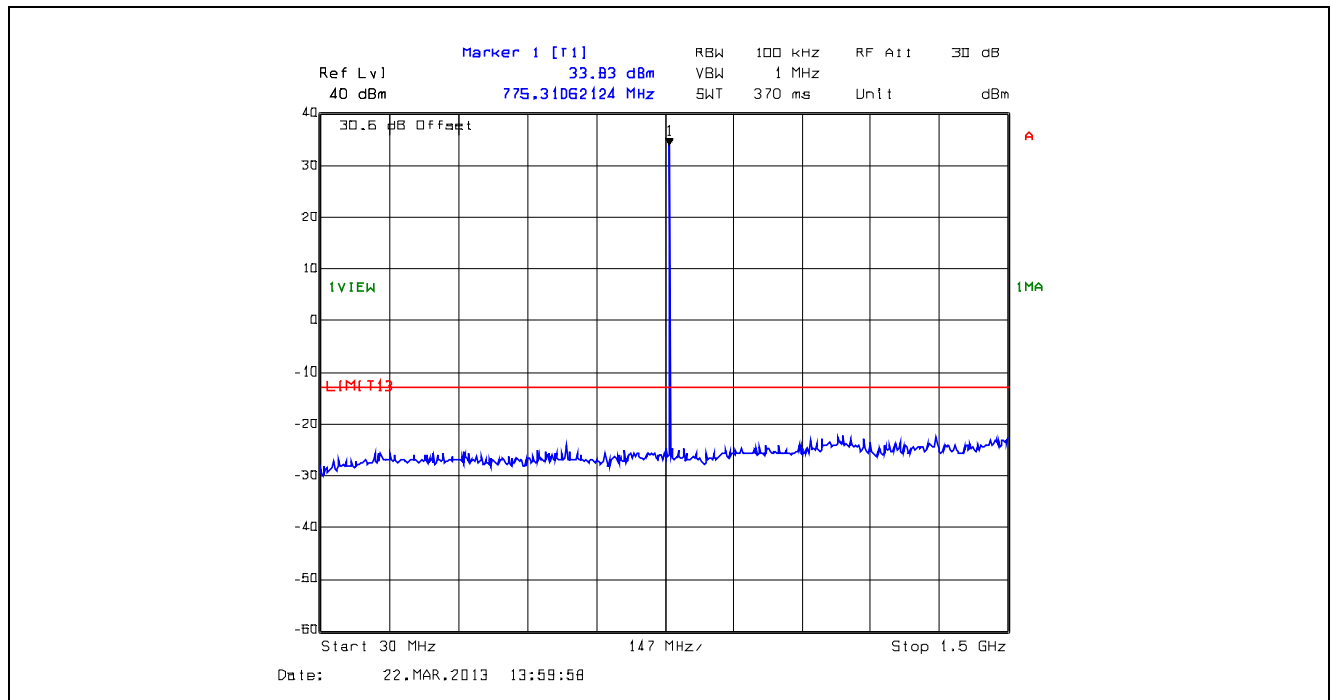
Plot 5.5.4.21. Conducted Transmitter Spurious Emissions, High Power, 774.9 MHz, 30 MHz - 1.5 GHz
