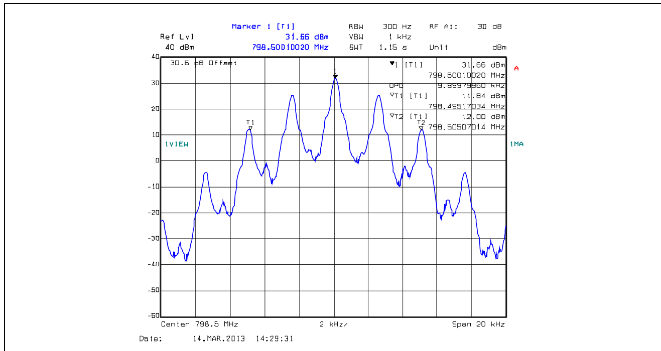
Plot 5.4.4.1.30. 99% Occupied Bandwidth, 12.5 kHz Channel Spacing, F3E, 798.5 MHz
