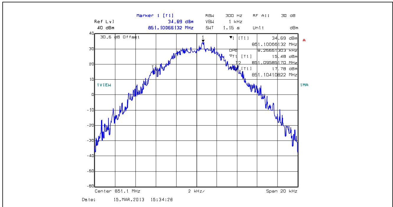
Plot 5.4.4.1.65. 99% Occupied Bandwidth, 12.5 kHz Channel Spacing, F1E, 851.1 MHz
