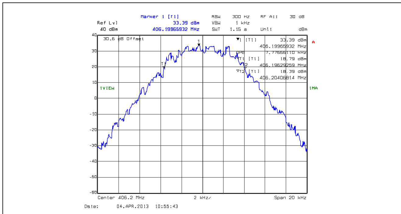
Plot 5.4.4.1.11. 99% Occupied Bandwidth, 12.5 kHz Channel Spacing, F1W, 406.2 MHz
