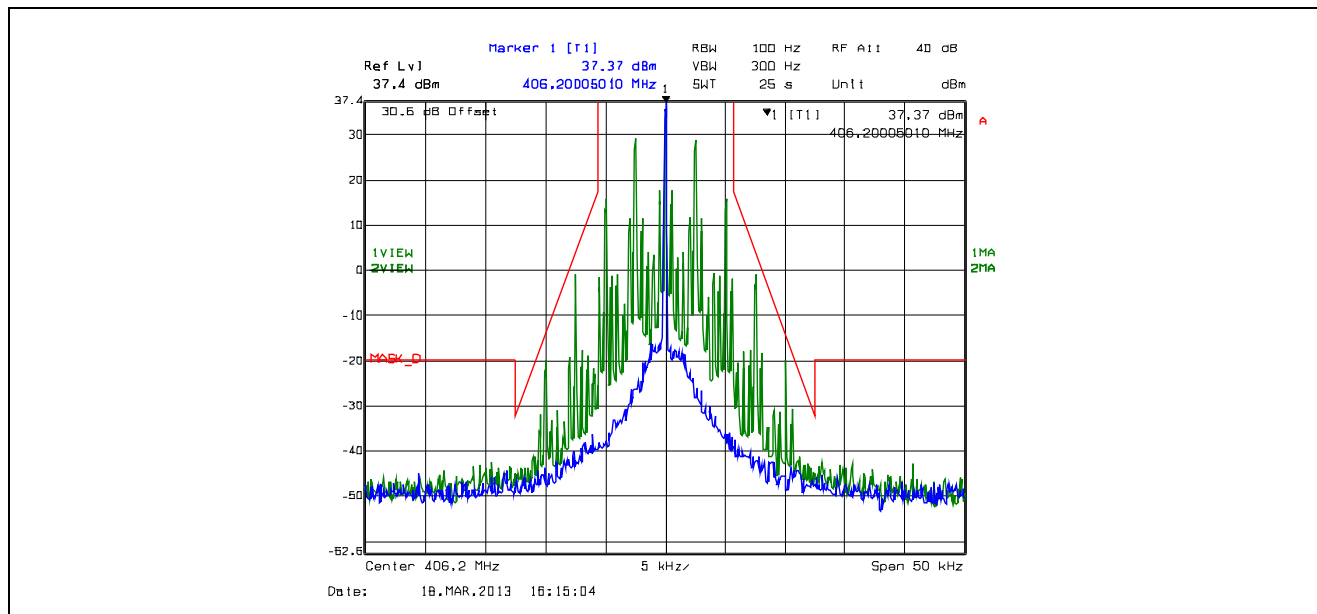
Plot 5.4.4.2.1. Emission Mask D, 12.5 kHz Channel Spacing, F3E, High Power, 406.2 MHz
