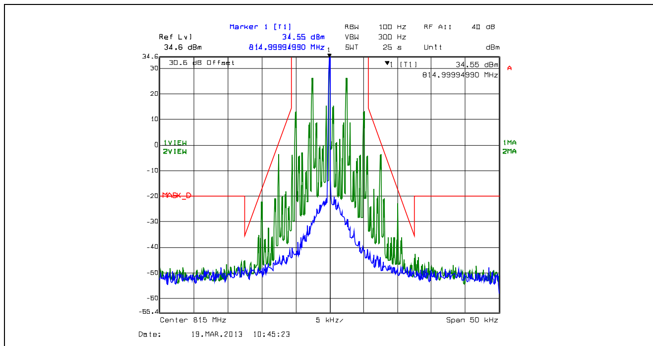
Plot 5.4.4.2.29. Emission Mask D, 12.5 kHz Channel Spacing, F3E, High Power, 815.0 MHz
