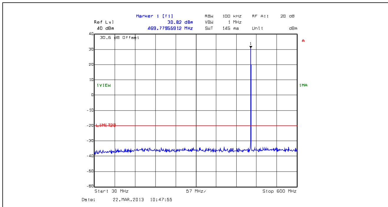
Plot 5.5.4.11. Conducted Transmitter Spurious Emissions, Low Power, 469.9 MHz, 30 MHz - 600 MHz
