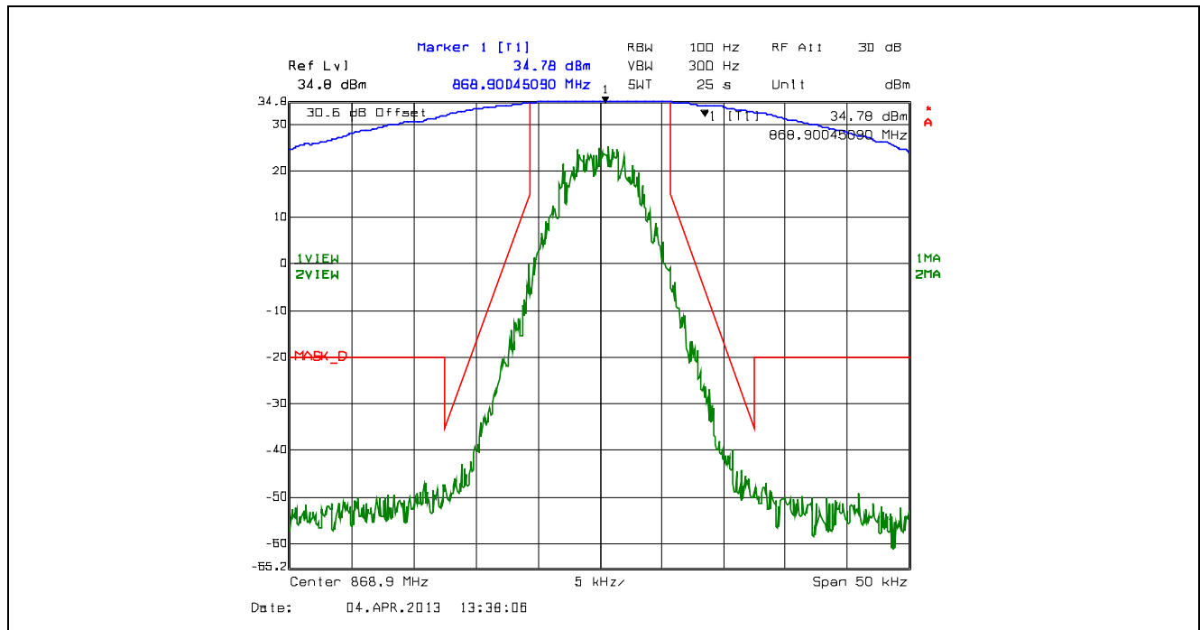
Plot 5.4.4.2.85. Emission Mask D, 12.5 kHz Channel Spacing, F1W, High Power, 868.9 MHz
