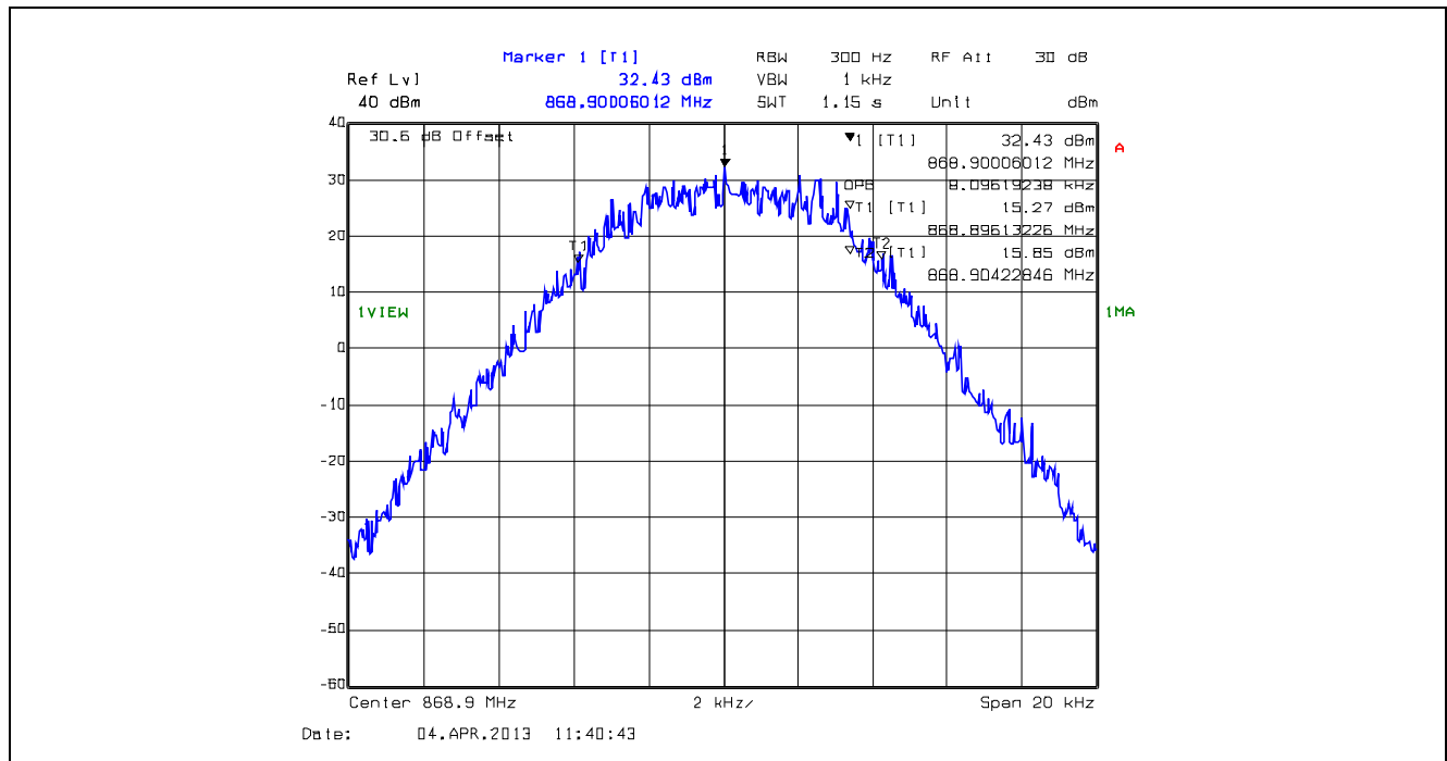
Plot 5.4.4.1.73. 99% Occupied Bandwidth, 12.5 kHz Channel Spacing, F1W, 868.9 MHz
