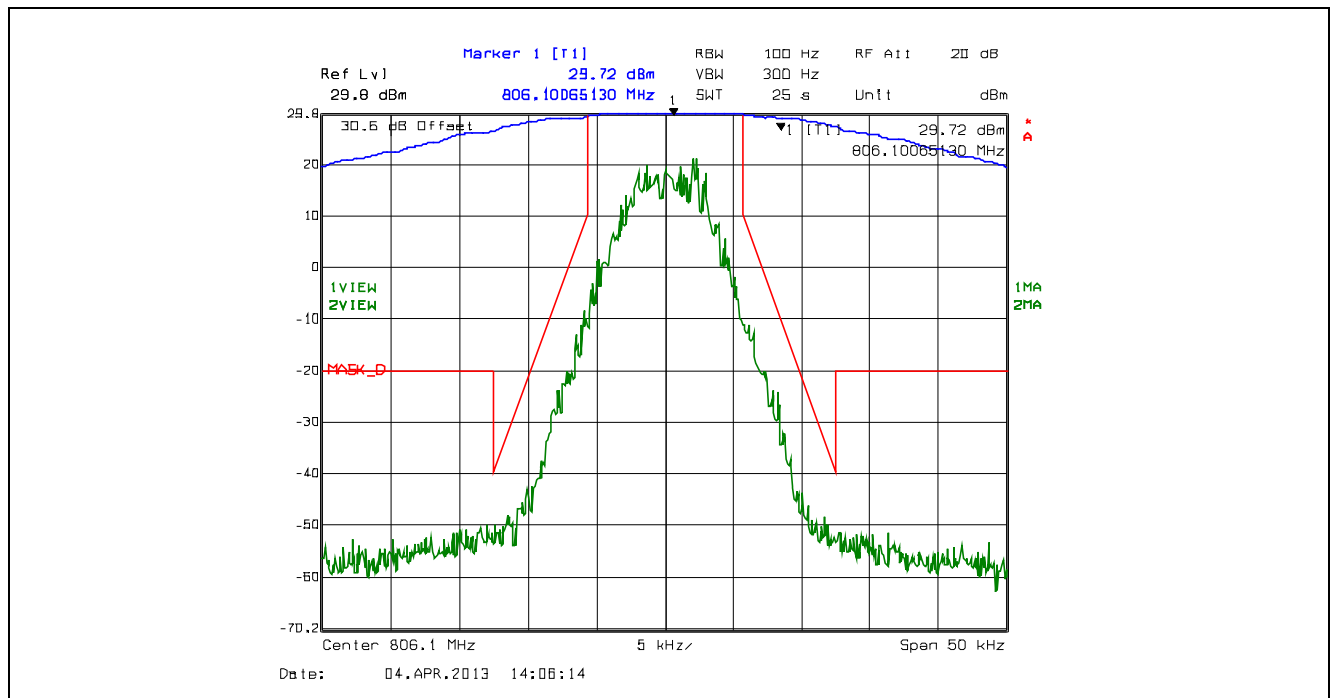
Plot 5.4.4.2.52. Emission Mask D, 12.5 kHz Channel Spacing, F1W, Low Power, 806.1 MHz
