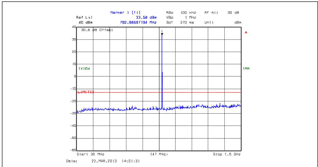
Plot 5.5.4.25. Conducted Transmitter Spurious Emissions, High Power, 794.1 MHz, 30 MHz - 1.5 GHz
