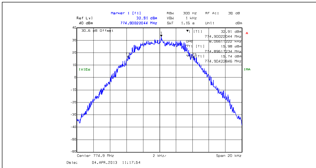
Plot 5.4.4.1.28. 99% Occupied Bandwidth, 12.5 kHz Channel Spacing, F1W, 774.9 MHz
