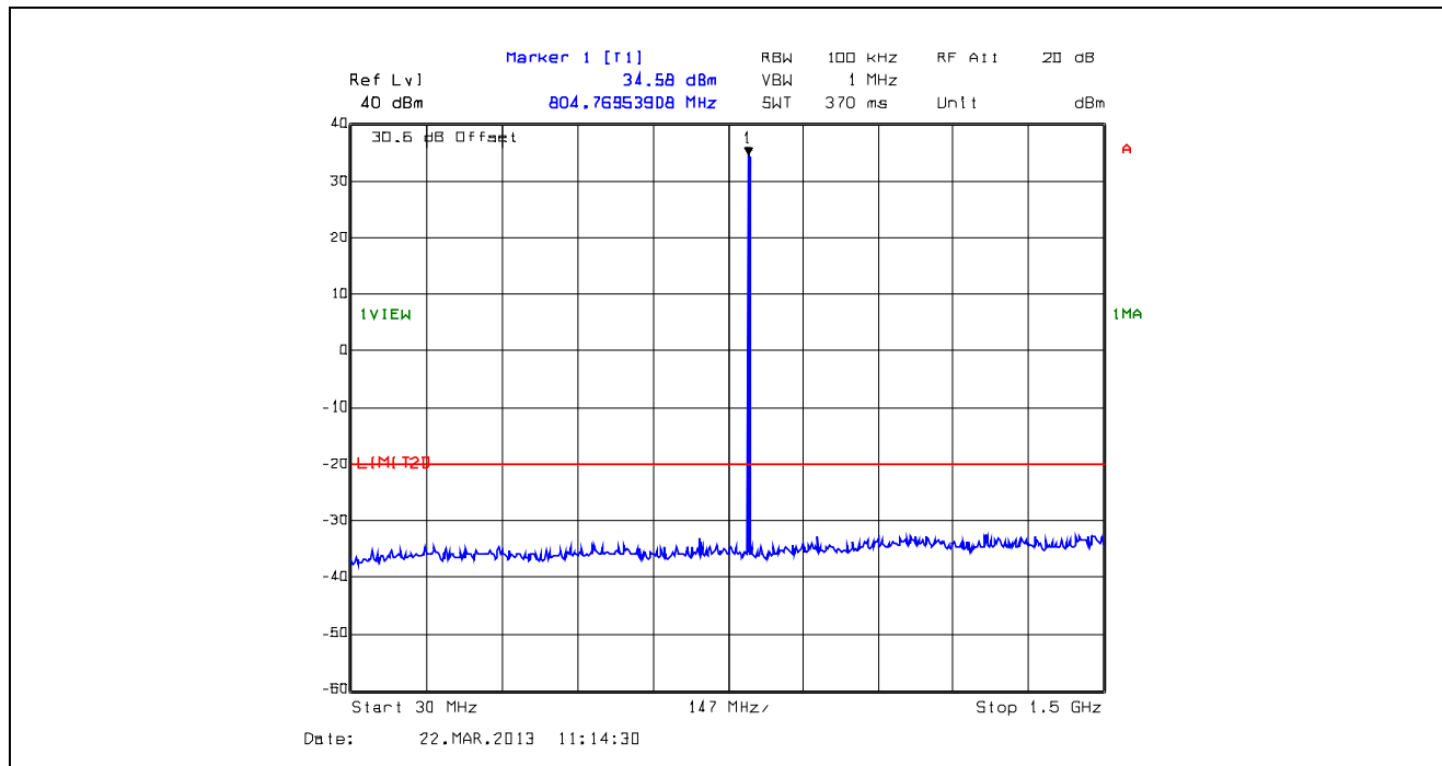
Plot 5.5.4.37. Conducted Transmitter Spurious Emissions, High Power, 806.1 MHz, 30 MHz - 1.5 GHz
