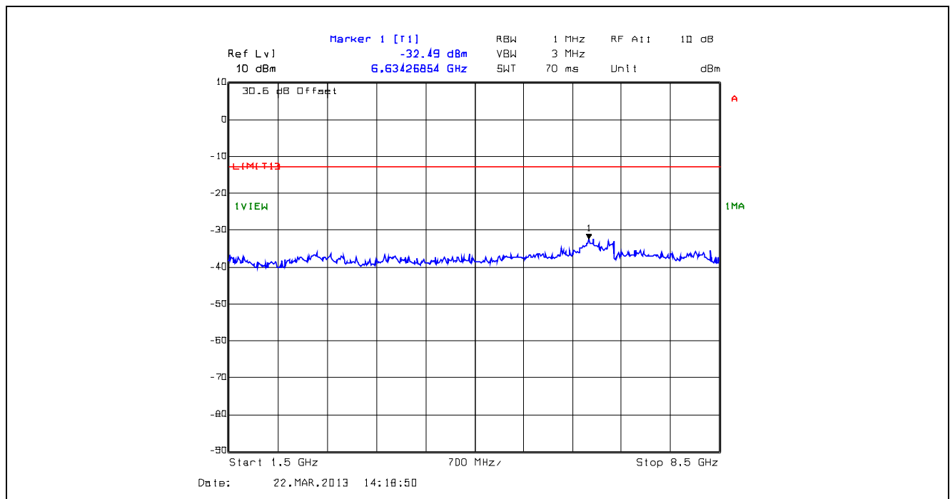
Plot 5.5.4.20. Conducted Transmitter Spurious Emissions, Low Power, 769.5 MHz, 1.5 GHz - 8.5 GHz
