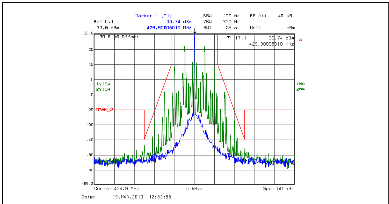
Plot 5.4.4.2.4. Emission Mask D, 12.5 kHz Channel Spacing, F3E, Low Power, 429.9 MHz
