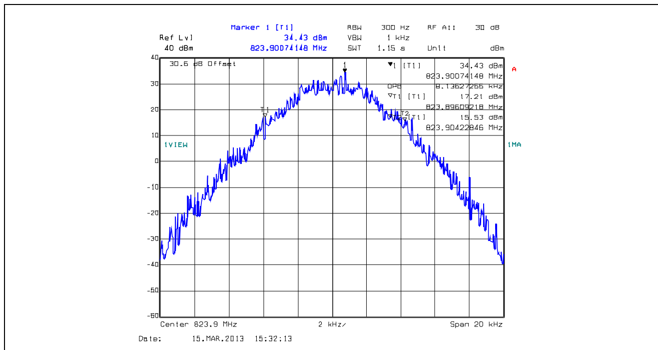
Plot 5.4.4.1.52. 99% Occupied Bandwidth, 12.5 kHz Channel Spacing, F1E, 823.9 MHz
