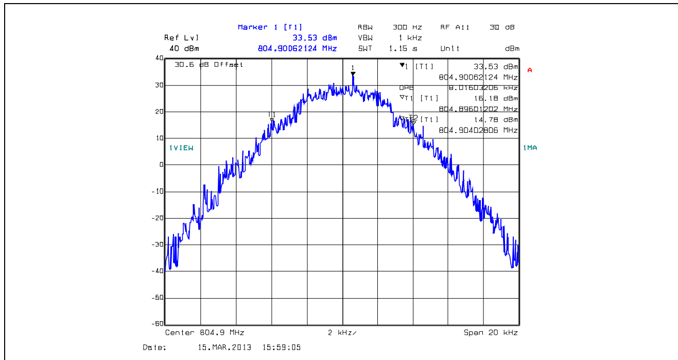
Plot 5.4.4.1.40. 99% Occupied Bandwidth, 12.5 kHz Channel Spacing, F1D, 804.9 MHz
