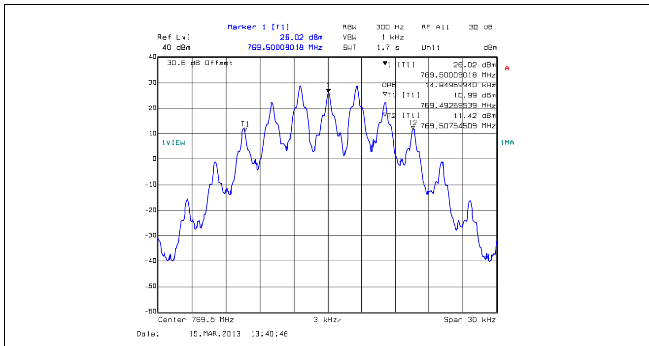
Plot 5.4.4.1.18. 99% Occupied Bandwidth, 25 kHz Channel Spacing, F3E, 769.5MHz
