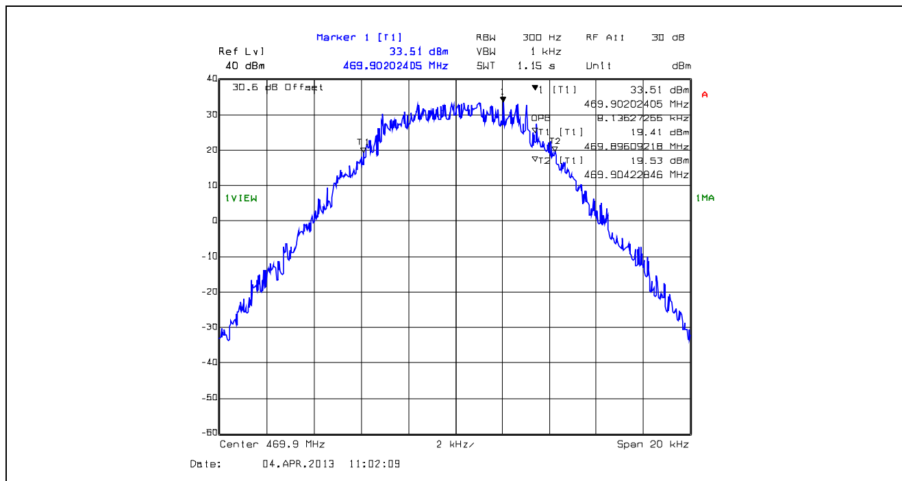
Plot 5.4.4.1.13. 99% Occupied Bandwidth, 12.5 kHz Channel Spacing, F1W, 469.9 MHz
