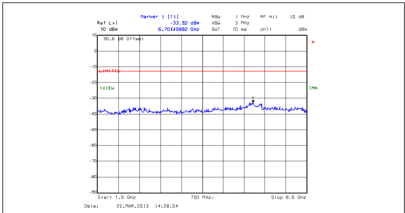
Plot 5.5.4.22. Conducted Transmitter Spurious Emissions, High Power, 774.9 MHz, 1.5 GHz - 8.5 GHz
