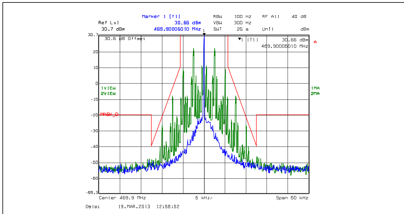
Plot 5.4.4.2.6. Emission Mask D, 12.5 kHz Channel Spacing, F3E, Low Power, 469.9 MHz
