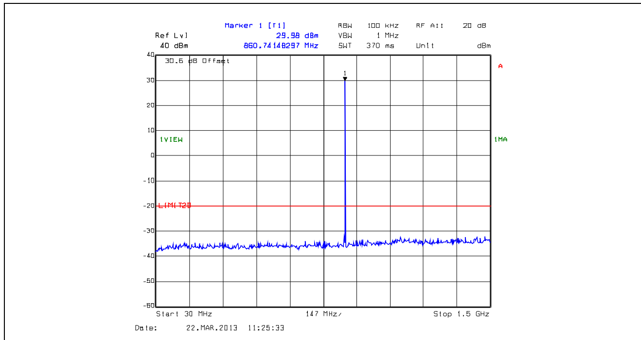
Plot 5.5.4.55. Conducted Transmitter Spurious Emissions, Low Power, 860.0 MHz, 30 MHz - 1.5 GHz
