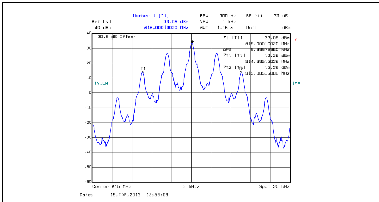
Plot 5.4.4.1.45. 99% Occupied Bandwidth, 12.5 kHz Channel Spacing, F3E, 815.0 MHz
