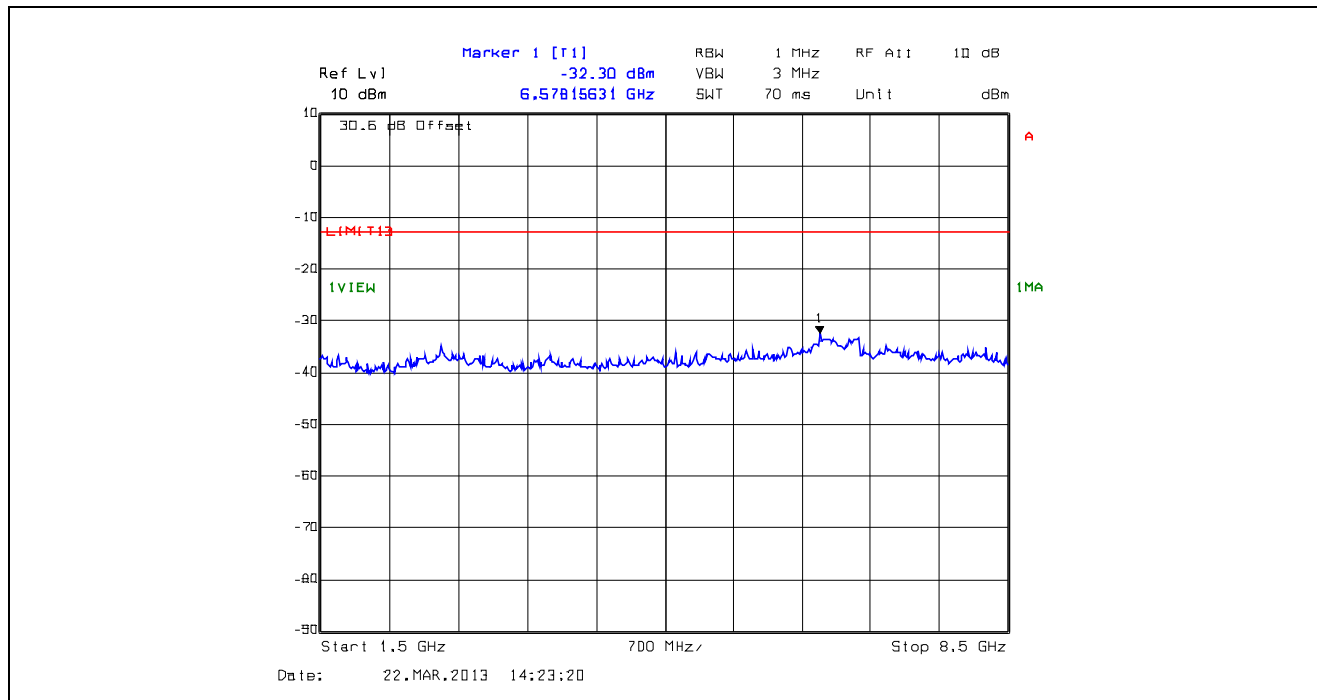
Plot 5.5.4.36. Conducted Transmitter Spurious Emissions, Low Power, 804.9 MHz, 1.5 GHz - 8.5 GHz
