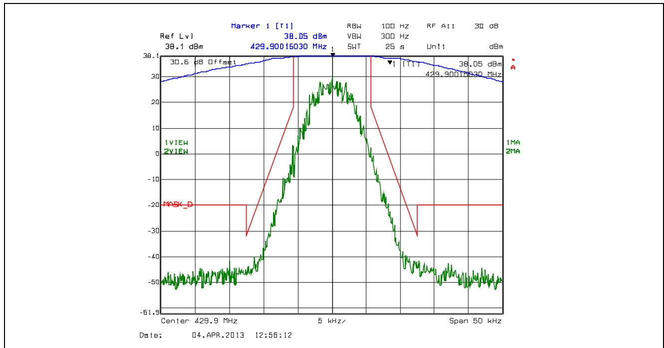
Plot 5.4.4.2.23. Emission Mask D, 12.5 kHz Channel Spacing, F1W, High Power, 429.9 MHz
