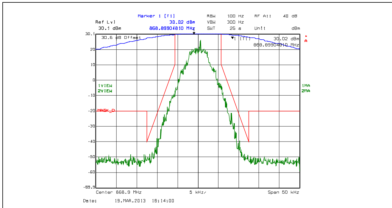
Plot 5.4.4.2.74. Emission Mask D, 12.5 kHz Channel Spacing, F1E, Low Power, 868.9 MHz
