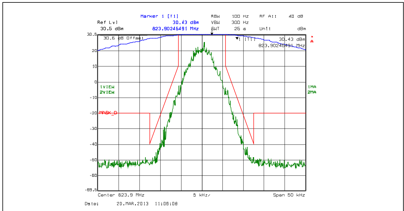
Plot 5.4.4.2.50. Emission Mask D, 12.5 kHz Channel Spacing, F1D, Low Power, 823.9 MHz
