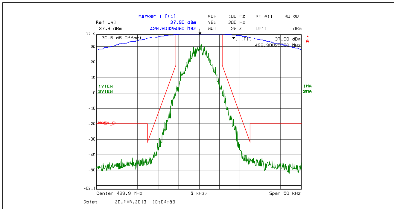
Plot 5.4.4.2.11. Emission Mask D, 12.5 kHz Channel Spacing, F1E, High Power, 429.9 MHz
