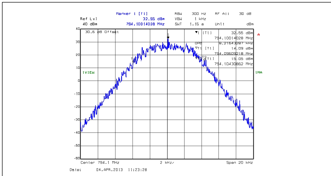
Plot 5.4.4.1.41. 99% Occupied Bandwidth, 12.5 kHz Channel Spacing, F1W, 794.1 MHz
