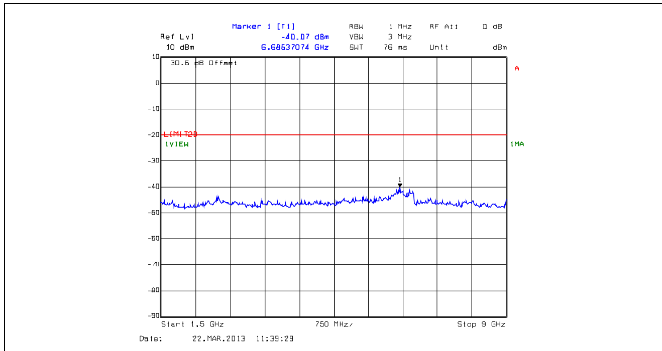
Plot 5.5.4.56. Conducted Transmitter Spurious Emissions, Low Power, 860.0 MHz, 1.5 GHz - 9 GHz
