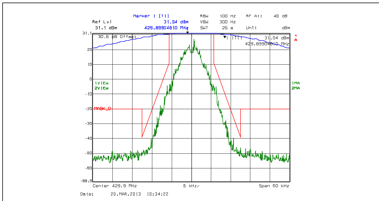
Plot 5.4.4.2.18. Emission Mask D, 12.5 kHz Channel Spacing, F1D, Low Power, 429.9 MHz
