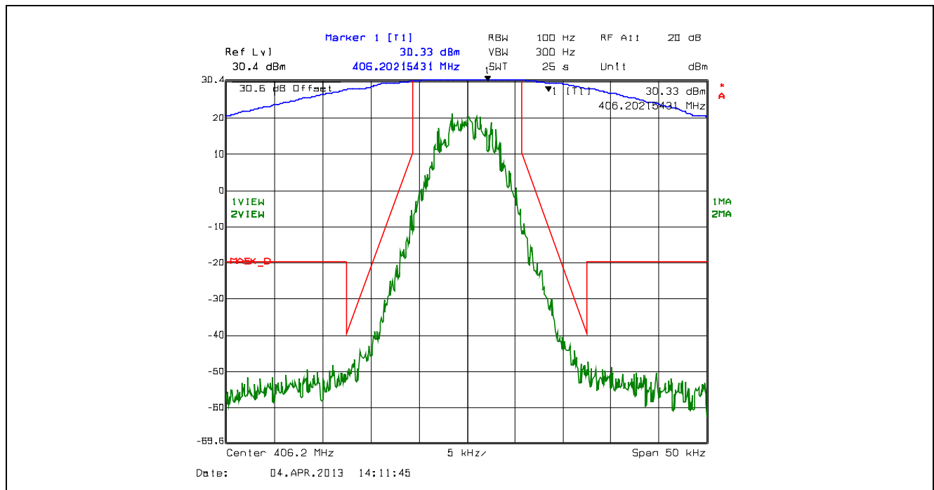
Plot 5.4.4.2.22. Emission Mask D, 12.5 kHz Channel Spacing, F1W, Low Power, 406.2 MHz
