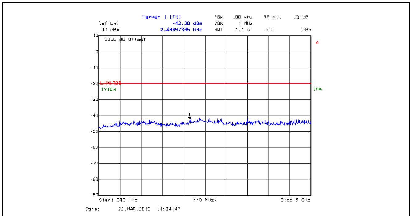
Plot 5.5.4.8. Conducted Transmitter Spurious Emissions, Low Power, 429.9 MHz, 600 MHz -5 GHz
