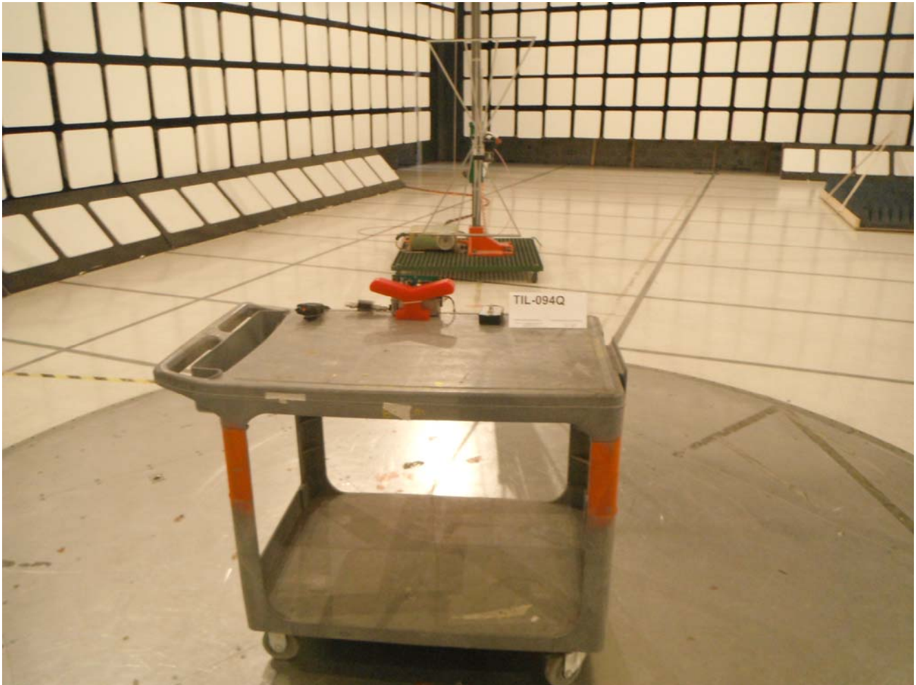
Radiated Emissions at 3 m, 30 - 1000 MHz Orthogonal Position 2
