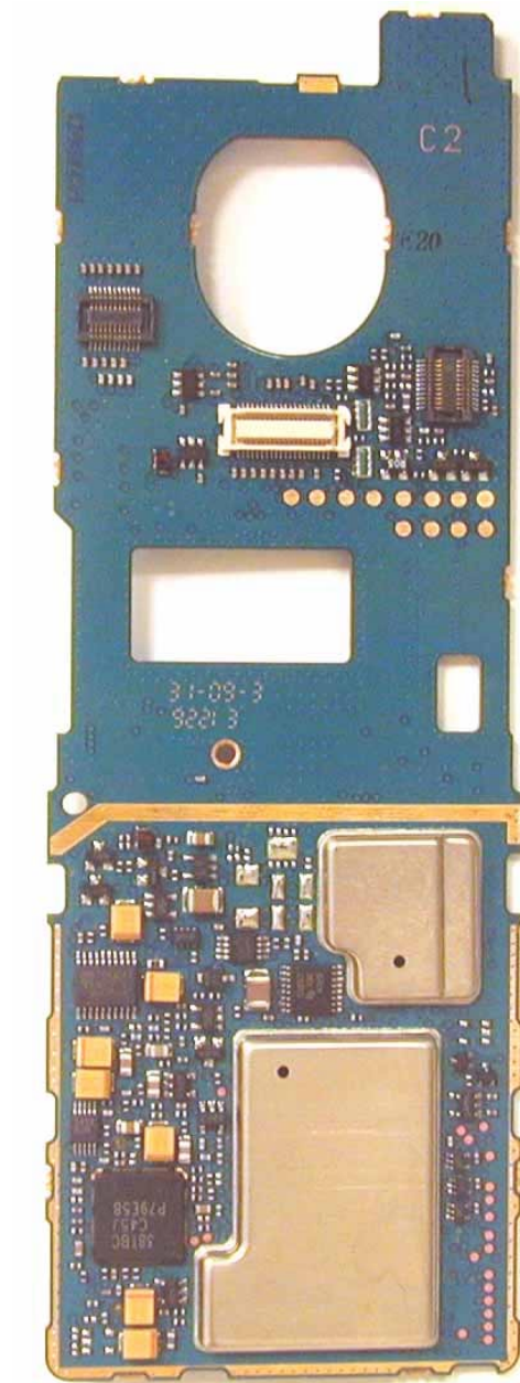
Vocon board with Shields (Top)
