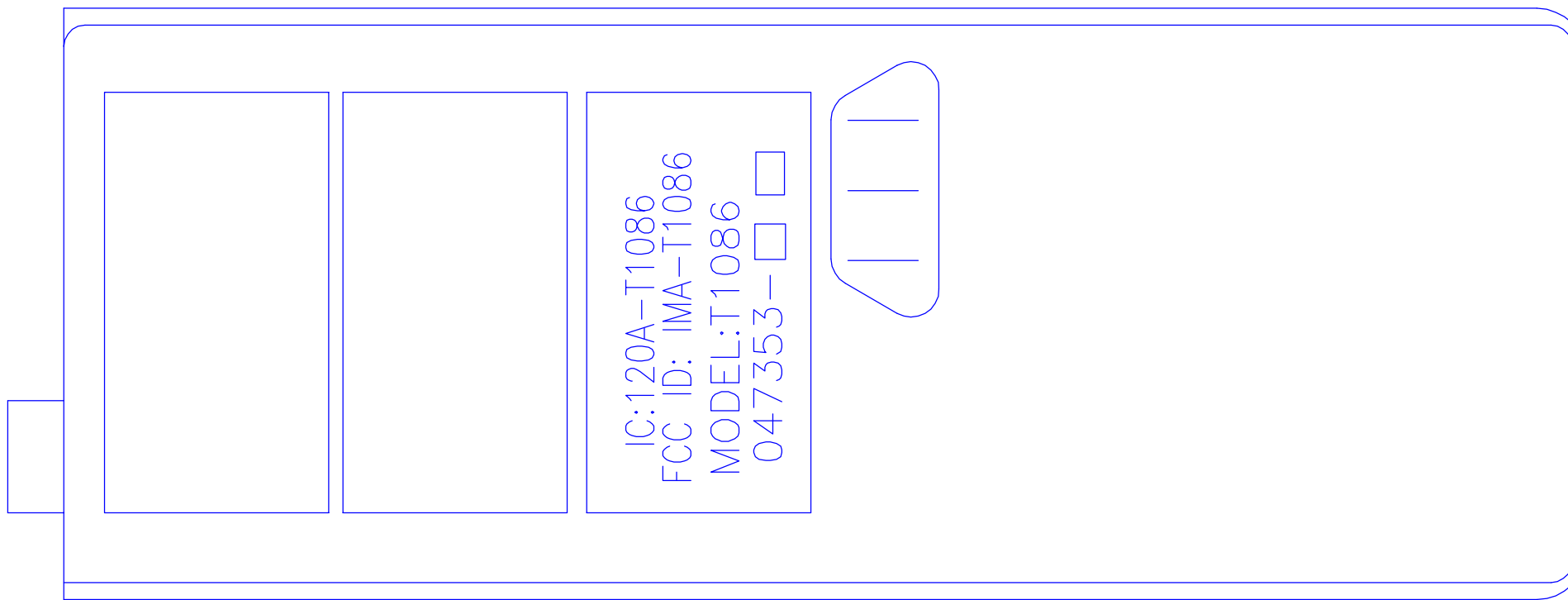
UHF-LO MODULE BOTTOM VIEW
