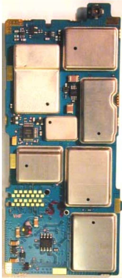
RF board with Shields (Top)
