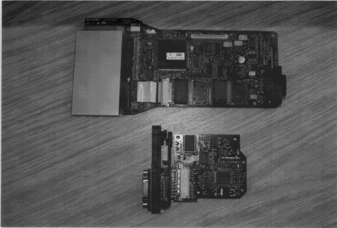
4.5 Component side of the Main Board & RS232/TTL Expansion Board
