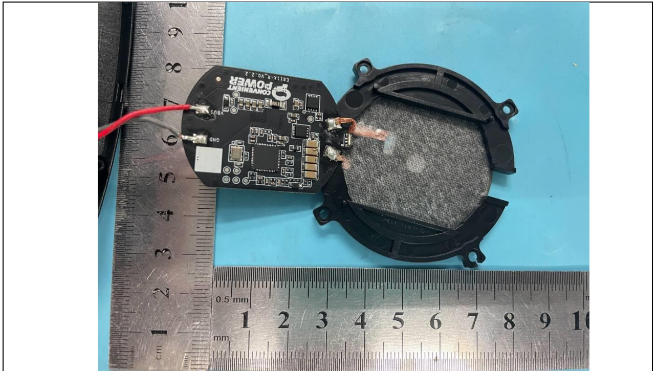
Details of: Wireless charger internal view-3 (Model: MPQ4)
