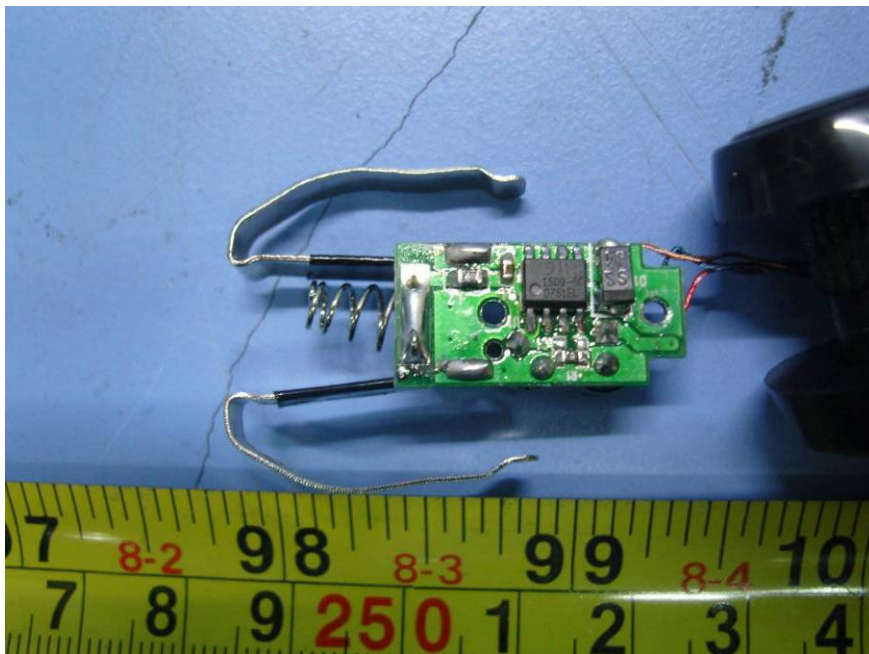
PCB3 - Back View
