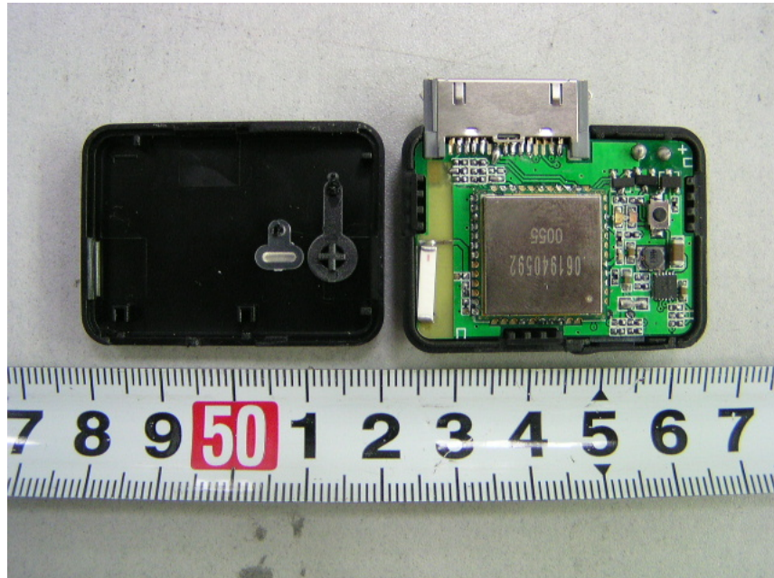
EUT-Inside View
