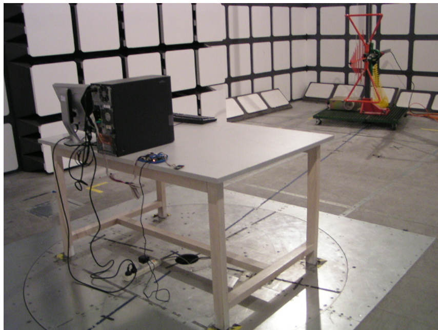
Radiated Emissions - Rear View (30-1000MHz)
