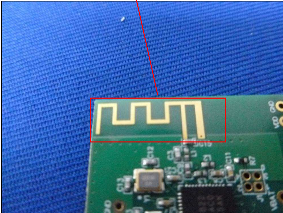
BT_LE Antenna
