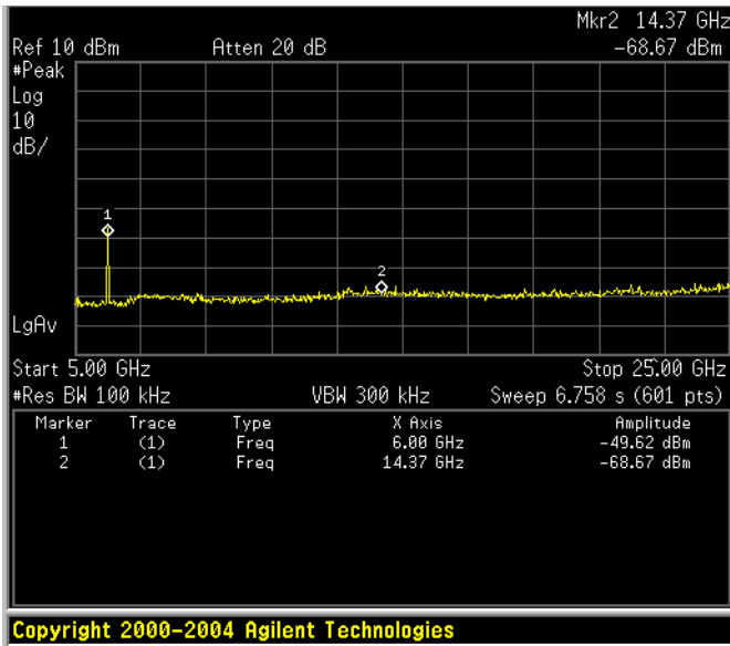
Figure 6.8-3: Conducted Spurious Emissions -3 (5 – 25 GHz) Channel = 2402MHz
