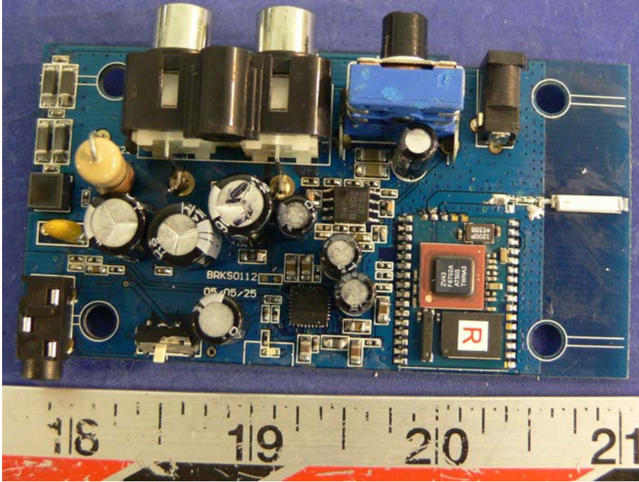
EUT – Sink Main Board Component View
