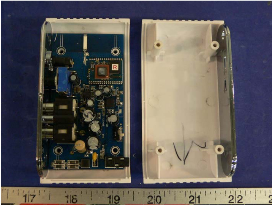
EUT – RX Cover Off View
