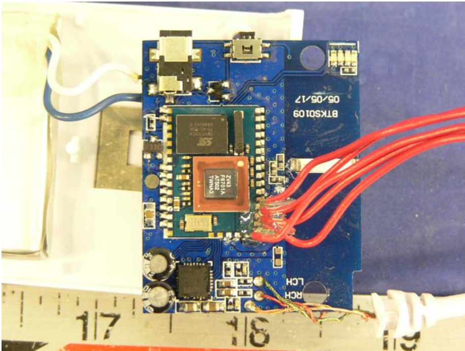
EUT – Source Main Board Component View
