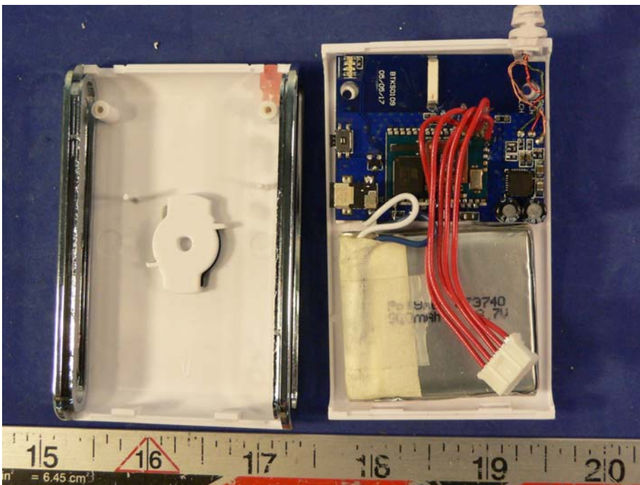
EUT – TX Cover Off View
