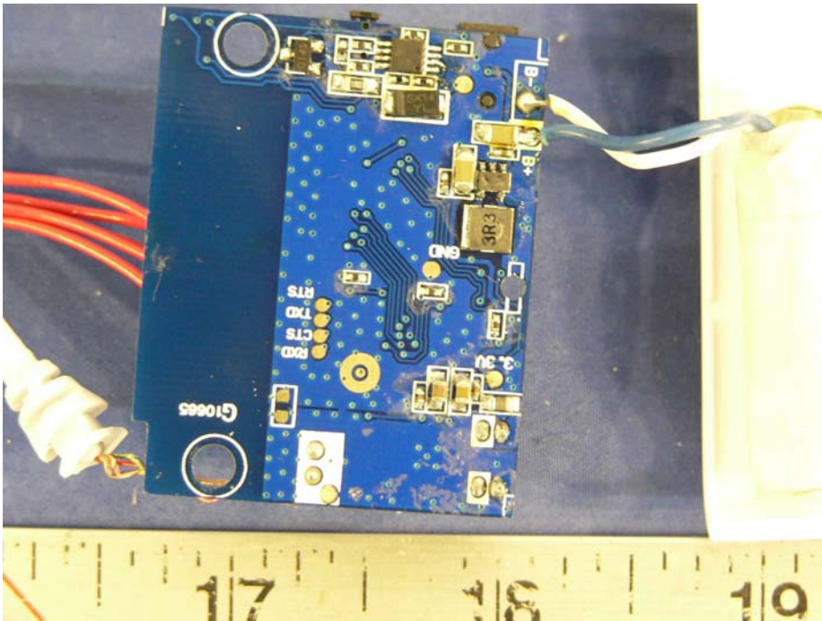
EUT – Source Main Board Solder View
