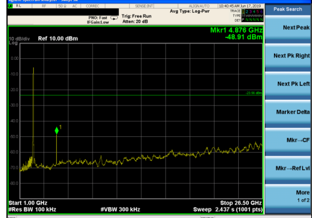
\pi/4 -DQPSK on channel 39
