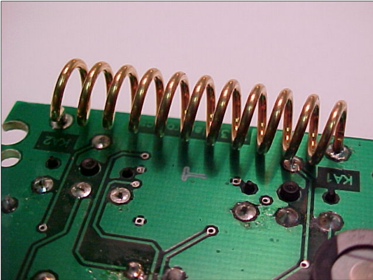
Photo Six – Internal Close-up of Antenna Connection
