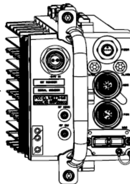
WAP25600 MOTOwi4™ Diversity Access Point @ 2500 MHz Label Diagram
