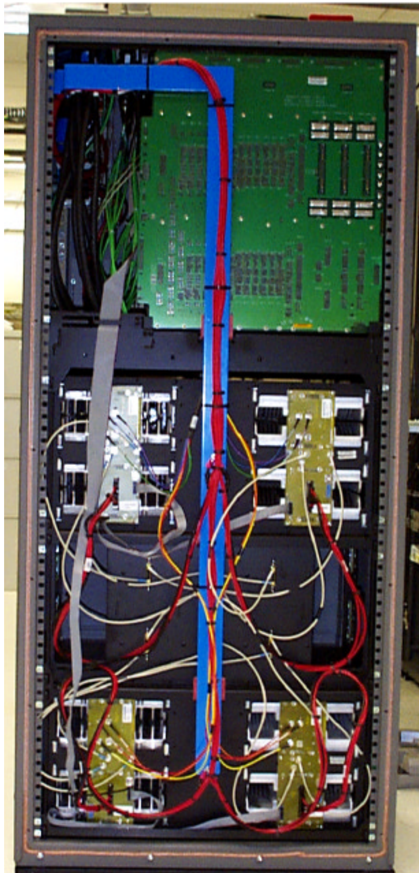
IHET6YR1 SC4812T 1.9 GHz Rear View without Panel
