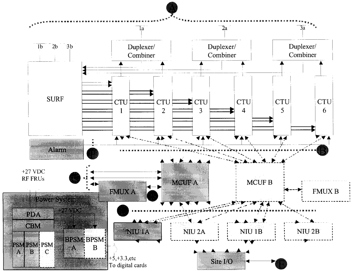
Figure 1 HorizonMacro Hardware Block Diagram
