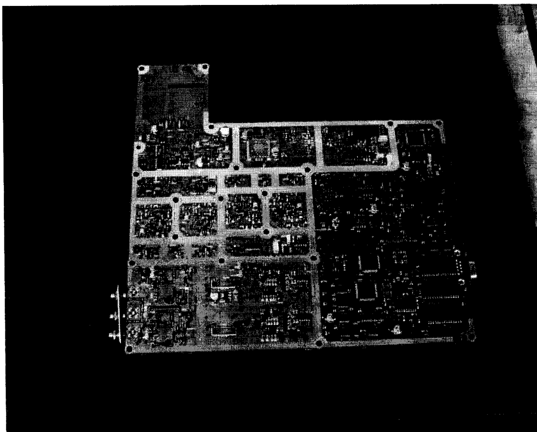
IHET6BV1 HorizonMacro1900 Transceiver Board Front View
