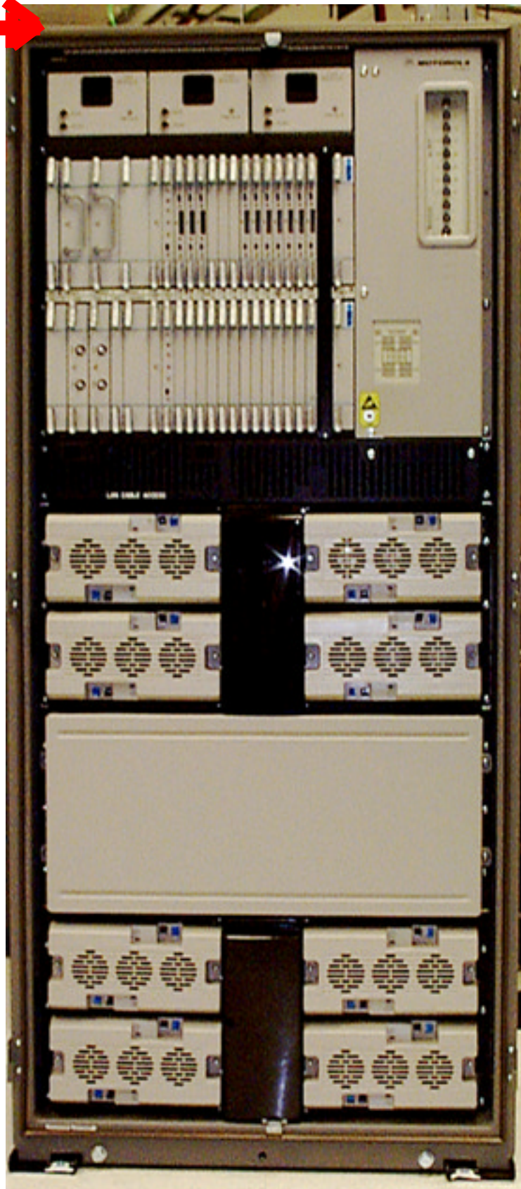
FCC Label Location IHET6BN1 SC4812T @ 1.9 GHz
