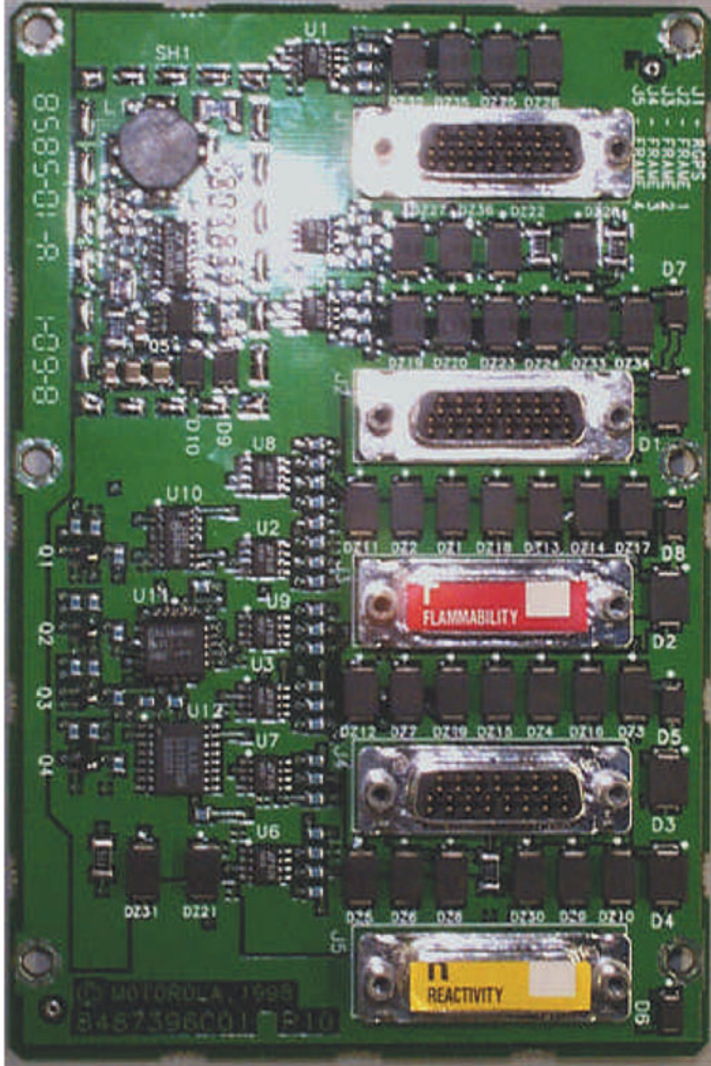
IJET6AP1 SC4812ET 1.9 GHz RGD Front
