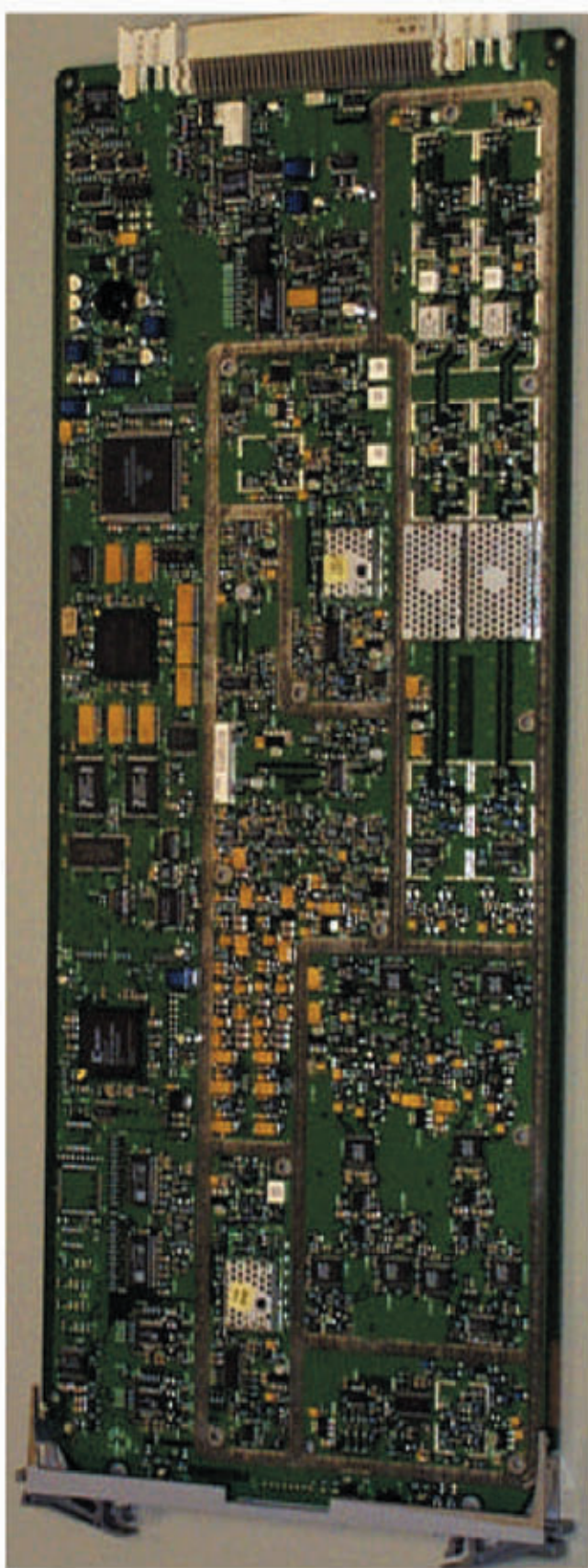
IHET6AP1 SC4812ET 1.9 GHz BBX2 without Cover
