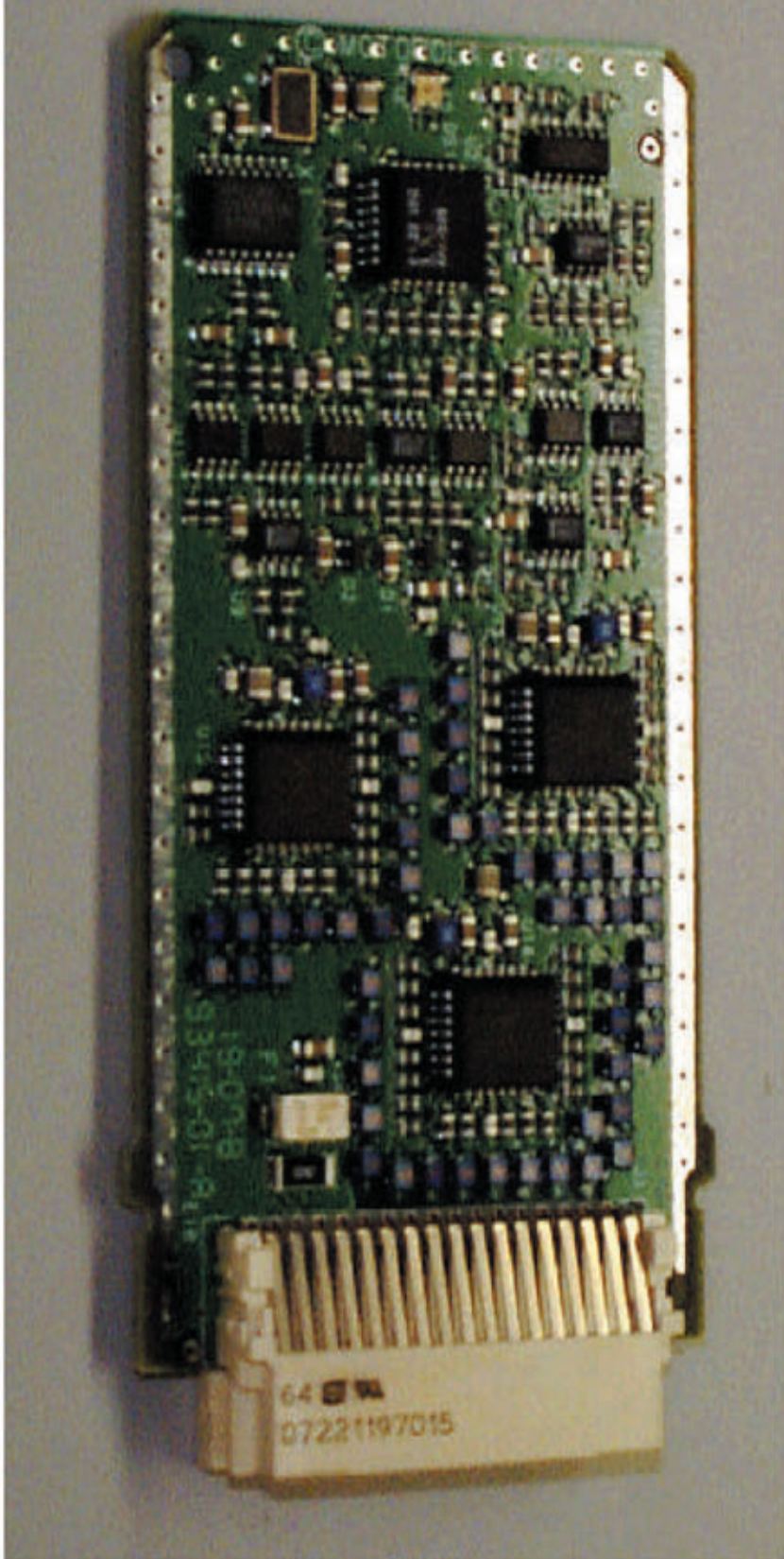
IHET6AP1 SC4812ET 1.9 GHz CCD Front
