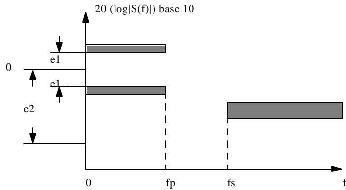
BASEBAND FILTERS FREQUENCY RESPONSE LIMITS
