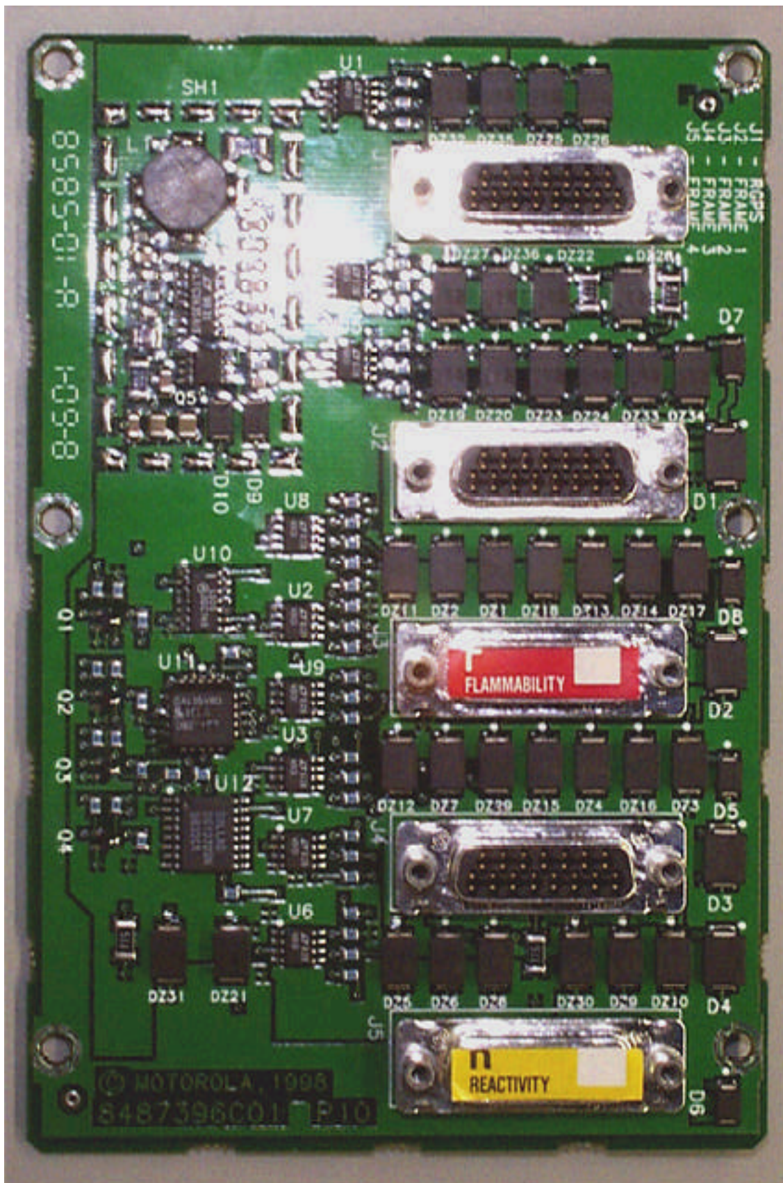
ITHET5ZR1 SC4812ET 800 MHz RGD Front
