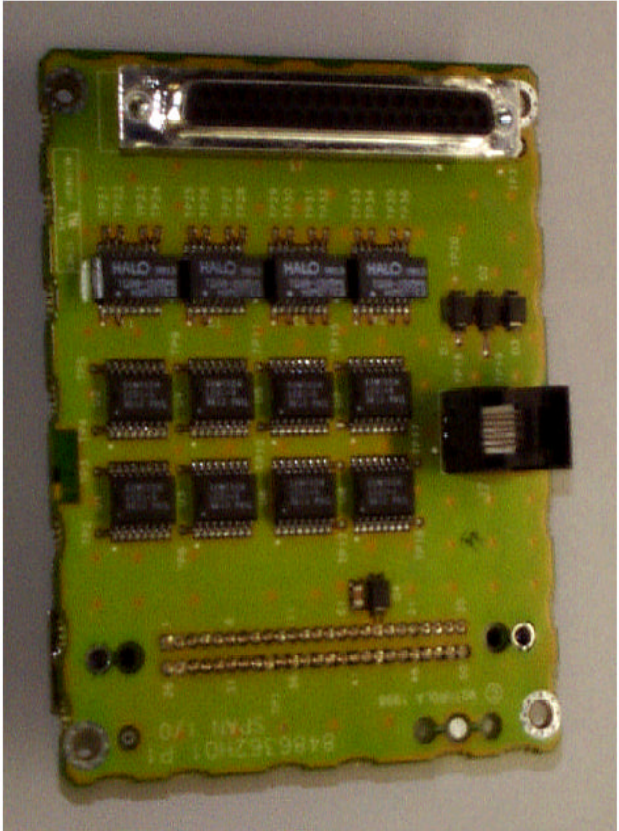
IHET5ZR1 SC4812ET 800 MHz Span I/O Back
