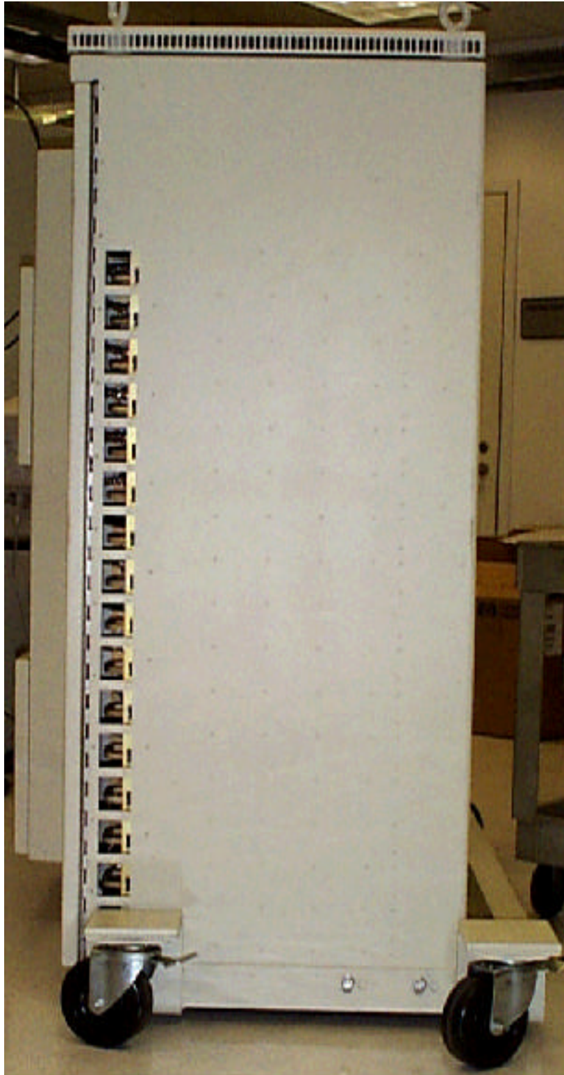
IHET5ZR1 SC4812ET 800 MHz Left Side View
