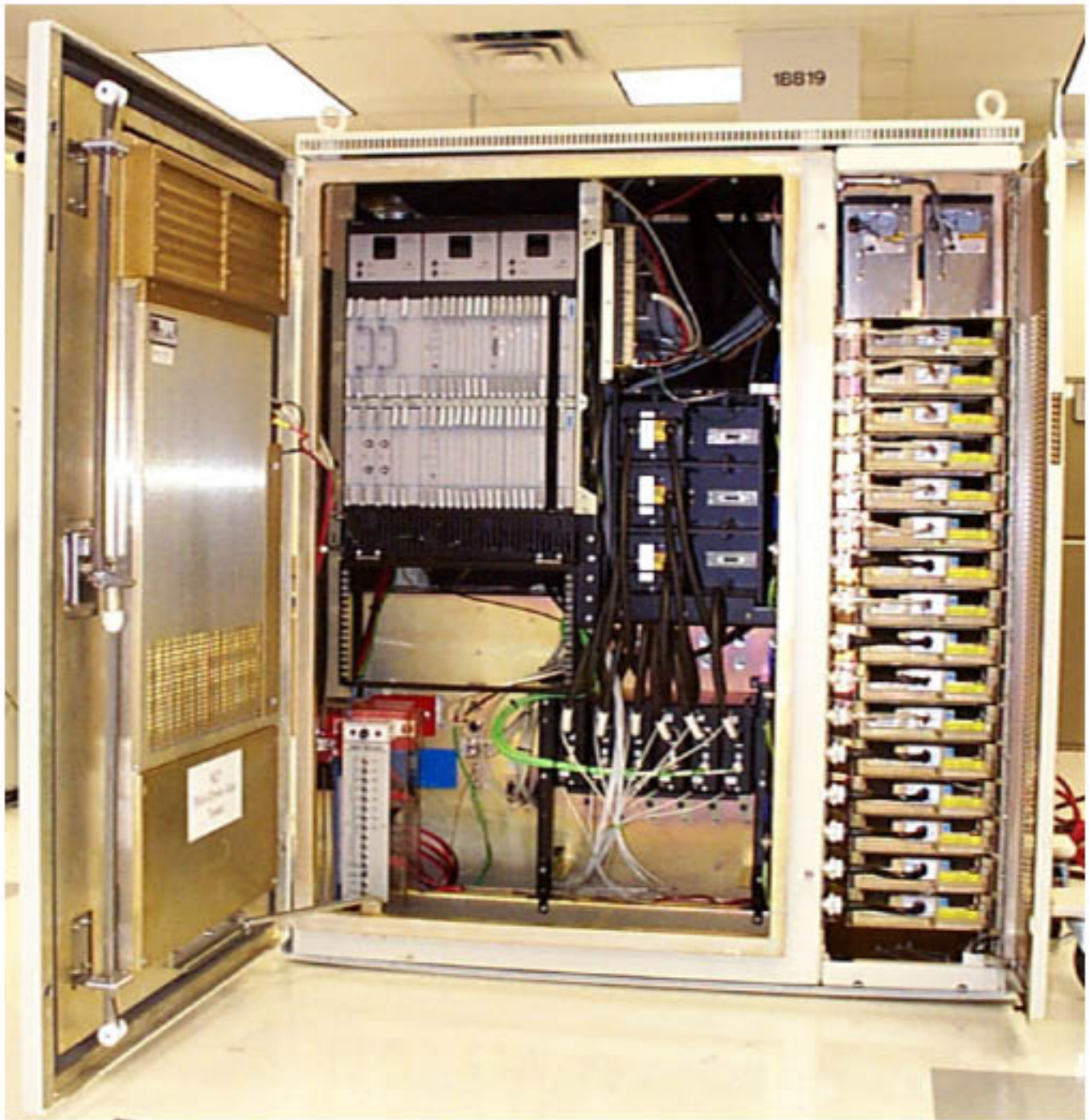
IHET5BQ1 SC4812ET @ 800 MHz Front View Doors Open
