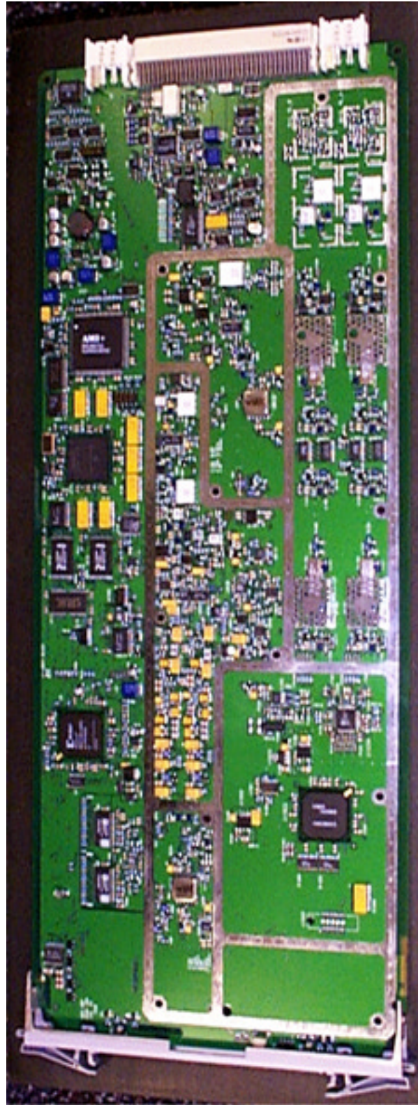
IHET5AW1 -48V SC4812T 800MHz DBPBBX Front without Cover
