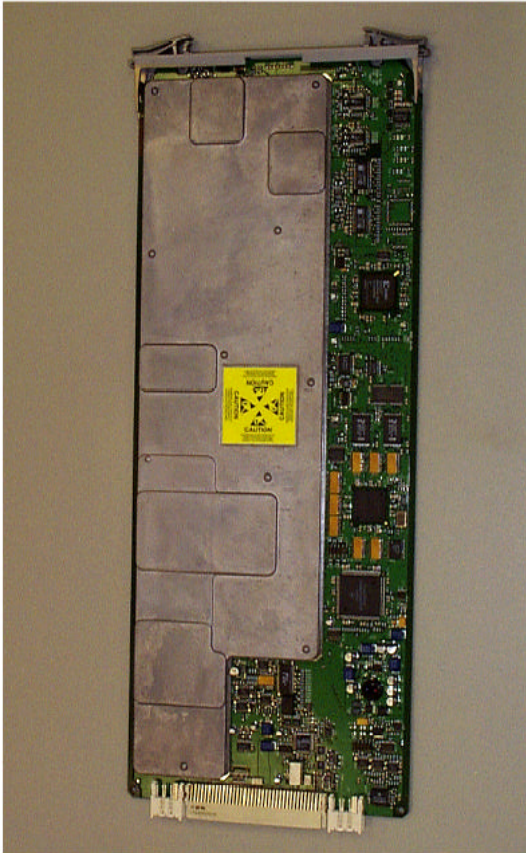
IHET5AW1 -48V SC4812T 800MHz BBX2 With Cover
