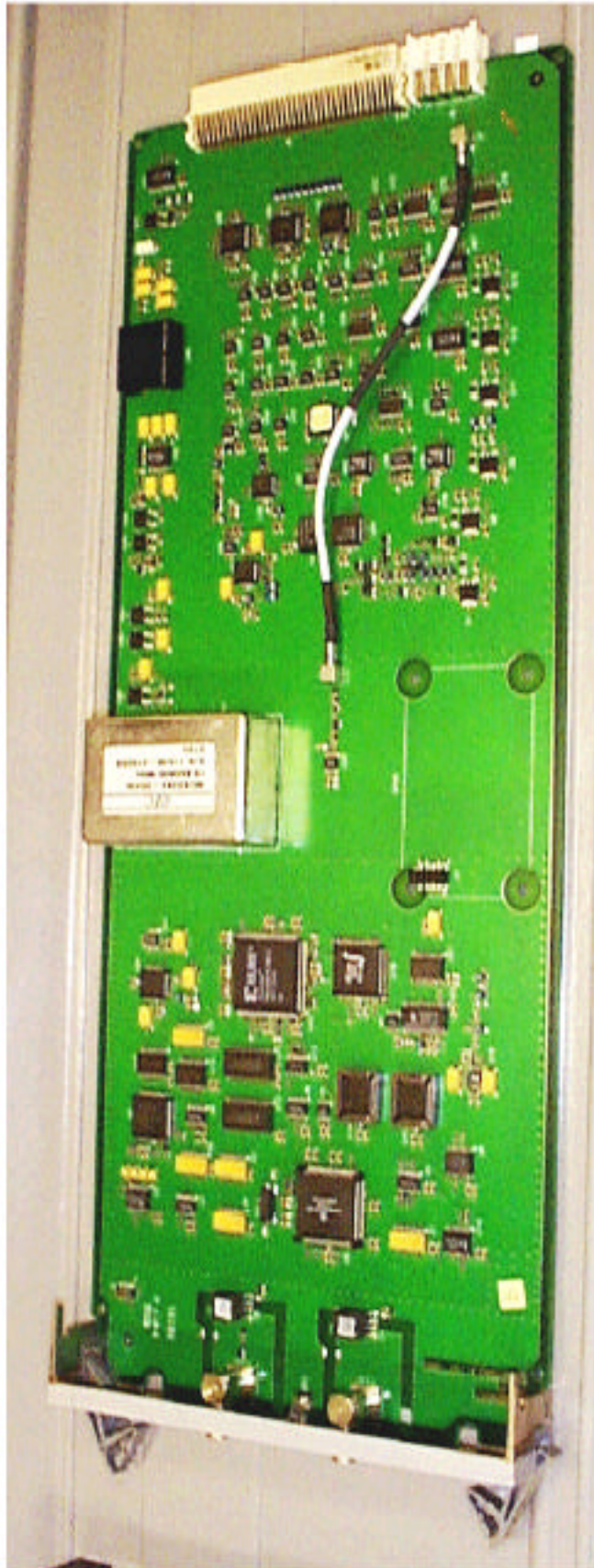
IHET5AW1 -48V SC4812T 800MHz CSM2 Front
