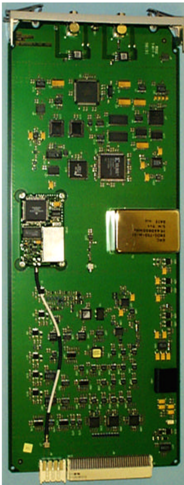
IHET5AW1 -48V SC4812T 800MHz CSM1 Front
