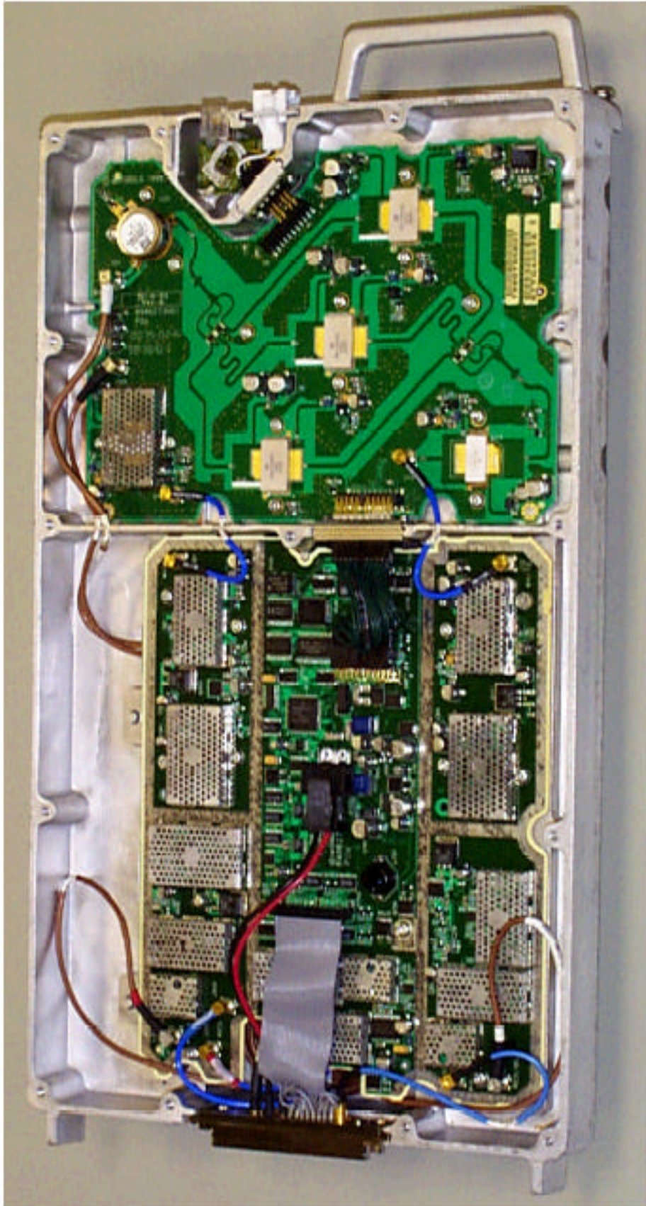
IHE5AW1 -48V SC4812T 800MHz LPA Without Cover
