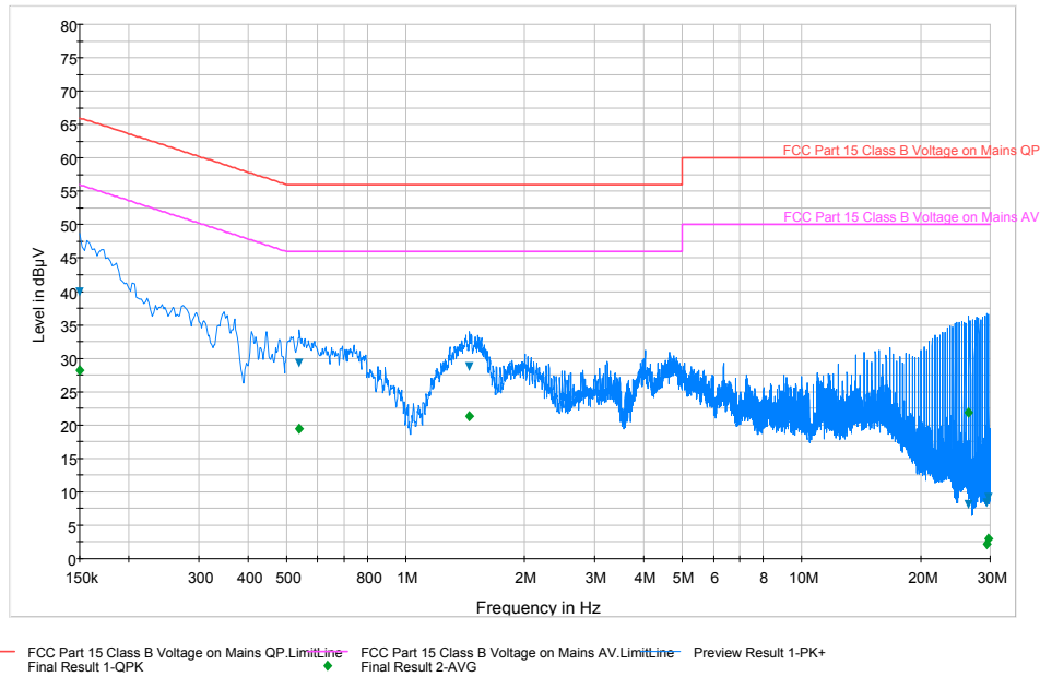
Plot 6-37. Line Conducted Plot with 802.11b (L1)
