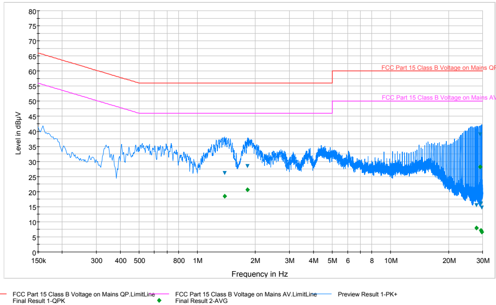
Plot 6-38. Line Conducted Plot with 802.11b (N)
