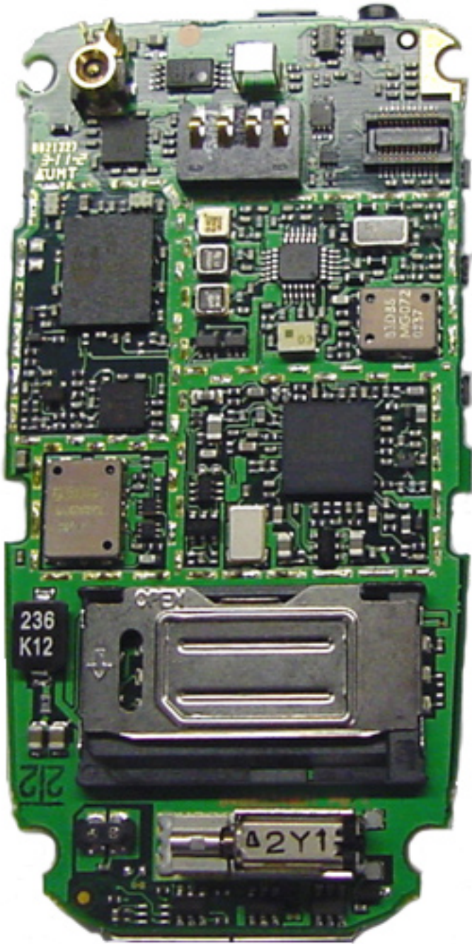
Rear View (Shields Removed)
