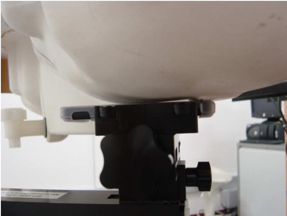
Figure 10. Phone with SYN1968A Soft Wrap Against the Head Phantom (Cheek Touch)
