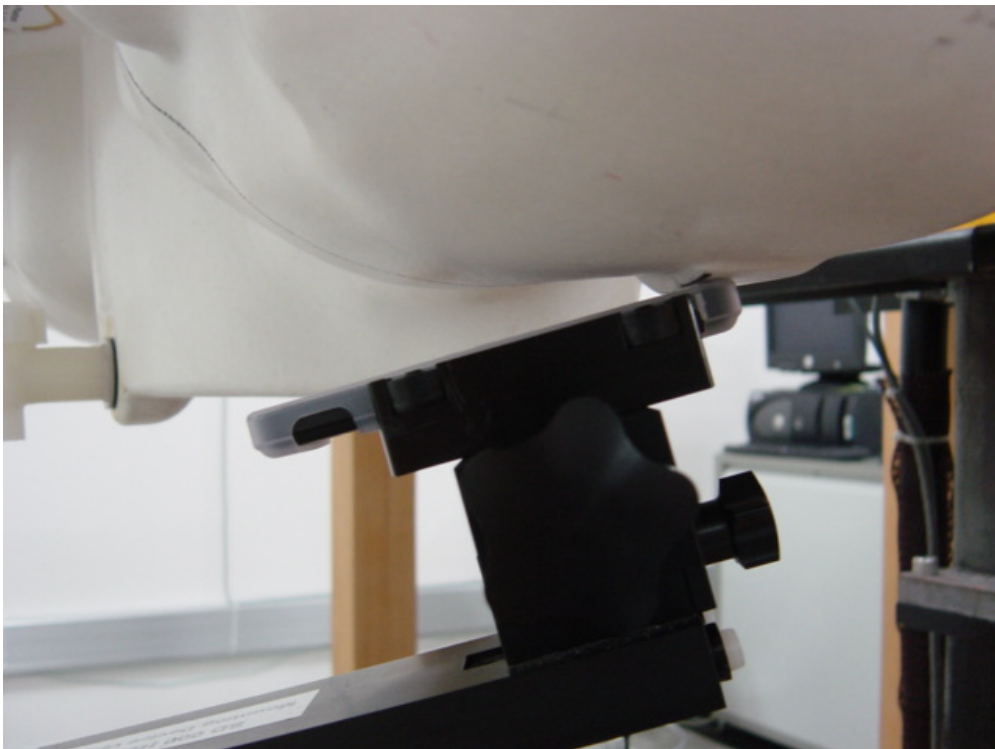
Figure 10. Phone with SYN1968A Soft Wrap Against the Head Phantom (15°Tilt)
