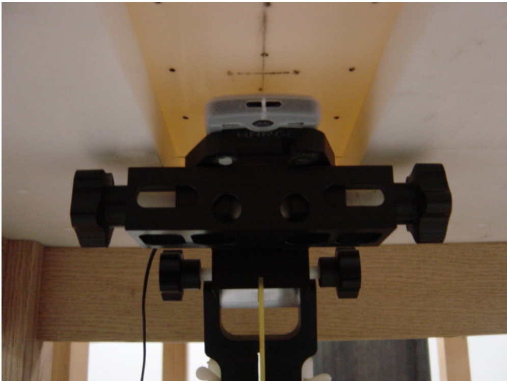
Figure 8: Phone with SYN1968A Soft Wrap Against the Flat Phantom
