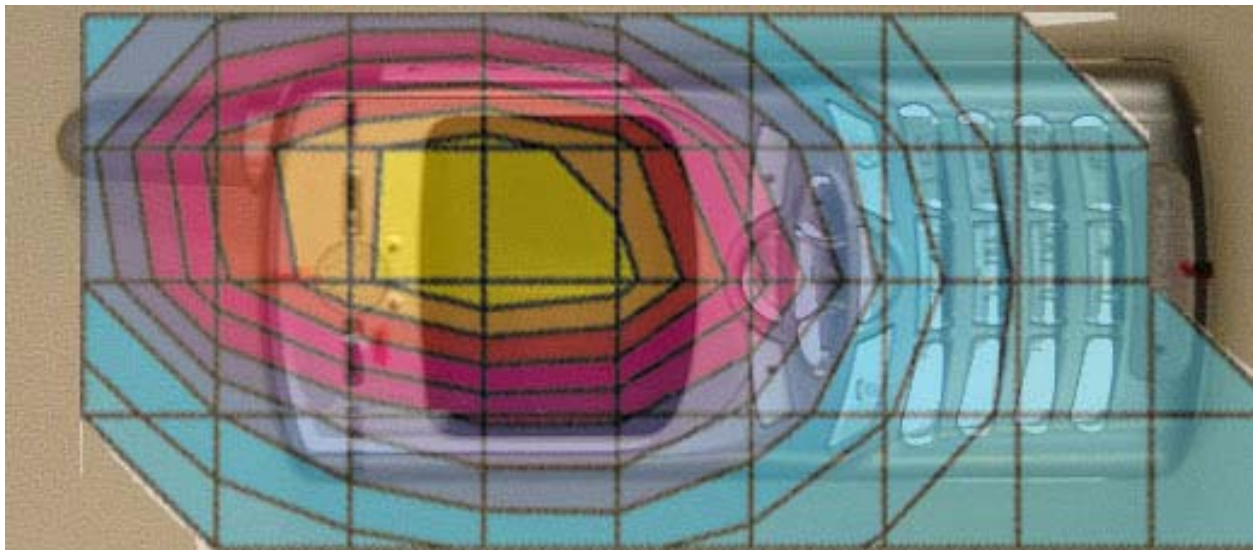
Figure 2. Typical 800MHz CDMA Head Adjacent Contour Overlaid on Phone (Cheek Touch)
