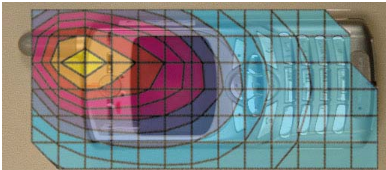
Figure 3. Typical 800MHz AMPS Head Adjacent Contour Overlaid on Phone (15 ° Tilt)
