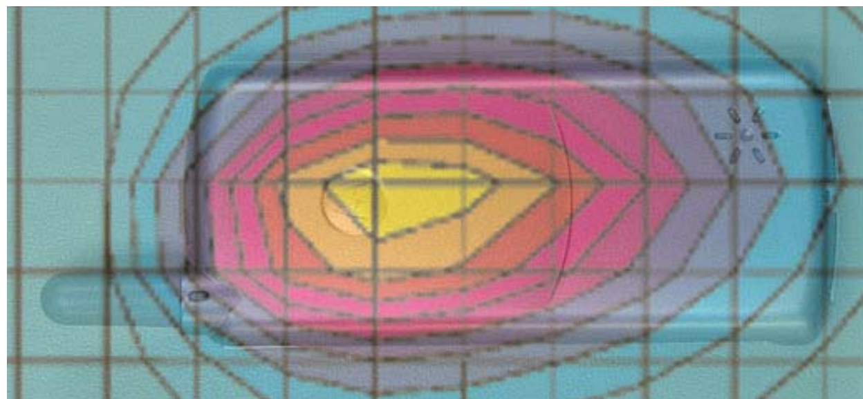
Figure 6. Typical 800 MHz CDMA Body-Worn Contour Overlaid on Phone
