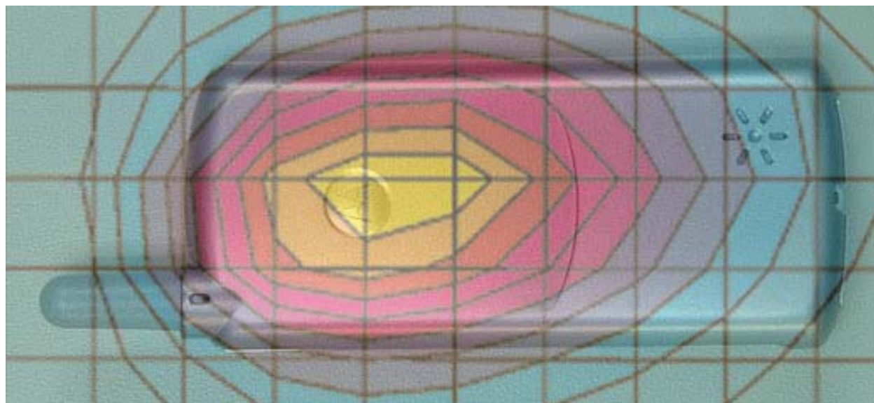
Figure 5. Typical 800 MHz AMPS Body-Worn Contour Overlaid on Phone
