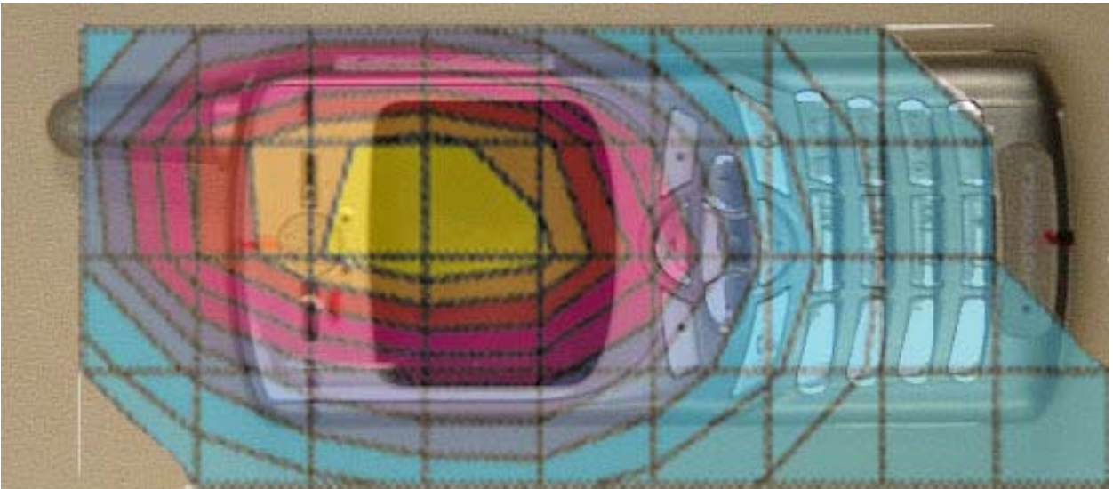
Figure 1. Typical 800MHz AMPS Head Adjacent Contour Overlaid on Phone (Cheek Touch)
