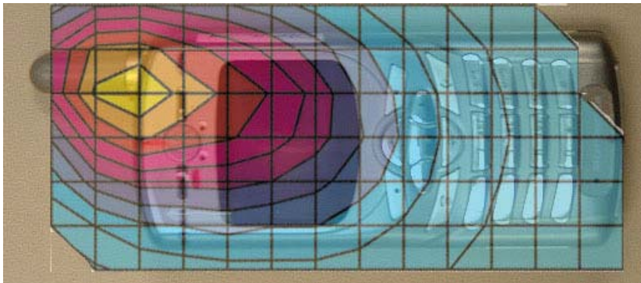
Figure 4. Typical 800MHz CDMA Head Adjacent Contour Overlaid on Phone (15 ° Tilt)
