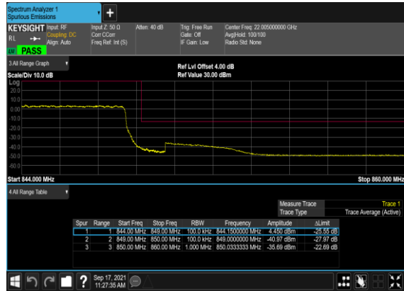
B7_N5(10M)_DFT-s- OFDM_BPSK_Outer_Full_High_CH
