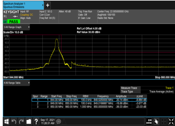
B7_N5(10M)_DFT-s- OFDM_BPSK_Edge_1RB_Right_High_CH
