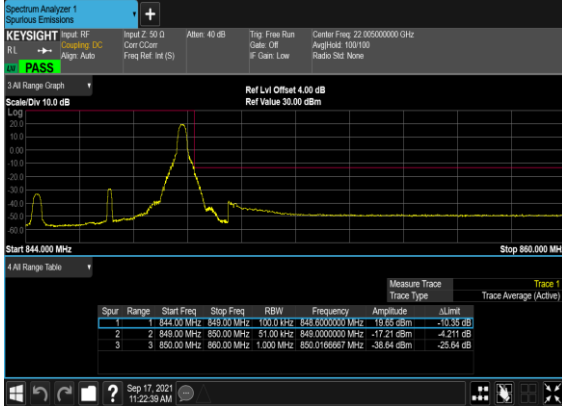
B7_N5(5M)_DFT-s-OFDM_QPSK_Edge_1RB_Right_High_CH
