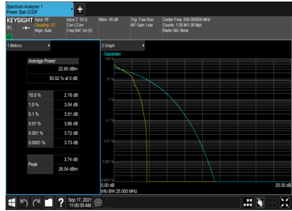
B7_N5(20M)_DFT-s-OFDM_PI_2-BPSK_Edge_1RB_Left_High_CH
