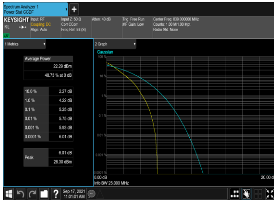
B7_N5(20M)_DFT-s-OFDM_QPSK_Outer_Full_High_CH
