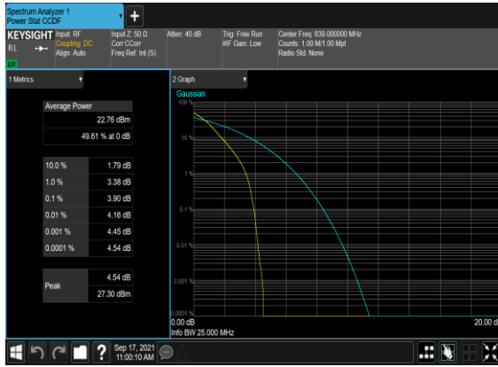
B7_N5(20M)_DFT-s-OFDM_PI_2-BPSK_Outer_Full_High_CH
