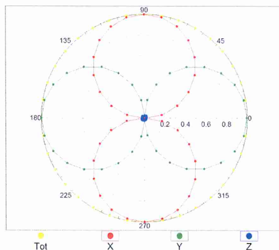
f=1800 MHz,R22,0°
