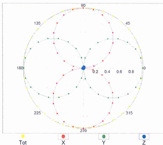
f=600 MHz,TEM,0°
