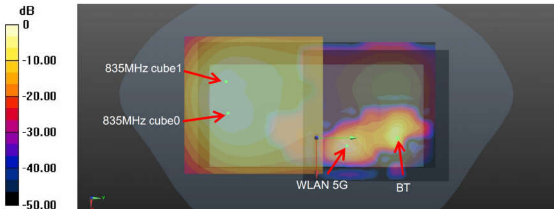
WWAN+WLAN5GHz+Bluetooth_Back 5mm
