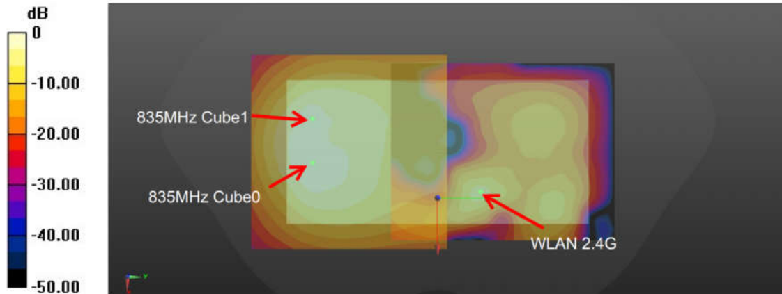
WWAN+WLAN2.4GHz_Back 5mm
