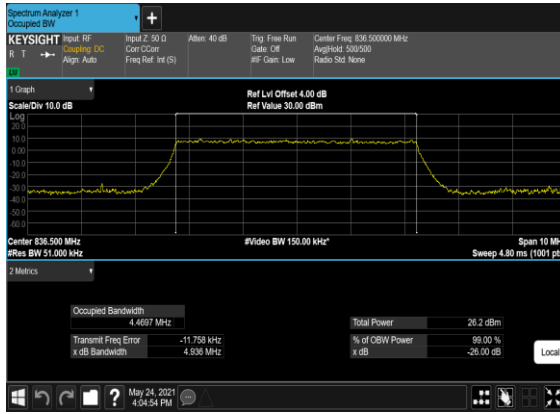
B7_N5(5M)_CP- OFDM_QPSK_Outer_Full_Mid_CH
