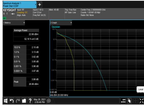
B66_N7(20M)_DFT-s-OFDM_PI_2-BPSK_Edge_1RB_Left_High_CH
