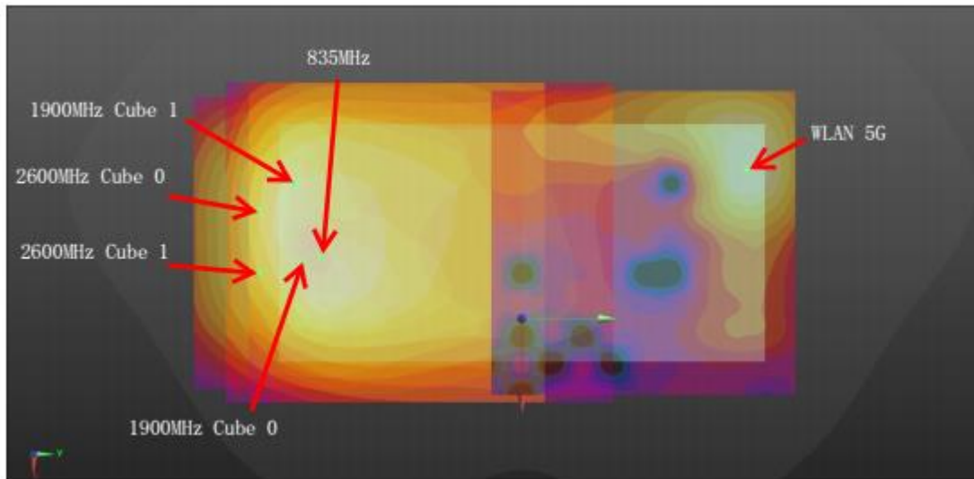
Back for WWAN+WLAN5GHz_5mm
