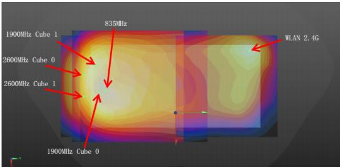
Back for WWAN+WLAN2.4GHz _5mm
