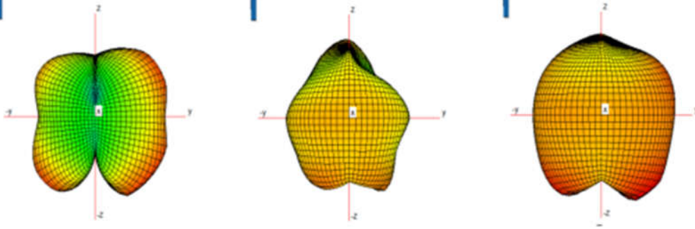
ANT3-WIFI 5G CH1 5500MHz
